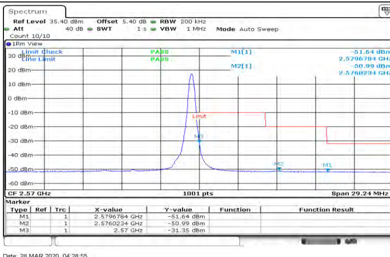
Band7-10MHz-64QAM-21400-50RB#0
