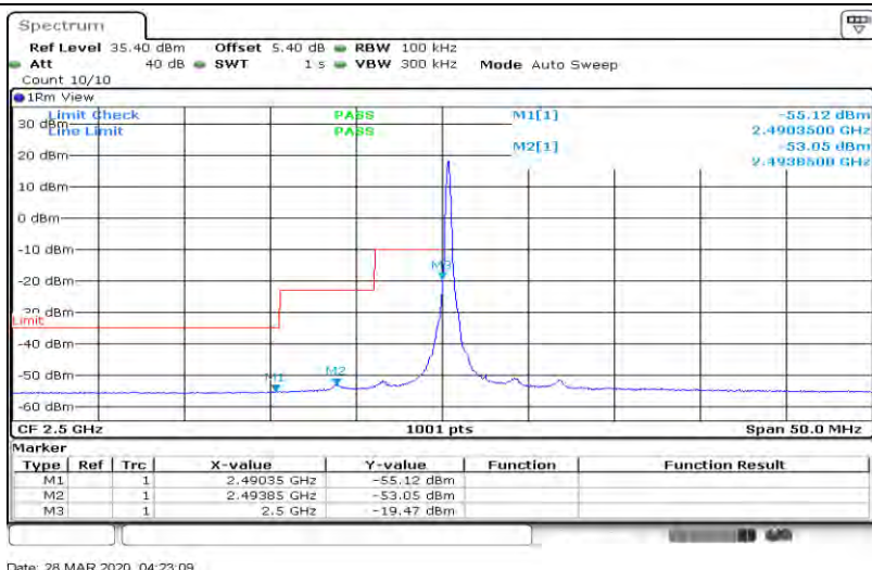
Band7-5MHz-16QAM-20775-25RB#0
