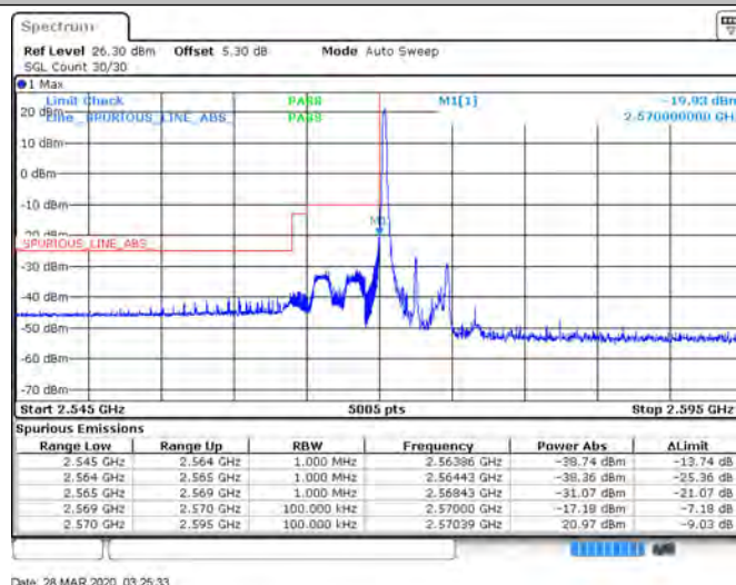
Band38_5MHz_QPSK_37775_25RB#0
