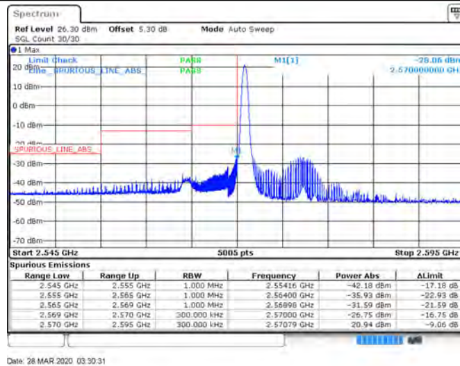
Band38_15MHz_64QAM_37825_75RB#0
