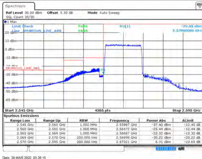
Band38_10MHz_16QAM_38200_1RB#49
