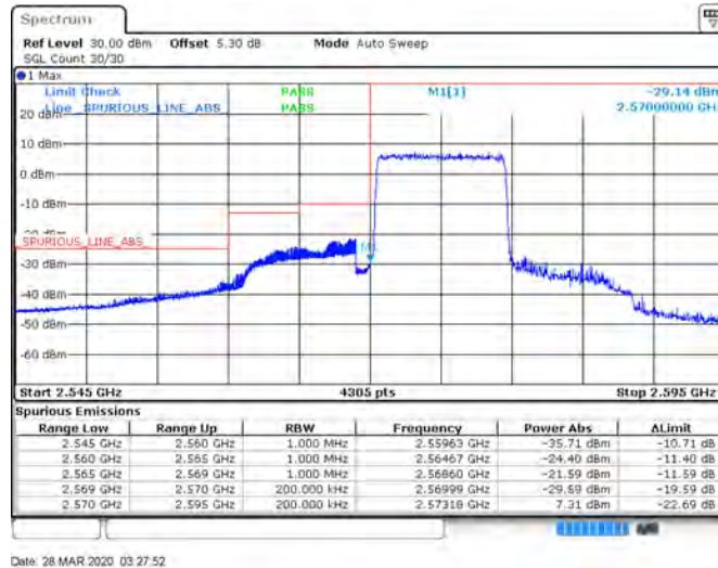
Band38_10MHz_QPSK_38200_1RB#49
