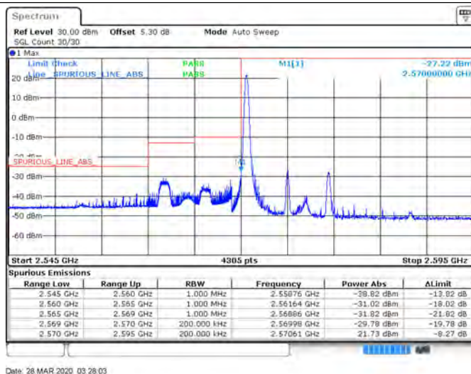
Band38_10MHz_16QAM_37800_50RB#0
