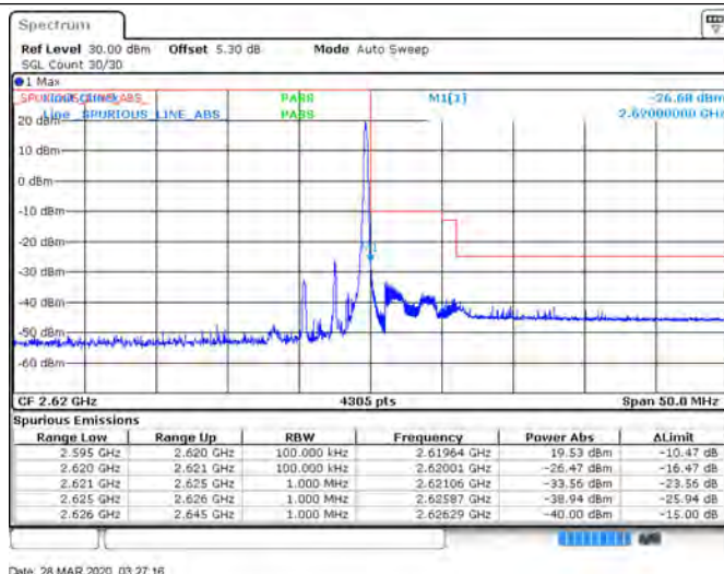
Band38_5MHz_64QAM_38225_25RB#0
