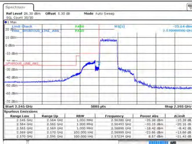
Band38_5MHz_QPSK_37775_25RB#0
