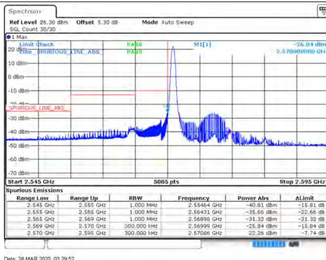
Band38_15MHz_QPSK_37825_75RB#0
