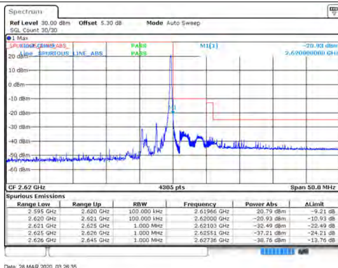
Band38_5MHz_QPSK_38225_25RB#0
