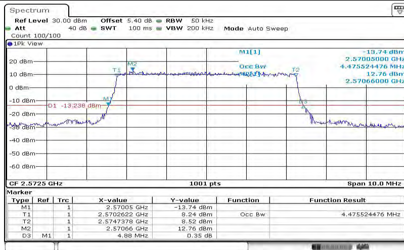
Band38-5MHz-QPSK-37775-25RB#0-4.476
