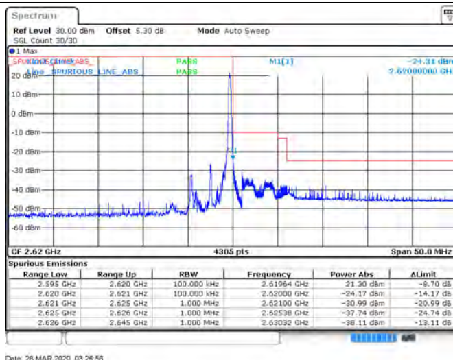
Band38_5MHz_16QAM_38225_25RB#0
