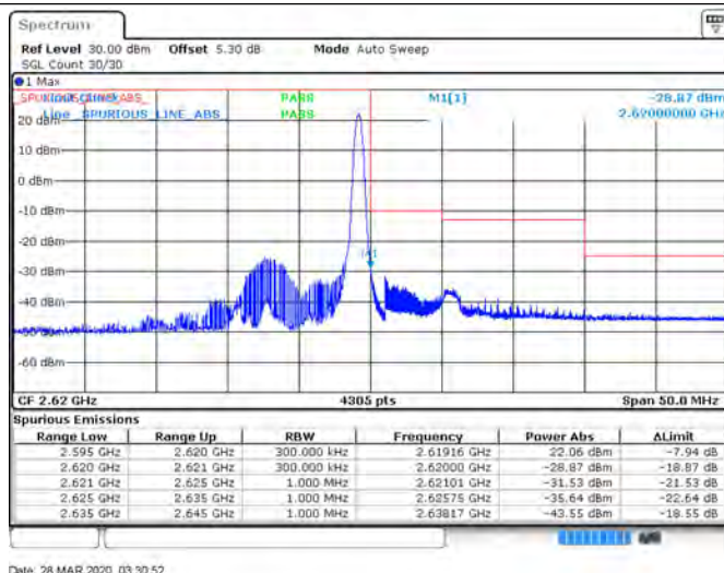
Band38_15MHz_QPSK_38175_75RB#0
