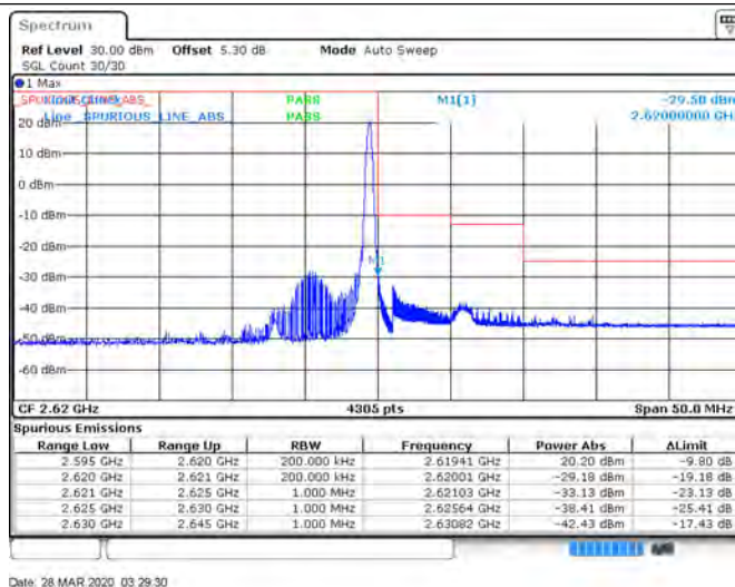
Band38_10MHz_64QAM_38200_50RB#0
