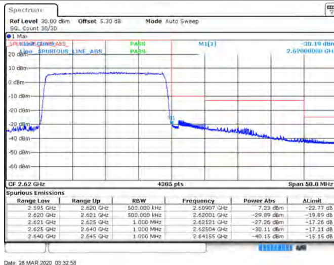
Band38_20MHz_64QAM_37850_1RB#0
