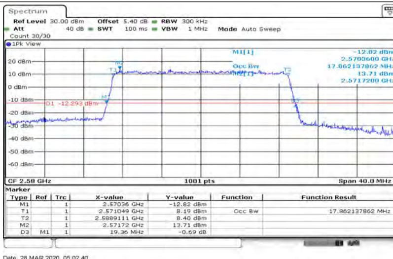
Band38-20MHz-64QAM-38000-100RB#0-17.862
