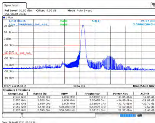
Band38_20MHz_64QAM_37850_100RB#0
