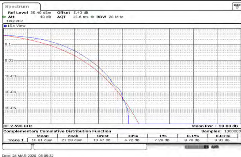
Band38-20MHz-64QAM-38150-100RB#0
