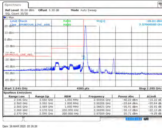
Band38_10MHz_64QAM_37800_50RB#0
