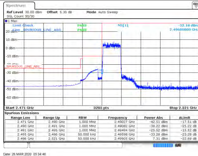
Band41_5MHz_64QAM_41565_1RB#24
