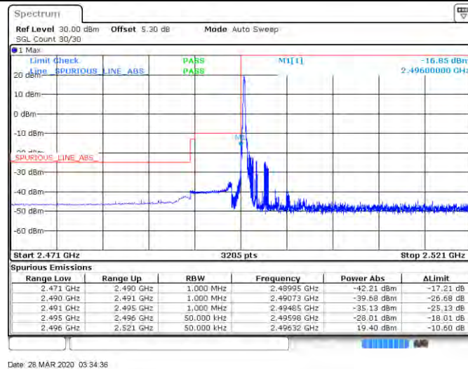
Band41_5MHz_64QAM_39675_25RB#0
