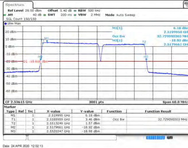
CA 7C 20+15 64QAM 21201+21372 100RB#0+75RB#0
