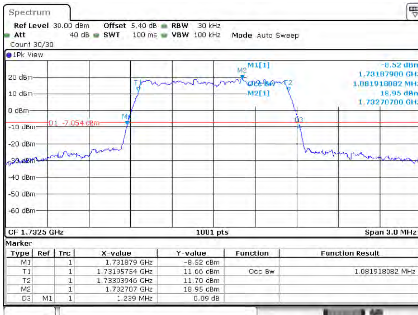
Band4-1.4MHz-QPSK-20175-6RB#0-1.082
