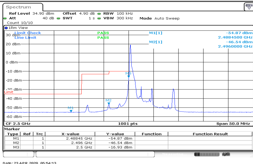
Band7-5MHz-QPSK-20775-25RB#0
