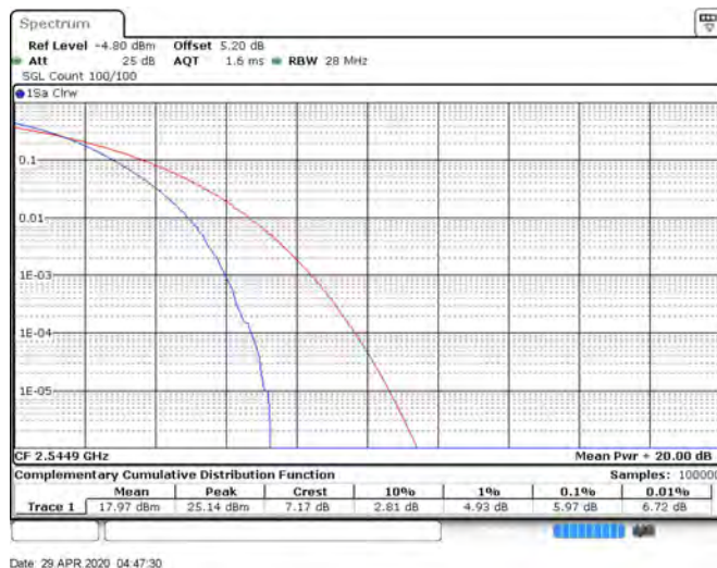
CA_7C_100RB+100RB_QPSK_21350+21152_100RB#0+100RB#0
