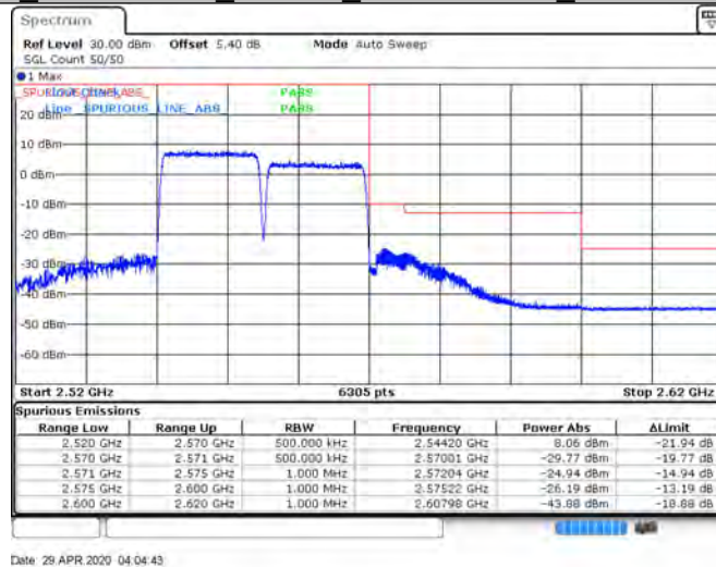
CA 7C 100RB+100RB QPSK 20850+21048 1RB#0+0RB#0
