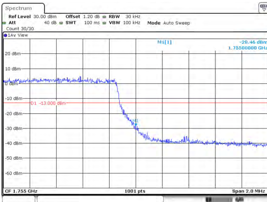
Band4-3MHz-QPSK-20385-15RB#0
