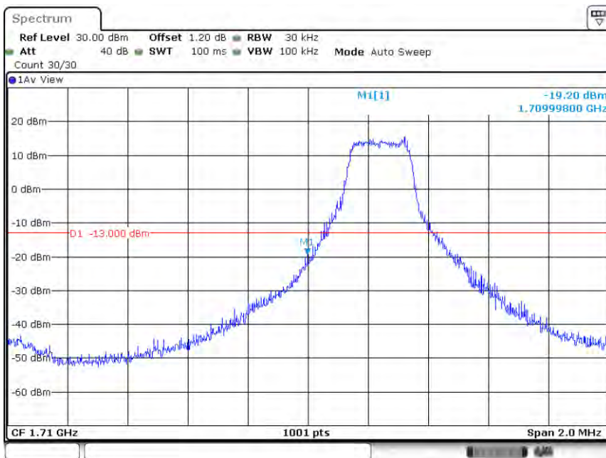
Band4-3MHz-16QAM-19965-1RB#0
