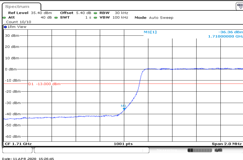
Band4-3MHz-64QAM-20385-1RB#14
