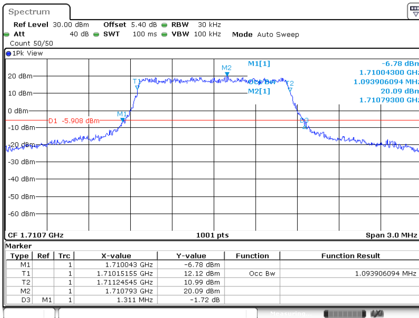
Band66-1.4MHz-QPSK-131979-6RB#0-1.094
