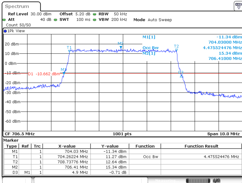
Band17-5MHz-QPSK-23755-25RB#0-4.476
