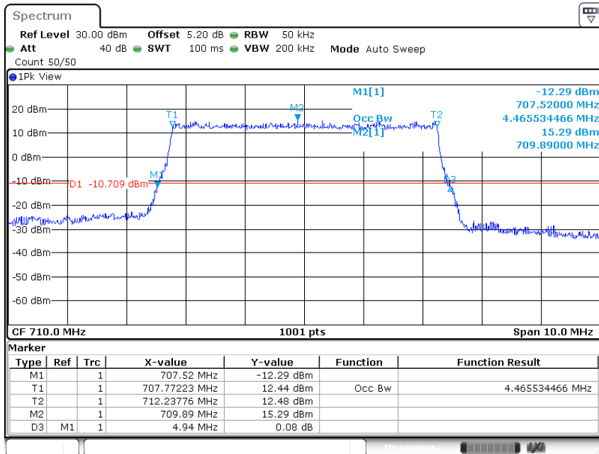
Band17-5MHz-QPSK-23790-25RB#0-4.466
