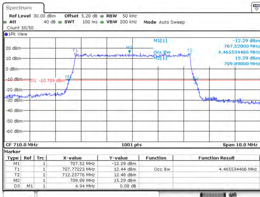
Band17-5MHz-QPSK-23790-25RB#0-4.466
