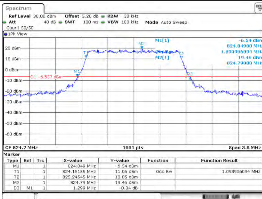
Band5-1.4MHz-QPSK-20407-6RB#0-1.094
