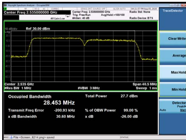
CA-7C 64QAM 15+15MHz CH- High
