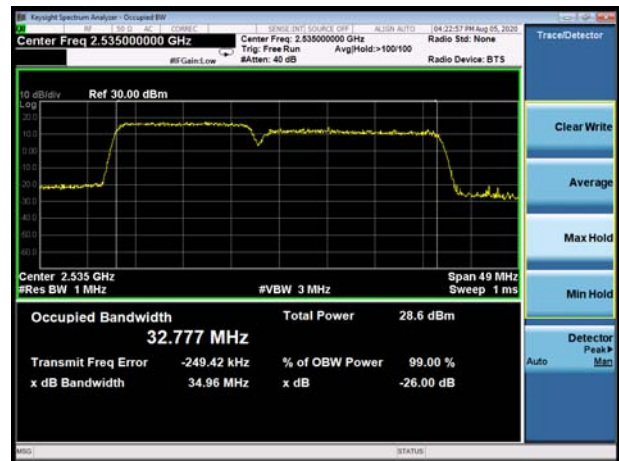
CA-7C 16QAM 15+20MHz CH- Middle
