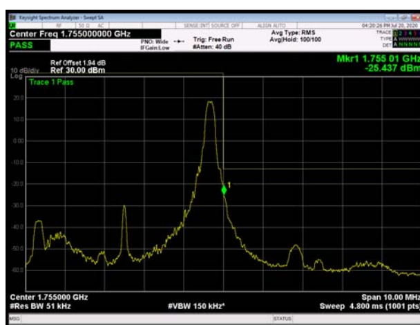
LTE Band 4 QPSK 5MHz CH-High, 100%RB
