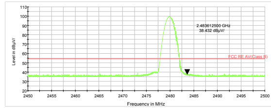
DH5-Channel 78: Average
