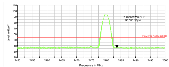
3DH5-Channel 78: Average
