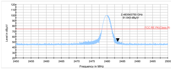
DH5-Channel 78: Peak
