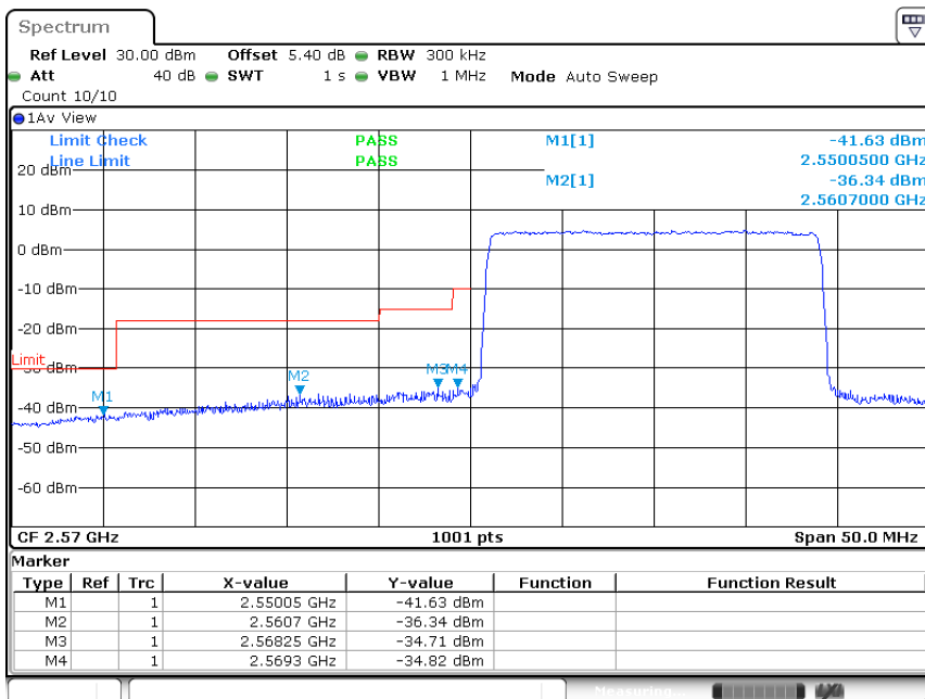
Band38-20MHz-16QAM-37850-100RB#0
