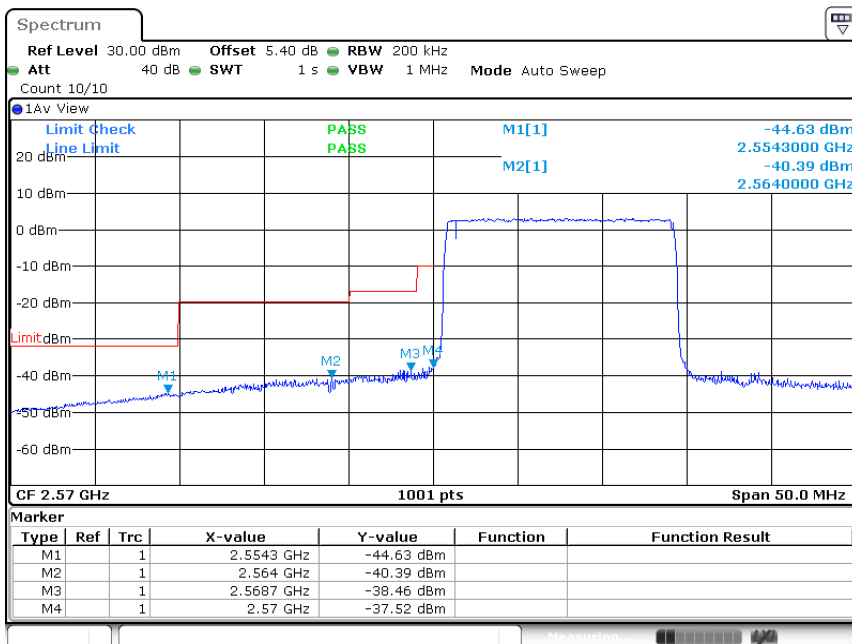
Band38-15MHz-64QAM-37825-75RB#0
