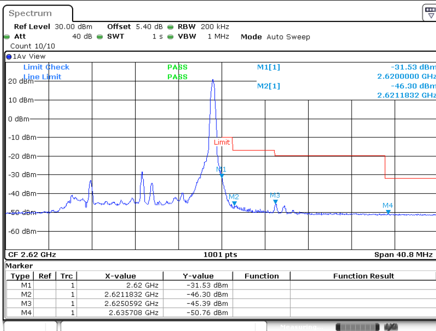
Band38-15MHz-64QAM-38175-1RB#74
