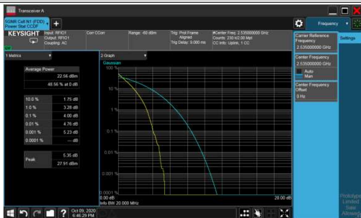
N7-20MHz-15KHz-TM1-507000-Outer Full
