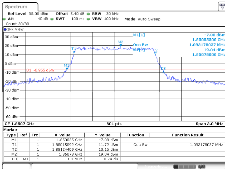
Band2-1.4MHz-QPSK-18607-6RB#0-1.093
