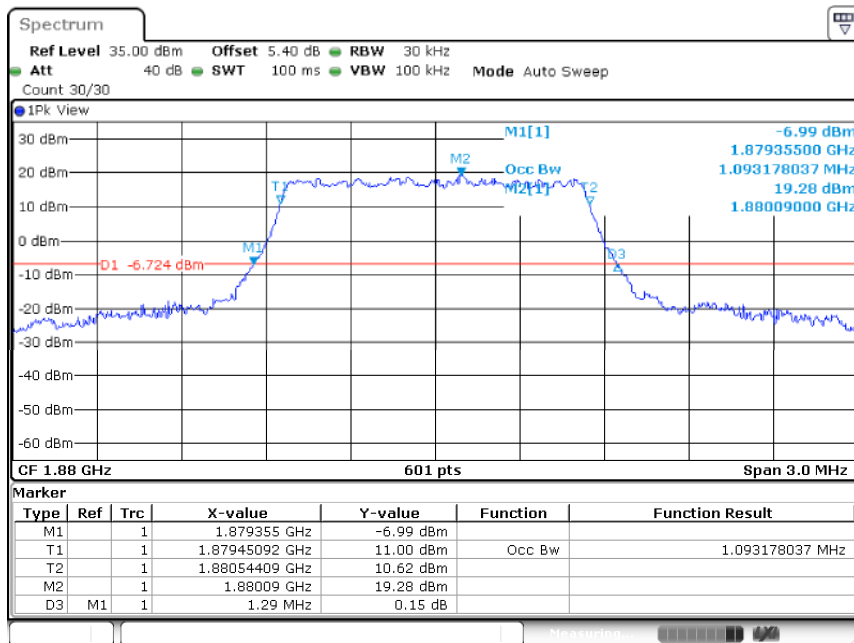
Band2-1.4MHz-QPSK-18900-6RB#0-1.093
