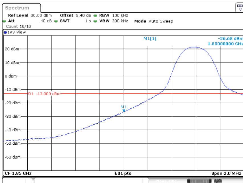
Band2-10MHz-16QAM-18650-1RB#0
