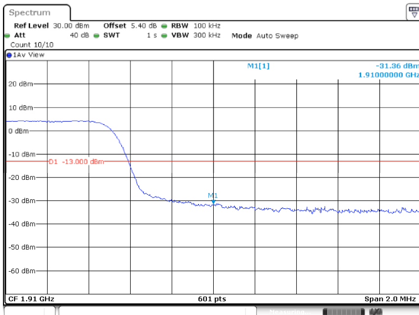
Band2-10MHz-QPSK-19150-50RB#0
