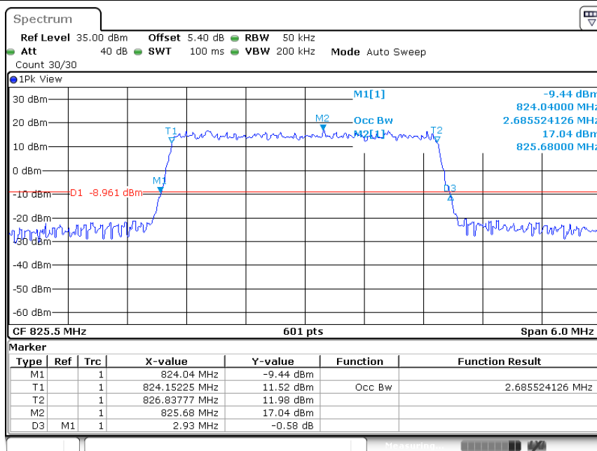
Band5-3MHz-16QAM-20415-15RB#0-2.686
