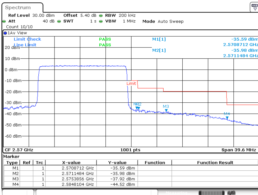
Band7-15MHz-16QAM-21375-75RB#0
