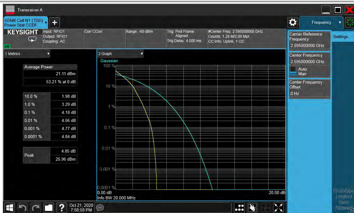
N38-20MHz-15KHz-TM1-519000-Outer Full
