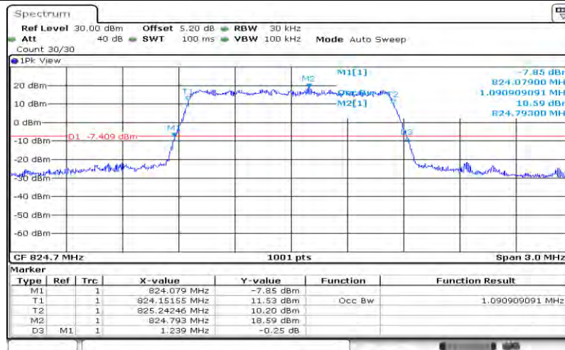
Band26-1.4MHz-QPSK-26797-6RB#0-1.091
