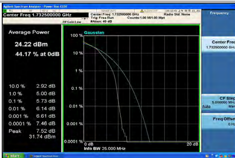
Band4-20MHz-64QAM-20300-100RB#0
