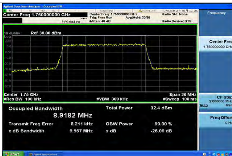
Band4-10MHz-16QAM-20000-50RB#0-8.9255
