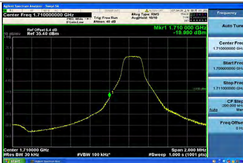
Band4-3MHz-64QAM-19965-15RB#0
