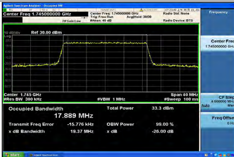
Band4-20MHz-16QAM-20300-100RB#0-17.889
