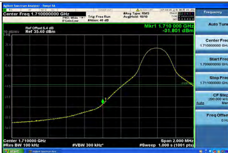
Band4-10MHz-64QAM-20000-50RB#0
