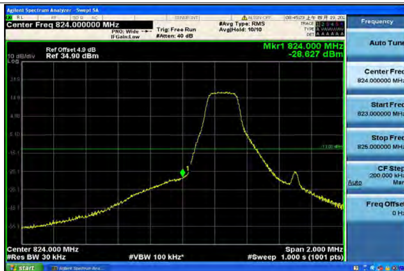
Band5-1.4MHz-64QAM-20407-6RB#0
