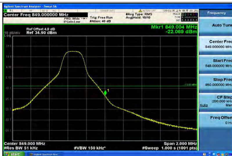
Band5-5MHz-64QAM-20625-25RB#0
