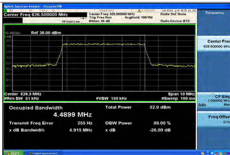
Band5-5MHz-16QAM-20525-25RB#0-4.4834
