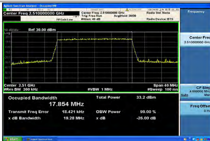
Band7-20MHz-16QAM-21100-100RB#0-17.855
