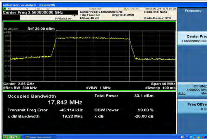
Band7-20MHz-16QAM-21350-100RB#0-17.842
