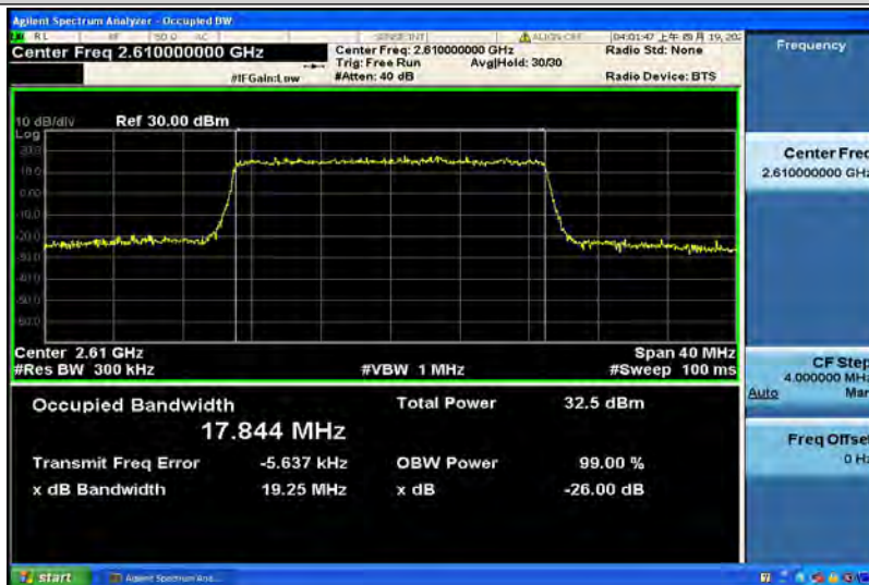
Band38-20MHz-16QAM-38150-100RB#0-17.844
