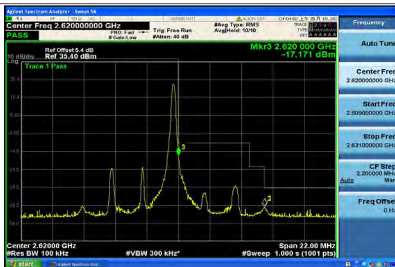
Band38-5MHz-16QAM-38225-25RB#0
