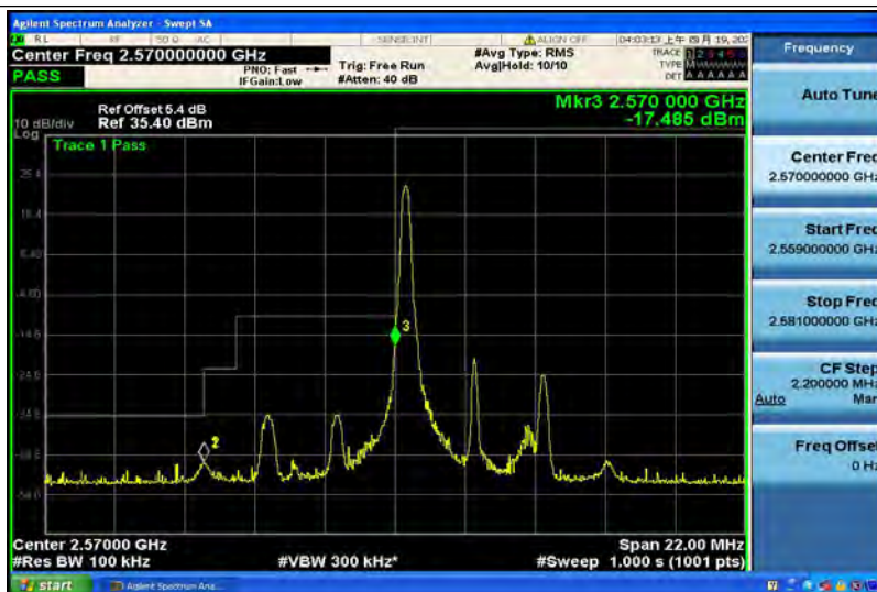
Band38-5MHz-64QAM-37775-25RB#0
