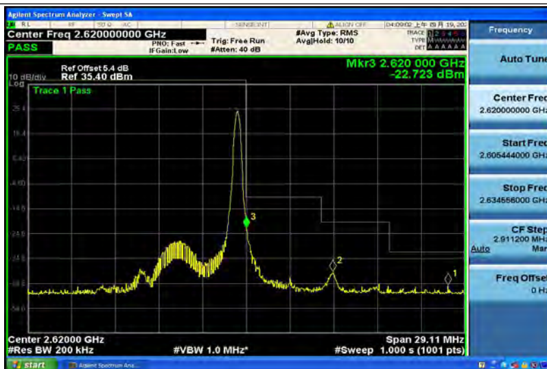
Band38-10MHz-64QAM-38200-50RB#0
