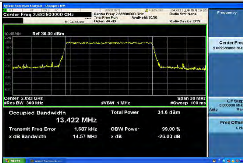
Band41-15MHz-16QAM-39725-75RB#0-13.430
