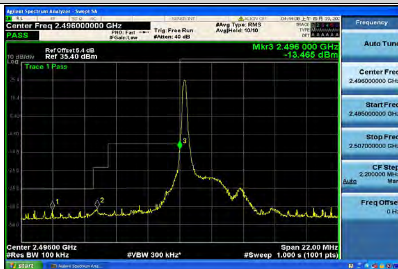
Band41-5MHz-QPSK-39675-25RB#0
