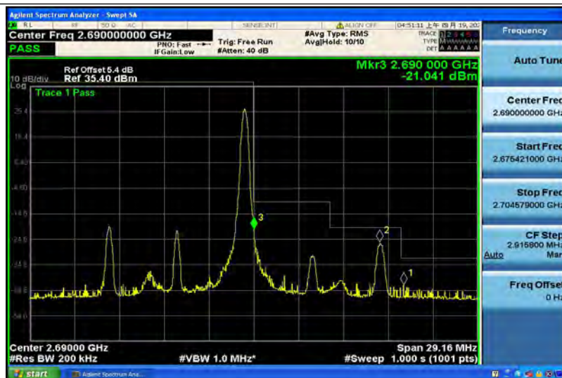
Band41-10MHz-64QAM-41540-50RB#0
