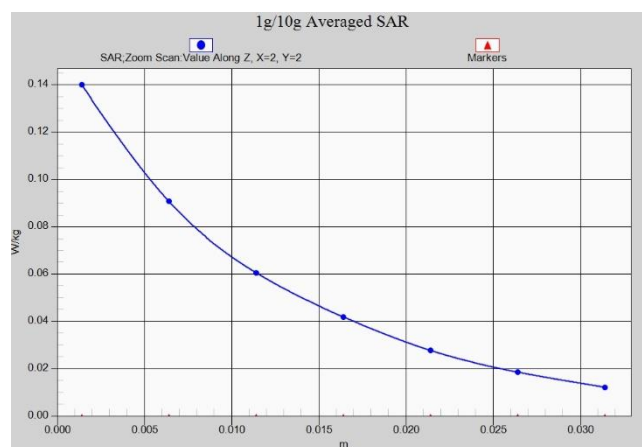
Fig. 1-32 Z-Scan at power reference point (LTE Band2)
