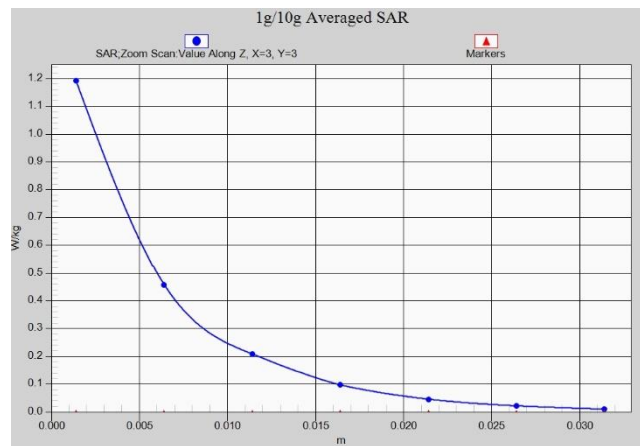
Fig. 1-46 Z-Scan at power reference point (2450 MHz)
