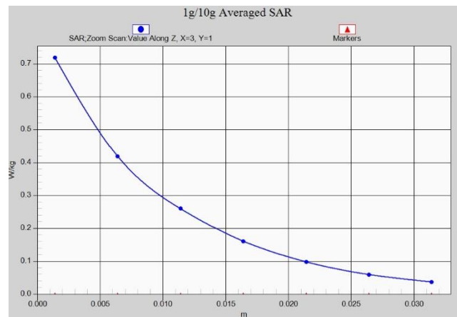
Fig. 1-37 Z-Scan at power reference point (LTE Band4)
