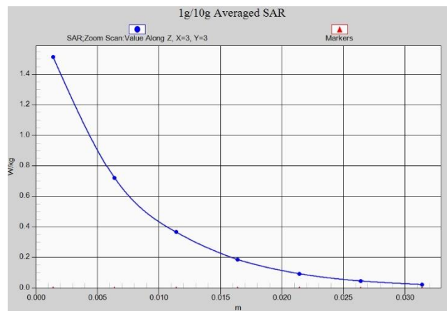
Fig. 1-47 Z-Scan at power reference point (2450 MHz)
