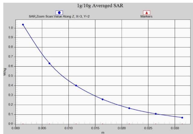
Fig. 1-29 Z-Scan at power reference point (WCDMA1700)
