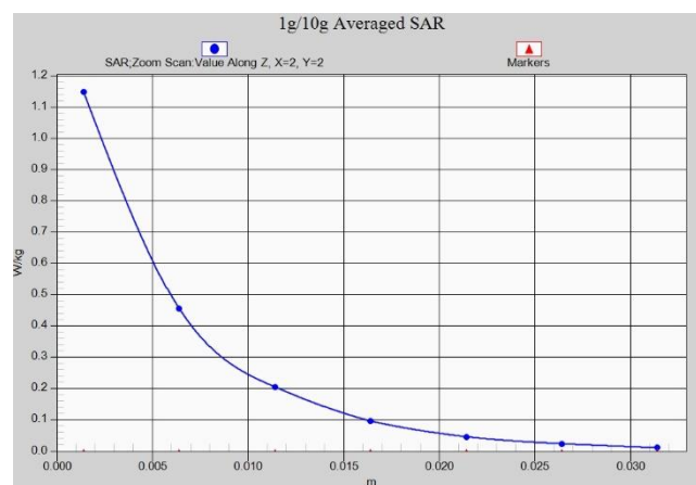
Fig. 1-50 Z-Scan at power reference point (BT)
