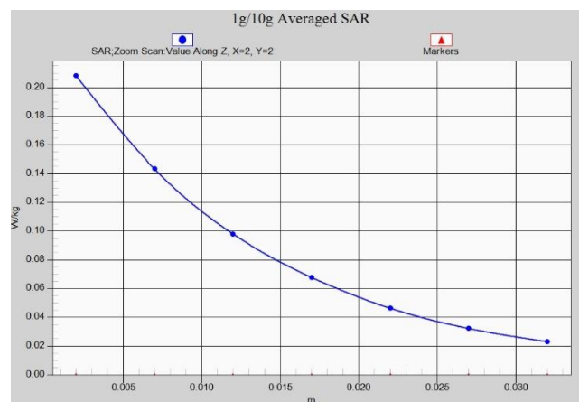
Fig. 1-24 Z-Scan at power reference point (WCDMA1900)
