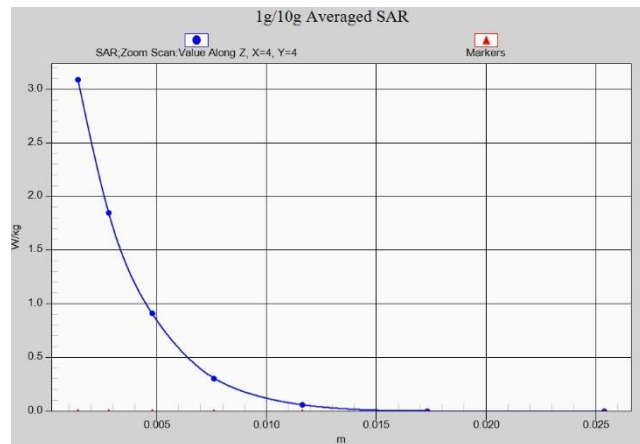
Fig. 1-48 Z-Scan at power reference point (5 GHz)
