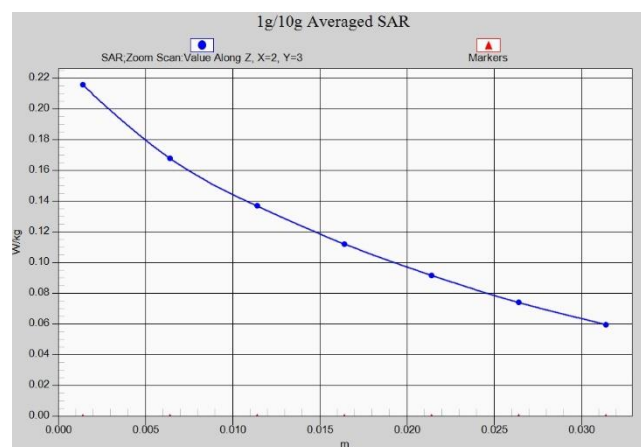
Fig. 1-38 Z-Scan at power reference point (LTE Band5)
