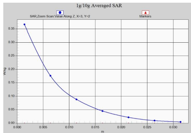
Fig. 1-45 Z-Scan at power reference point (LTE Band38)
