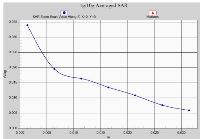
Fig. 1-25 Z-Scan at power reference point (WCDMA1900)
