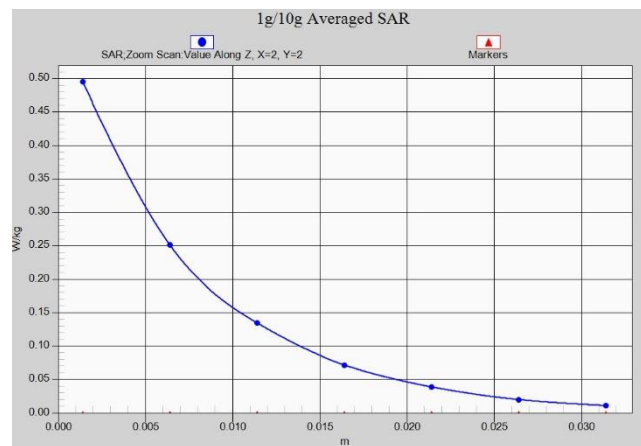
Fig. 1-51 Z-Scan at power reference point (BT)
