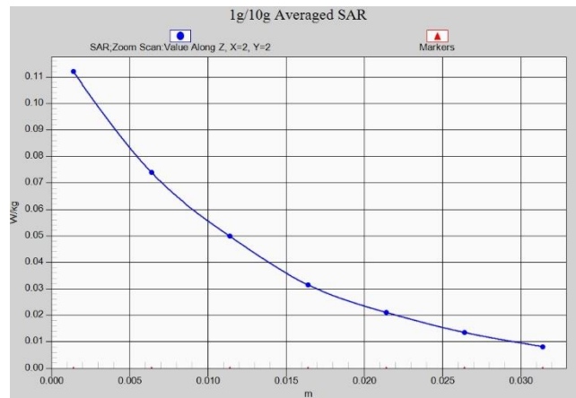
Fig. 1-21 Z-Scan at power reference point (PCS1900)
