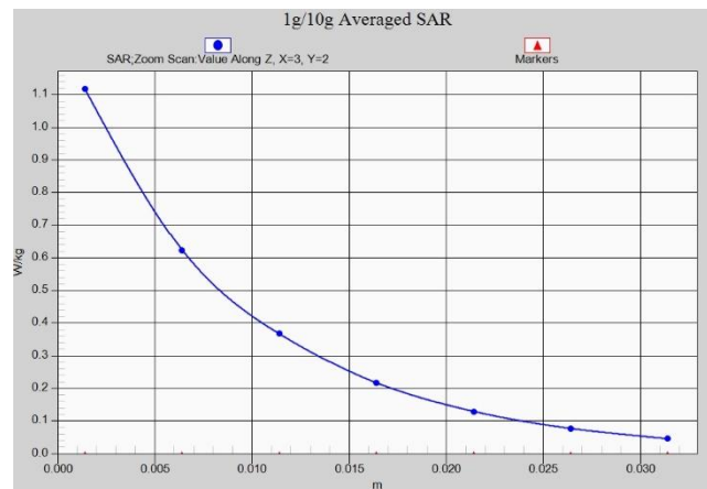
Fig. 1-22 Z-Scan at power reference point (PCS1900)
