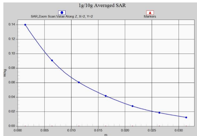
Fig. 1-43 Z-Scan at power reference point (LTE Band38)
