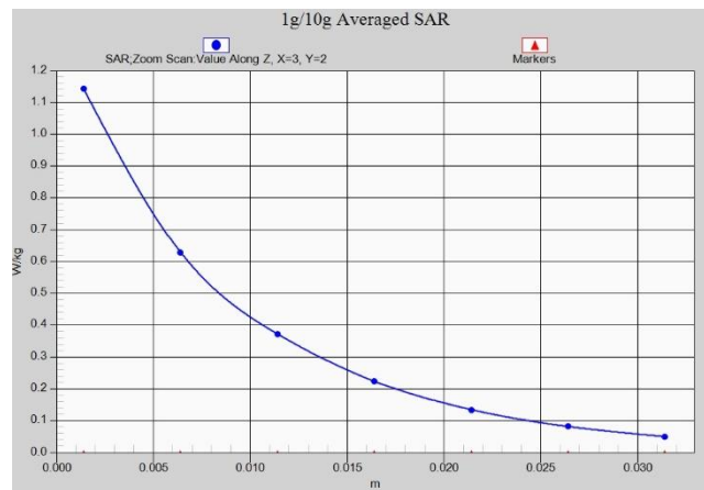
Fig. 1-28 Z-Scan at power reference point (WCDMA1700)
