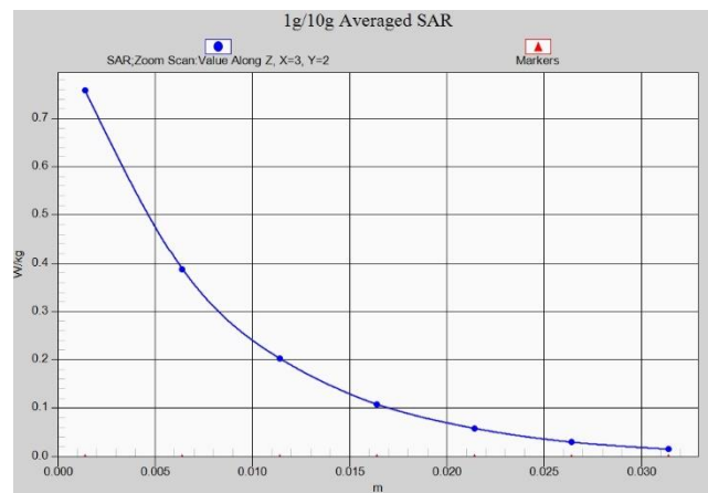
Fig. 1-42 Z-Scan at power reference point (LTE Band 7)
