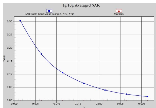
Fig. 1-23 Z-Scan at power reference point (PCS1900)
