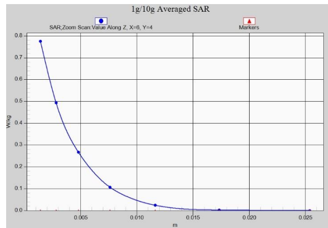
Fig. 1-49 Z-Scan at power reference point (5 GHz)
