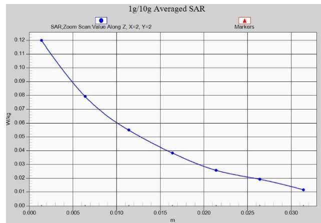
Fig. 1-40 Z-Scan at power reference point (LTE Band 7)
