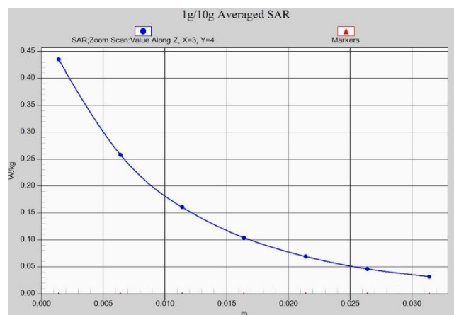
Fig. 1-39 Z-Scan at power reference point (LTE Band5)
