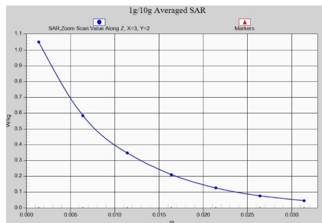
Fig. 1-36 Z-Scan at power reference point (LTE Band4)
