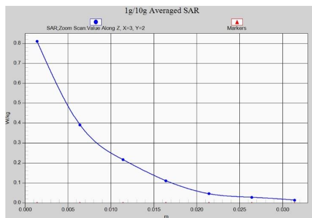
Fig. 1-44 Z-Scan at power reference point (LTE Band38)
