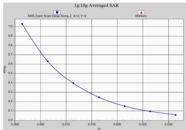
Fig. 1-26 Z-Scan at power reference point (WCDMA1900)
