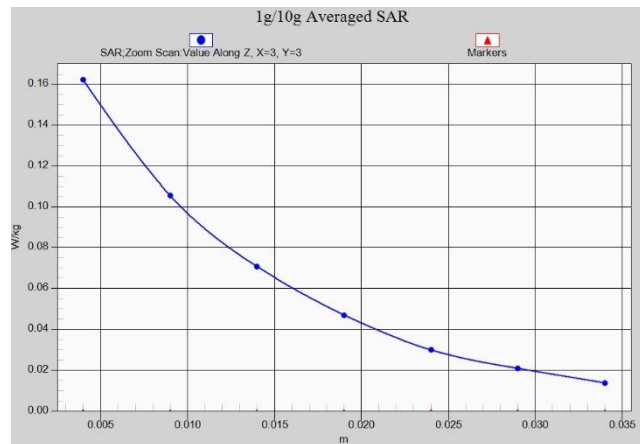
Fig. 1-27 Z-Scan at power reference point (WCDMA1700)
