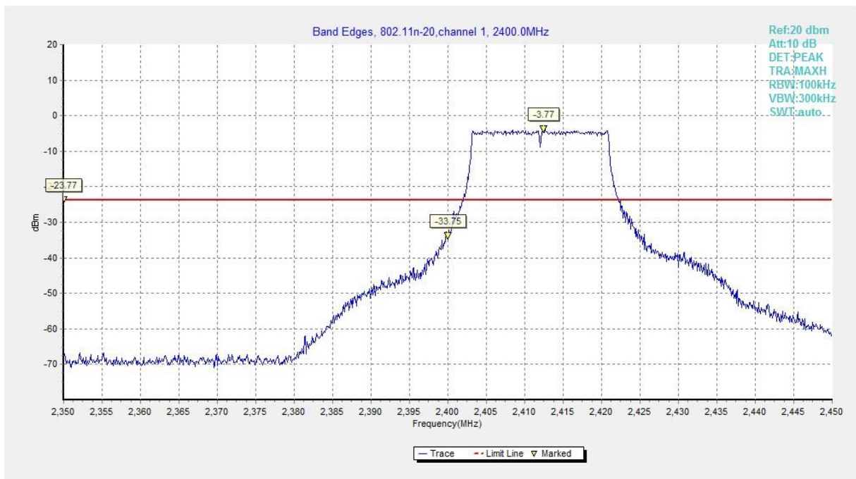
Fig.A.5.21 Band Edges (802.11n-HT20, Ch 1)
