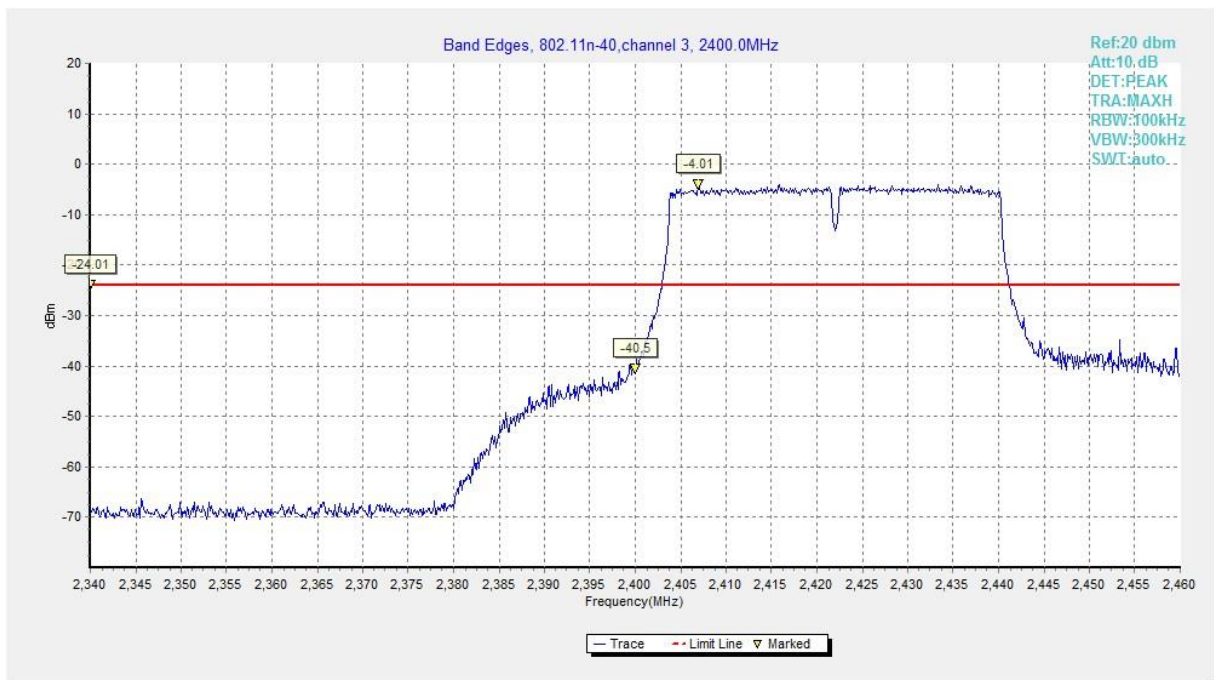
Fig.A.5.23 Band Edges (802.11n-HT40, Ch 3)
