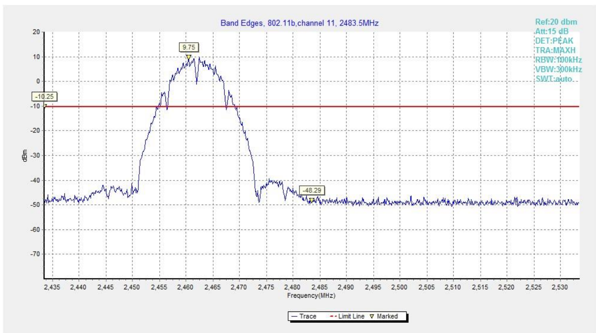
Fig.A.5.18 Band Edges (802.11b, Ch 11)
