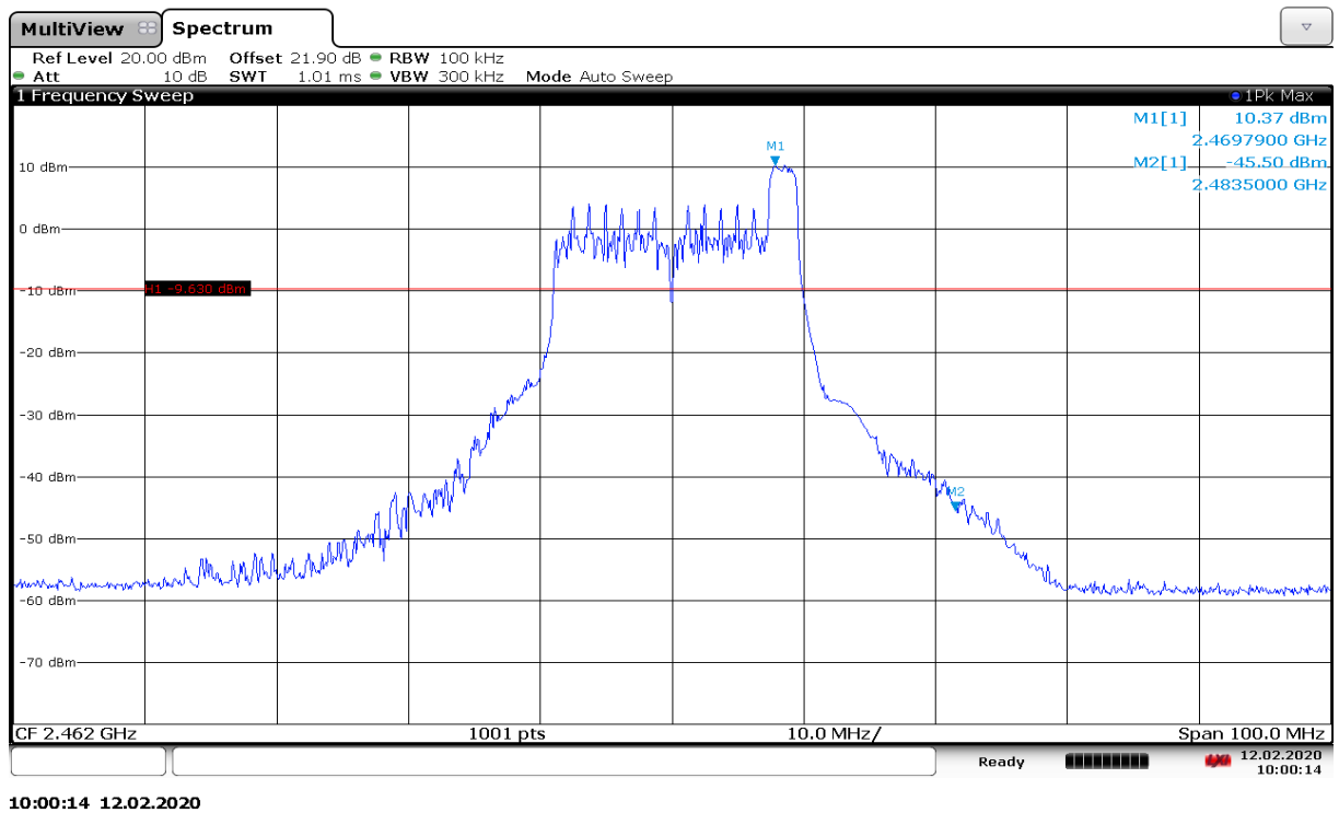
Fig.A.5.10 Band Edges (802.11n-HE20-RU26-right, Ch 11)
