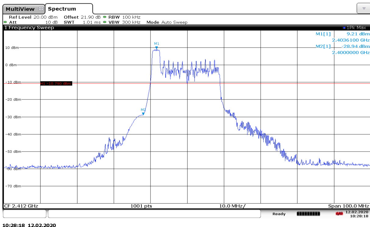
Fig.A.5.25 Band Edges (802.11n-HE20-RU26-left, Ch 1)
