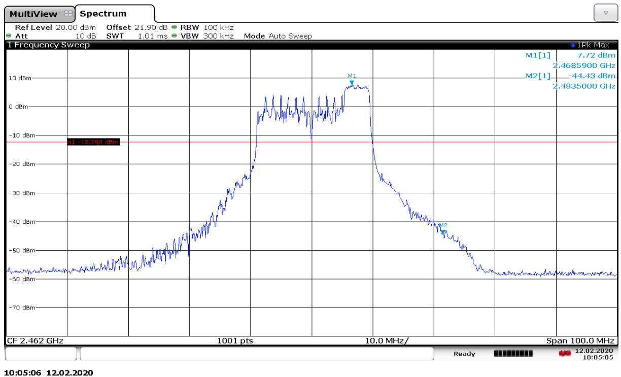
Fig.A.5.12 Band Edges (802.11n-HE20-RU52-right, Ch 11)
