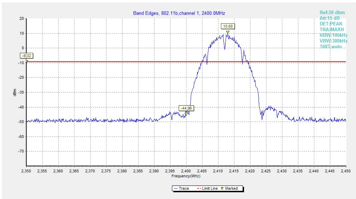
Fig.A.5.17 Band Edges (802.11b, Ch 1)
