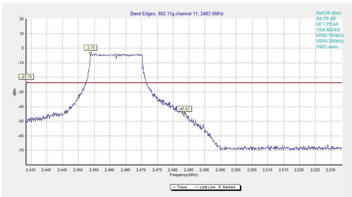
Fig.A.5.20 Band Edges (802.11g, Ch 11)
