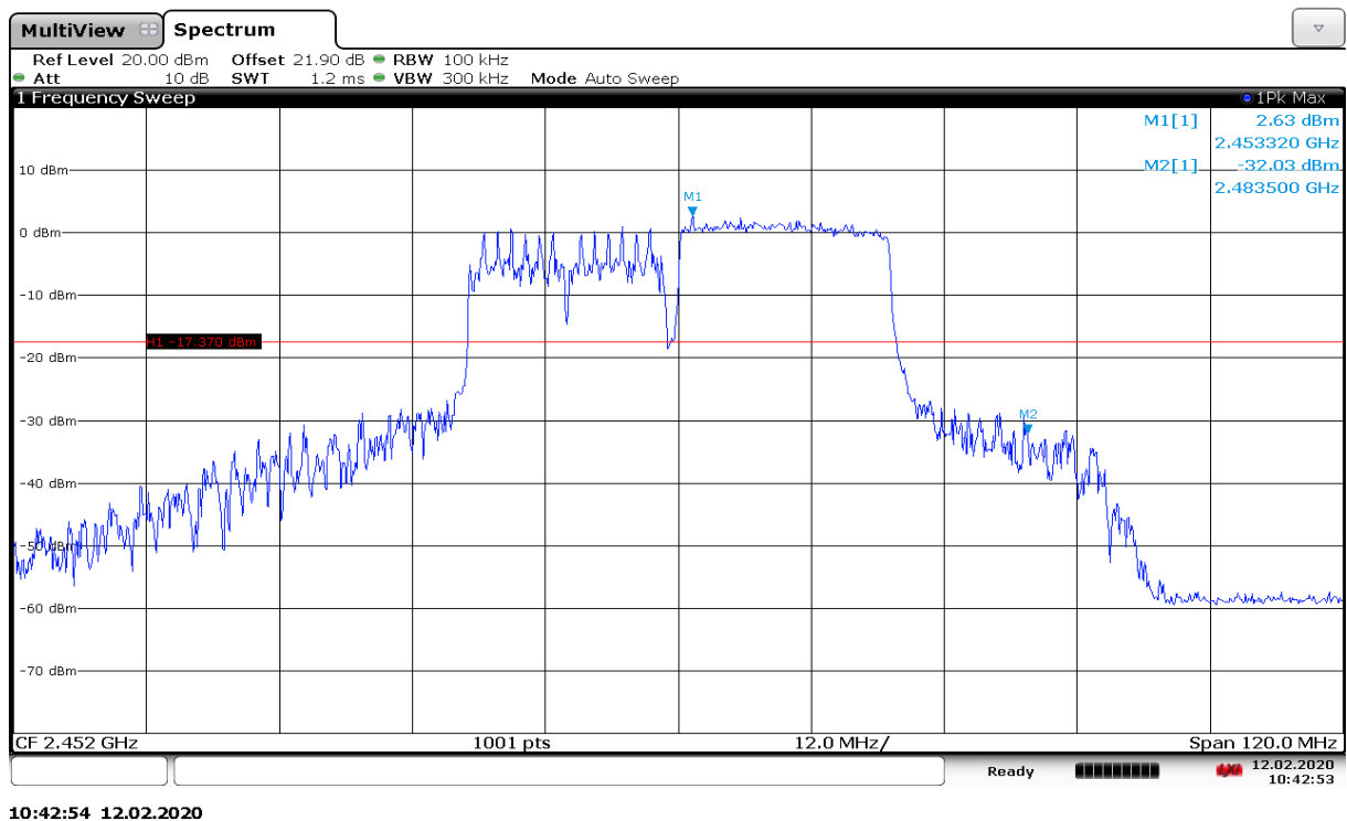
Fig.A.5.32 Band Edges (802.11n-HE40-RU242-right, Ch 9)
