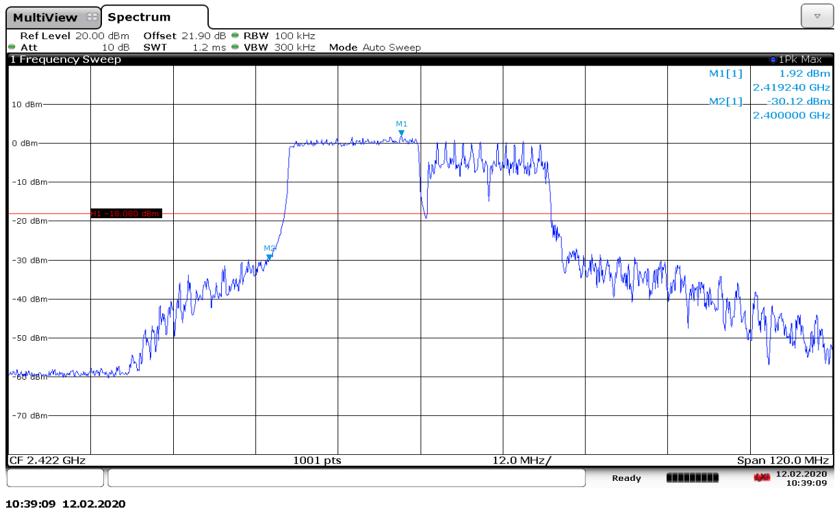
Fig.A.5.31 Band Edges (802.11n-HE40-RU242-left, Ch 3)
