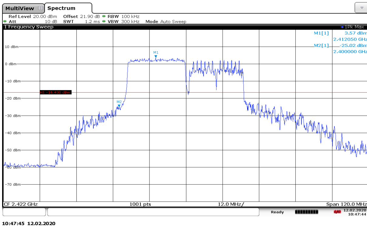
Fig.A.5.15 Band Edges (802.11n-HE40-RU242-left, Ch 3)
