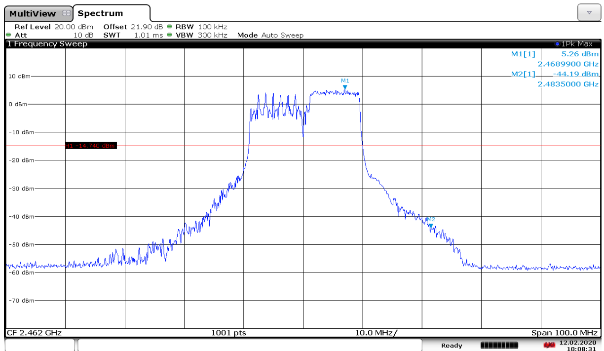
Fig.A.5.14 Band Edges (802.11n-HE20-RU106-right, Ch 11)
