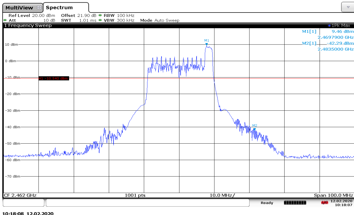
Fig.A.5.26 Band Edges (802.11n-HE20-RU26-right, Ch 11)
