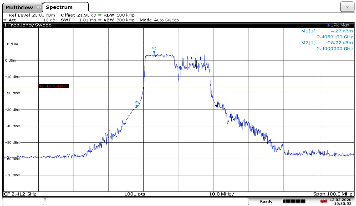
Fig.A.5.29 Band Edges (802.11n-HE20-RU106-left, Ch 1)
