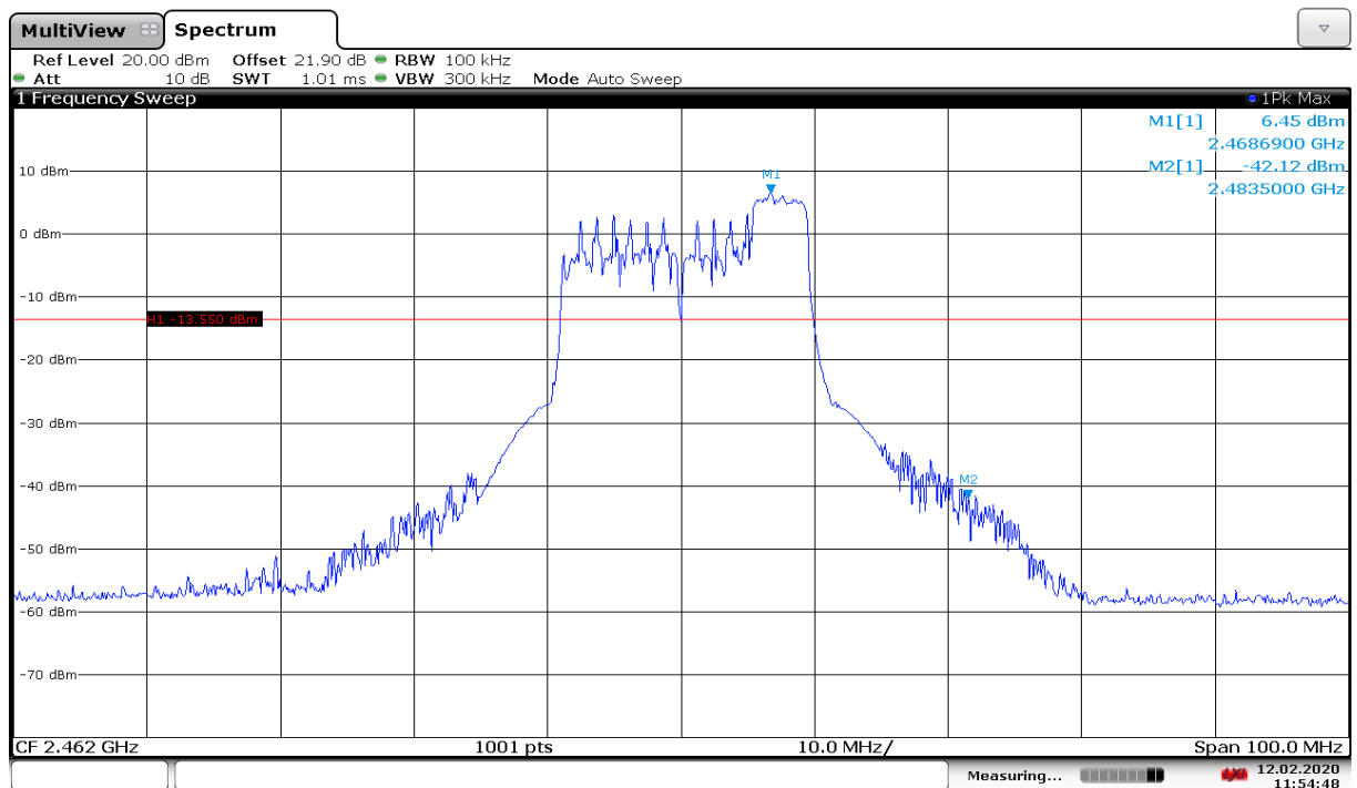
Fig.A.5.28 Band Edges (802.11n-HE20-RU52-right, Ch 11)
