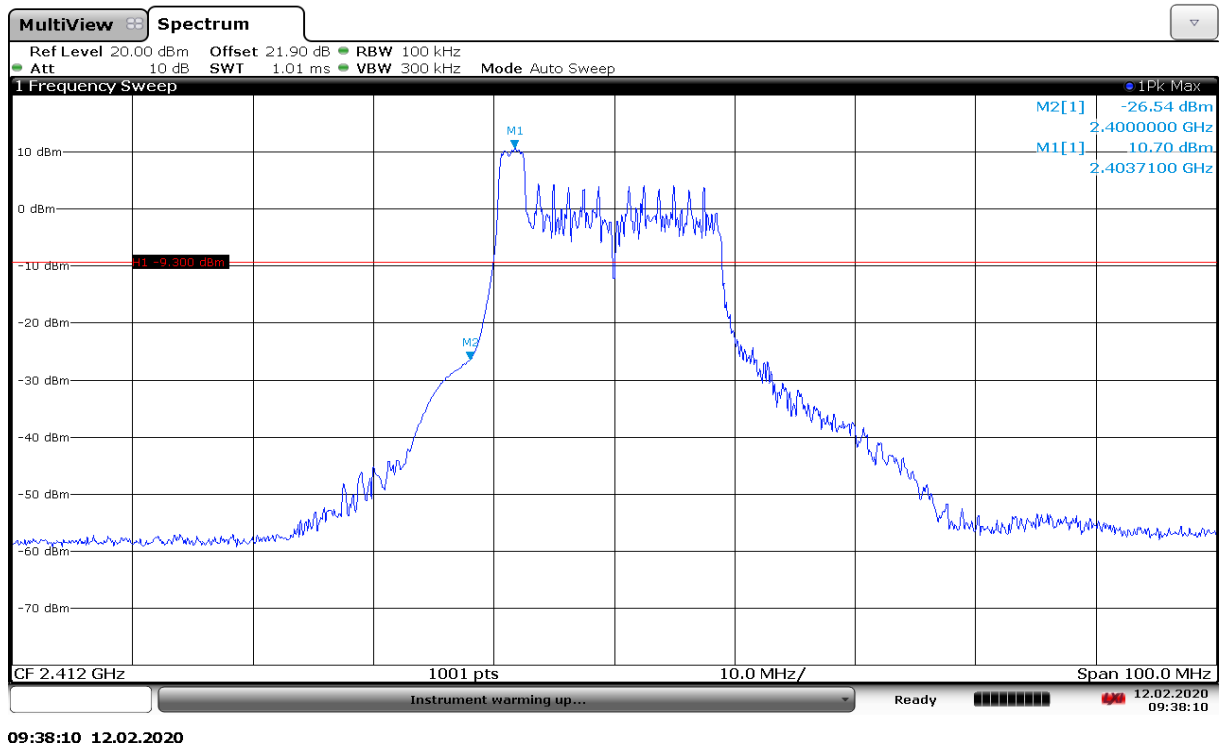
Fig.A.5.9 Band Edges (802.11n-HE20-RU26-left, Ch 1)
