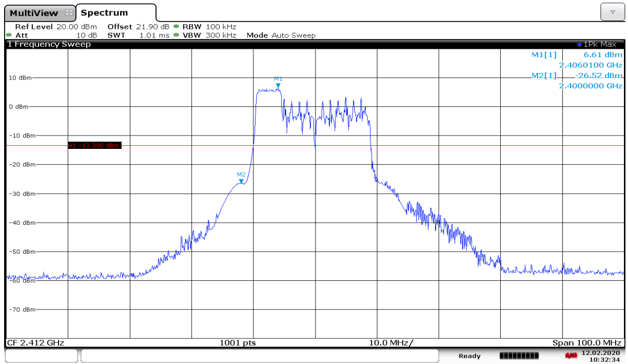
Fig.A.5.27 Band Edges (802.11n-HE20-RU52-left, Ch 1)
