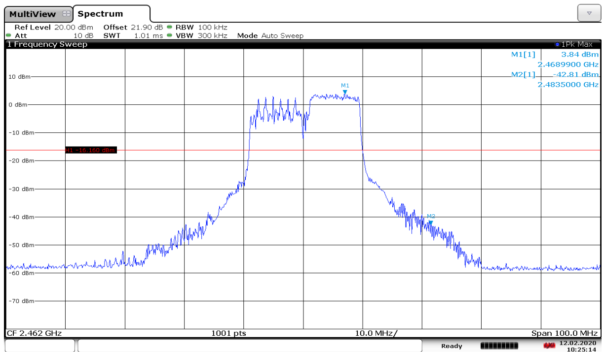
Fig.A.5.30 Band Edges (802.11n-HE20-RU106-right, Ch 11)
