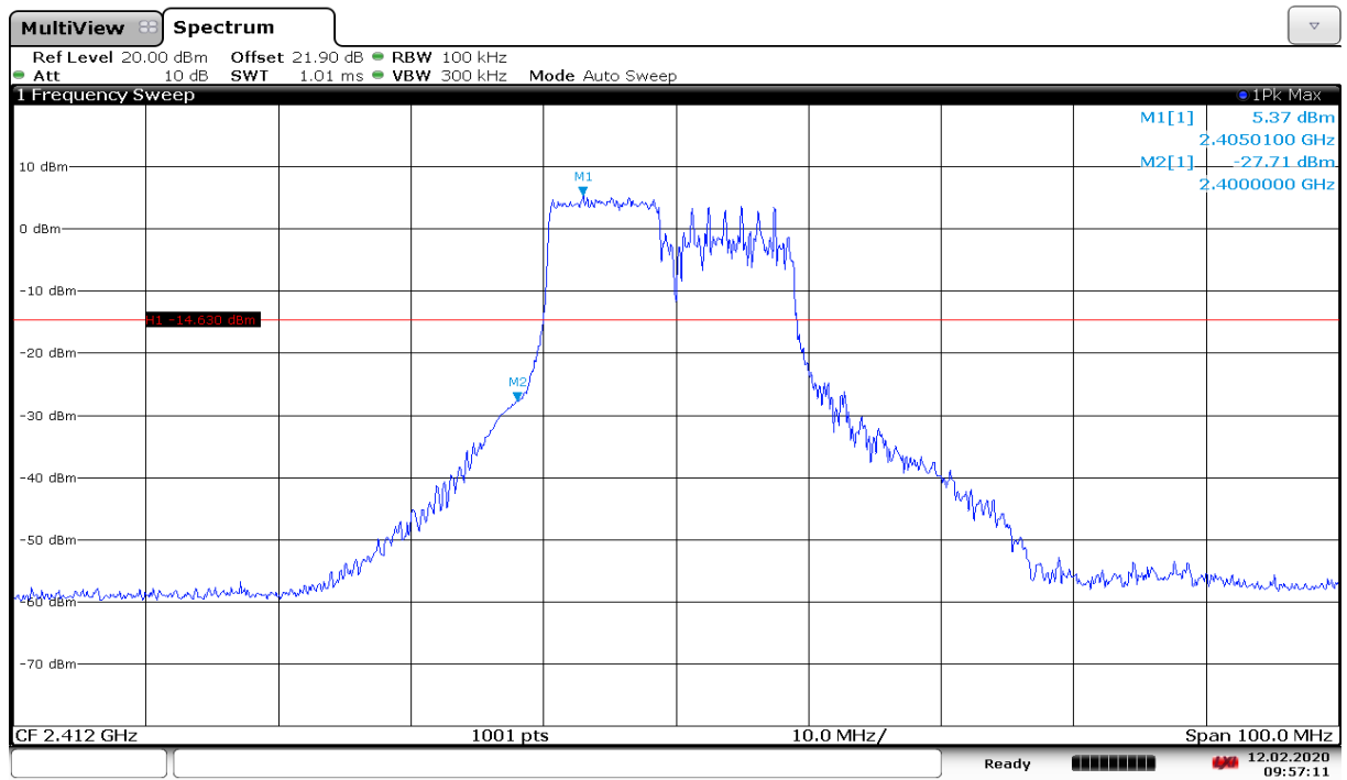
Fig.A.5.13 Band Edges (802.11n-HE20-RU106-left, Ch 1)
