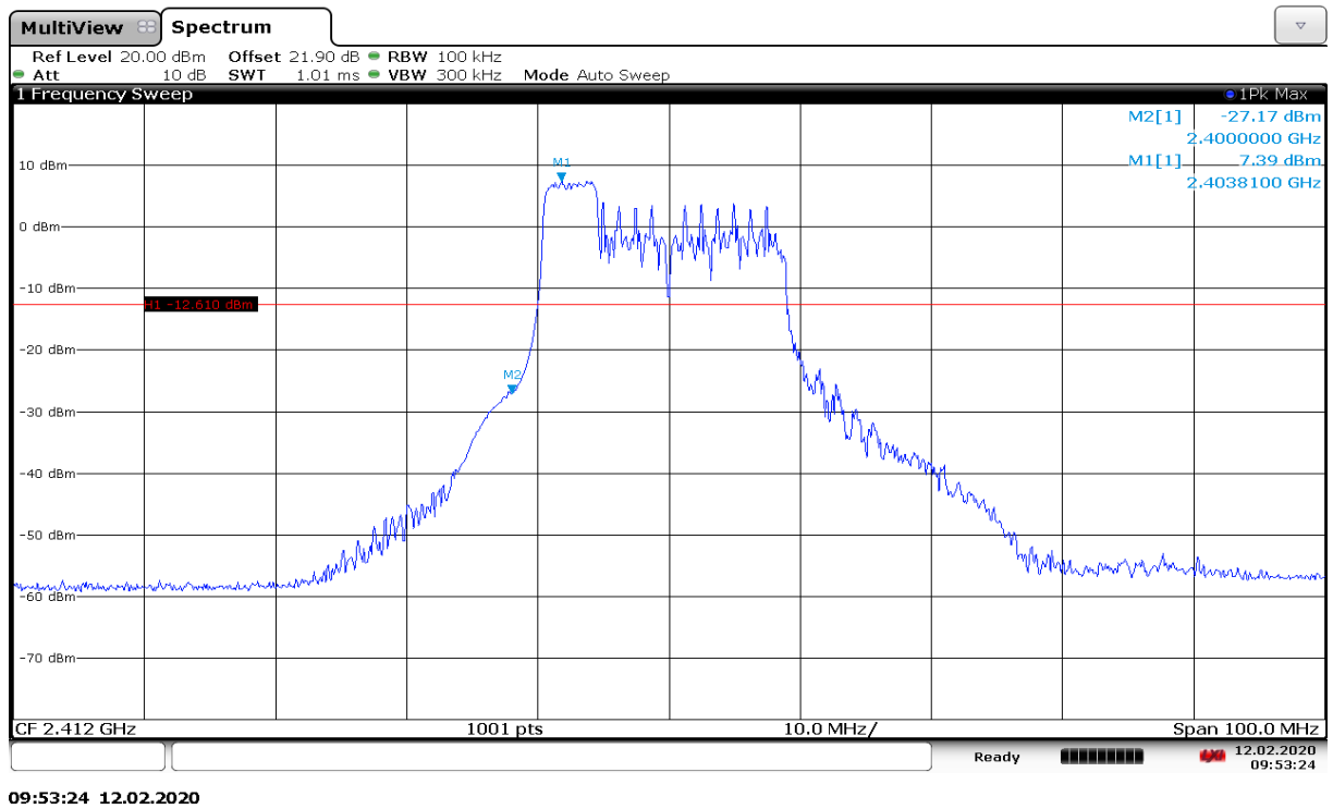
Fig.A.5.11 Band Edges (802.11n-HE20-RU52-left, Ch 1)
