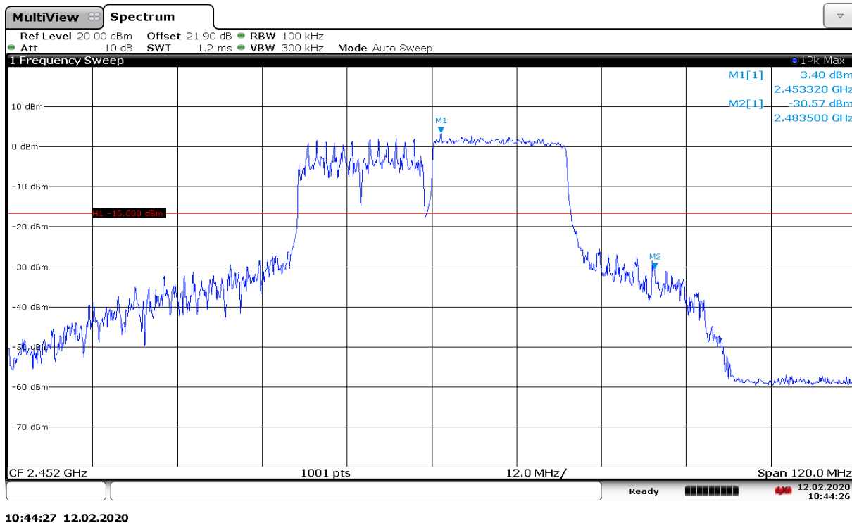
Fig.A.5.16 Band Edges (802.11n-HE40-RU242-right, Ch 9)
