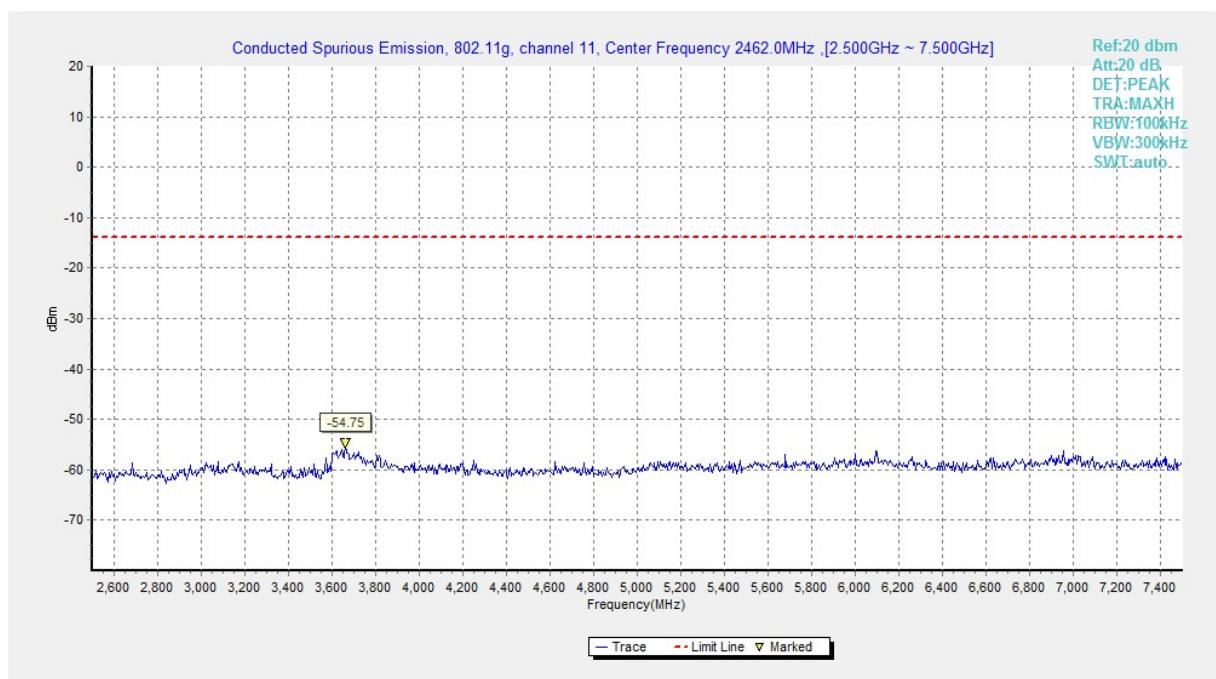
Fig.A.6.1.146 Transmitter Spurious Emission - Conducted (802.11g, Ch11, 2.5 GHz-7.5 GHz)
