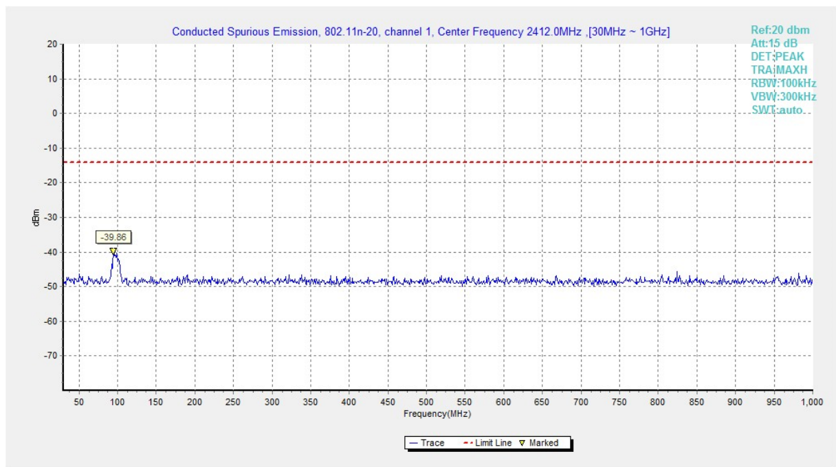
Fig.A.6.1.152 Transmitter Spurious Emission - Conducted (802.11n-HT20, Ch1, 30 MHz-1 GHz)
