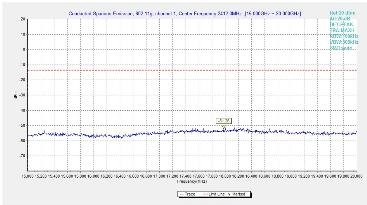
Fig.A.6.1.133 Transmitter Spurious Emission - Conducted (802.11g, Ch1, 15 GHz-20 GHz)
