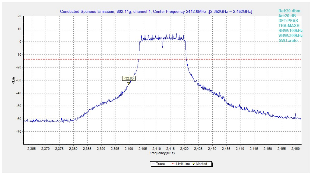
Fig.A.6.1.127 Transmitter Spurious Emission - Conducted (802.11g, Ch1, Center Frequency)
