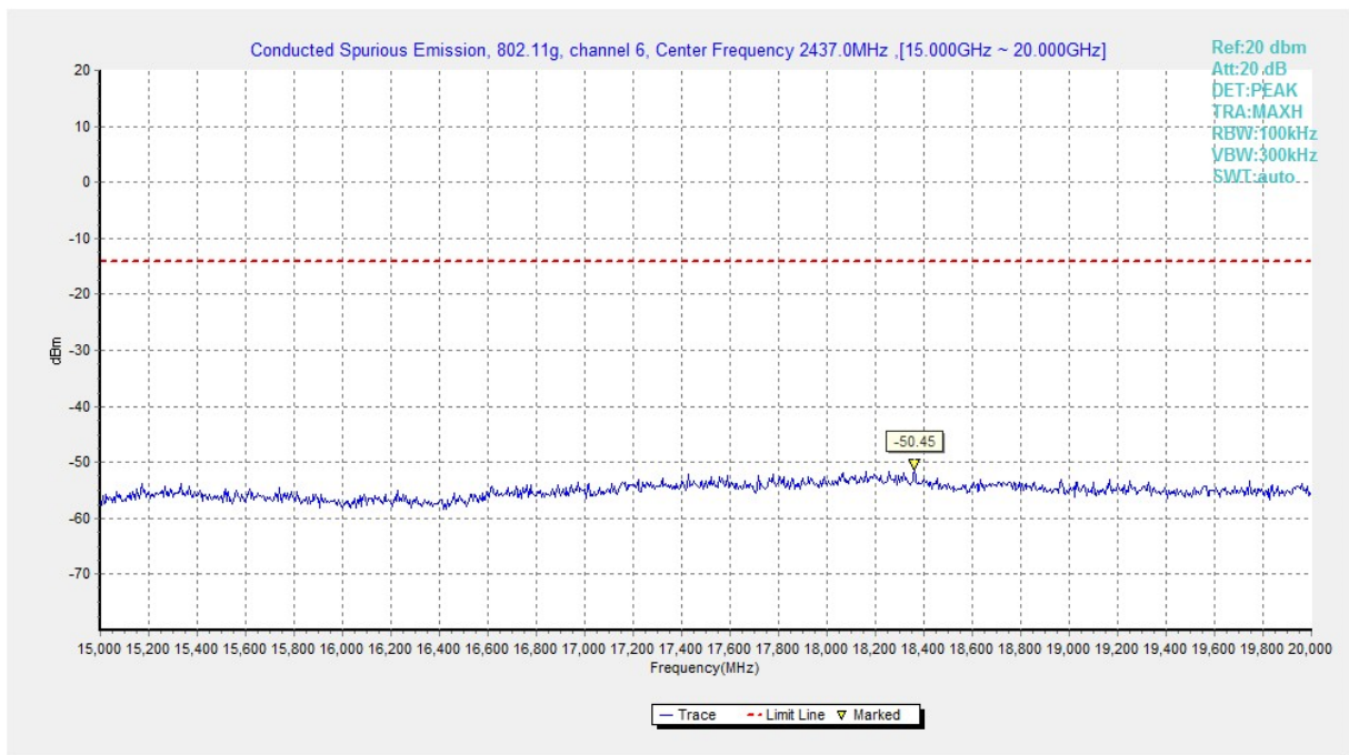
Fig.A.6.1.141 Transmitter Spurious Emission - Conducted (802.11g, Ch6, 15 GHz-20 GHz)
