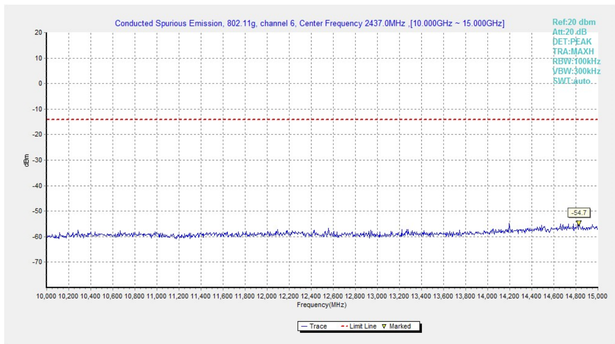
Fig.A.6.1.140 Transmitter Spurious Emission - Conducted (802.11g, Ch6, 10 GHz-15 GHz)
