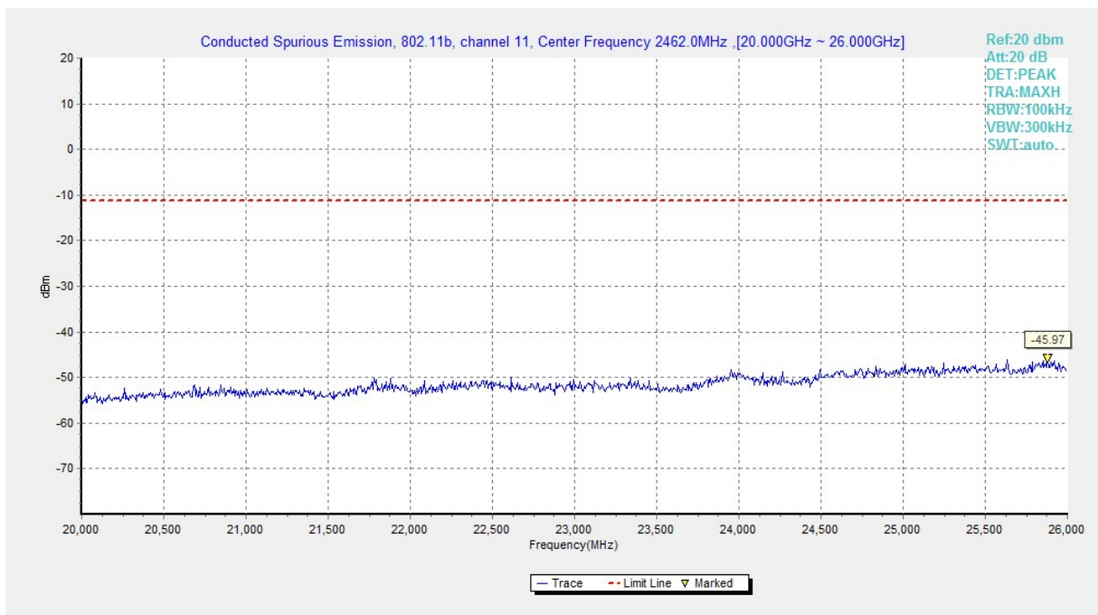
Fig.A.6.1.126 Transmitter Spurious Emission - Conducted (802.11b, Ch11, 20 GHz-26 GHz)
