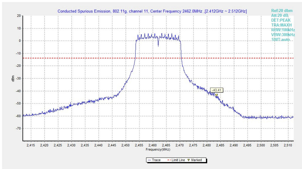
Fig.A.6.1.143 Transmitter Spurious Emission - Conducted (802.11g, Ch11, Center Frequency)
