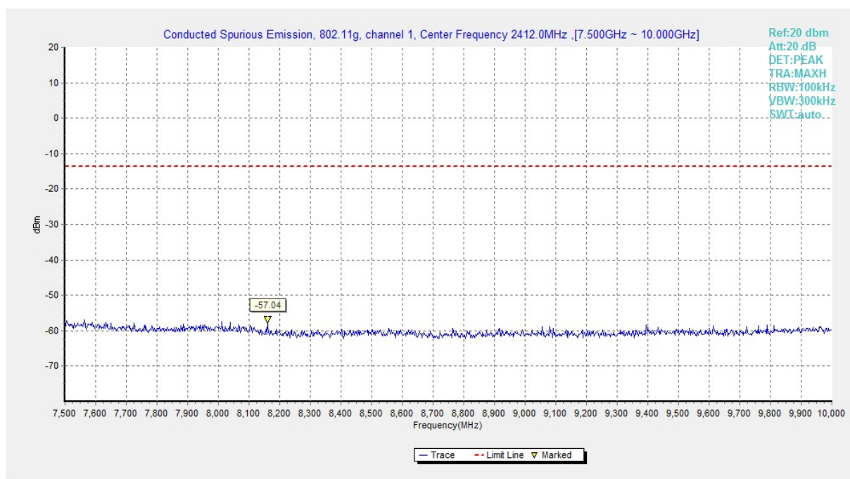
Fig.A.6.1.131 Transmitter Spurious Emission - Conducted (802.11g, Ch1, 7.5 GHz-10 GHz)
