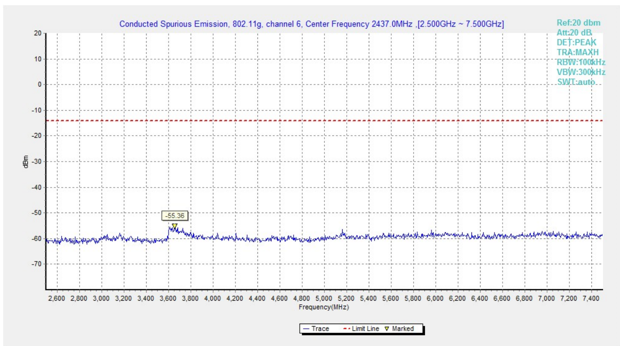
Fig.A.6.1.138 Transmitter Spurious Emission - Conducted (802.11g, Ch6, 2.5 GHz-7.5 GHz)
