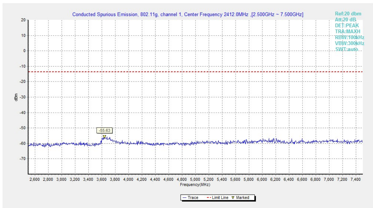
Fig.A.6.1.130 Transmitter Spurious Emission - Conducted (802.11g, Ch1, 2.5 GHz-7.5 GHz)
