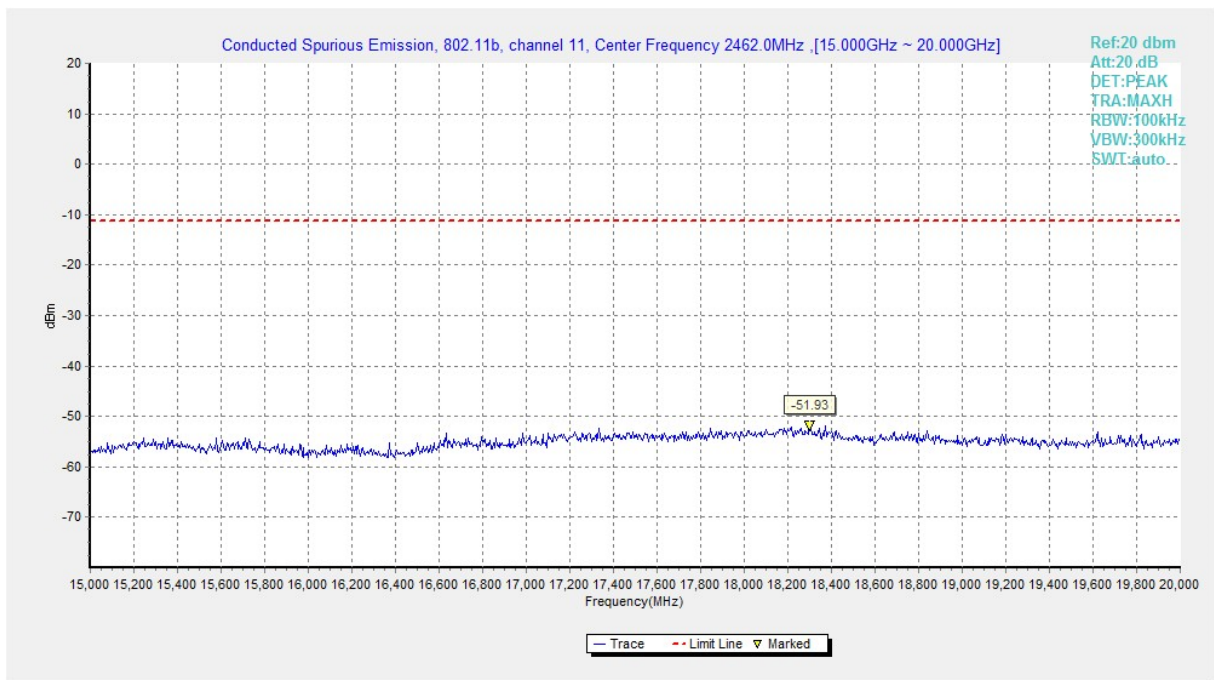
Fig.A.6.1.125 Transmitter Spurious Emission - Conducted (802.11b, Ch11, 15 GHz-20 GHz)
