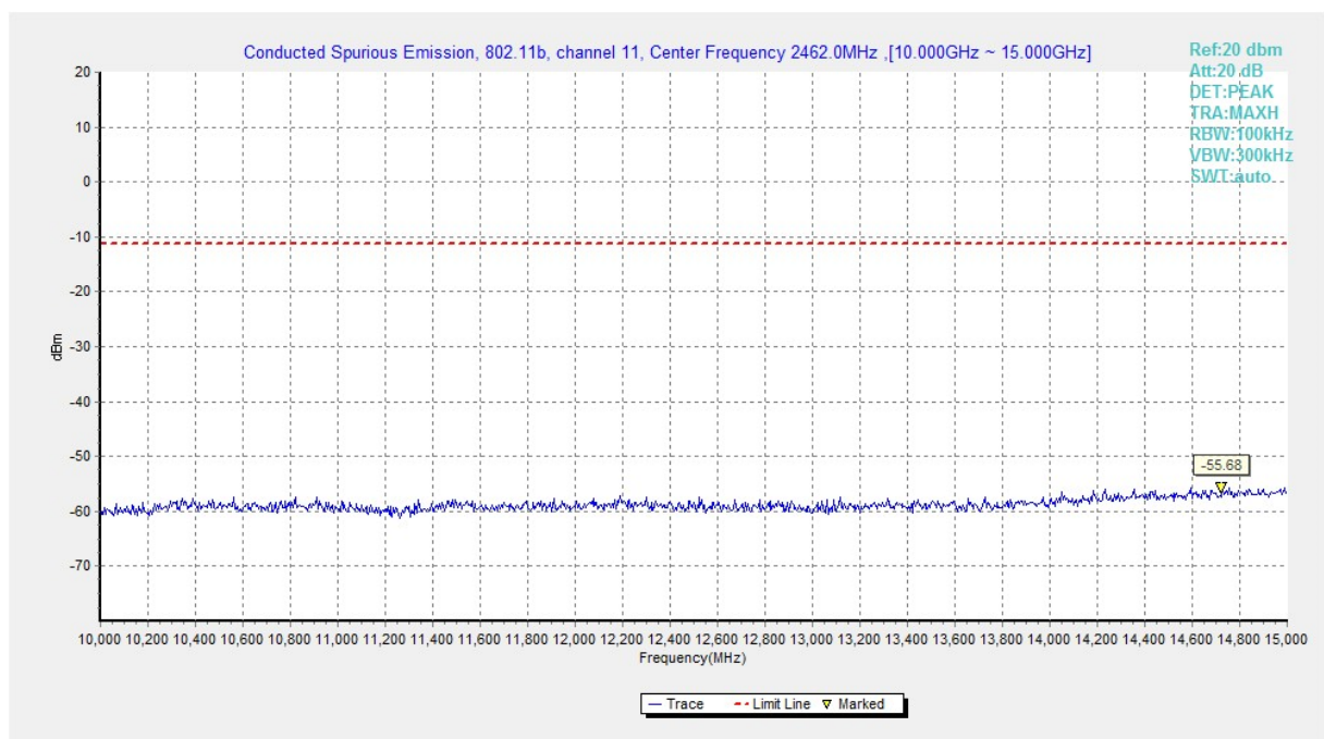
Fig.A.6.1.124 Transmitter Spurious Emission - Conducted (802.11b, Ch11, 10 GHz-15 GHz)
