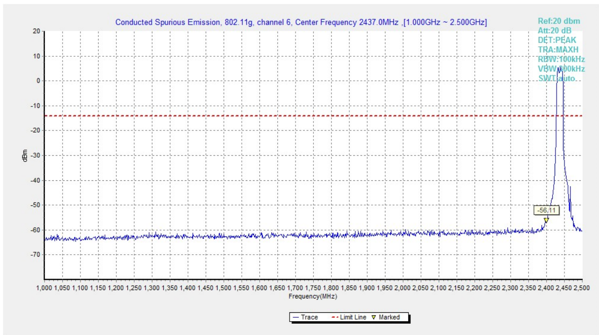
Fig.A.6.1.137 Transmitter Spurious Emission - Conducted (802.11g, Ch6, 1 GHz-2.5 GHz)
