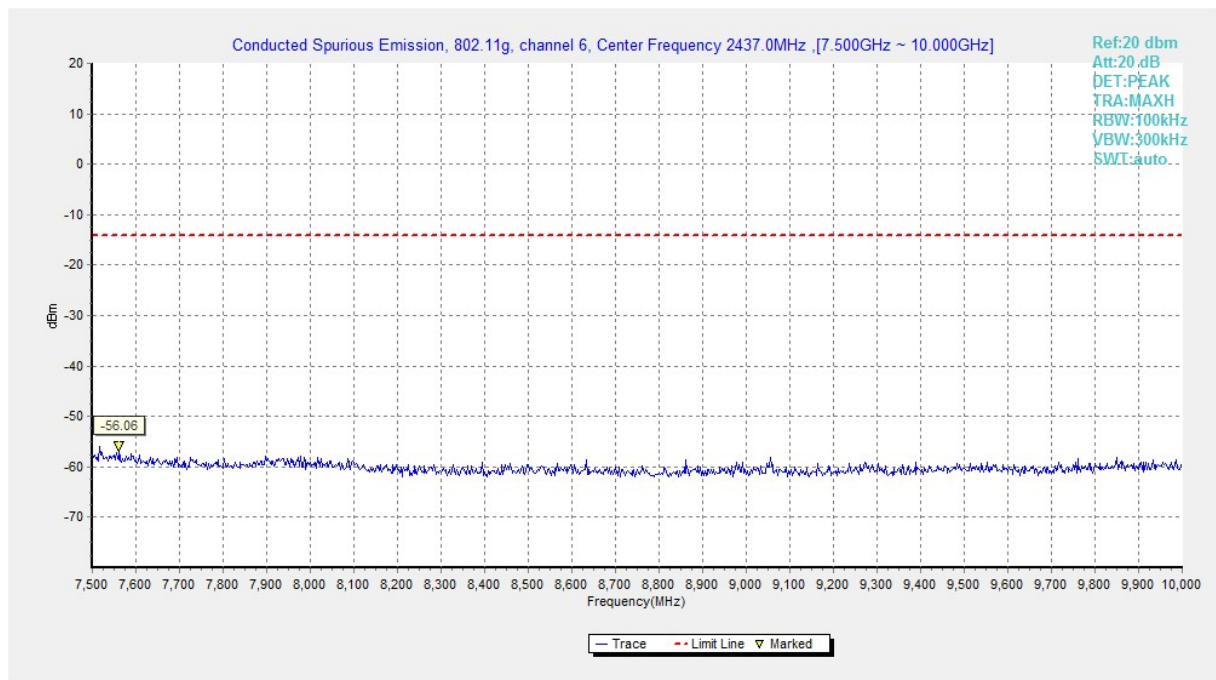
Fig.A.6.1.139 Transmitter Spurious Emission - Conducted (802.11g, Ch6, 7.5 GHz-10 GHz)
