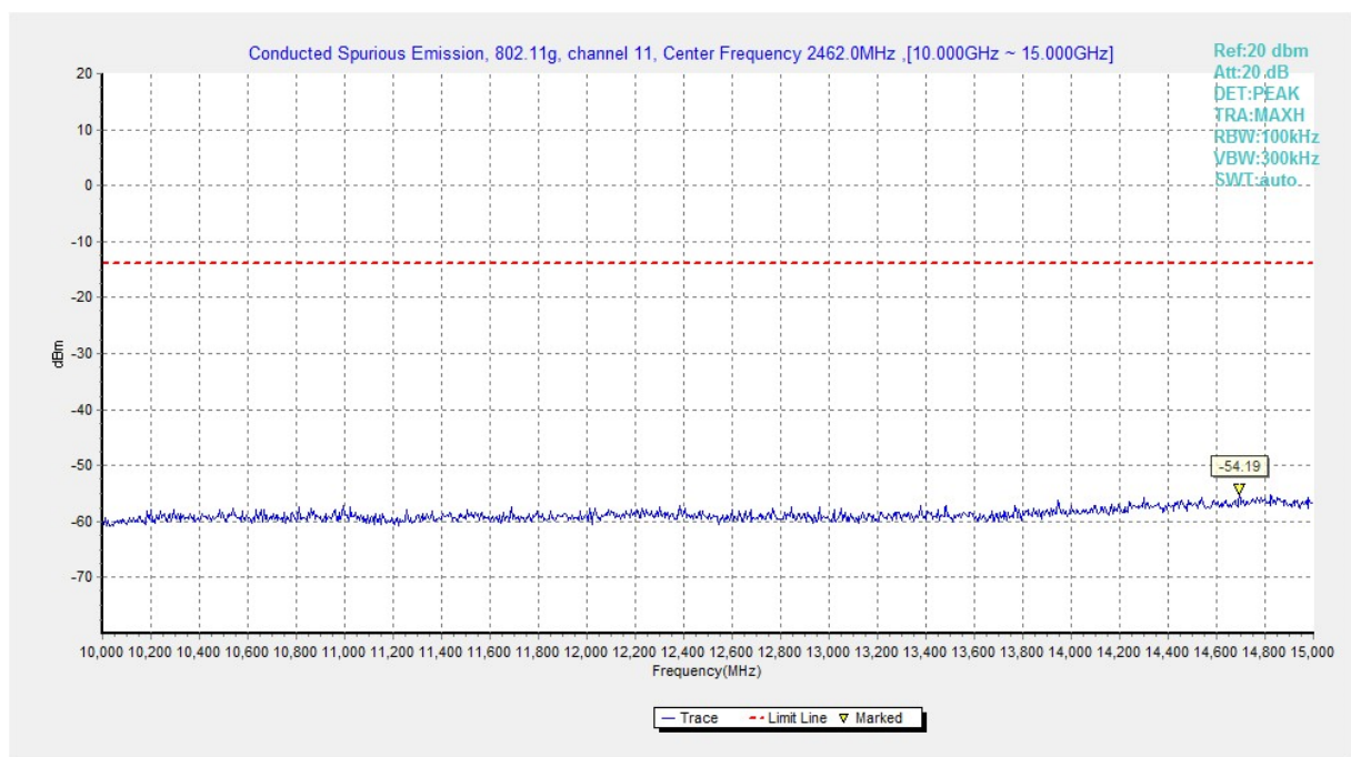
Fig.A.6.1.148 Transmitter Spurious Emission - Conducted (802.11g, Ch11, 10 GHz-15 GHz)
