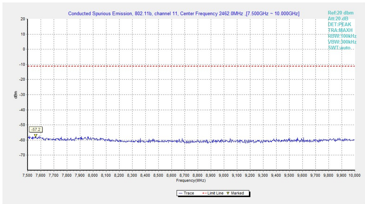
Fig.A.6.1.123 Transmitter Spurious Emission - Conducted (802.11b, Ch11, 7.5 GHz-10 GHz)
