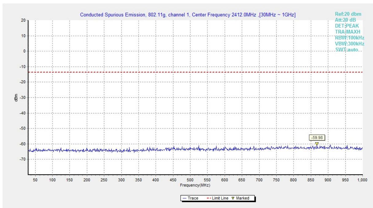
Fig.A.6.1.128 Transmitter Spurious Emission - Conducted (802.11g, Ch1, 30 MHz-1 GHz)
