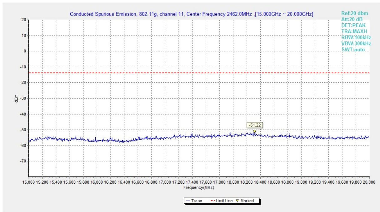
Fig.A.6.1.149 Transmitter Spurious Emission - Conducted (802.11g, Ch11, 15 GHz-20 GHz)
