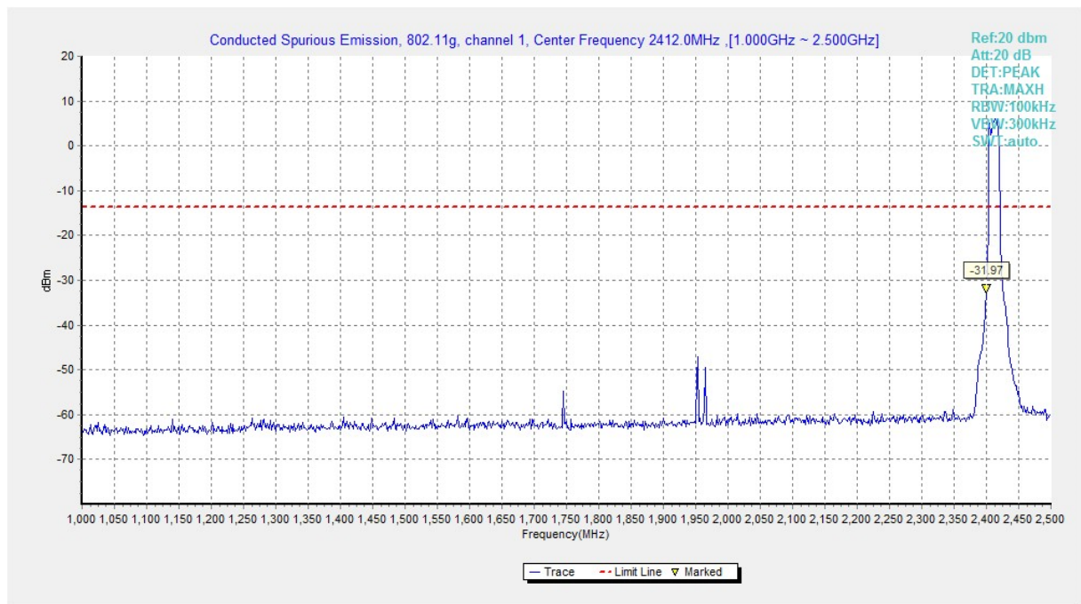
Fig.A.6.1.129 Transmitter Spurious Emission - Conducted (802.11g, Ch1, 1 GHz-2.5 GHz)
