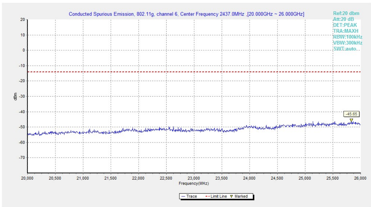
Fig.A.6.1.142 Transmitter Spurious Emission - Conducted (802.11g, Ch6, 20 GHz-26 GHz)
