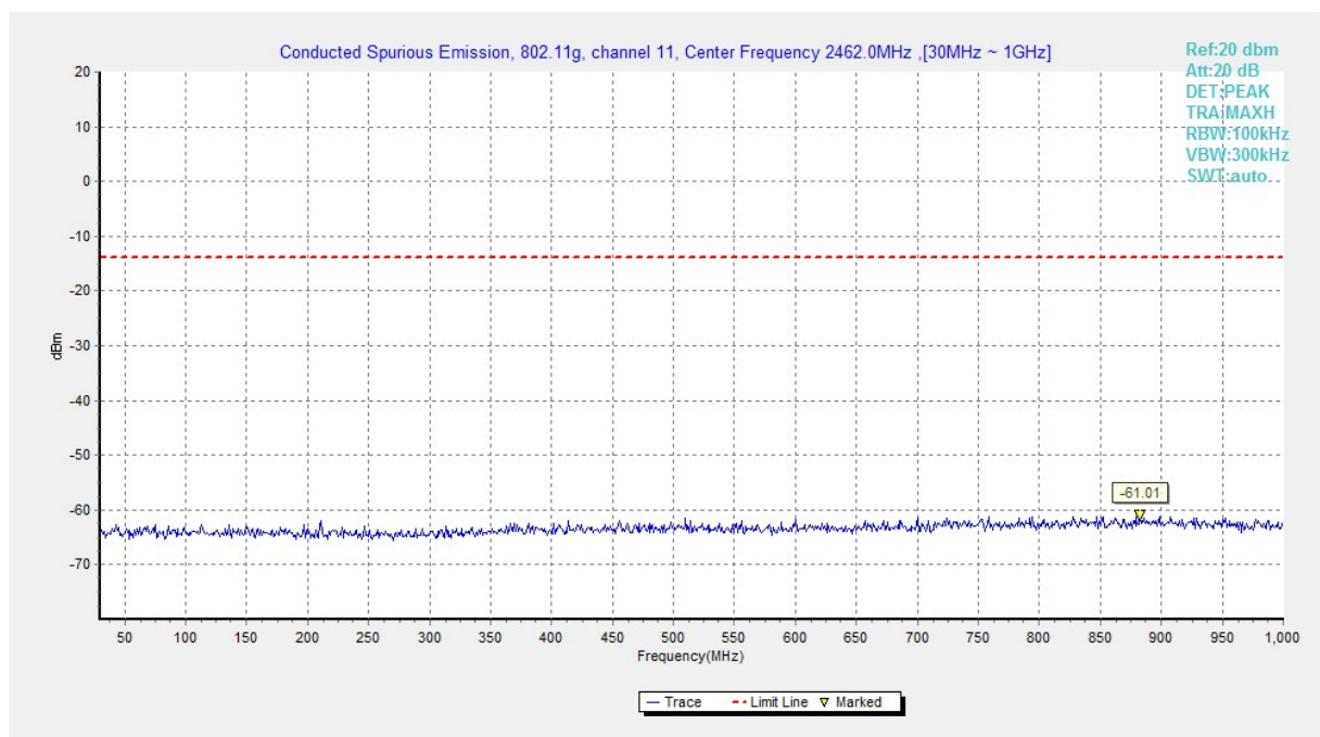
Fig.A.6.1.144 Transmitter Spurious Emission - Conducted (802.11g, Ch11, 30 MHz-1 GHz)
