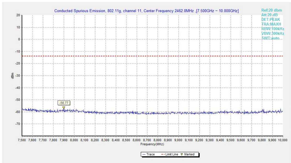
Fig.A.6.1.147 Transmitter Spurious Emission - Conducted (802.11g, Ch11, 7.5 GHz-10 GHz)
