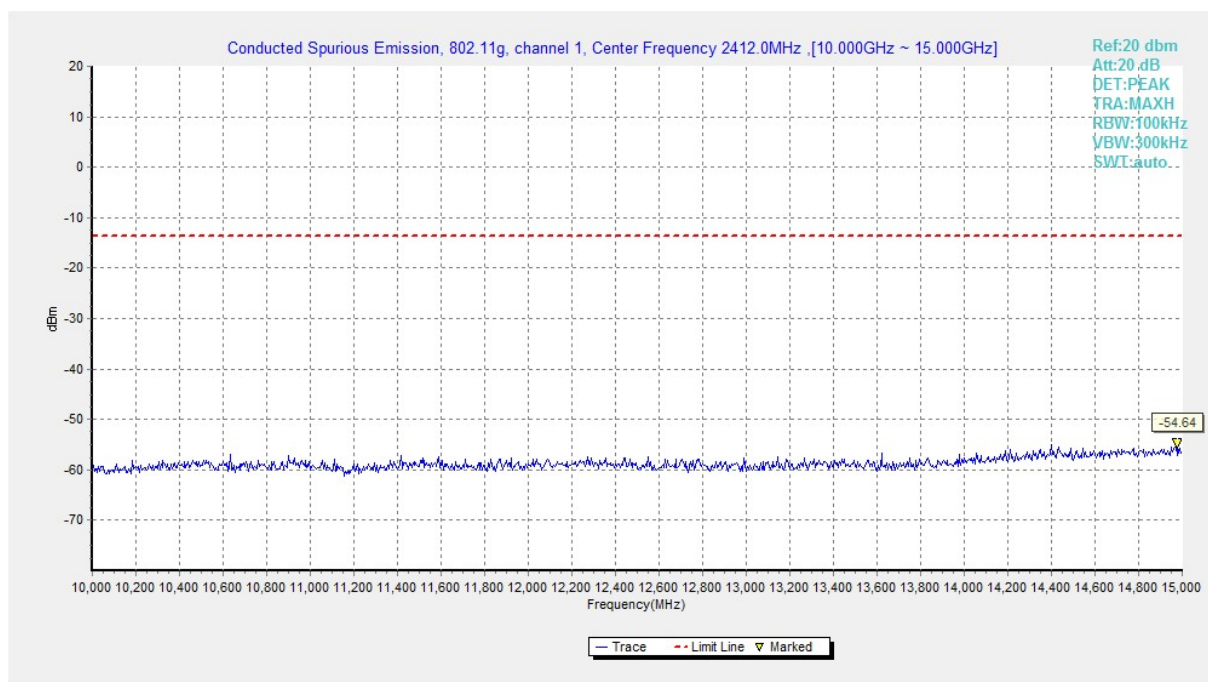
Fig.A.6.1.132 Transmitter Spurious Emission - Conducted (802.11g, Ch1, 10 GHz-15 GHz)
