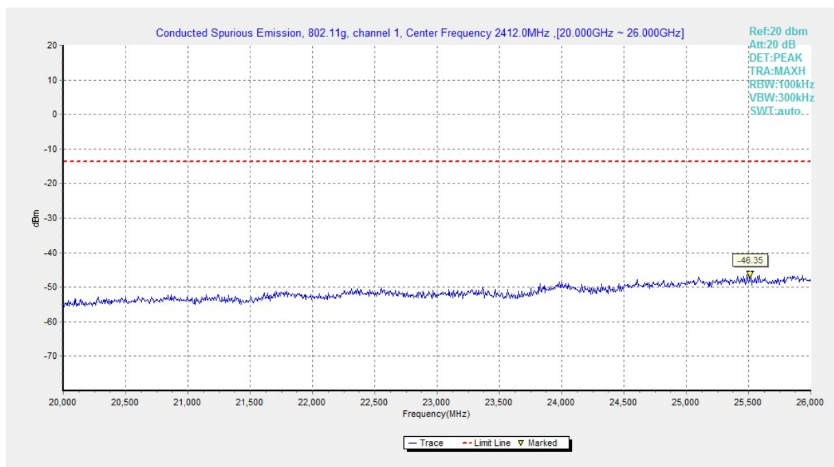
Fig.A.6.1.134 Transmitter Spurious Emission - Conducted (802.11g, Ch1, 20 GHz-26 GHz)
