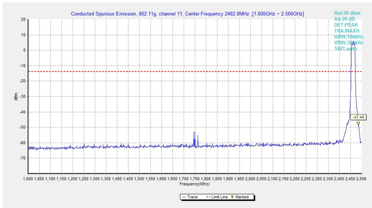
Fig.A.6.1.145 Transmitter Spurious Emission - Conducted (802.11g, Ch11, 1 GHz-2.5 GHz)
