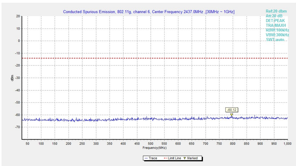
Fig.A.6.1.136 Transmitter Spurious Emission - Conducted (802.11g, Ch6, 30 MHz-1 GHz)
