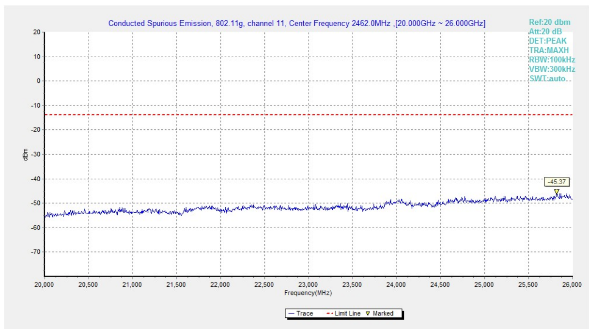
Fig.A.6.1.150 Transmitter Spurious Emission - Conducted (802.11g, Ch11, 20 GHz-26 GHz)
