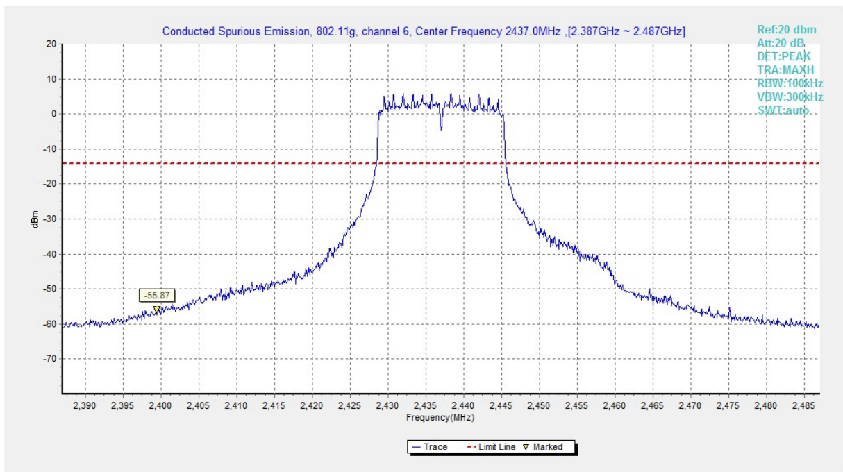
Fig.A.6.1.135 Transmitter Spurious Emission - Conducted (802.11g, Ch6, Center Frequency)
