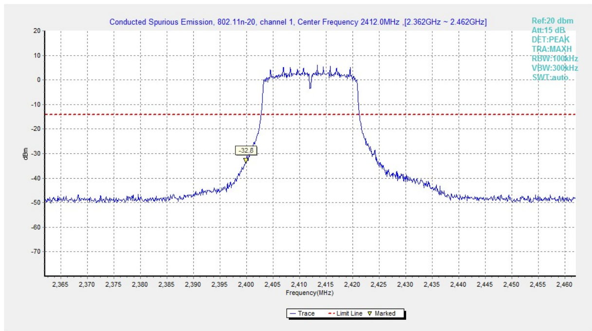
Fig.A.6.1.151 Transmitter Spurious Emission - Conducted (802.11n-HT20, Ch1, Center Frequency)
