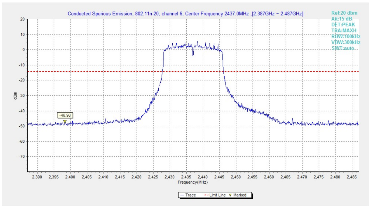
Fig.A.6.1.159 Transmitter Spurious Emission - Conducted (802.11n-HT20, Ch6, Center Frequency)
