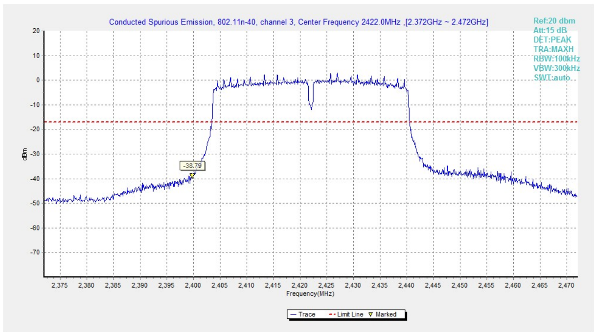
Fig.A.6.1.175 Transmitter Spurious Emission - Conducted (802.11n-HT40, Ch3, Center Frequency)
