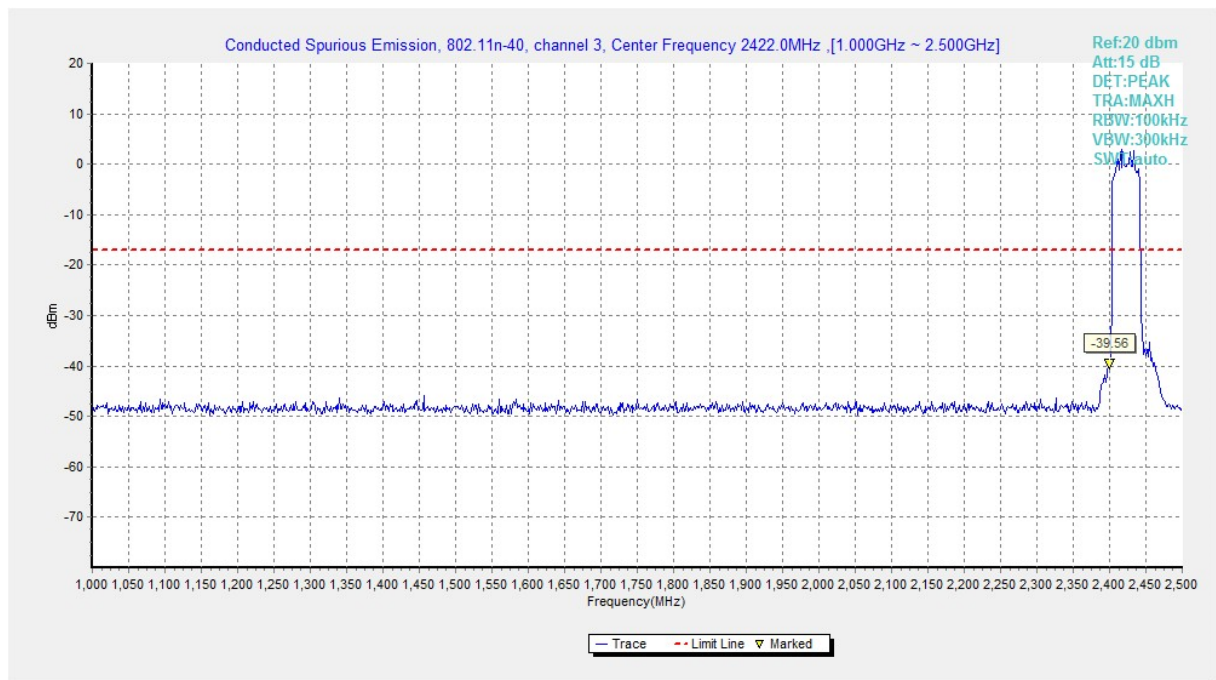
Fig.A.6.1.177 Transmitter Spurious Emission - Conducted (802.11n-HT40, Ch3, 1 GHz-2.5 GHz)
