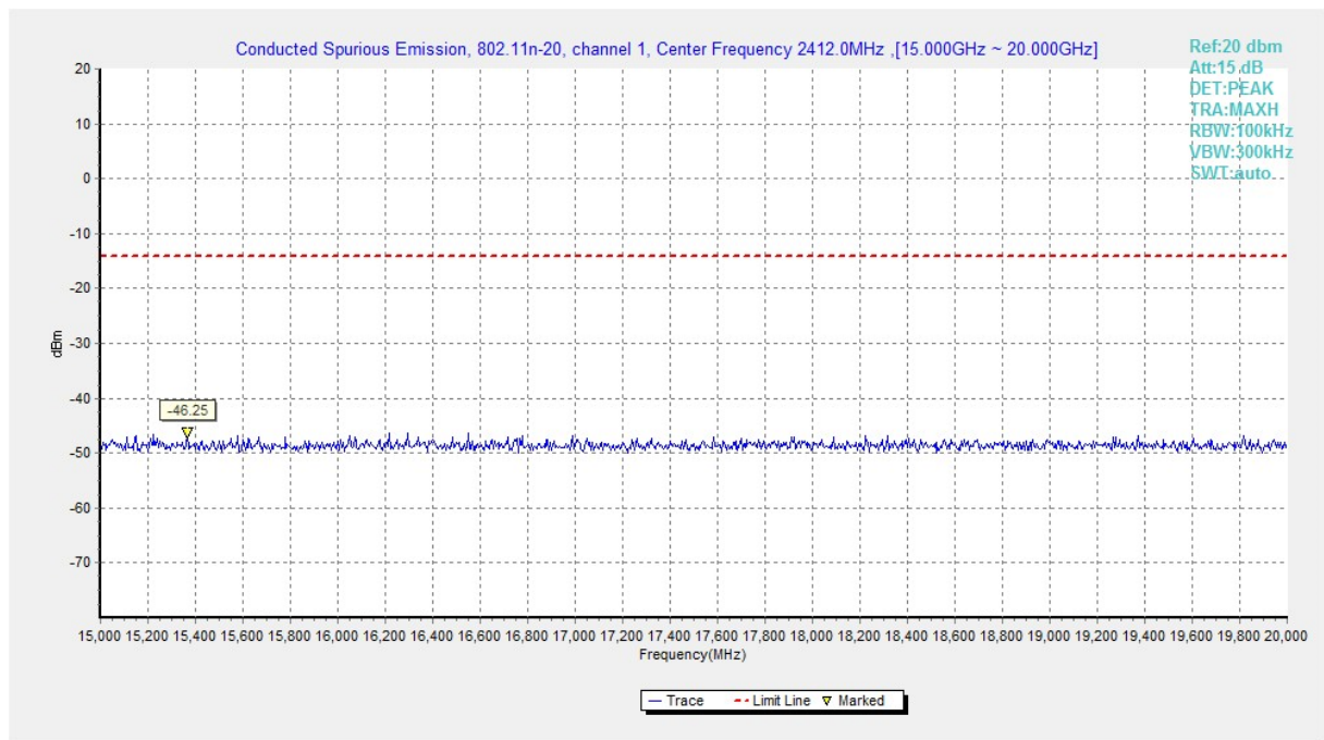
Fig.A.6.1.157 Transmitter Spurious Emission - Conducted (802.11n-HT20, Ch1, 15 GHz-20 GHz)
