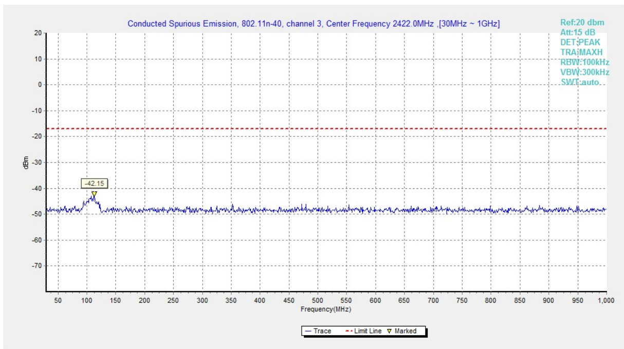
Fig.A.6.1.176 Transmitter Spurious Emission - Conducted (802.11n-HT40, Ch3, 30 MHz-1 GHz)
