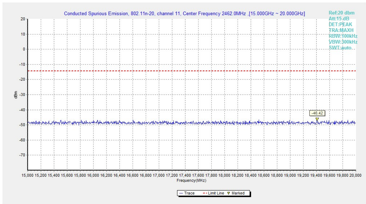
Fig.A.6.1.173 Transmitter Spurious Emission - Conducted (802.11n-HT20, Ch11, 15 GHz-20 GHz)
