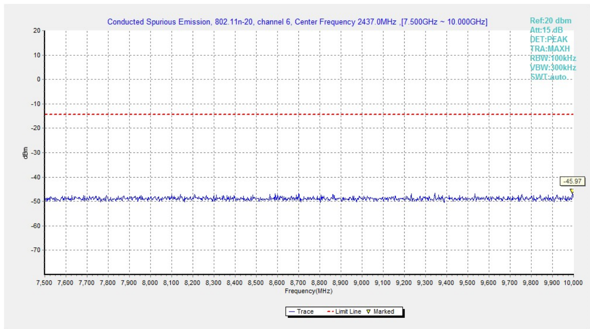
Fig.A.6.1.163 Transmitter Spurious Emission - Conducted (802.11n-HT20, Ch6, 7.5 GHz-10 GHz)
