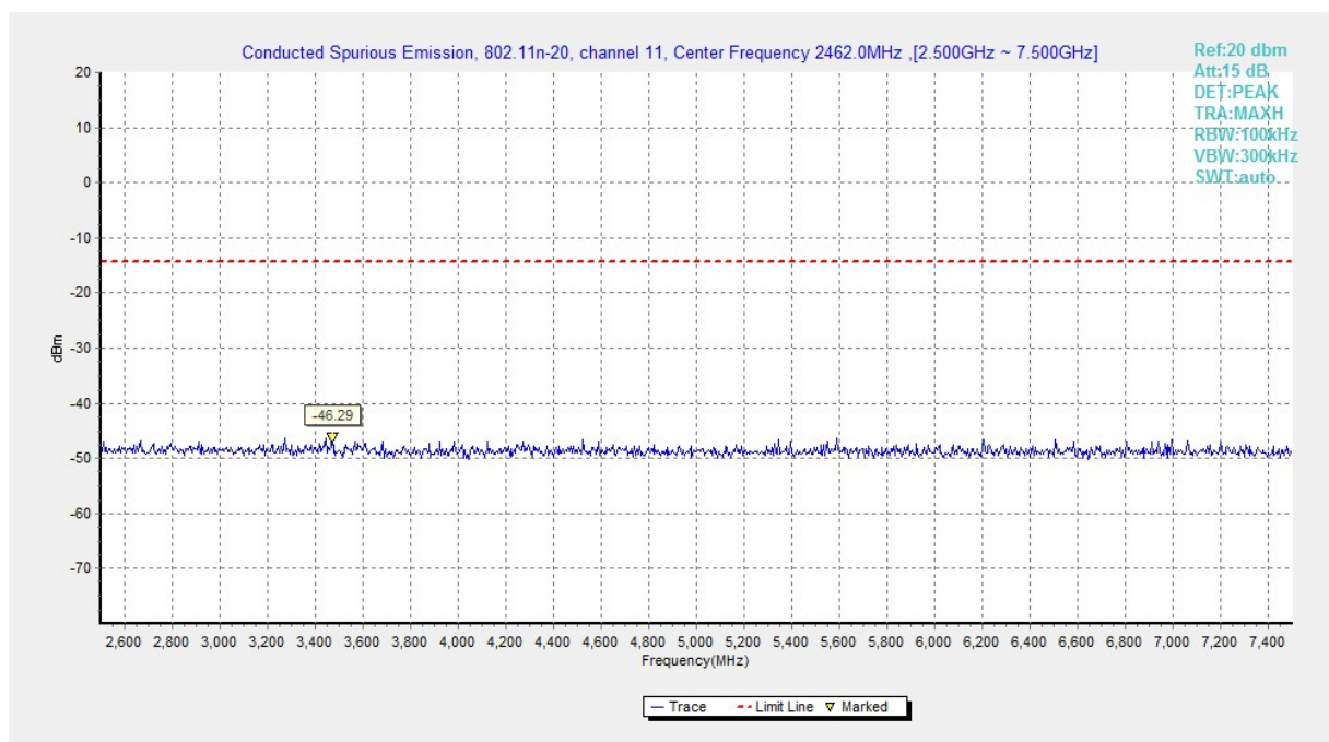
Fig.A.6.1.170 Transmitter Spurious Emission - Conducted (802.11n-HT20, Ch11, 2.5 GHz-7.5 GHz)
