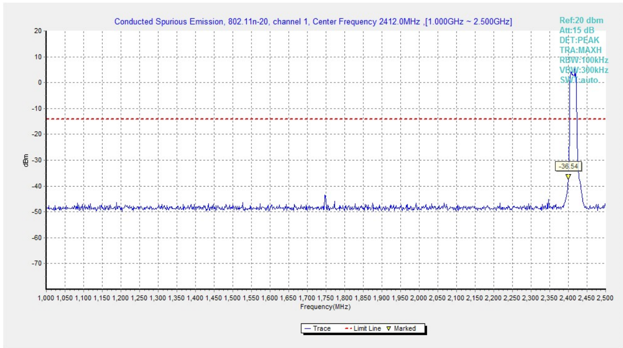
Fig.A.6.1.153 Transmitter Spurious Emission - Conducted (802.11n-HT20, Ch1, 1 GHz-2.5 GHz)
