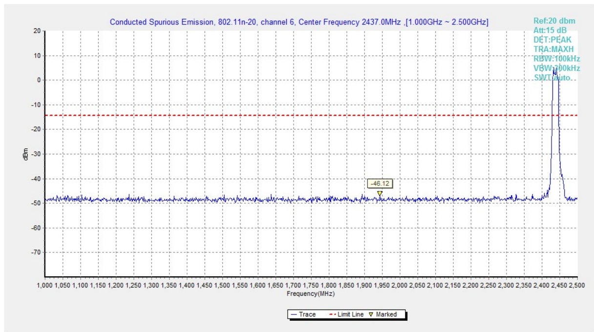
Fig.A.6.1.161 Transmitter Spurious Emission - Conducted (802.11n-HT20, Ch6, 1 GHz-2.5 GHz)
