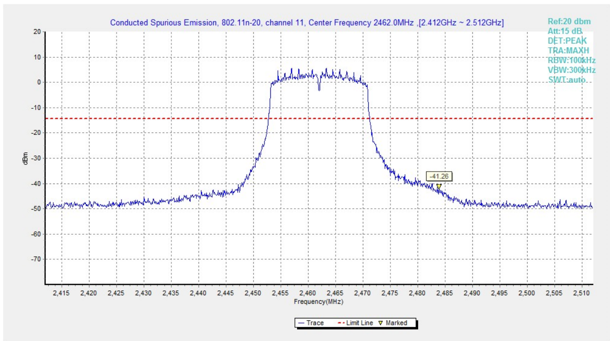
Fig.A.6.1.167 Transmitter Spurious Emission - Conducted (802.11n-HT20, Ch11, Center Frequency)
