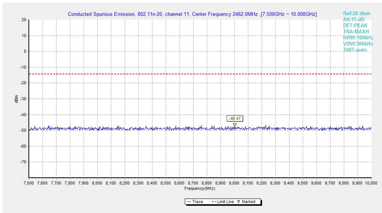
Fig.A.6.1.171 Transmitter Spurious Emission - Conducted (802.11n-HT20, Ch11, 7.5 GHz-10 GHz)
