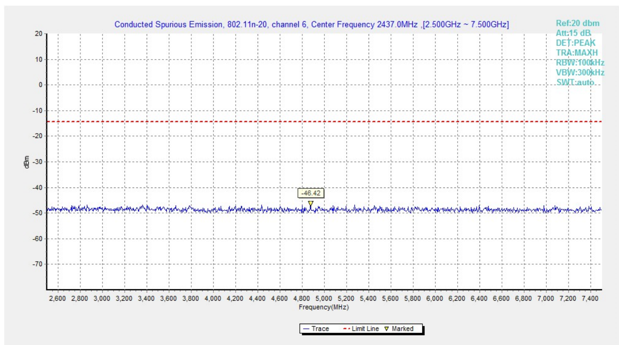
Fig.A.6.1.162 Transmitter Spurious Emission - Conducted (802.11n-HT20, Ch6, 2.5 GHz-7.5 GHz)
