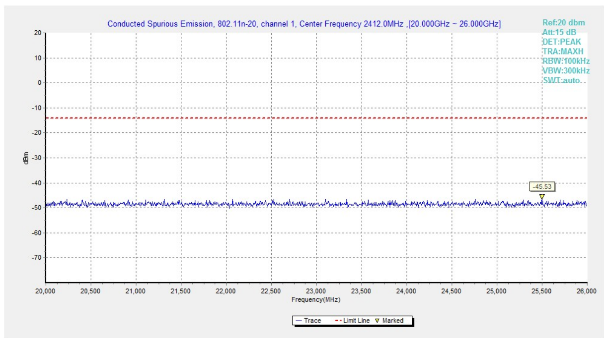
Fig.A.6.1.158 Transmitter Spurious Emission - Conducted (802.11n-HT20, Ch1, 20 GHz-26 GHz)
