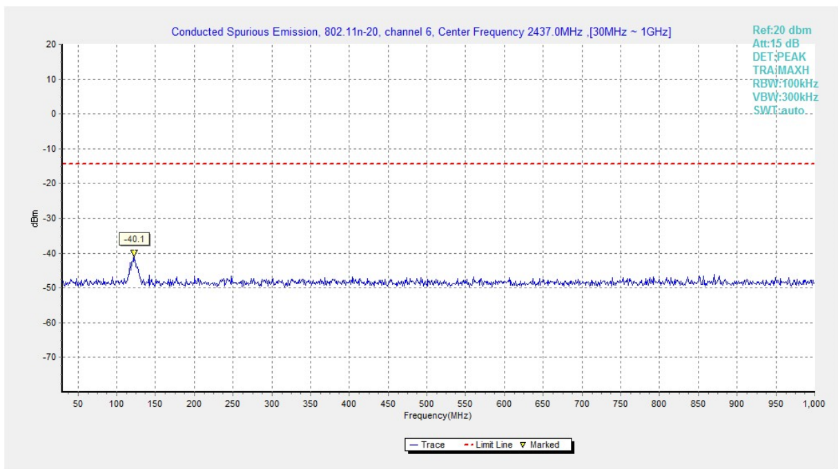
Fig.A.6.1.160 Transmitter Spurious Emission - Conducted (802.11n-HT20, Ch6, 30 MHz-1 GHz)
