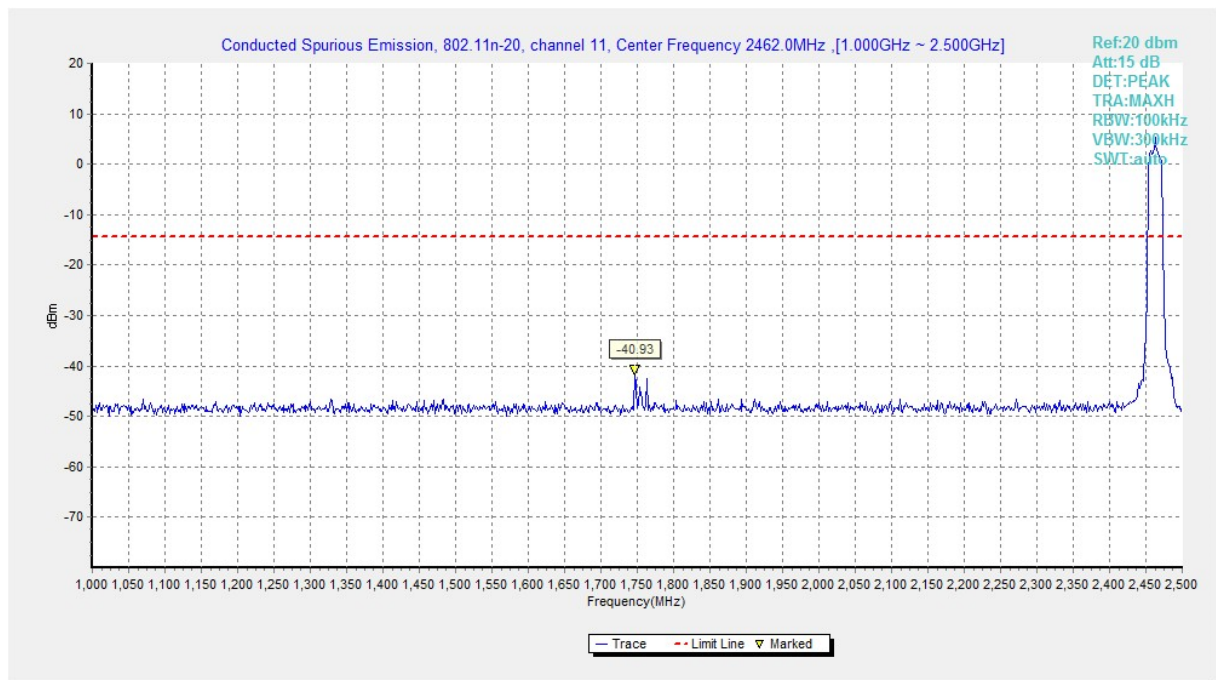
Fig.A.6.1.169 Transmitter Spurious Emission - Conducted (802.11n-HT20, Ch11, 1 GHz-2.5 GHz)
