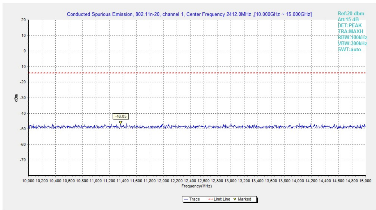
Fig.A.6.1.156 Transmitter Spurious Emission - Conducted (802.11n-HT20, Ch1, 10 GHz-15 GHz)
