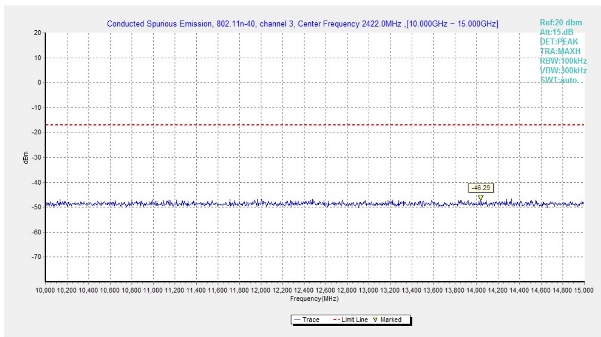
Fig.A.6.1.180 Transmitter Spurious Emission - Conducted (802.11n-HT40, Ch3, 10 GHz-15 GHz)
