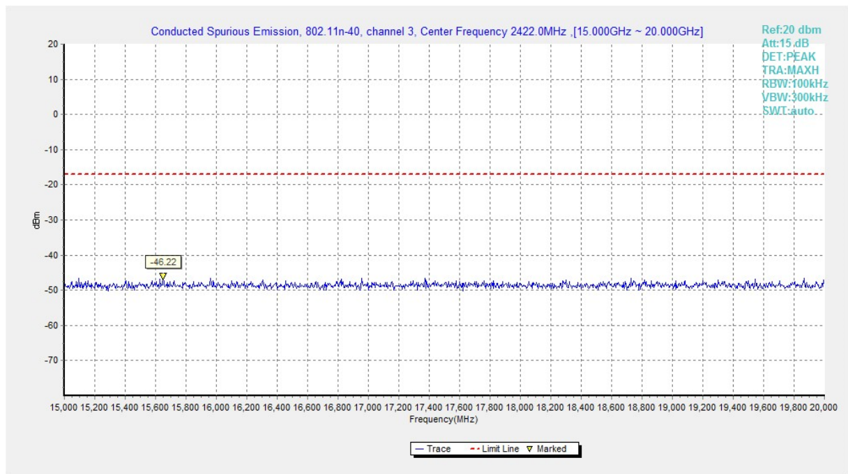
Fig.A.6.1.181 Transmitter Spurious Emission - Conducted (802.11n-HT40, Ch3, 15 GHz-20 GHz)
