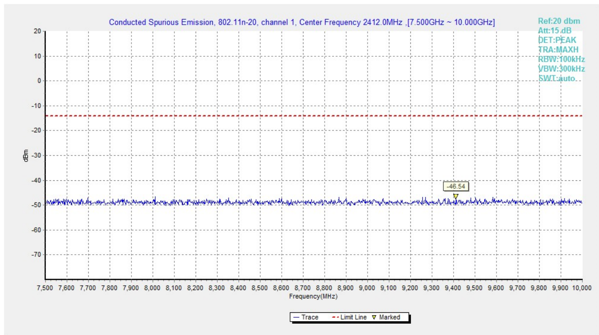
Fig.A.6.1.155 Transmitter Spurious Emission - Conducted (802.11n-HT20, Ch1, 7.5 GHz-10 GHz)
