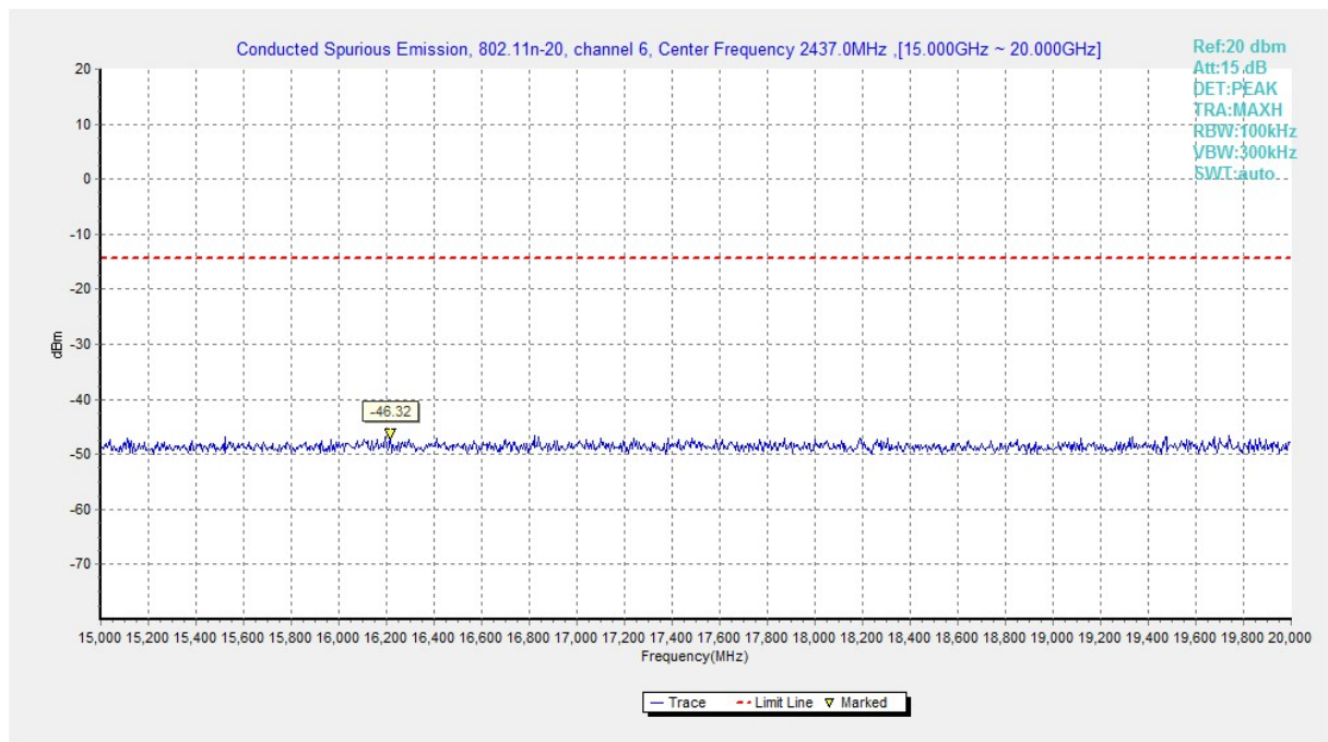
Fig.A.6.1.165 Transmitter Spurious Emission - Conducted (802.11n-HT20, Ch6, 15 GHz-20 GHz)
