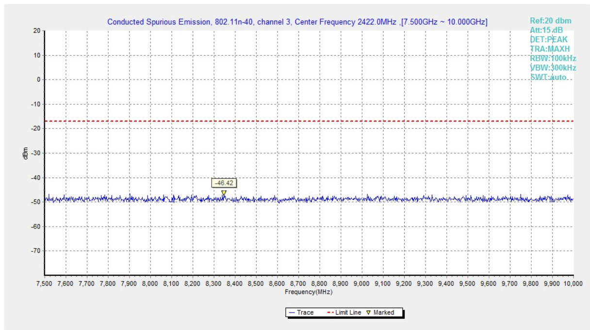
Fig.A.6.1.179 Transmitter Spurious Emission - Conducted (802.11n-HT40, Ch3, 7.5 GHz-10 GHz)
