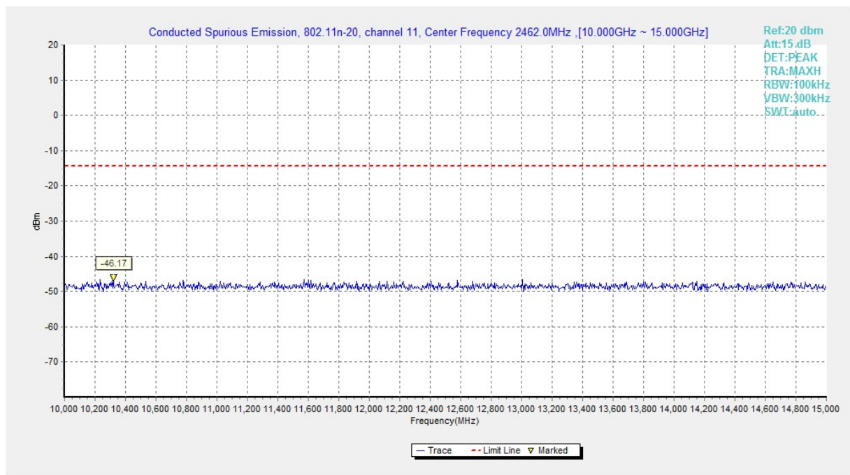
Fig.A.6.1.172 Transmitter Spurious Emission - Conducted (802.11n-HT20, Ch11, 10 GHz-15 GHz)
