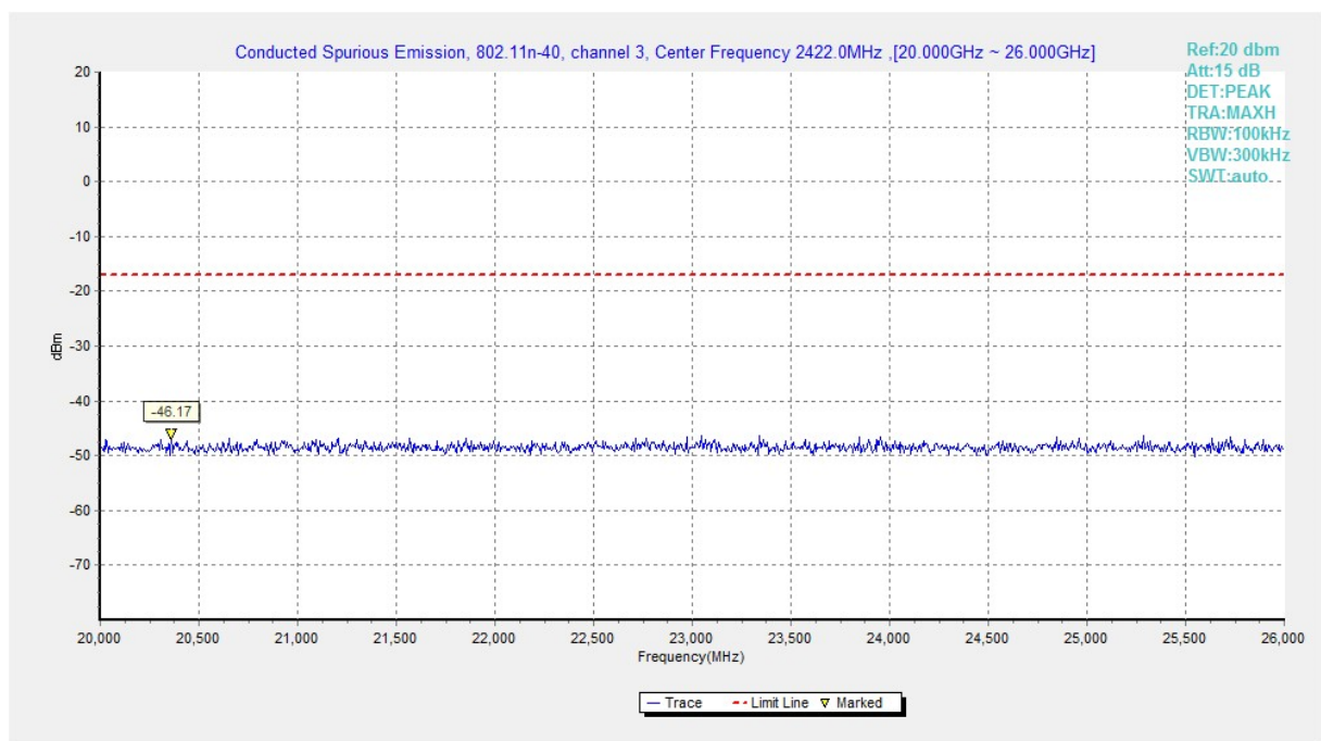
Fig.A.6.1.182 Transmitter Spurious Emission - Conducted (802.11n-HT40, Ch3, 20 GHz-26 GHz)
