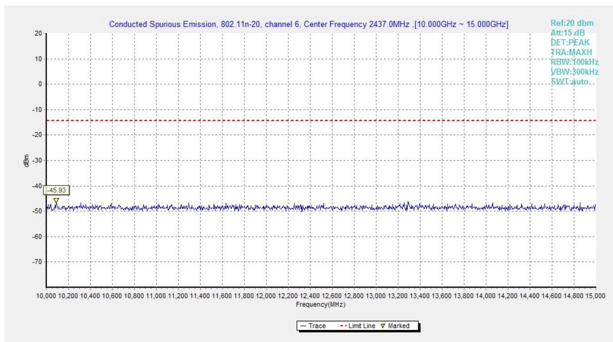
Fig.A.6.1.164 Transmitter Spurious Emission - Conducted (802.11n-HT20, Ch6, 10 GHz-15 GHz)
