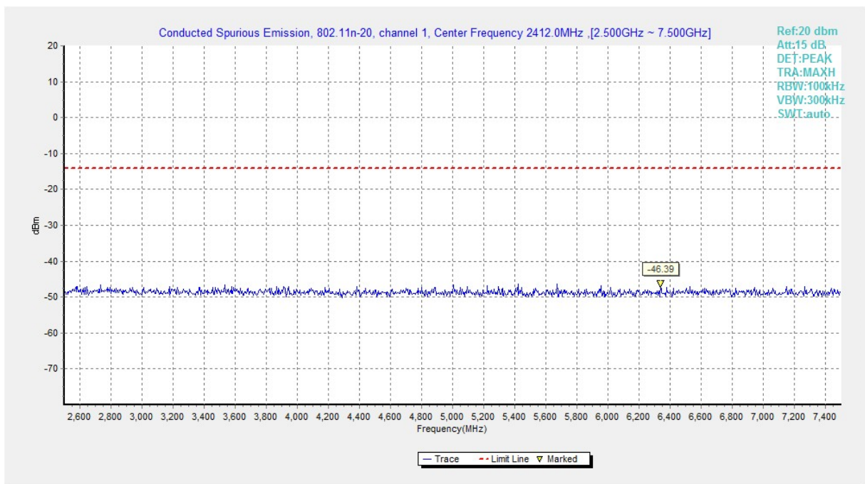
Fig.A.6.1.154 Transmitter Spurious Emission - Conducted (802.11n-HT20, Ch1, 2.5 GHz-7.5 GHz)
