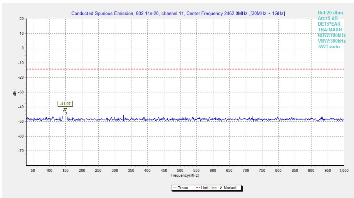
Fig.A.6.1.168 Transmitter Spurious Emission - Conducted (802.11n-HT20, Ch11, 30 MHz-1 GHz)
