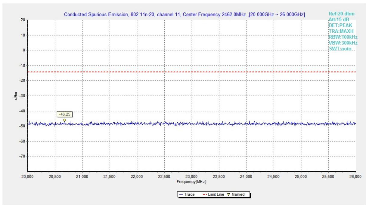
Fig.A.6.1.174 Transmitter Spurious Emission - Conducted (802.11n-HT20, Ch11, 20 GHz-26 GHz)
