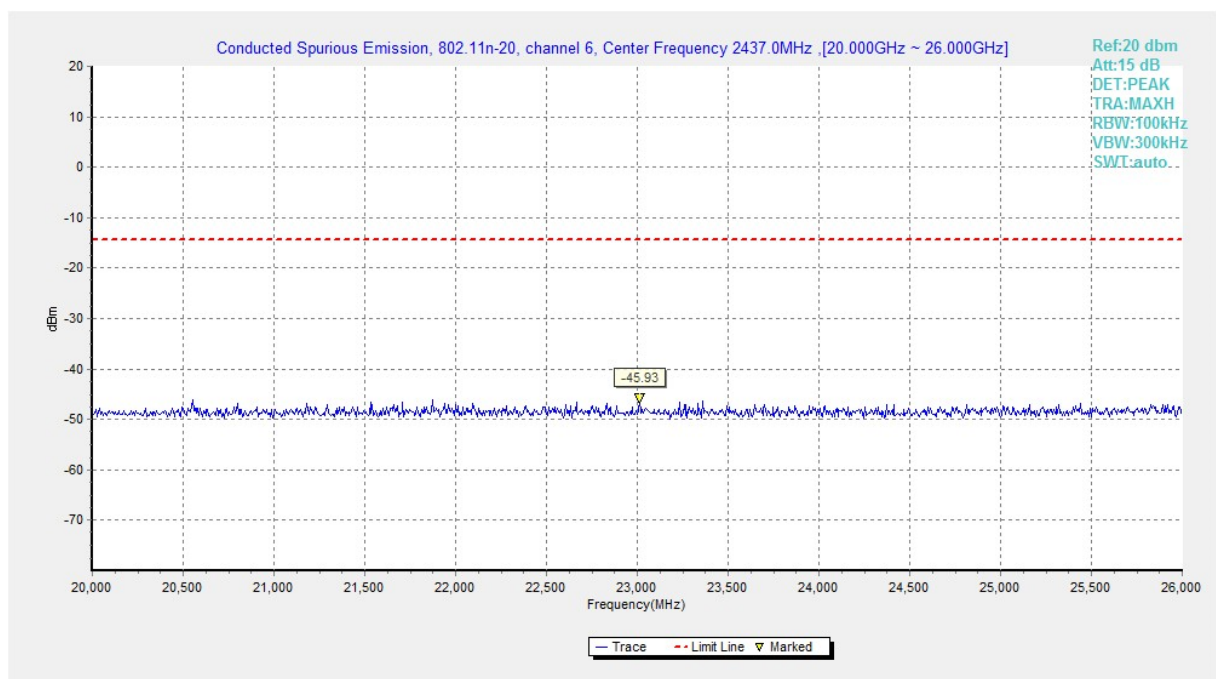
Fig.A.6.1.166 Transmitter Spurious Emission - Conducted (802.11n-HT20, Ch6, 20 GHz-26 GHz)
