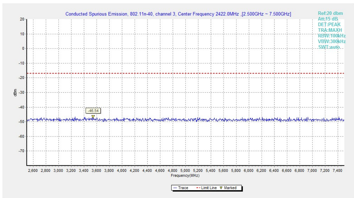
Fig.A.6.1.178 Transmitter Spurious Emission - Conducted (802.11n-HT40, Ch3, 2.5 GHz-7.5 GHz)
