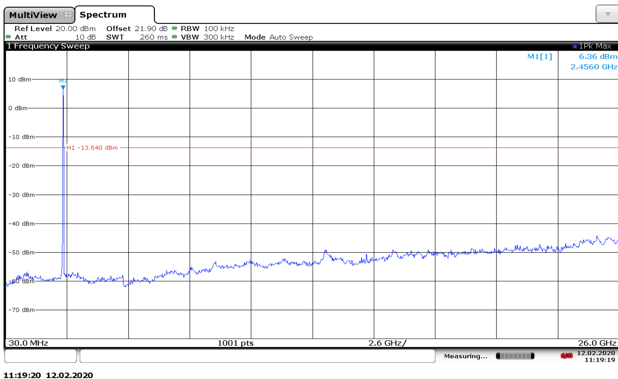
Fig.A.6.1.201 Transmitter Spurious Emission - Conducted (802.11ax-HE20-RU52-middle, Ch11, 30 MHz-26 GHz)
