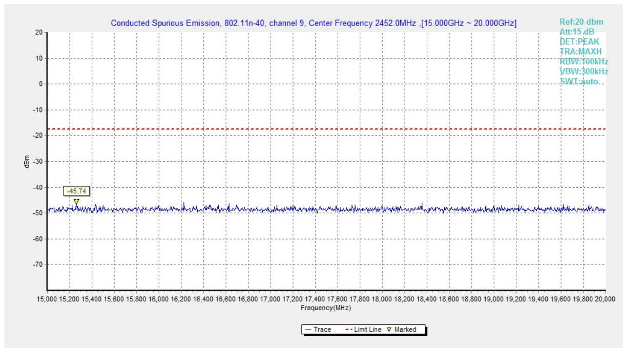
Fig.A.6.1.197 Transmitter Spurious Emission - Conducted (802.11n-HT40, Ch9, 15 GHz-20 GHz)
