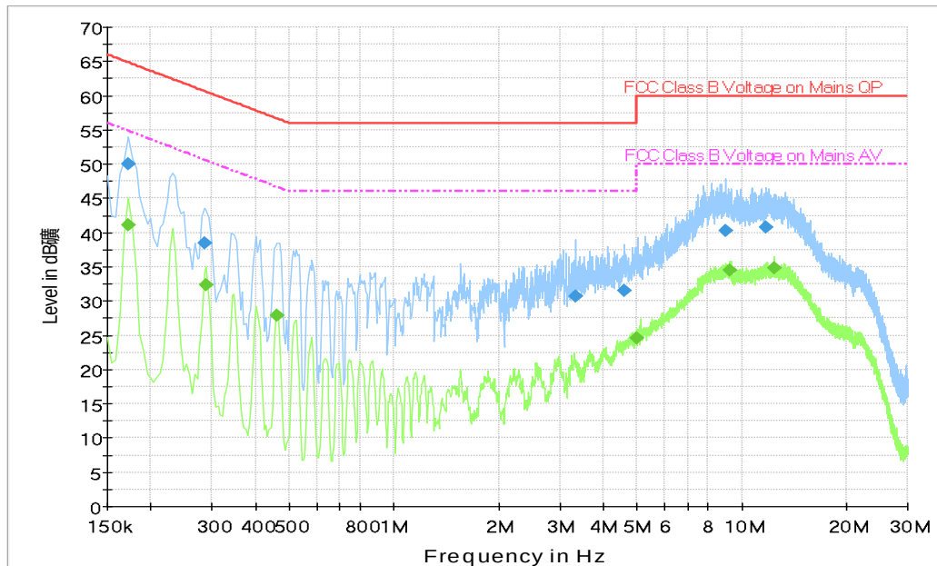
Fig.A.7.2 AC Powerline Conducted Emission-Idle EUT4(M2001J2G)+AE1+AE3+AE6
