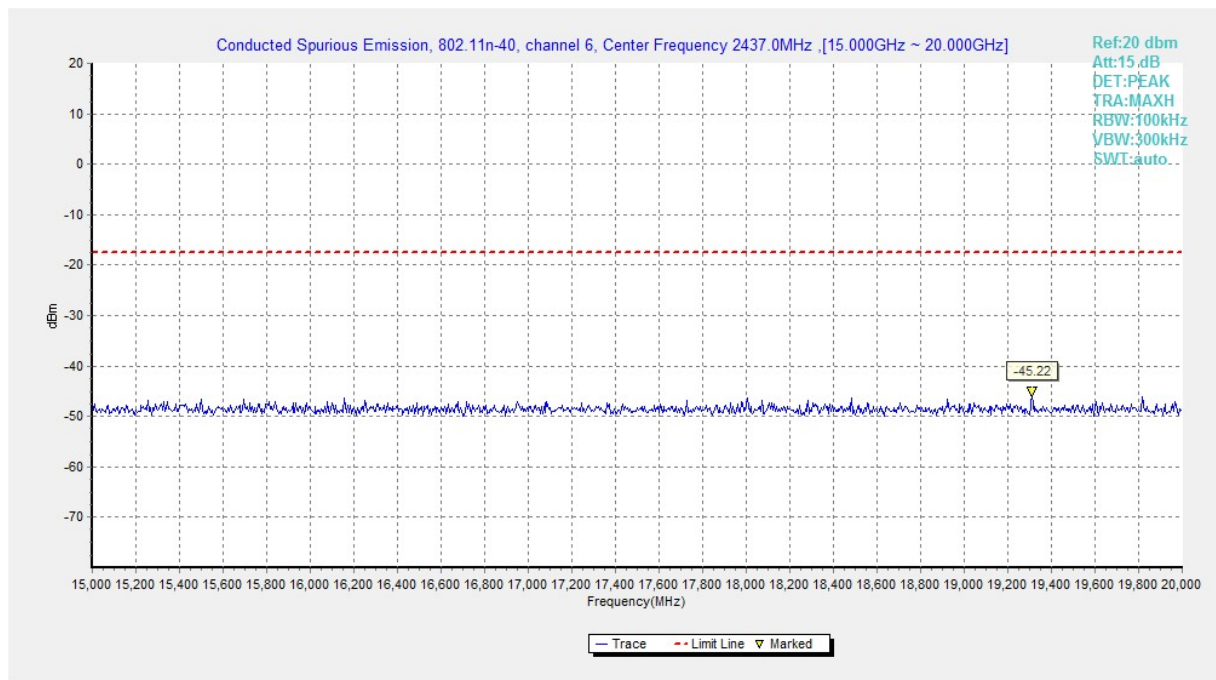
Fig.A.6.1.189 Transmitter Spurious Emission - Conducted (802.11n-HT40, Ch6, 15 GHz-20 GHz)
