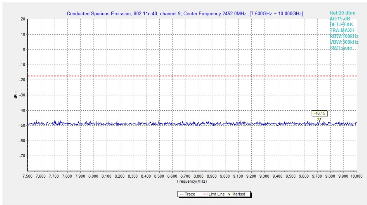
Fig.A.6.1.195 Transmitter Spurious Emission - Conducted (802.11n-HT40, Ch9, 7.5 GHz-10 GHz)
