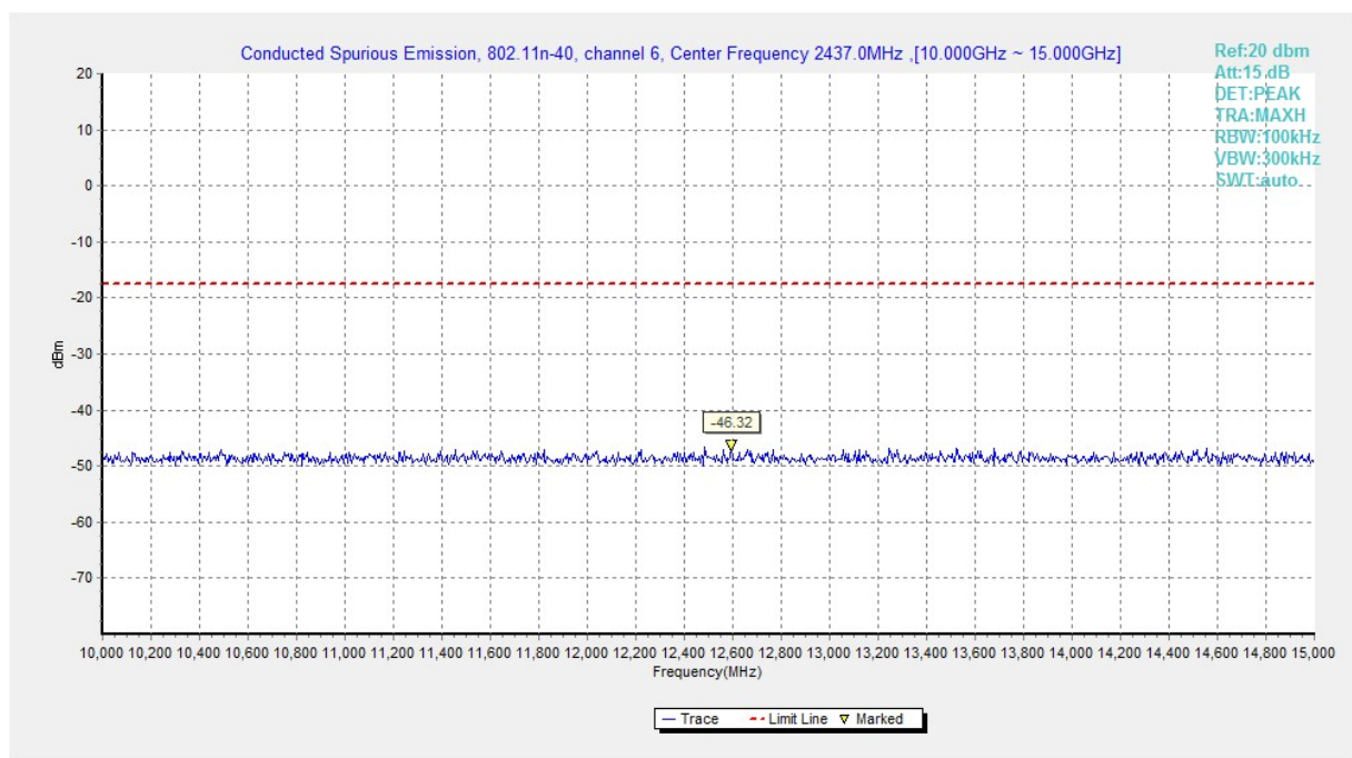
Fig.A.6.1.188 Transmitter Spurious Emission - Conducted (802.11n-HT40, Ch6, 10 GHz-15 GHz)
