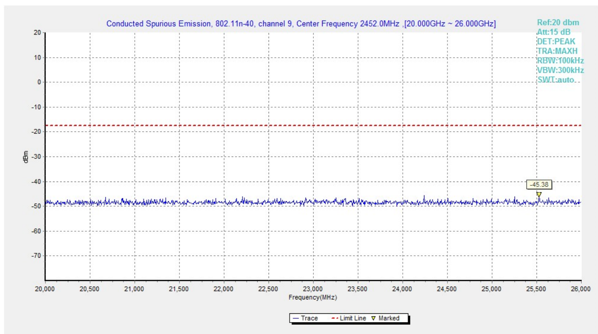
Fig.A.6.1.198 Transmitter Spurious Emission - Conducted (802.11n-HT40, Ch9, 20 GHz-26 GHz)
