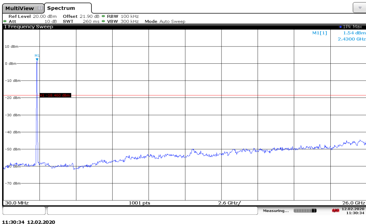
Fig.A.6.1.202 Transmitter Spurious Emission - Conducted (802.11ax-HE40-RU242-right, Ch3, 30 MHz-26 GHz)
