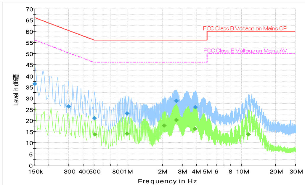
Fig.A.7.3 AC Powerline Conducted Emission-802.11b EUT4(M2001J2G)+AE1+AE3+AE6
