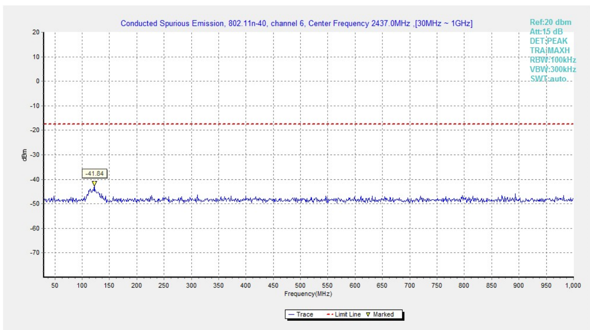
Fig.A.6.1.184 Transmitter Spurious Emission - Conducted (802.11n-HT40, Ch6, 30 MHz-1 GHz)
