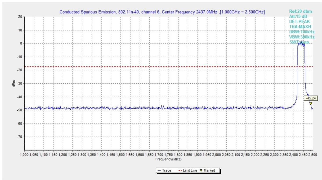
Fig.A.6.1.185 Transmitter Spurious Emission - Conducted (802.11n-HT40, Ch6, 1 GHz-2.5 GHz)
