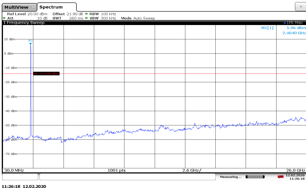
Fig.A.6.1.199 Transmitter Spurious Emission - Conducted (802.11ax-HE20-RU52-middle, Ch1, 30 MHz-26 GHz)
