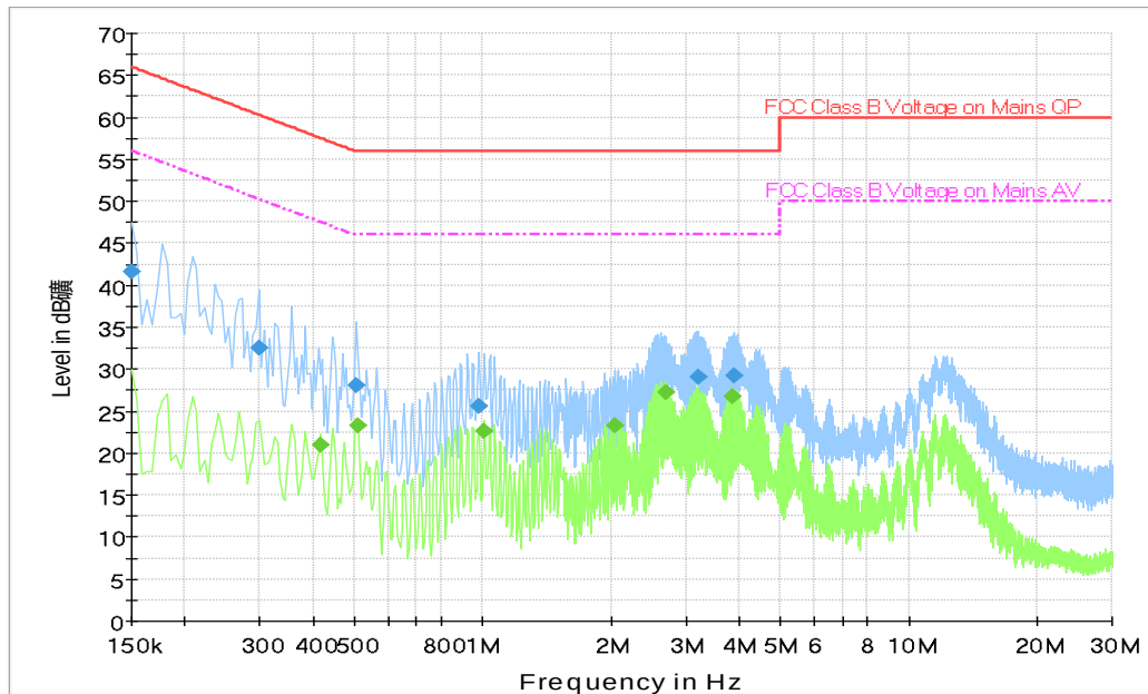
Fig.A.7.4 AC Powerline Conducted Emission-Idle EUT4(M2001J2G)+AE1+AE3+AE6
