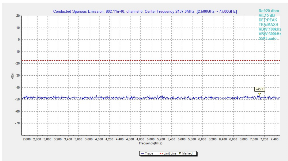
Fig.A.6.1.186 Transmitter Spurious Emission - Conducted (802.11n-HT40, Ch6, 2.5 GHz-7.5 GHz)
