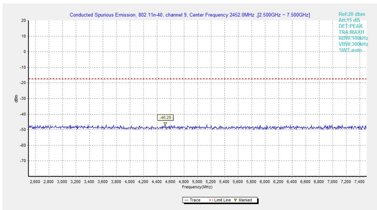
Fig.A.6.1.194 Transmitter Spurious Emission - Conducted (802.11n-HT40, Ch9, 2.5 GHz-7.5 GHz)
