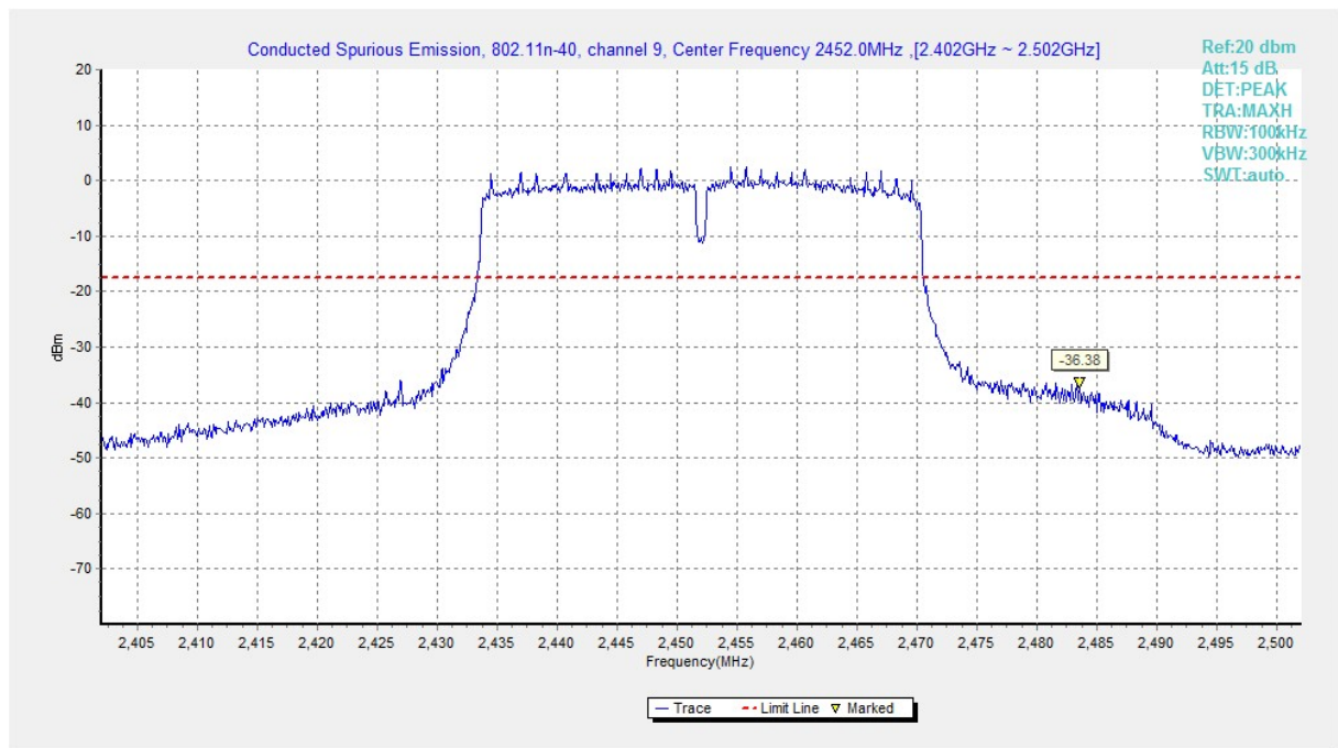
Fig.A.6.1.191 Transmitter Spurious Emission - Conducted (802.11n-HT40, Ch9, Center Frequency)
