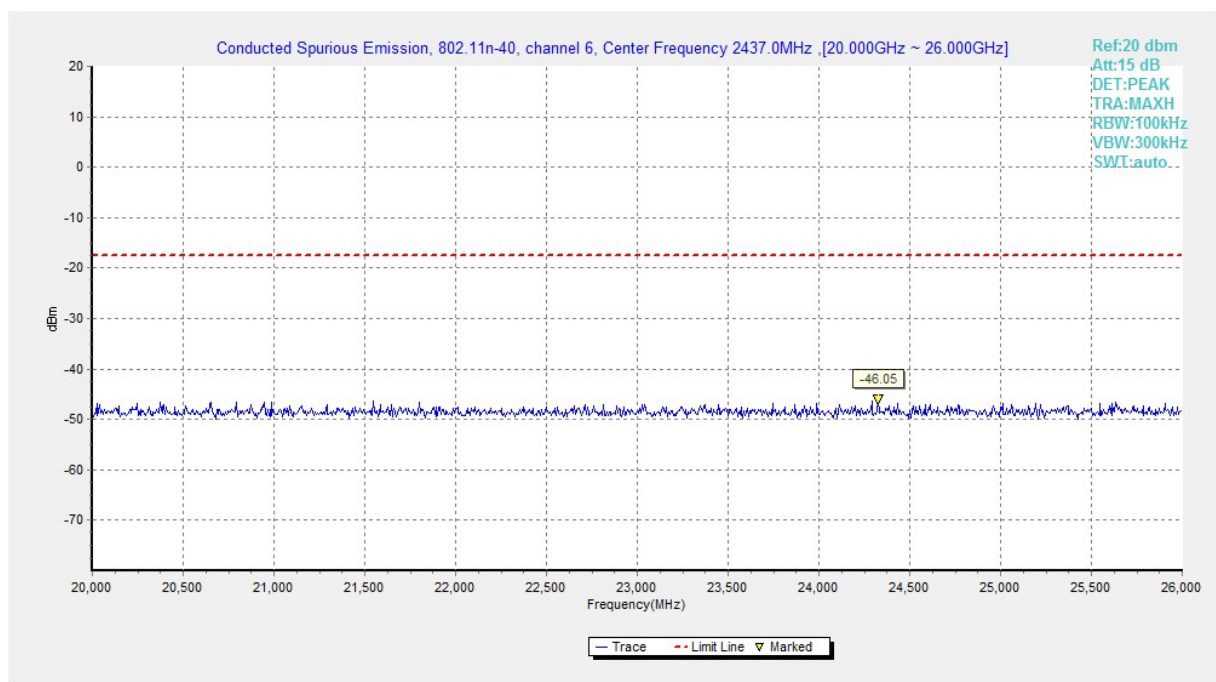
Fig.A.6.1.190 Transmitter Spurious Emission - Conducted (802.11n-HT40, Ch6, 20 GHz-26 GHz)
