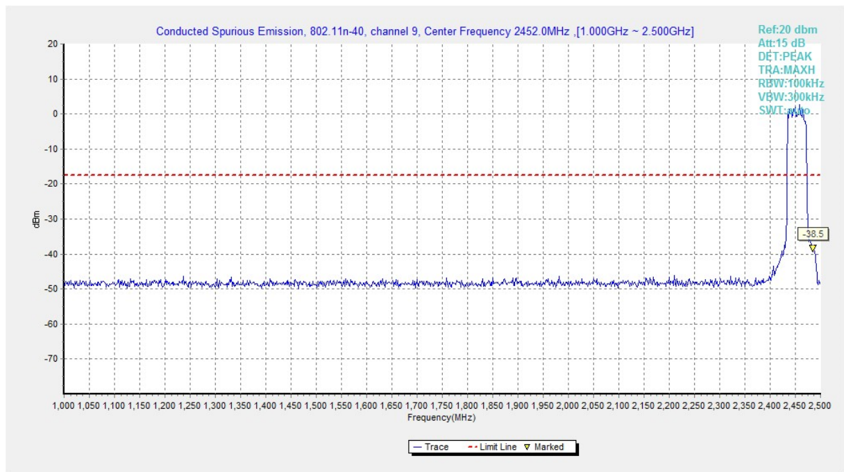
Fig.A.6.1.193 Transmitter Spurious Emission - Conducted (802.11n-HT40, Ch9, 1 GHz-2.5 GHz)
