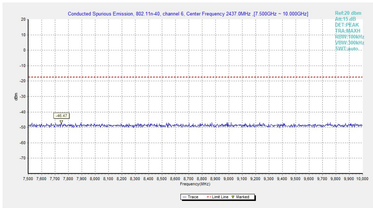
Fig.A.6.1.187 Transmitter Spurious Emission - Conducted (802.11n-HT40, Ch6, 7.5 GHz-10 GHz)
