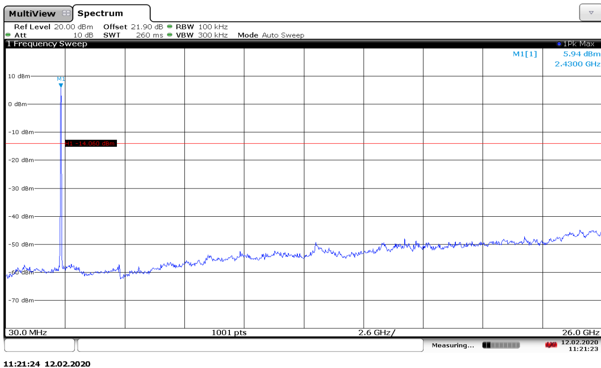
Fig.A.6.1.200 Transmitter Spurious Emission - Conducted (802.11ax-HE20-RU52-middle, Ch6, 30 MHz-26 GHz)
