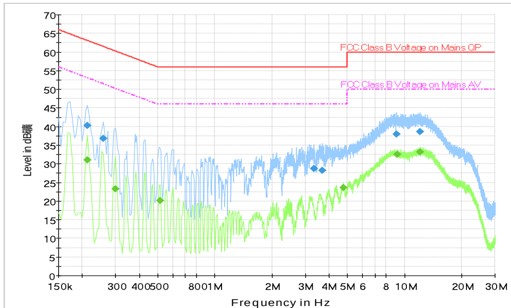
Fig.A.7.1 AC Powerline Conducted Emission-802.11b EUT4(M2001J2G)+AE1+AE3+AE6
