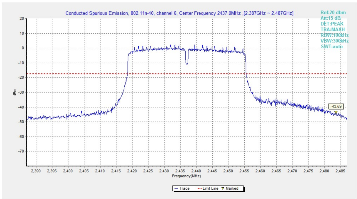
Fig.A.6.1.183 Transmitter Spurious Emission - Conducted (802.11n-HT40, Ch6, Center Frequency)
