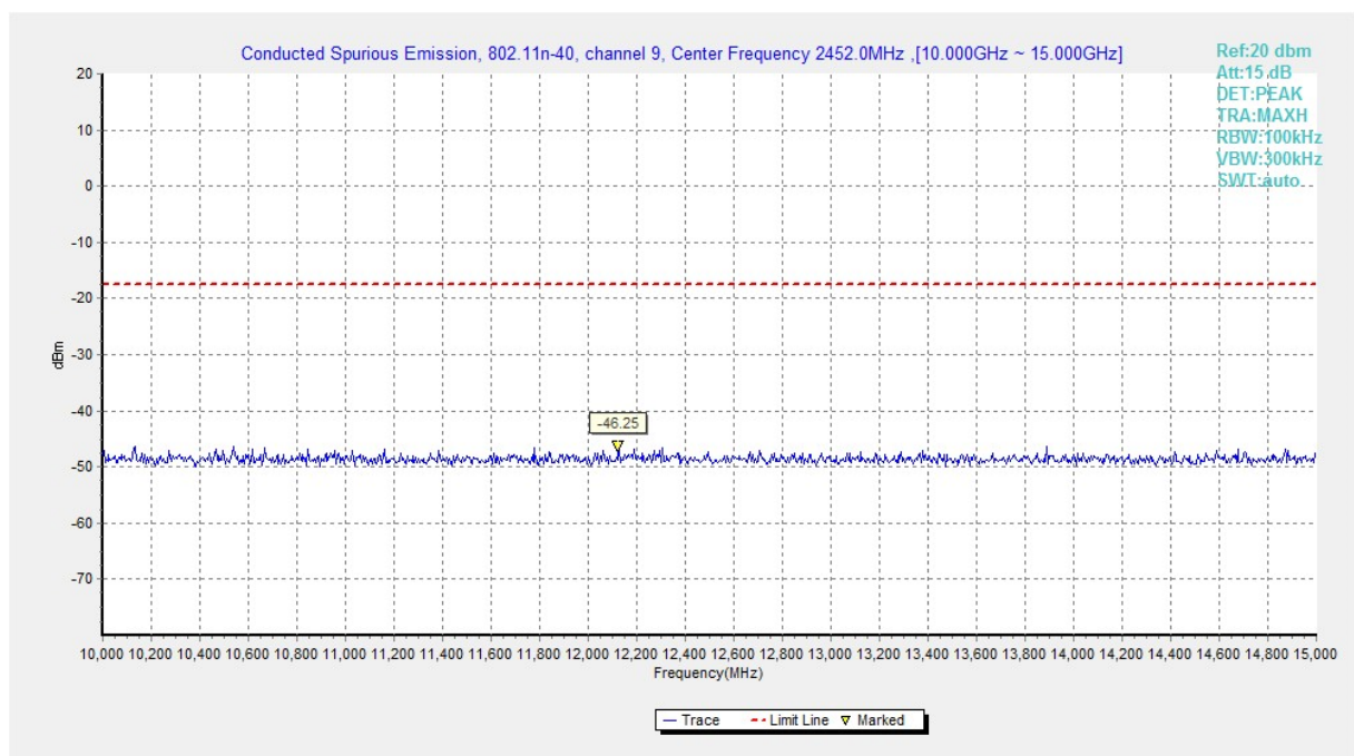
Fig.A.6.1.196 Transmitter Spurious Emission - Conducted (802.11n-HT40, Ch9, 10 GHz-15 GHz)
