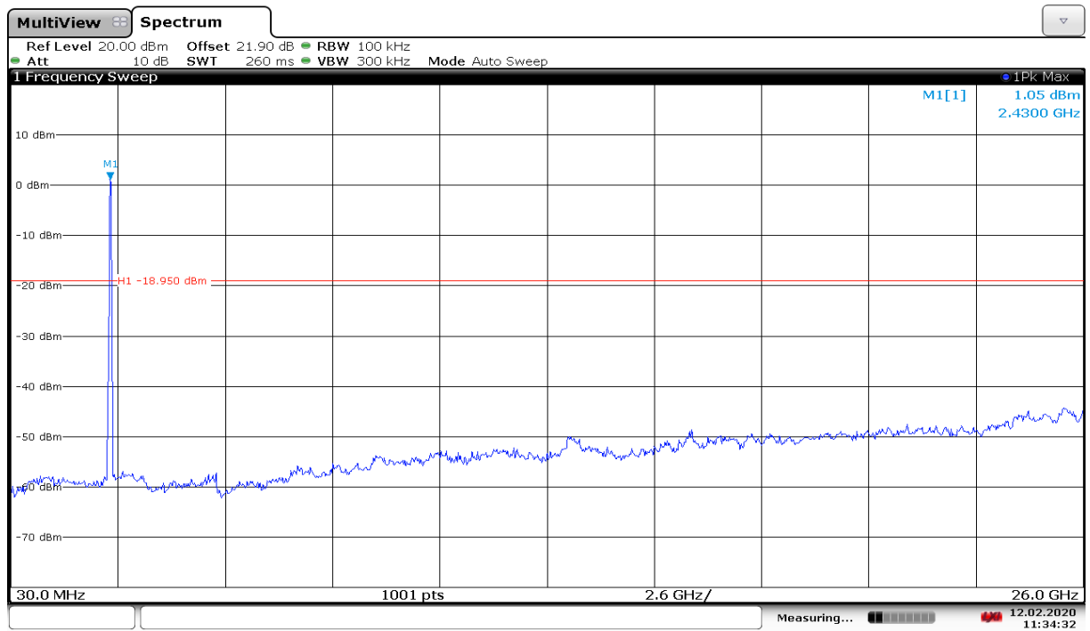
Fig.A.6.1.203 Transmitter Spurious Emission - Conducted (802.11ax-HE40-RU242-right, Ch6, 30 MHz-26 GHz)
