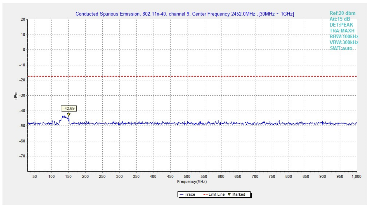
Fig.A.6.1.192 Transmitter Spurious Emission - Conducted (802.11n-HT40, Ch9, 30 MHz-1 GHz)
