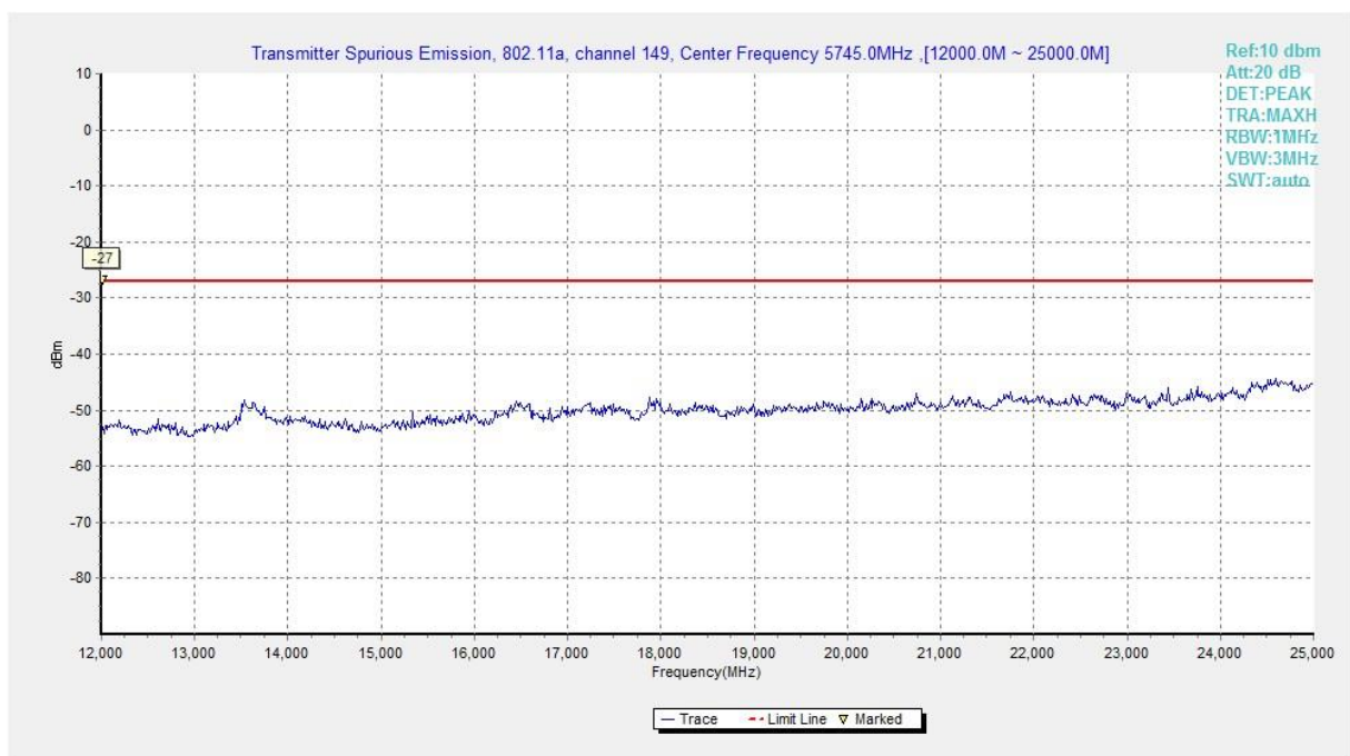
Fig. 5 Conducted Spurious Emission (802.11a, Ch149, 12 GHz-25 GHz)
