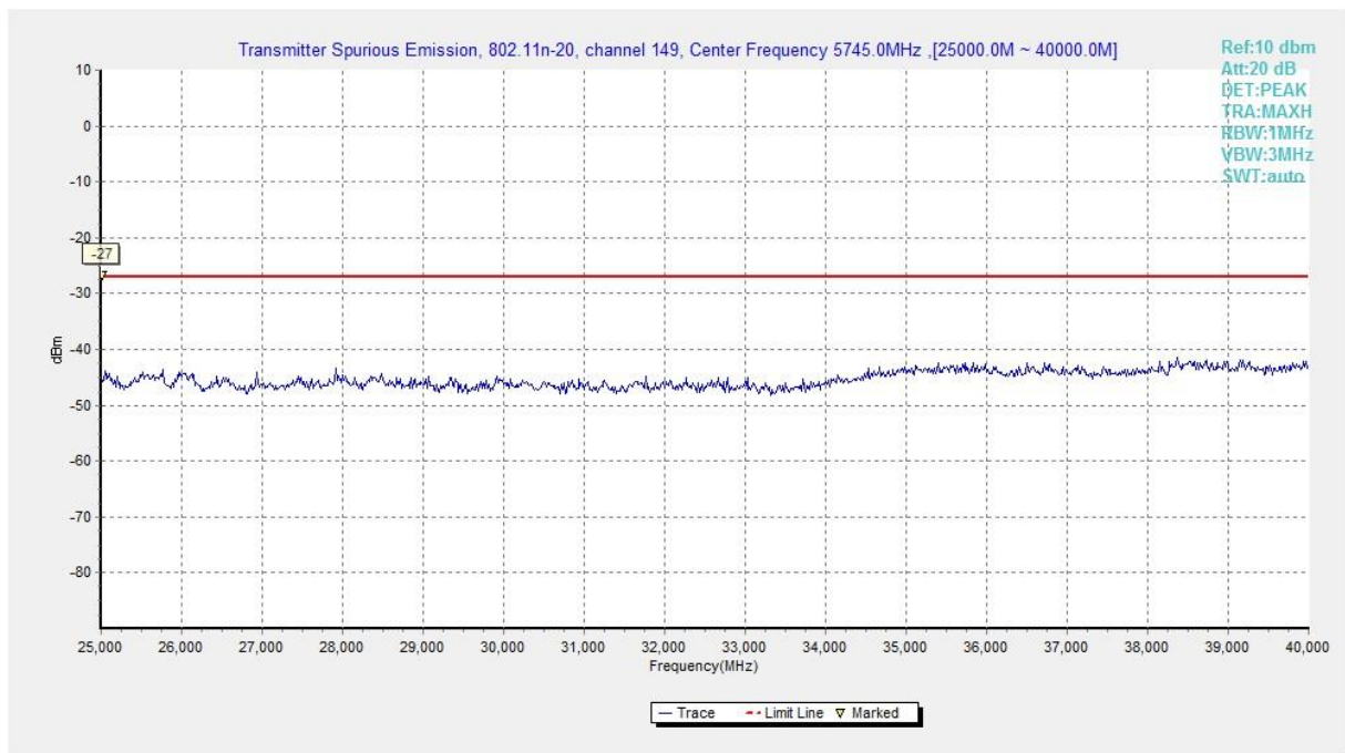
Fig. 18 Conducted Spurious Emission (802.11n-HT20, Ch149, 25 GHz-40 GHz)
