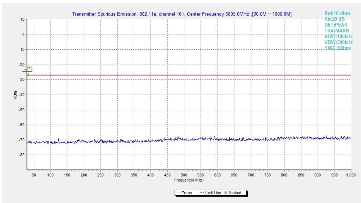
Fig. 11 Conducted Spurious Emission (802.11a, Ch161, 30 MHz-1 GHz)
