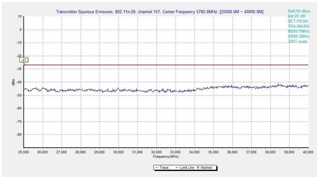
Fig. 22 Conducted Spurious Emission (802.11n-HT20, Ch157, 25 GHz-40 GHz)
