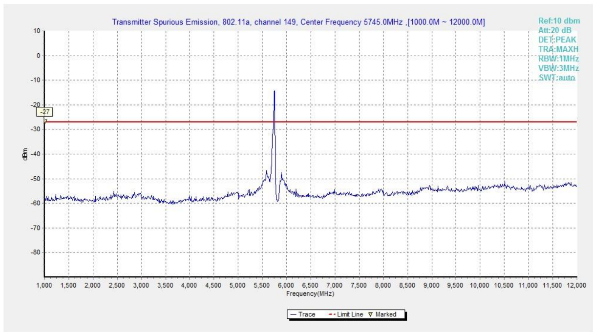
Fig. 4 Conducted Spurious Emission (802.11a, Ch149, 1 GHz -12 GHz)
