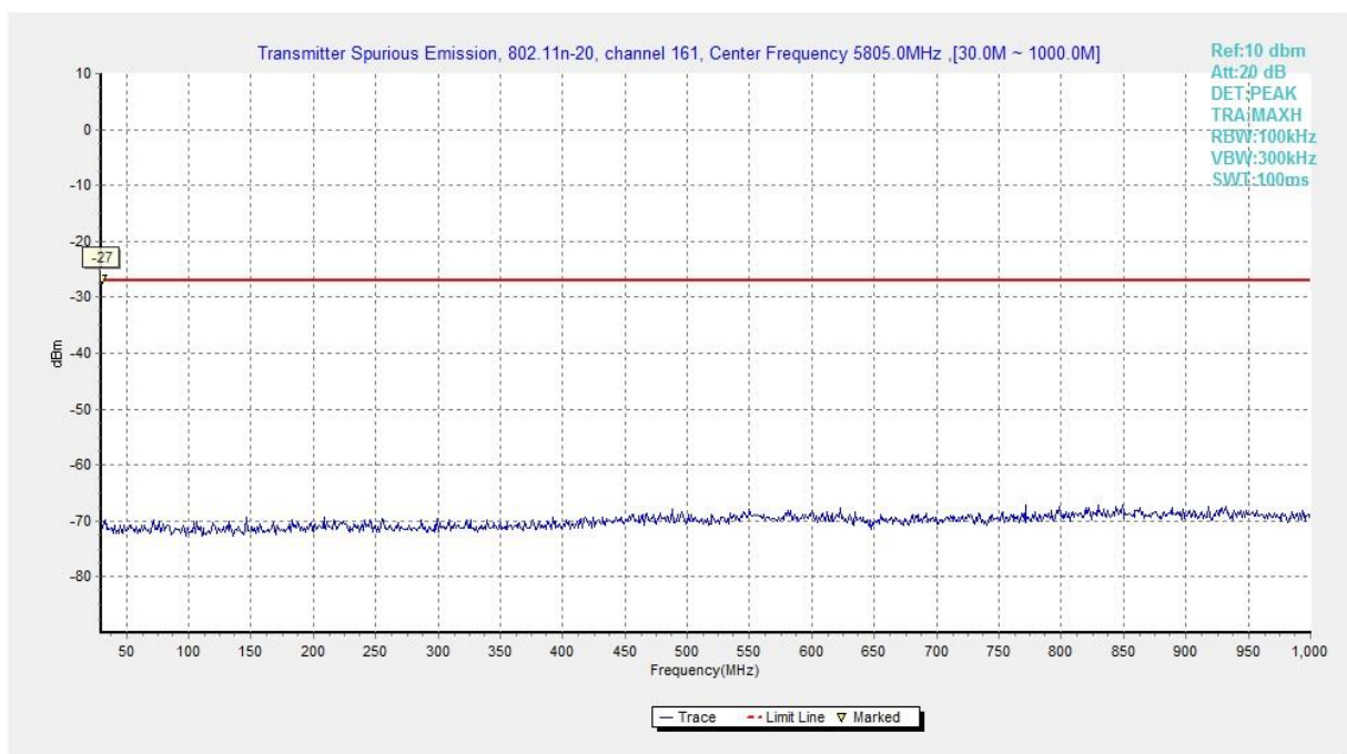
Fig. 23 Conducted Spurious Emission (802.11n-HT20, Ch161, 30 MHz-1 GHz)
