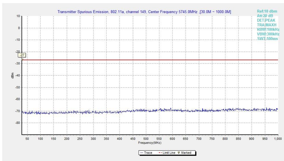
Fig. 3 Conducted Spurious Emission (802.11a, Ch149, 30 MHz-1 GHz)
