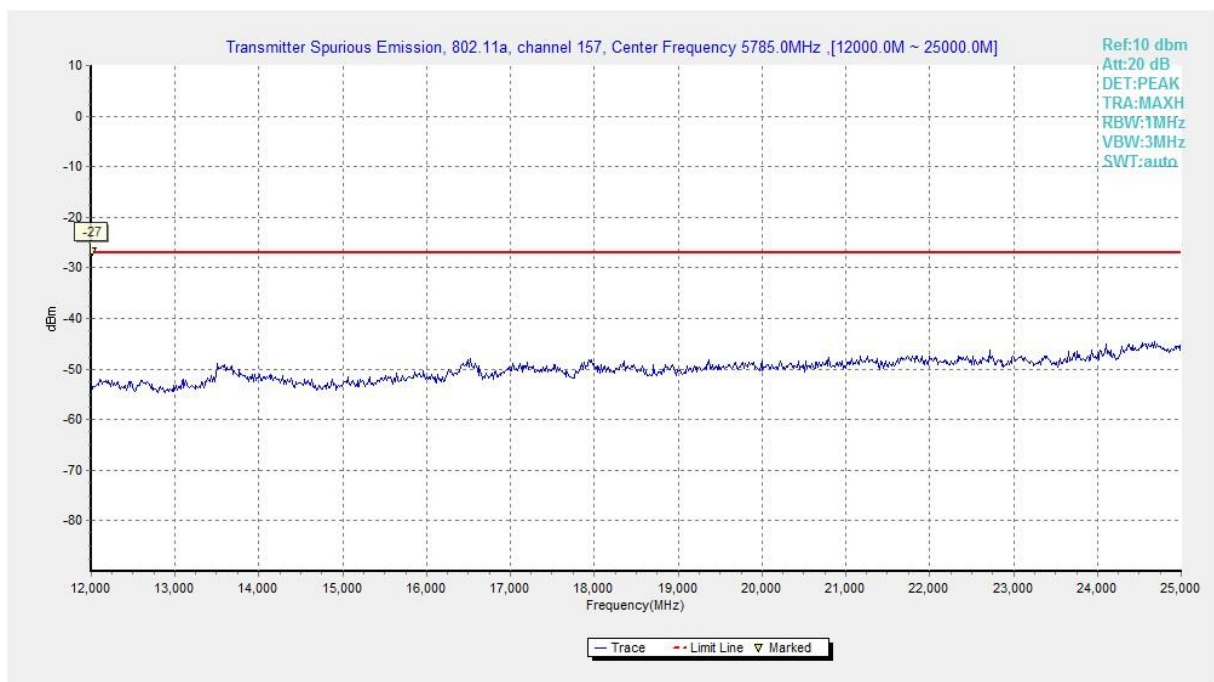
Fig. 9 Conducted Spurious Emission (802.11a, Ch157, 12 GHz-25 GHz)
