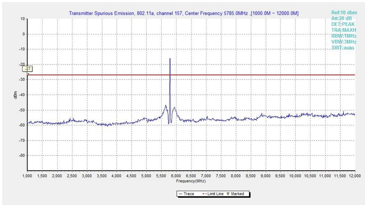
Fig. 8 Conducted Spurious Emission (802.11a, Ch157, 1 GHz -12 GHz)
