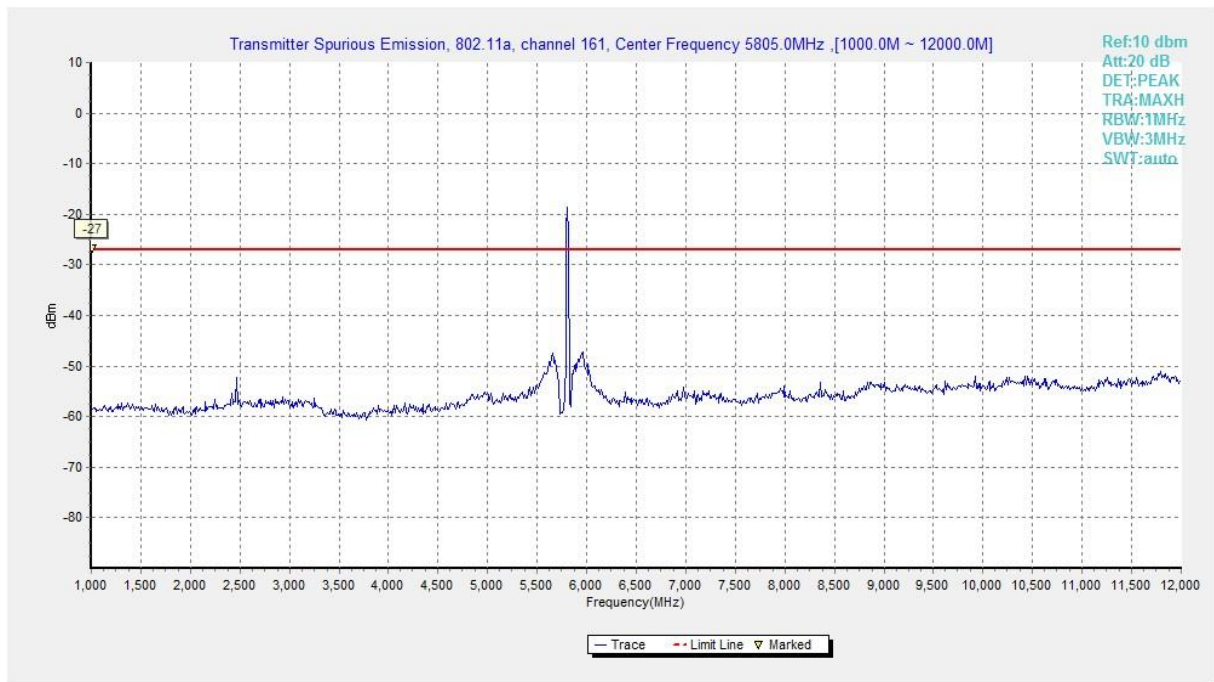
Fig. 12 Conducted Spurious Emission (802.11a, Ch161, 1 GHz -12 GHz)
