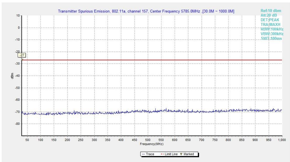
Fig. 7 Conducted Spurious Emission (802.11a, Ch157, 30 MHz-1 GHz)
