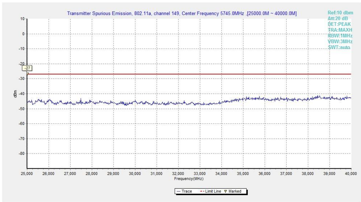
Fig. 6 Conducted Spurious Emission (802.11a, Ch149, 25 GHz-40 GHz)
