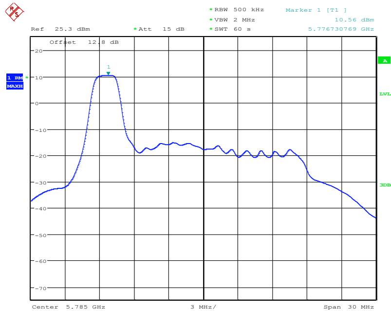
Fig.1 ANT3 802.11ax-HE20 RU26-left ch157
