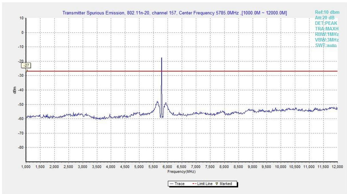
Fig. 20 Conducted Spurious Emission (802.11n-HT20, Ch157, 1 GHz -12 GHz)
