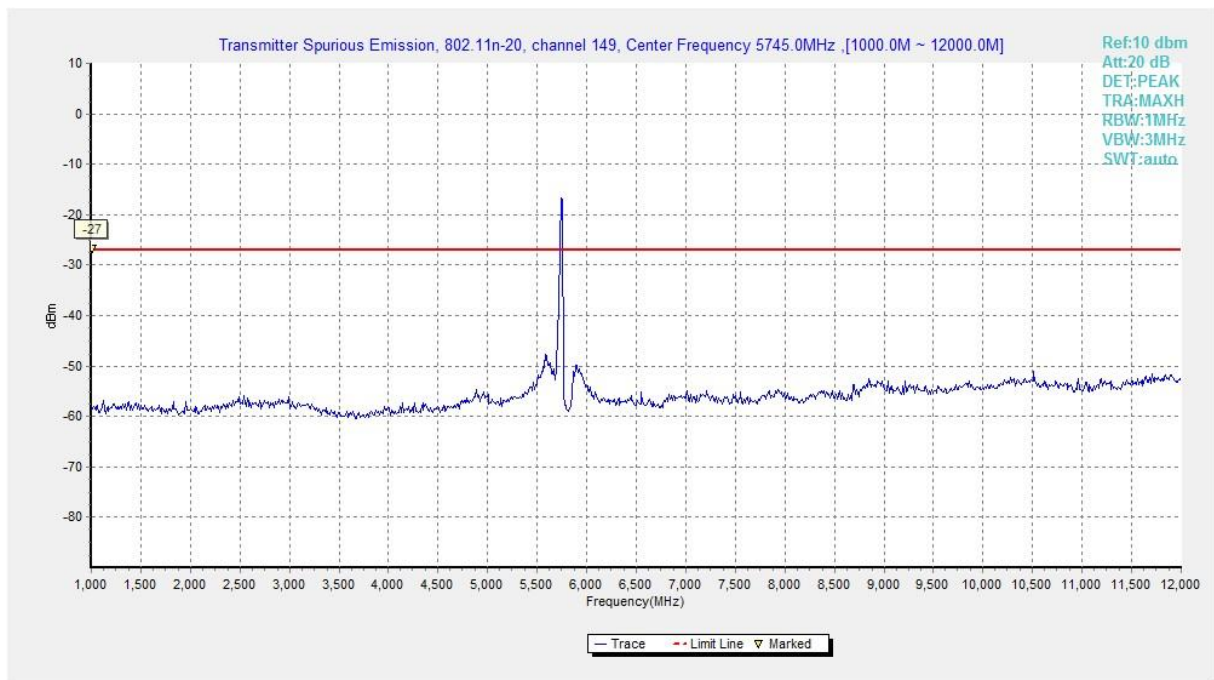
Fig. 16 Conducted Spurious Emission (802.11n-HT20, Ch149, 1 GHz -12 GHz)
