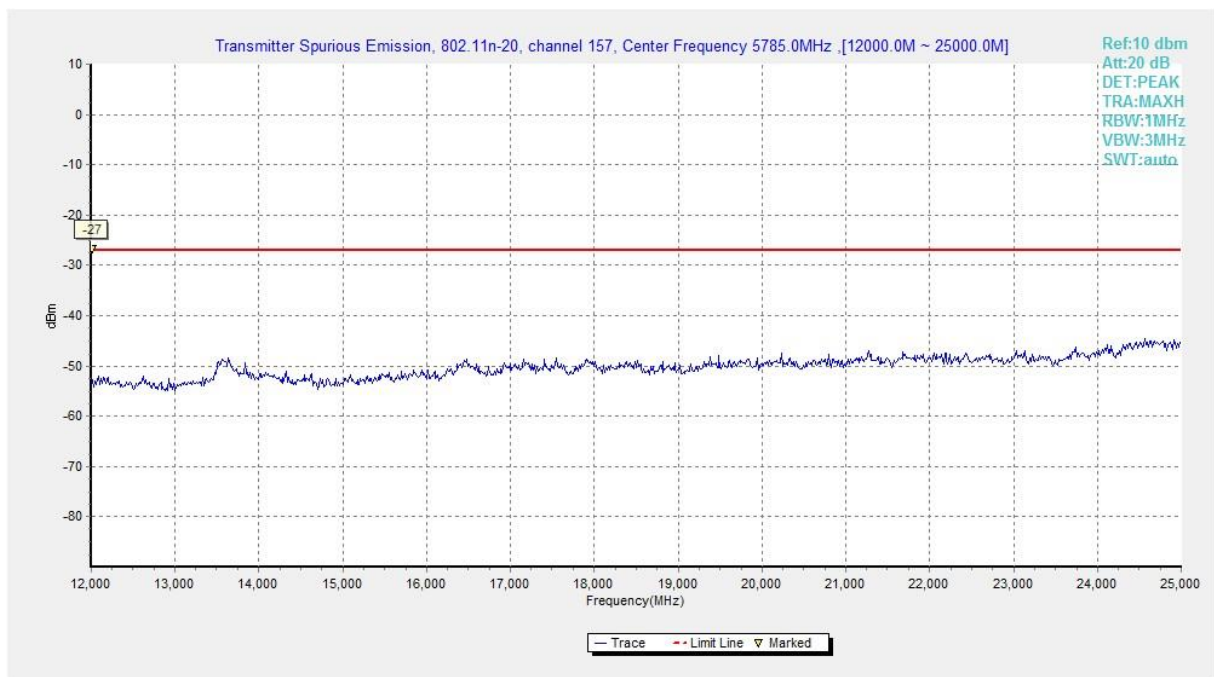
Fig. 21 Conducted Spurious Emission (802.11n-HT20, Ch157, 12 GHz-25 GHz)
