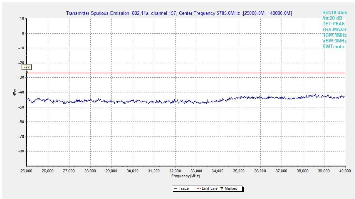
Fig. 10 Conducted Spurious Emission (802.11a, Ch157, 25 GHz-40 GHz)
