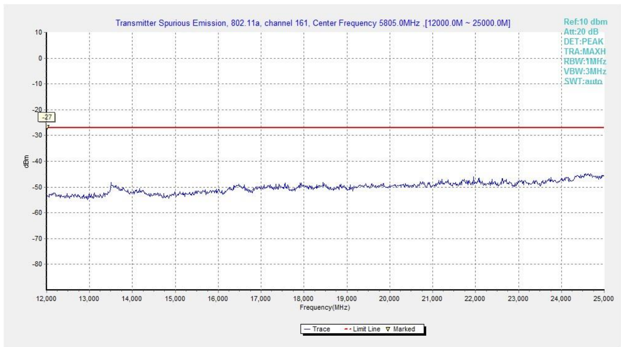
Fig. 13 Conducted Spurious Emission (802.11a, Ch161, 12 GHz-25 GHz)
