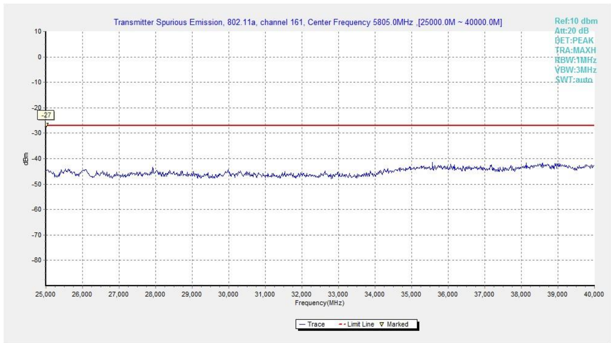
Fig. 14 Conducted Spurious Emission (802.11a, Ch161, 25 GHz-40 GHz)
