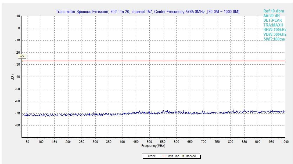
Fig. 19 Conducted Spurious Emission (802.11n-HT20, Ch157, 30 MHz-1 GHz)
