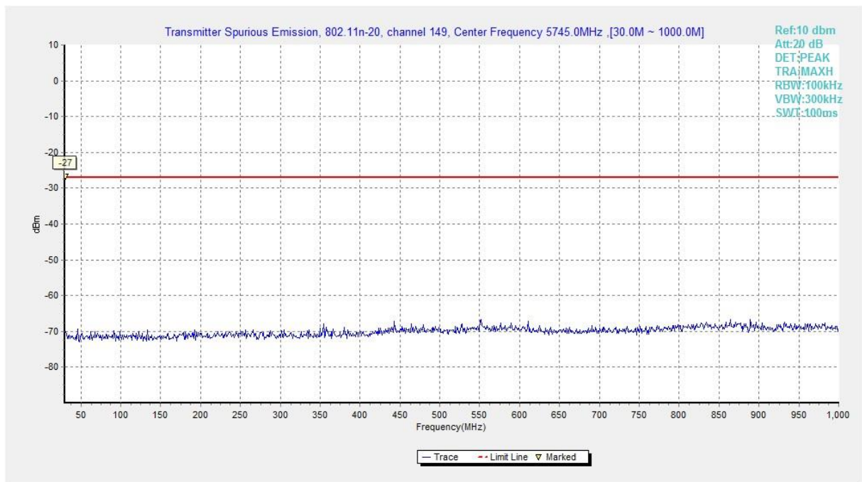
Fig. 15 Conducted Spurious Emission (802.11n-HT20, Ch149, 30 MHz-1 GHz)
