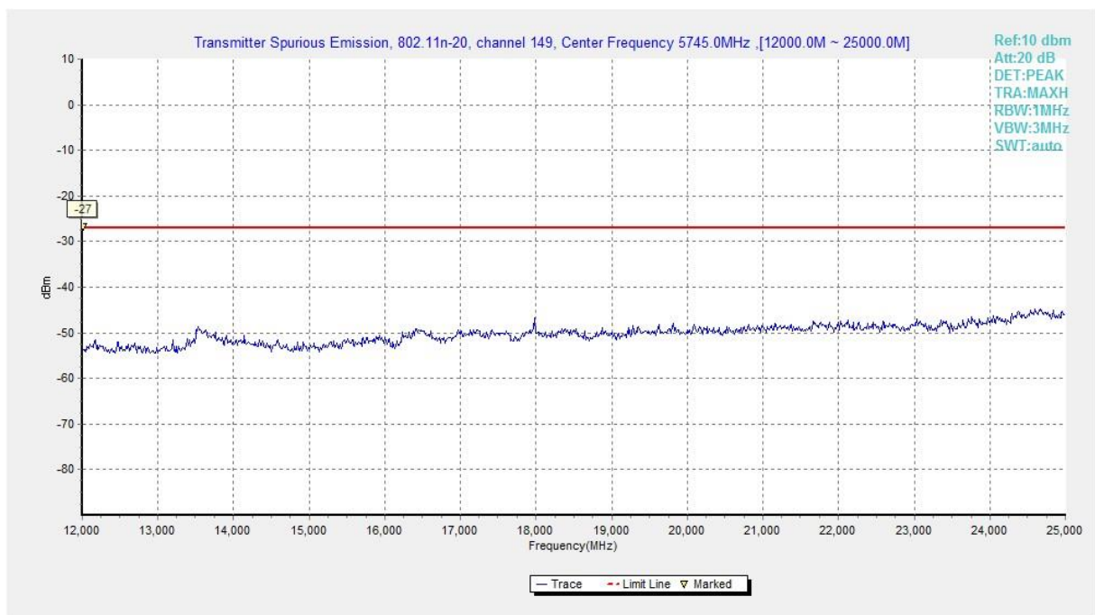
Fig. 17 Conducted Spurious Emission (802.11n-HT20, Ch149, 12 GHz-25 GHz)
