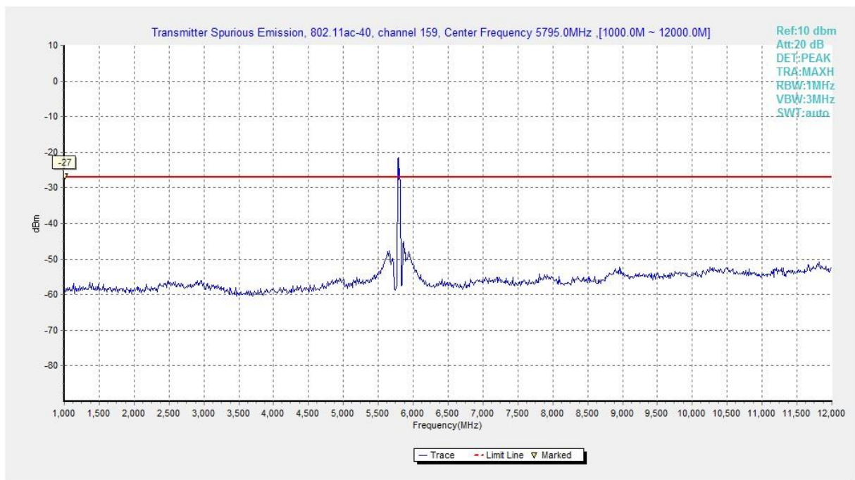
Fig. 52 Conducted Spurious Emission (802.11ac-HT40, Ch159, 1 GHz -12 GHz)
