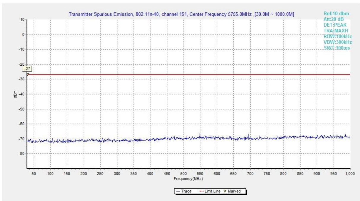
Fig. 39 Conducted Spurious Emission (802.11n-HT40, Ch151, 30 MHz-1 GHz)
