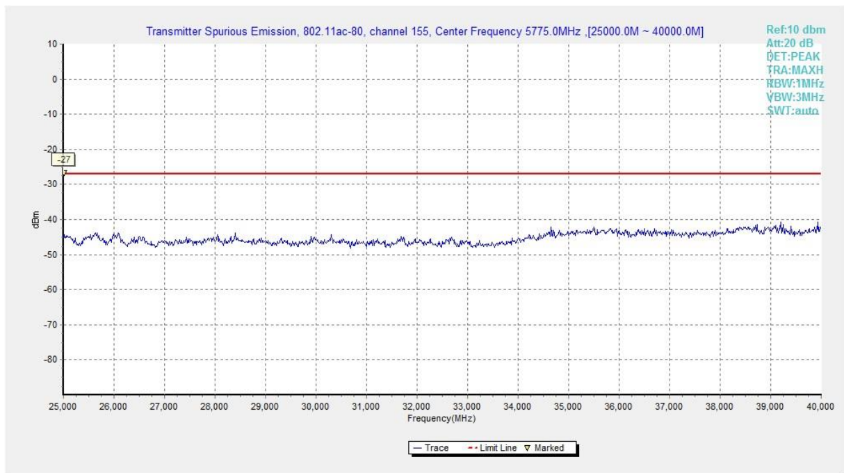
Fig. 58 Conducted Spurious Emission (802.11ac-HT80, Ch155, 25 GHz-40 GHz)
