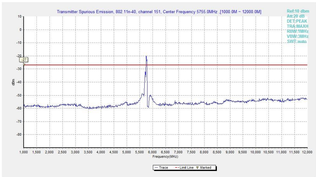
Fig. 40 Conducted Spurious Emission (802.11n-HT40, Ch151, 1 GHz -12 GHz)
