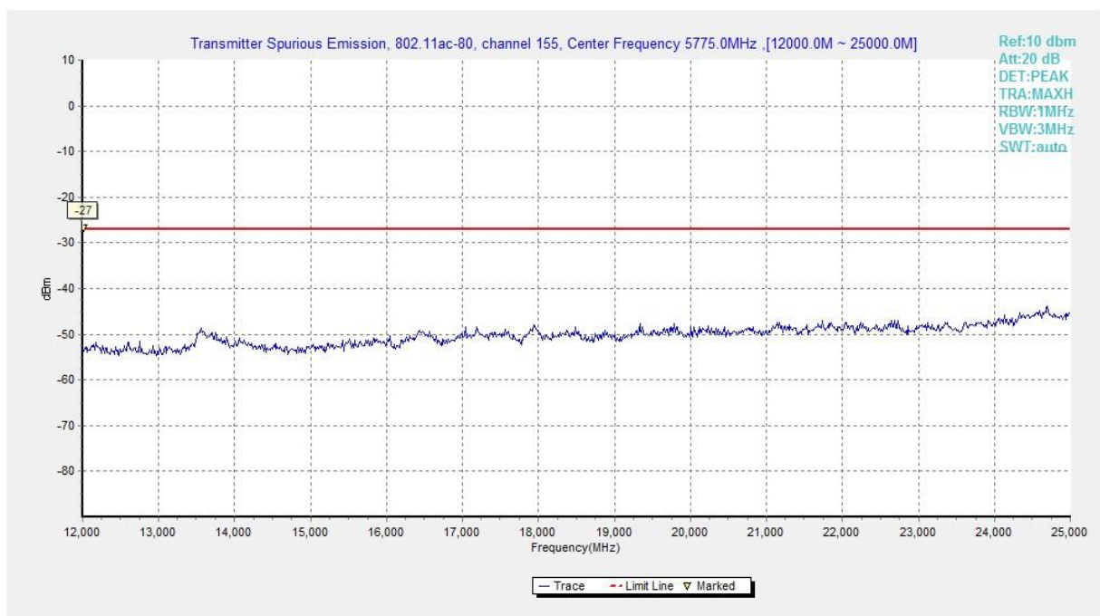
Fig. 57 Conducted Spurious Emission (802.11ac-HT80, Ch155, 12 GHz-25 GHz)
