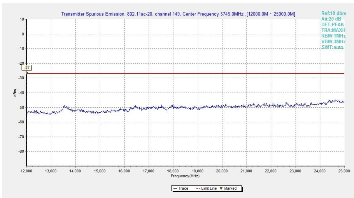
Fig. 29 Conducted Spurious Emission (802.11ac-HT20, Ch149, 12 GHz-25 GHz)
