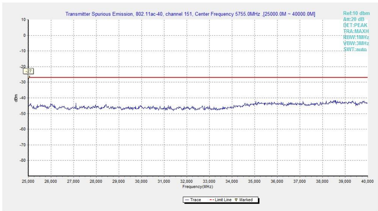
Fig. 50 Conducted Spurious Emission (802.11ac-HT40, Ch151, 25 GHz-40 GHz)
