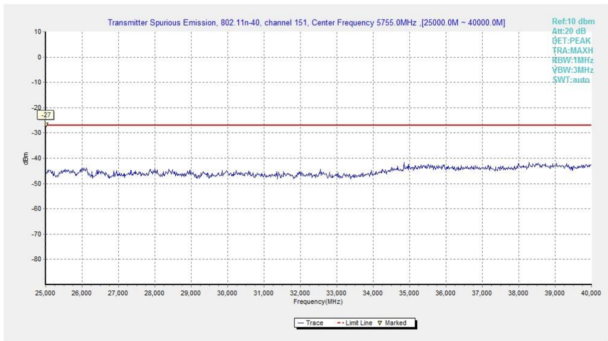
Fig. 42 Conducted Spurious Emission (802.11n-HT40, Ch151, 25 GHz-40 GHz)
