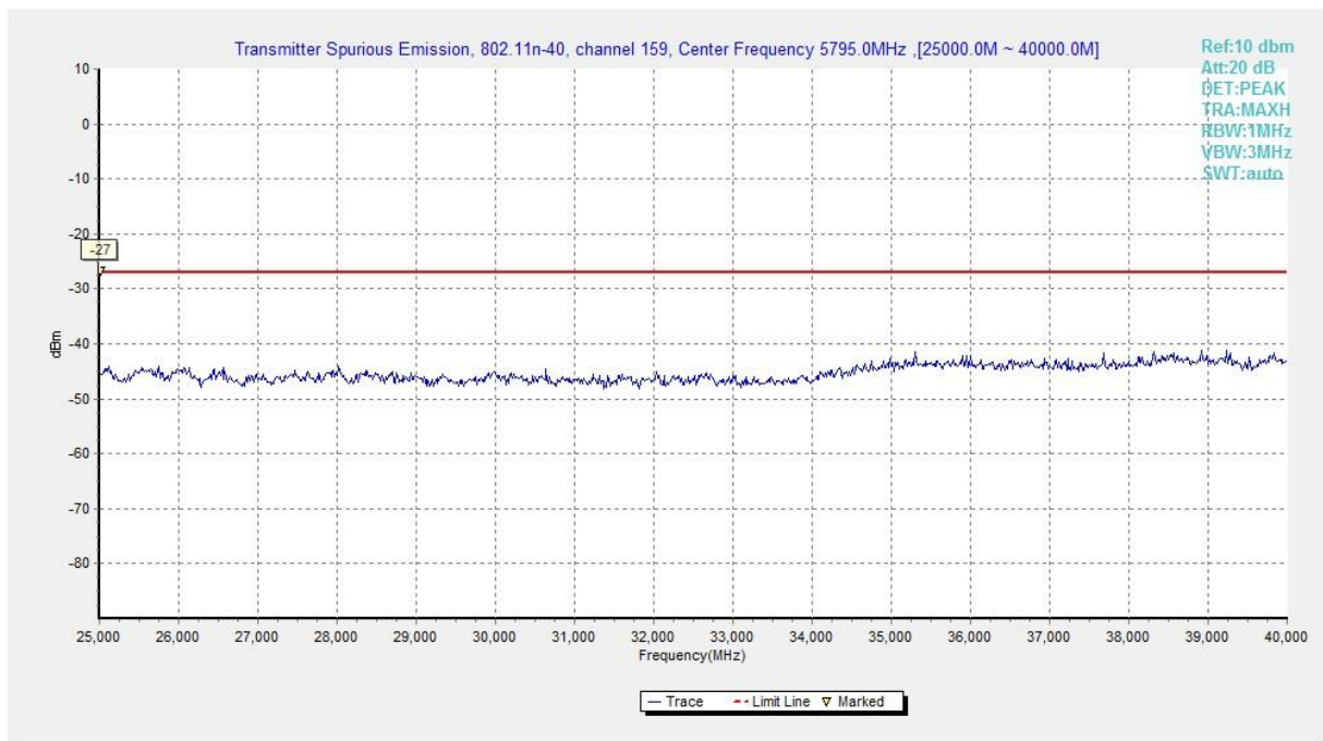
Fig. 46 Conducted Spurious Emission (802.11n-HT40, Ch159, 25 GHz-40 GHz)
