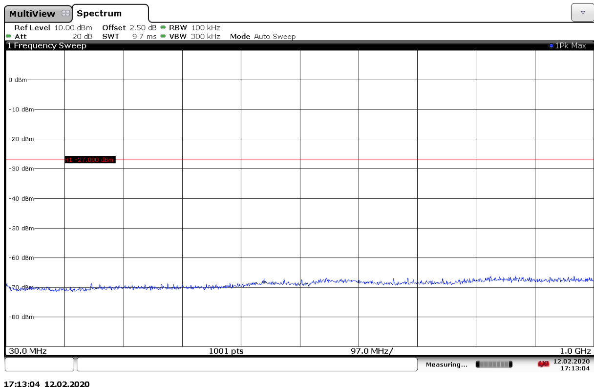
Fig. 59 Conducted Spurious Emission (802.11ax-HE20-RU106-right, Ch149, 30 MHz-1 GHz)
