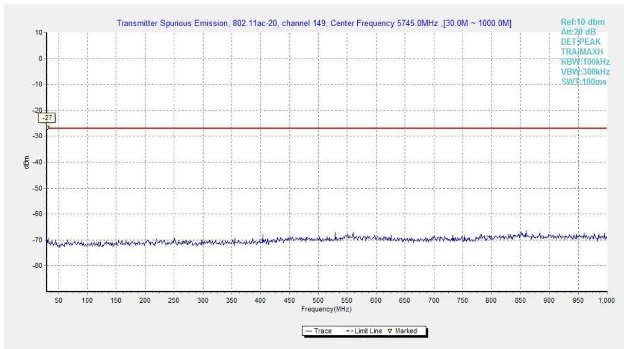
Fig. 27 Conducted Spurious Emission (802.11ac-HT20, Ch149, 30 MHz-1 GHz)
