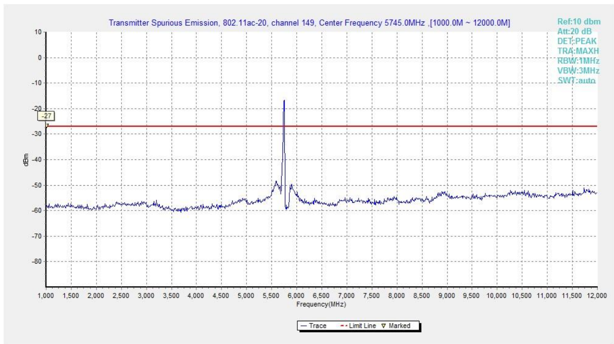
Fig. 28 Conducted Spurious Emission (802.11ac-HT20, Ch149, 1 GHz -12 GHz)
