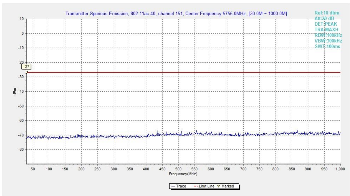
Fig. 47 Conducted Spurious Emission (802.11ac-HT40, Ch151, 30 MHz-1 GHz)
