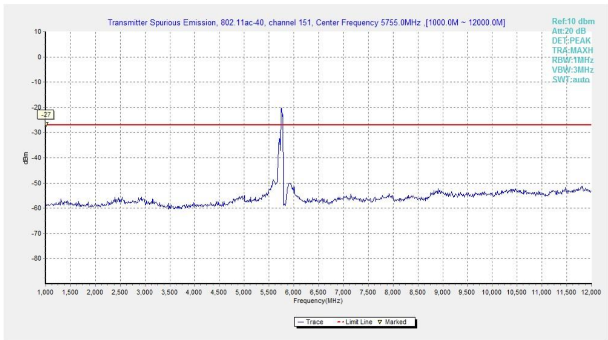
Fig. 48 Conducted Spurious Emission (802.11ac-HT40, Ch151, 1 GHz -12 GHz)
