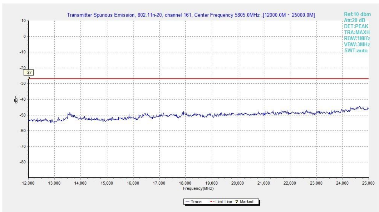
Fig. 25 Conducted Spurious Emission (802.11n-HT20, Ch161, 12 GHz-25 GHz)
