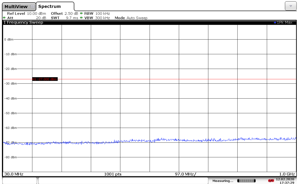
Fig. 63 Conducted Spurious Emission (802.11ax-HE20-RU106-right, Ch161, 30 MHz-1 GHz)
