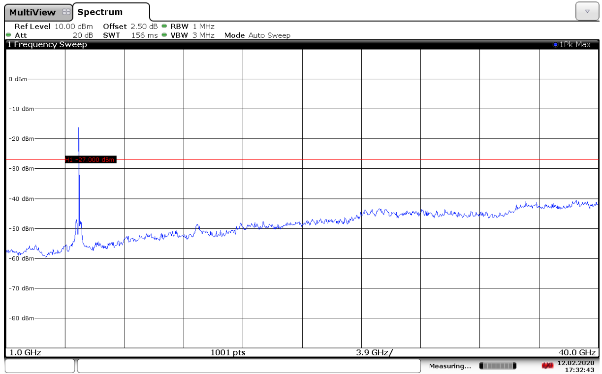
Fig. 62 Conducted Spurious Emission (802.11ax-HE20-RU106-right, Ch157, 1 GHz-40 GHz)
