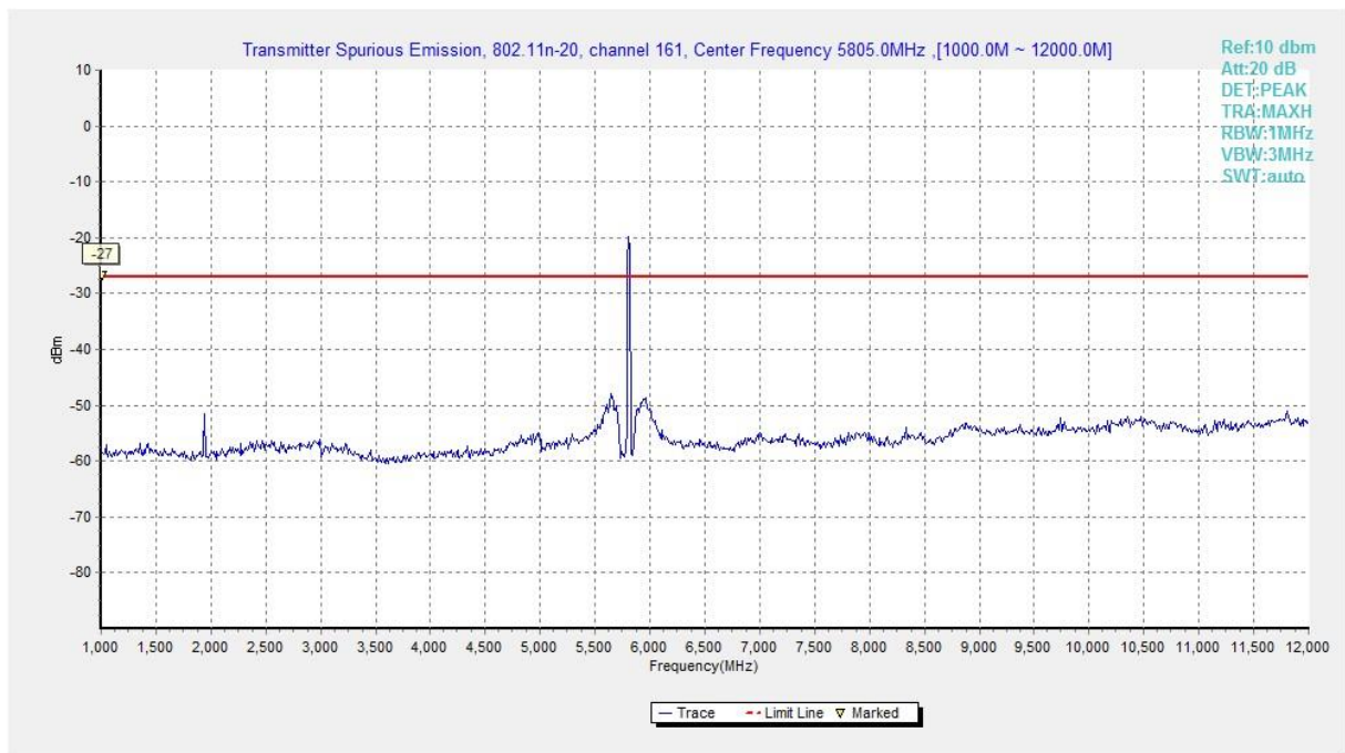
Fig. 24 Conducted Spurious Emission (802.11n-HT20, Ch161, 1 GHz -12 GHz)
