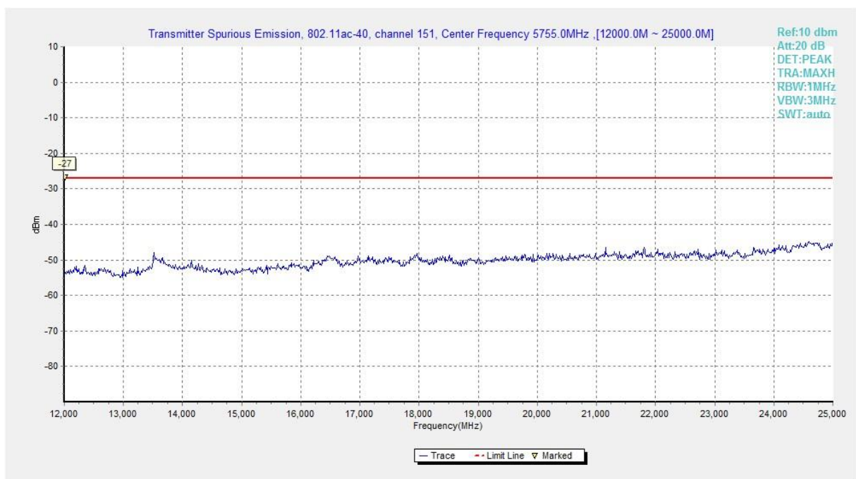
Fig. 49 Conducted Spurious Emission (802.11ac-HT40, Ch151, 12 GHz-25 GHz)
