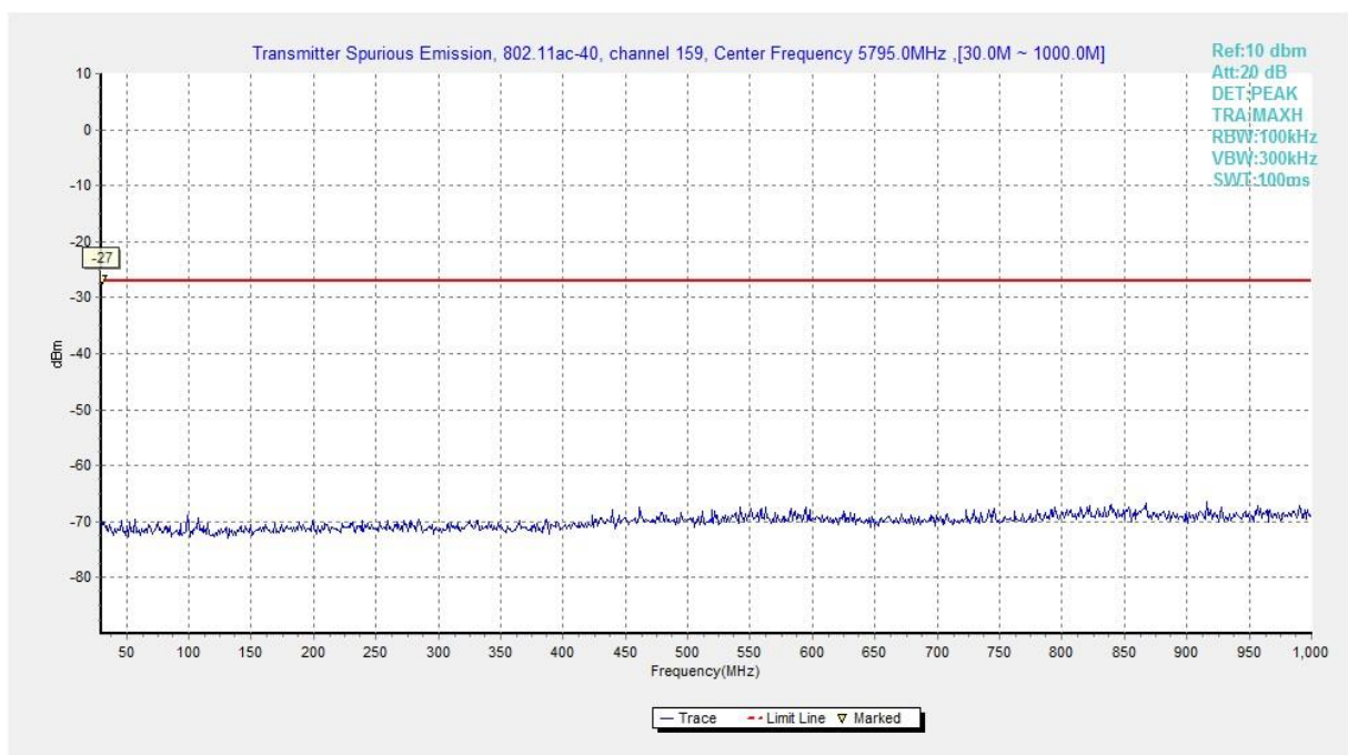
Fig. 51 Conducted Spurious Emission (802.11ac-HT40, Ch159, 30 MHz-1 GHz)
