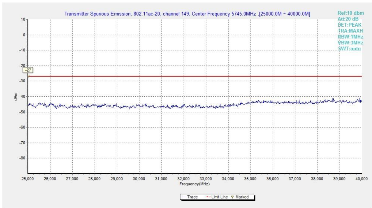
Fig. 30 Conducted Spurious Emission (802.11ac-HT20, Ch149, 25 GHz-40 GHz)
