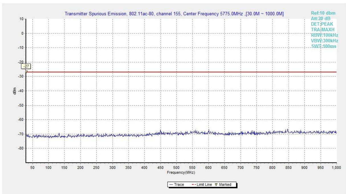
Fig. 55 Conducted Spurious Emission (802.11ac-HT80, Ch155, 30 MHz-1 GHz)
