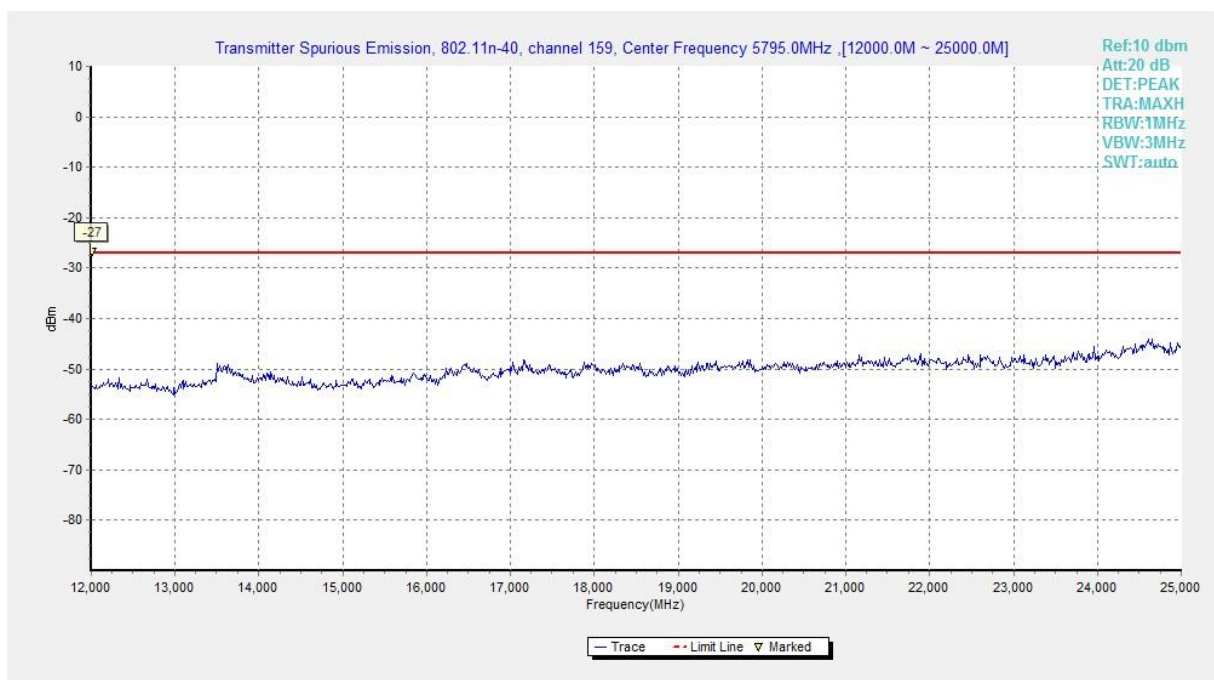
Fig. 45 Conducted Spurious Emission (802.11n-HT40, Ch159, 12 GHz-25 GHz)
