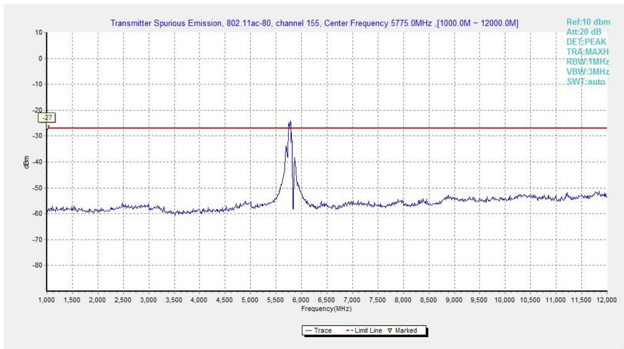
Fig. 56 Conducted Spurious Emission (802.11ac-HT80, Ch155, 1 GHz -12 GHz)
