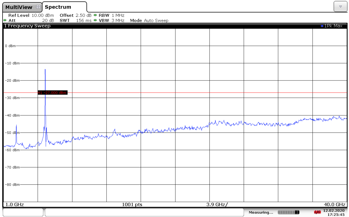
Fig. 60 Conducted Spurious Emission (802.11ax-HE20-RU106-right, Ch149, 1 GHz-40 GHz)
