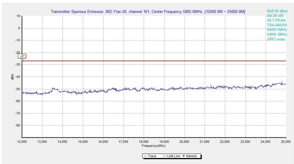
Fig. 37 Conducted Spurious Emission (802.11ac-HT20, Ch161, 12 GHz-25 GHz)
