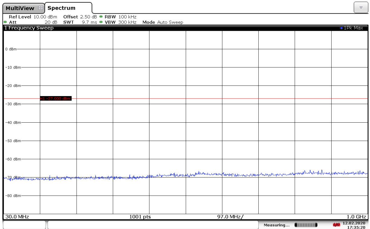
Fig. 61 Conducted Spurious Emission (802.11ax-HE20-RU106-right, Ch157, 30 MHz-1 GHz)
