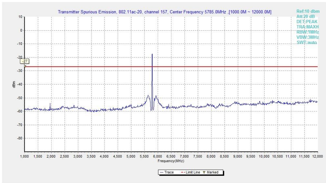
Fig. 32 Conducted Spurious Emission (802.11ac-HT20, Ch157, 1 GHz -12 GHz)
