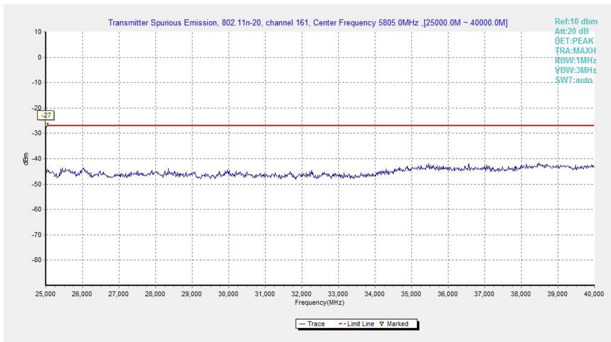
Fig. 26 Conducted Spurious Emission (802.11n-HT20, Ch161, 25 GHz-40 GHz)
