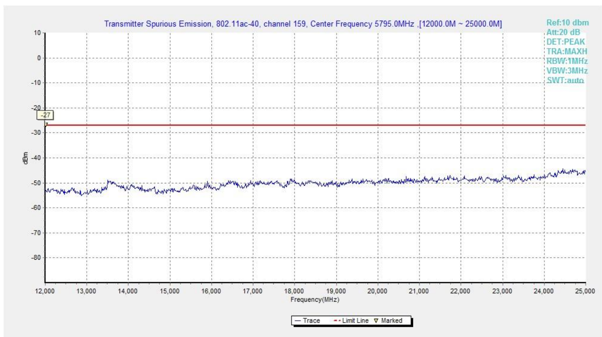
Fig. 53 Conducted Spurious Emission (802.11ac-HT40, Ch159, 12 GHz-25 GHz)
