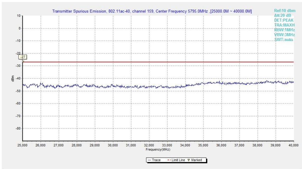
Fig. 54 Conducted Spurious Emission (802.11ac-HT40, Ch159, 25 GHz-40 GHz)
