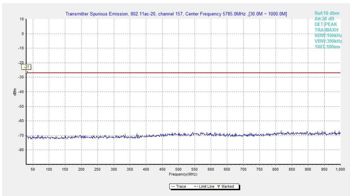
Fig. 31 Conducted Spurious Emission (802.11ac-HT20, Ch157, 30 MHz-1 GHz)
