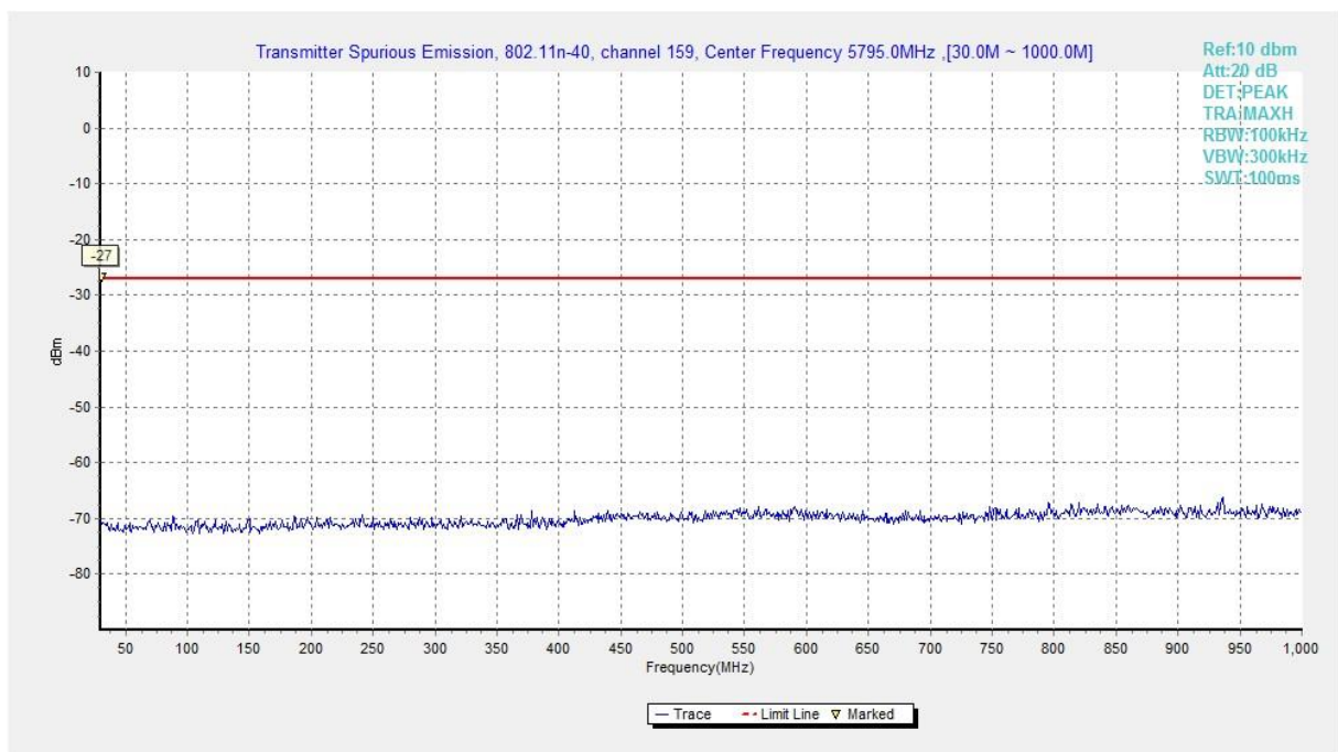
Fig. 43 Conducted Spurious Emission (802.11n-HT40, Ch159, 30 MHz-1 GHz)
