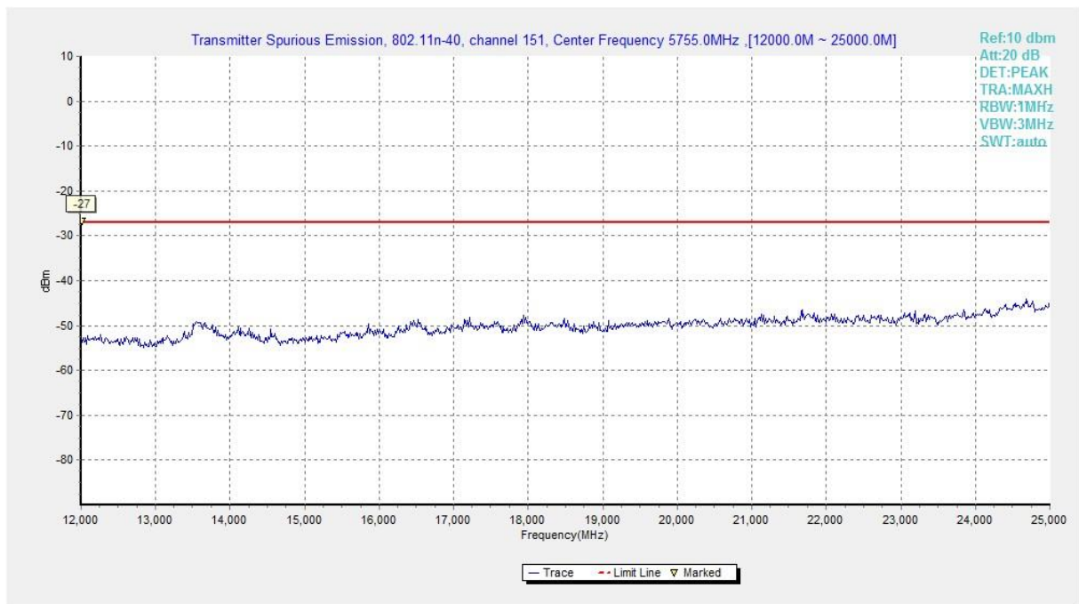
Fig. 41 Conducted Spurious Emission (802.11n-HT40, Ch151, 12 GHz-25 GHz)
