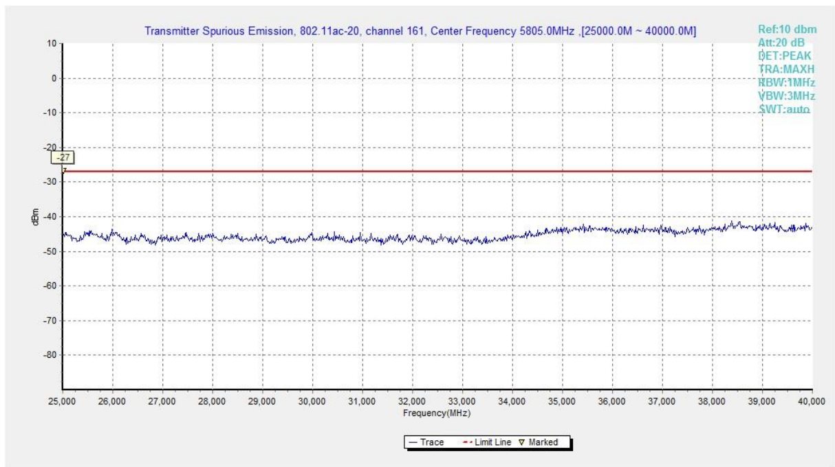
Fig. 38 Conducted Spurious Emission (802.11ac-HT20, Ch161, 25 GHz-40 GHz)
