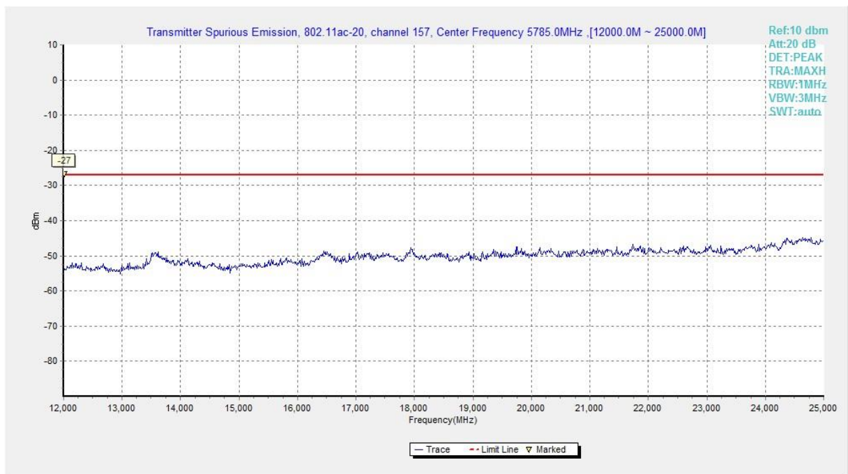
Fig. 33 Conducted Spurious Emission (802.11ac-HT20, Ch157, 12 GHz-25 GHz)
