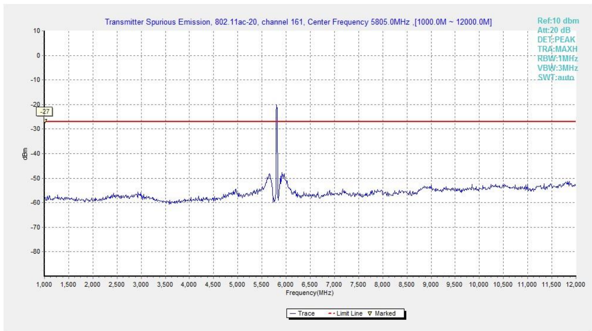
Fig. 36 Conducted Spurious Emission (802.11ac-HT20, Ch161, 1 GHz -12 GHz)
