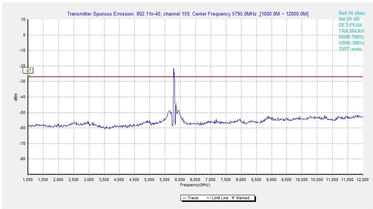
Fig. 44 Conducted Spurious Emission (802.11n-HT40, Ch159, 1 GHz -12 GHz)
