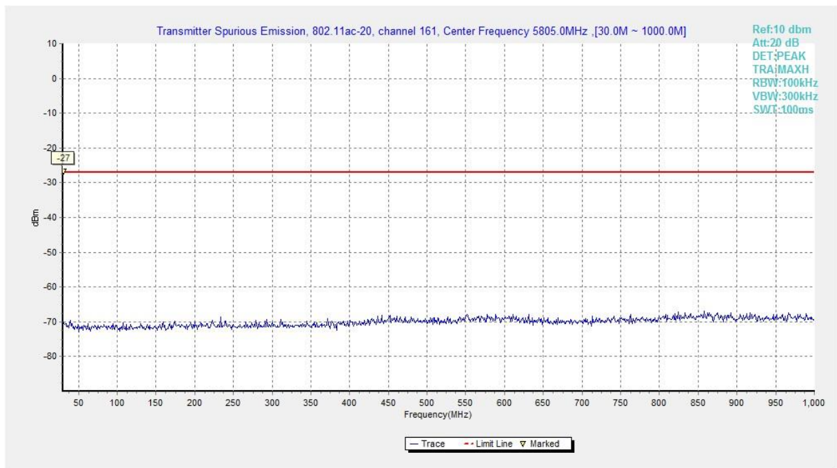
Fig. 35 Conducted Spurious Emission (802.11ac-HT20, Ch161, 30 MHz-1 GHz)
