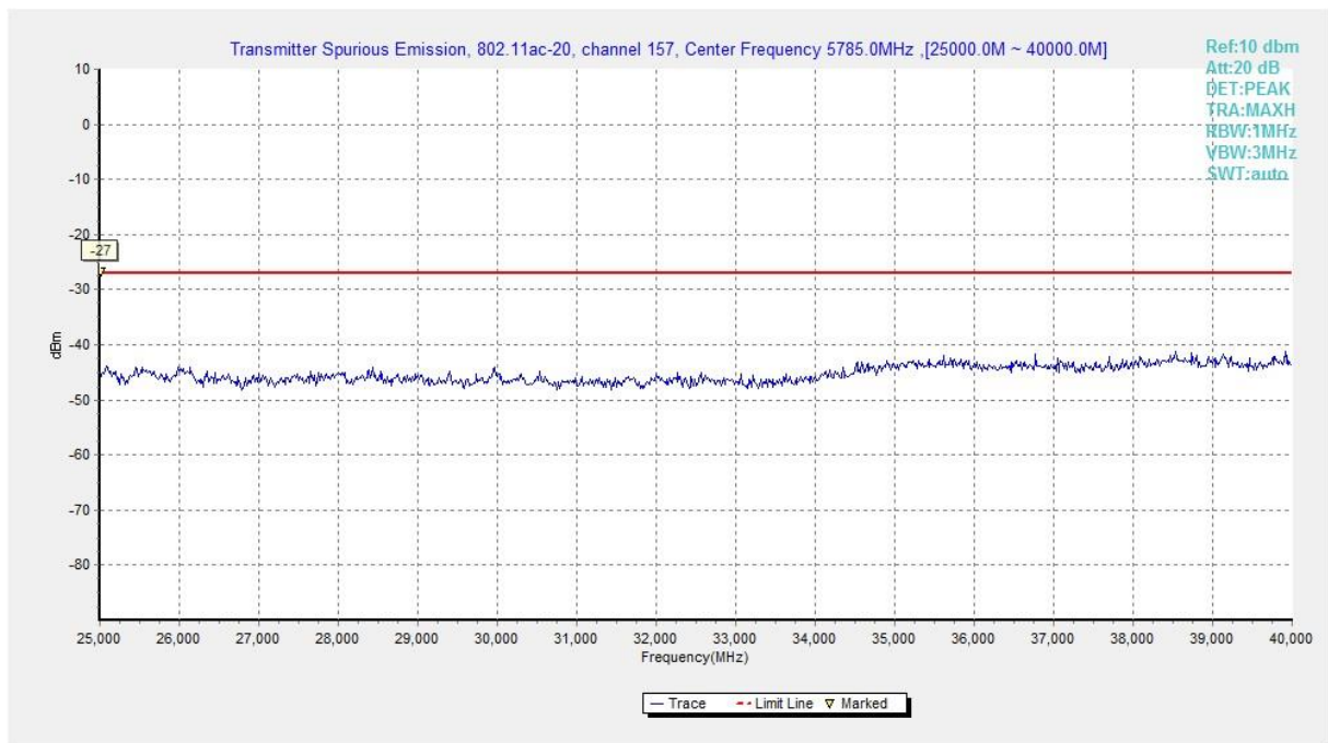
Fig. 34 Conducted Spurious Emission (802.11ac-HT20, Ch157, 25 GHz-40 GHz)
