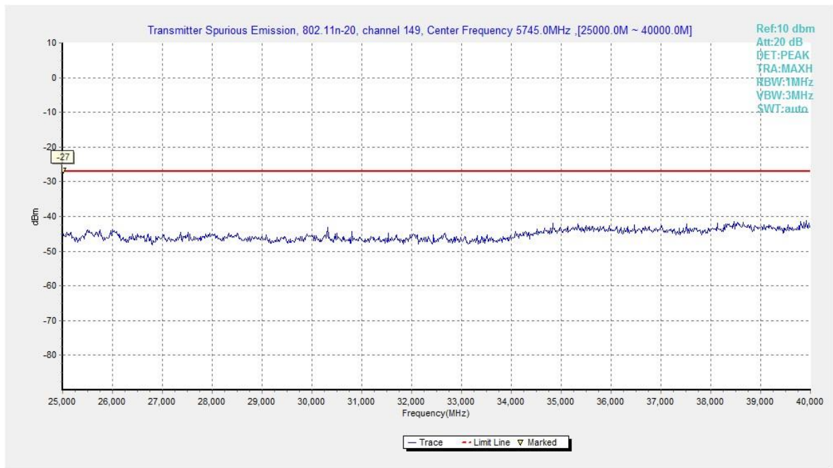
Fig. 86 Conducted Spurious Emission (802.11n-HT20, Ch149, 25 GHz-40 GHz)
