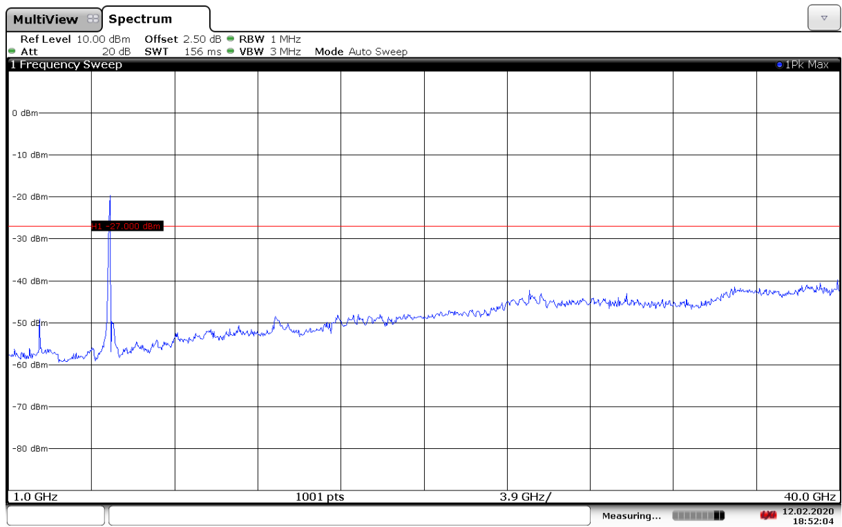
Fig. 134 Conducted Spurious Emission (802.11ax-HE40-RU242-right, Ch151, 1 GHz-40 GHz)
