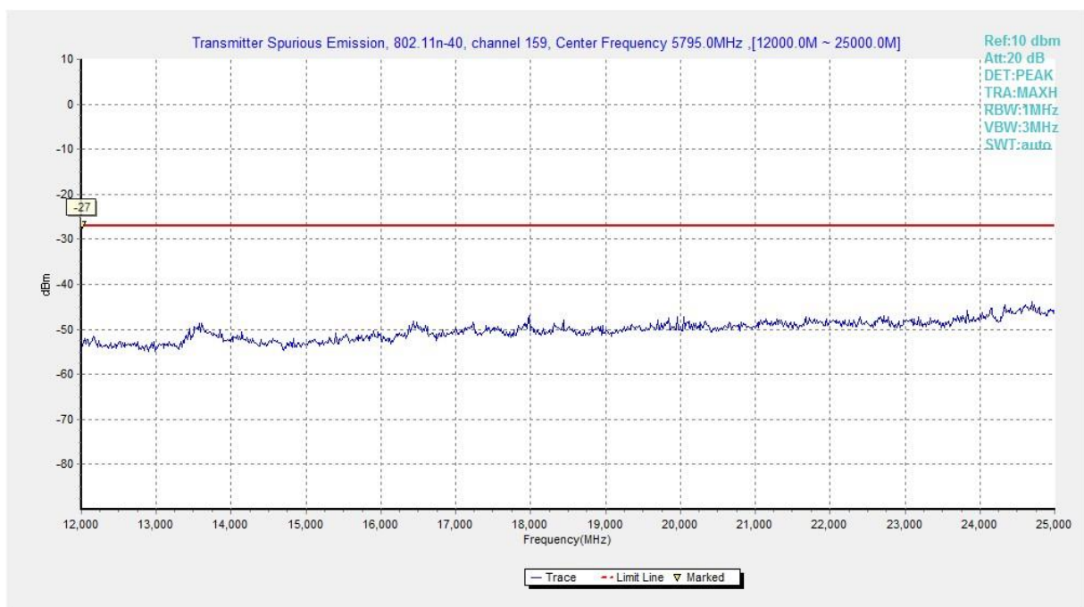
Fig. 113 Conducted Spurious Emission (802.11n-HT40, Ch159, 12 GHz-25 GHz)
