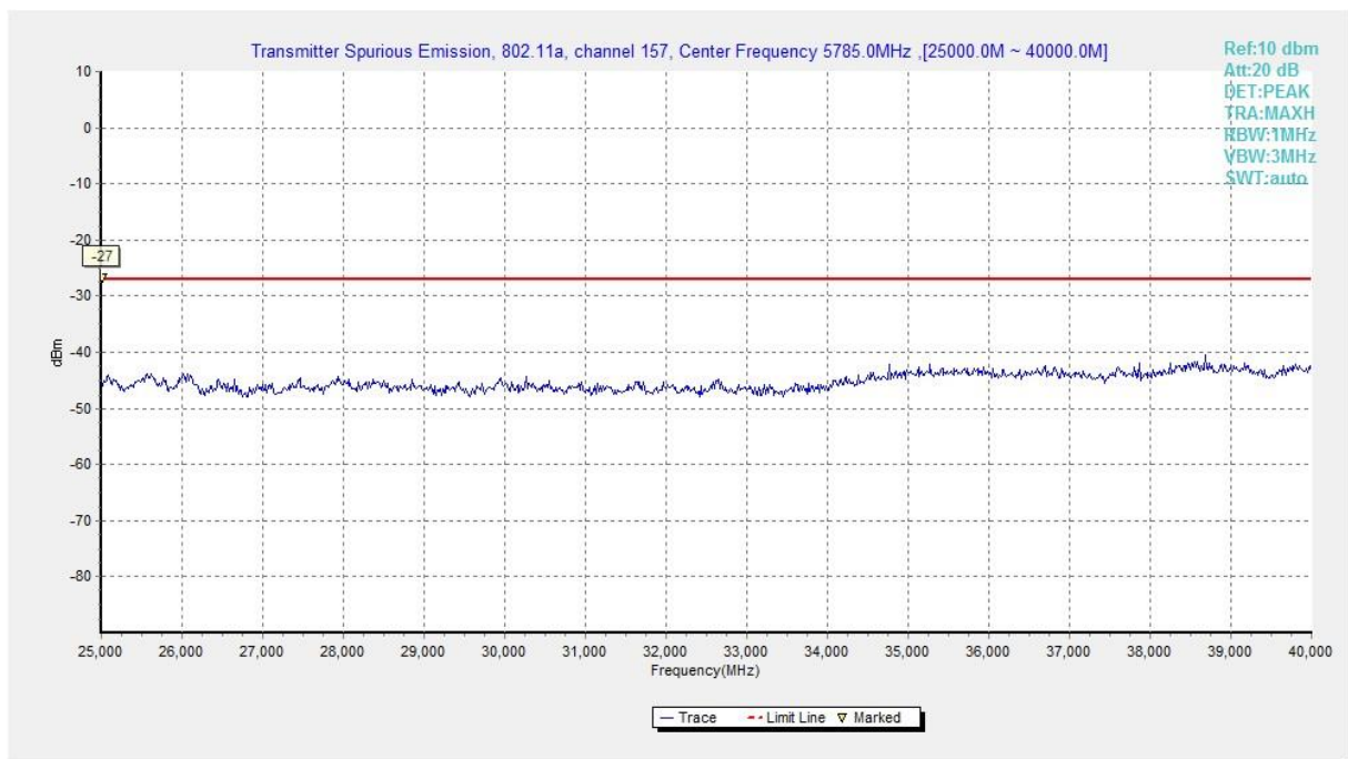
Fig. 78 Conducted Spurious Emission (802.11a, Ch157, 25 GHz-40 GHz)
