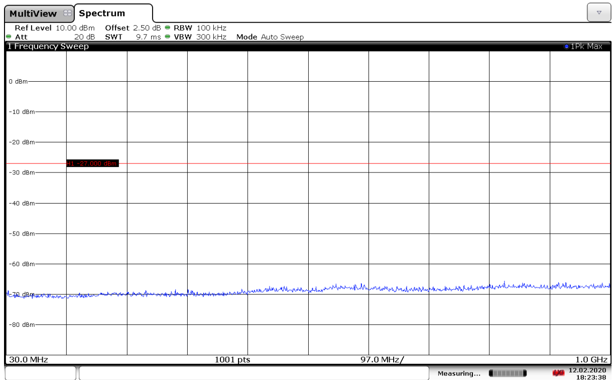
Fig. 137 Conducted Spurious Emission (802.11ax-HE80-RU484-right, Ch155, 30 MHz-1 GHz)
