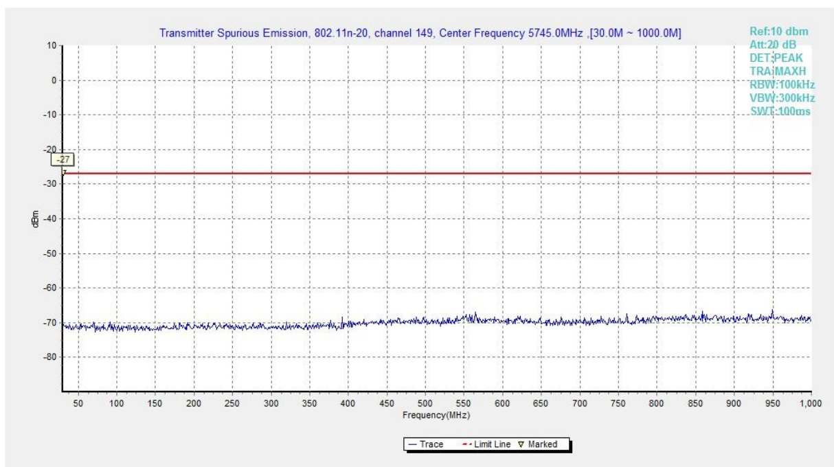
Fig. 83 Conducted Spurious Emission (802.11n-HT20, Ch149, 30 MHz-1 GHz)
