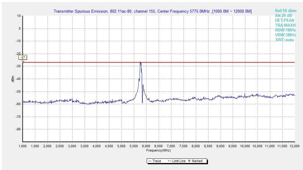
Fig. 124 Conducted Spurious Emission (802.11ac-HT80, Ch155, 1 GHz -12 GHz)
