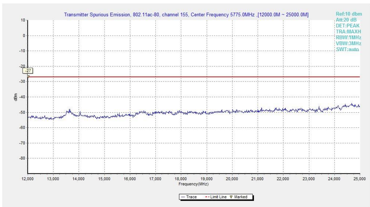
Fig. 125 Conducted Spurious Emission (802.11ac-HT80, Ch155, 12 GHz-25 GHz)
