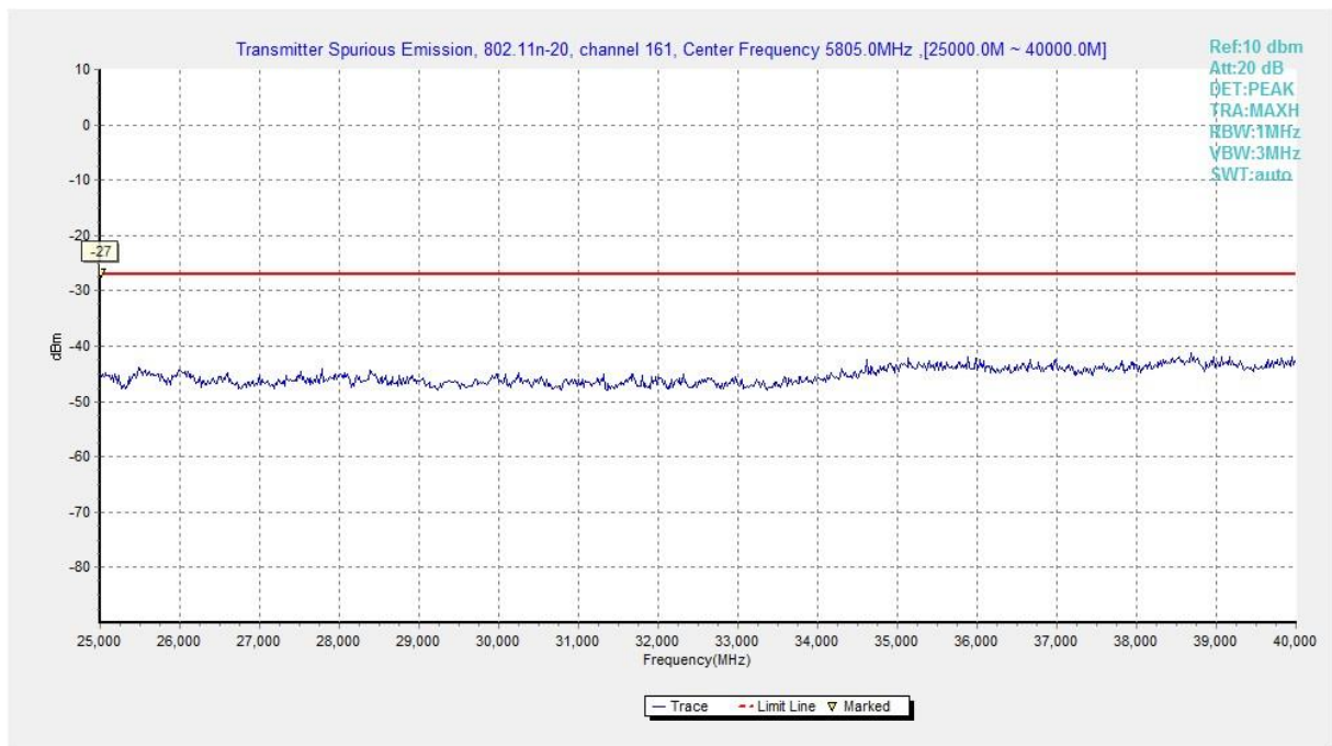
Fig. 94 Conducted Spurious Emission (802.11n-HT20, Ch161, 25 GHz-40 GHz)
