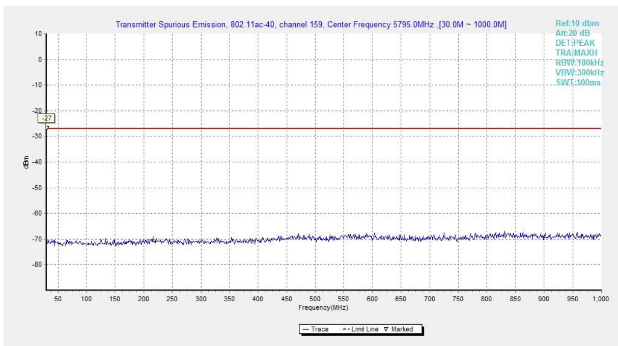
Fig. 119 Conducted Spurious Emission (802.11ac-HT40, Ch159, 30 MHz-1 GHz)
