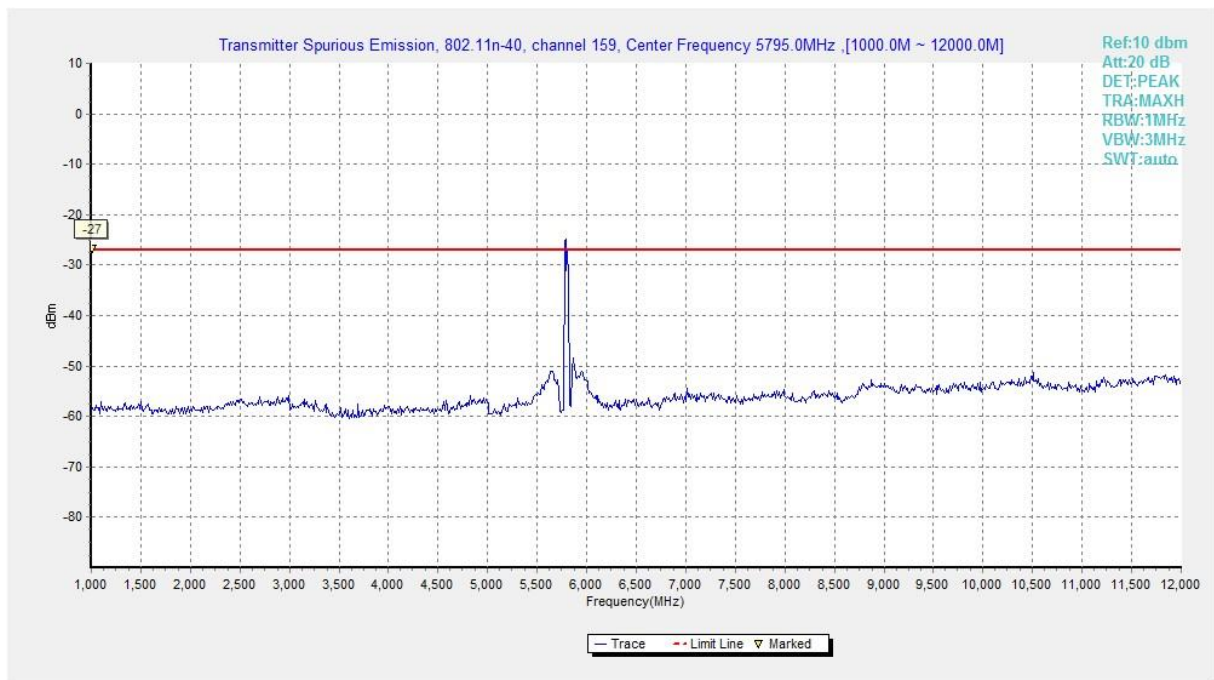
Fig. 112 Conducted Spurious Emission (802.11n-HT40, Ch159, 1 GHz -12 GHz)
