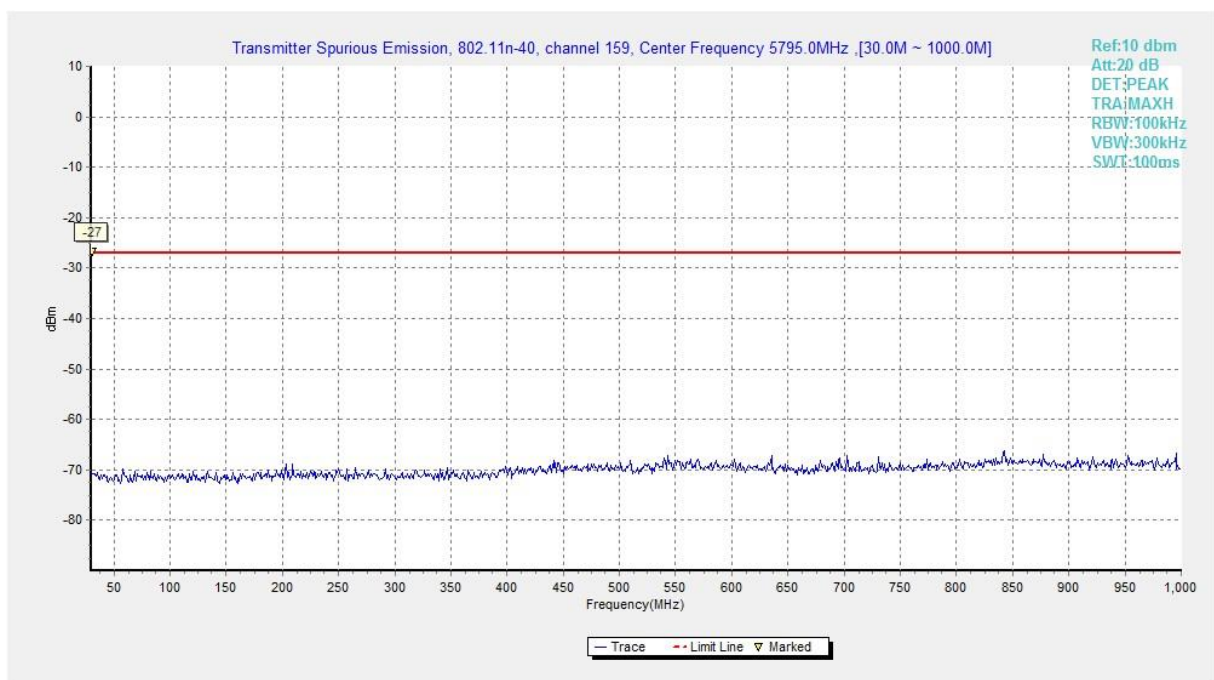
Fig. 111 Conducted Spurious Emission (802.11n-HT40, Ch159, 30 MHz-1 GHz)
