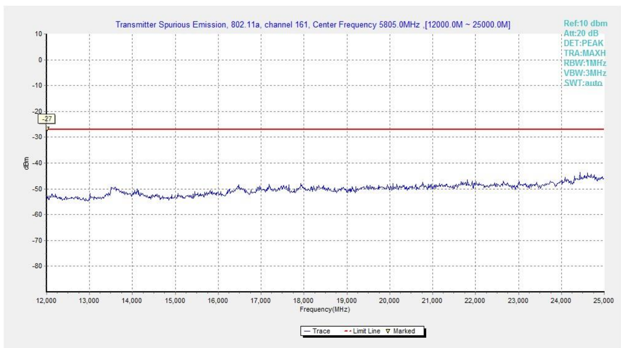
Fig. 81 Conducted Spurious Emission (802.11a, Ch161, 12 GHz-25 GHz)
