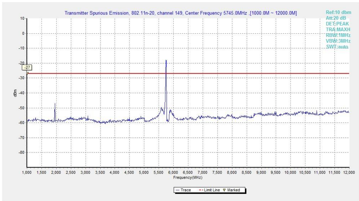
Fig. 84 Conducted Spurious Emission (802.11n-HT20, Ch149, 1 GHz -12 GHz)
