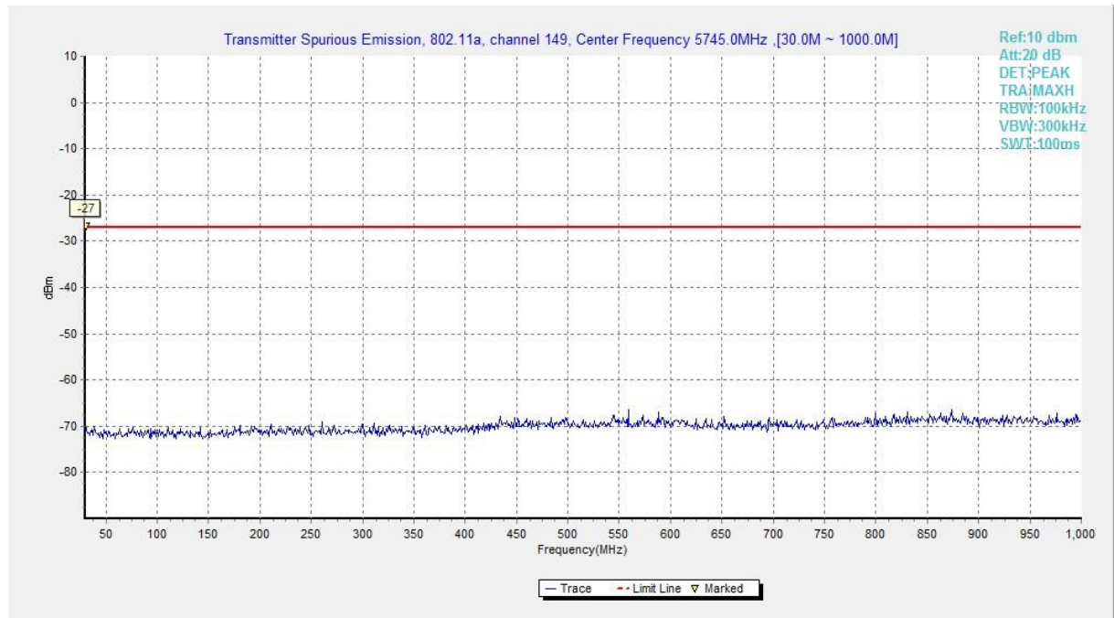
Fig. 71 Conducted Spurious Emission (802.11a, Ch149, 30 MHz-1 GHz)
