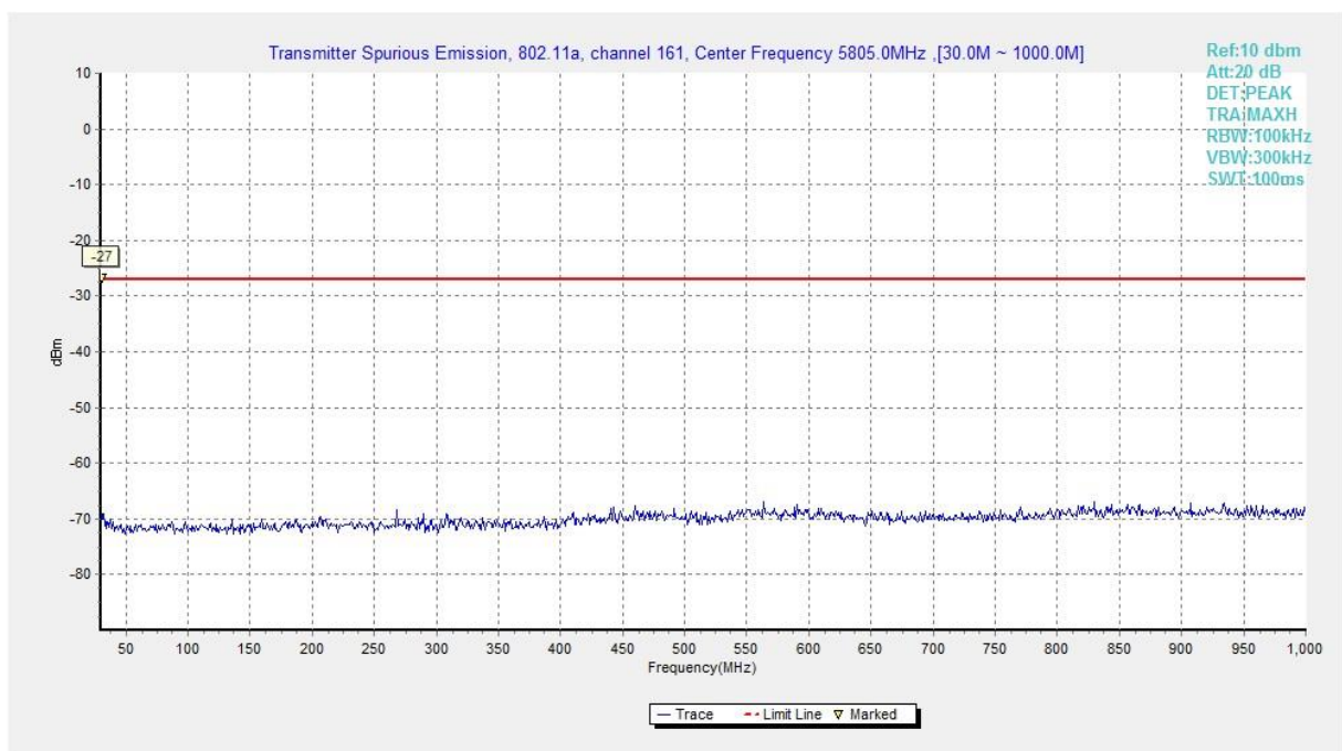
Fig. 79 Conducted Spurious Emission (802.11a, Ch161, 30 MHz-1 GHz)
