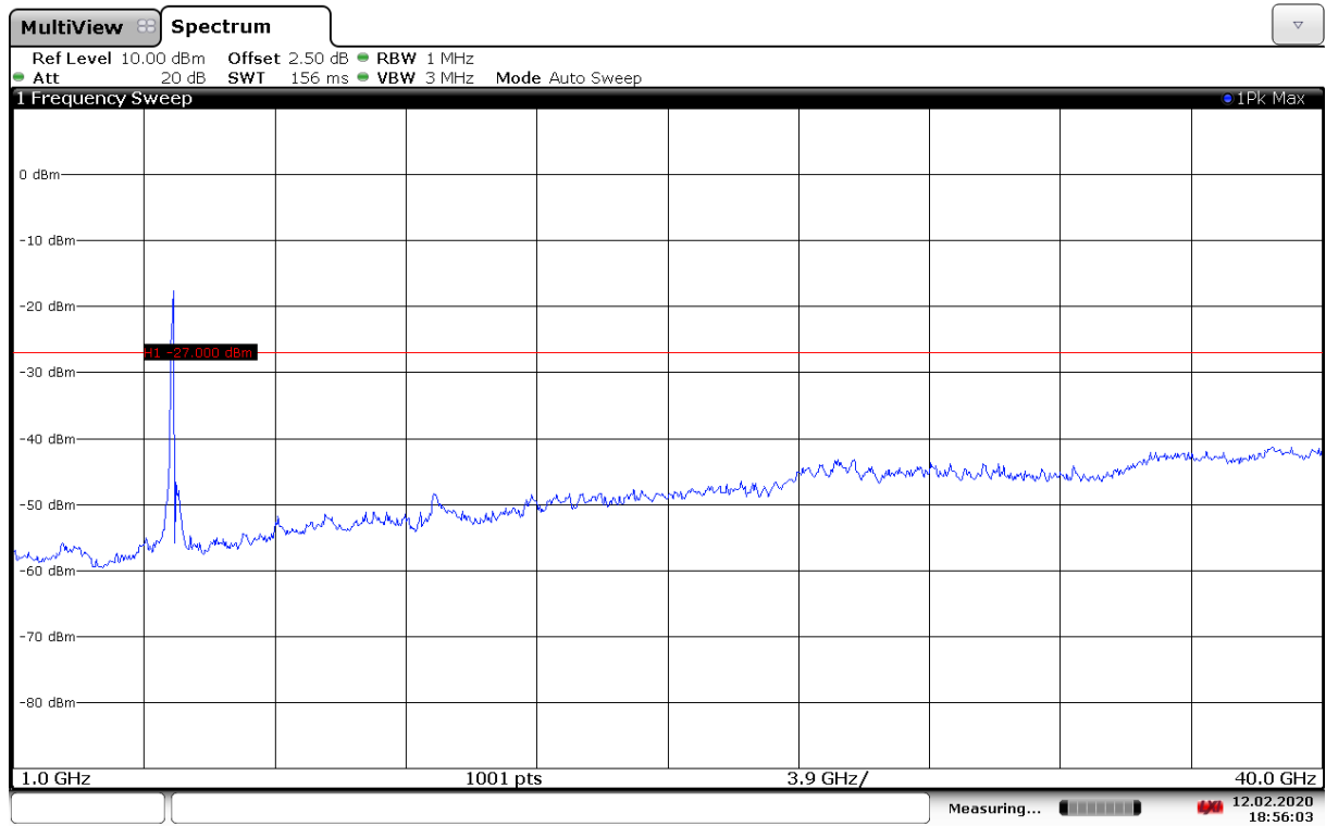
Fig. 66 Conducted Spurious Emission (802.11ax-HE40-RU242-right, Ch151, 1 GHz-40 GHz)
