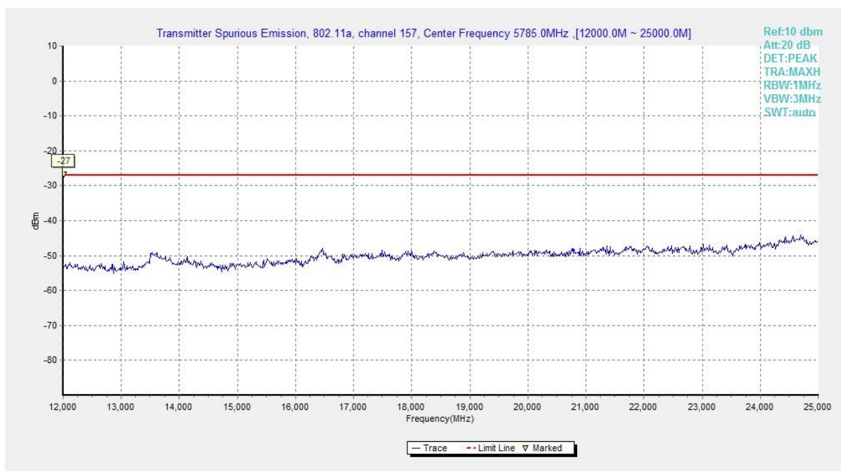
Fig. 77 Conducted Spurious Emission (802.11a, Ch157, 12 GHz-25 GHz)
