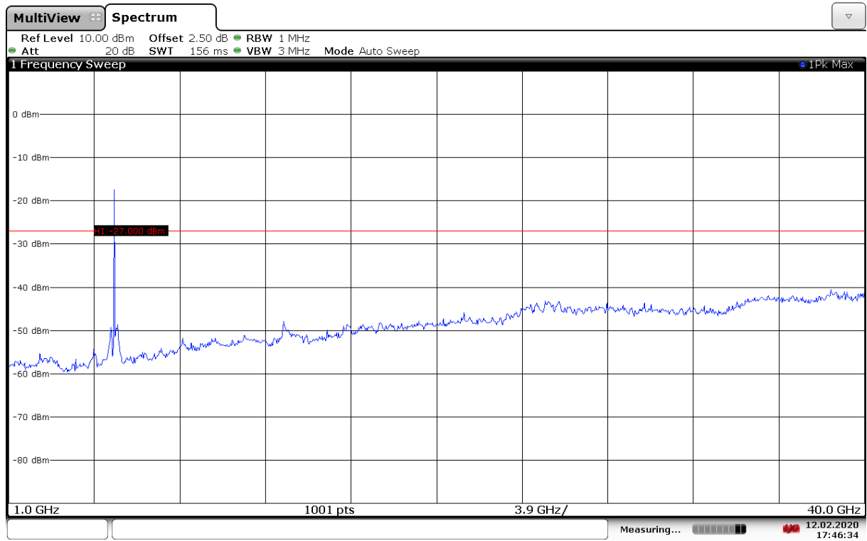
Fig. 132 Conducted Spurious Emission (802.11ax-HE20-RU106-right, Ch161, 1 GHz-40 GHz)
