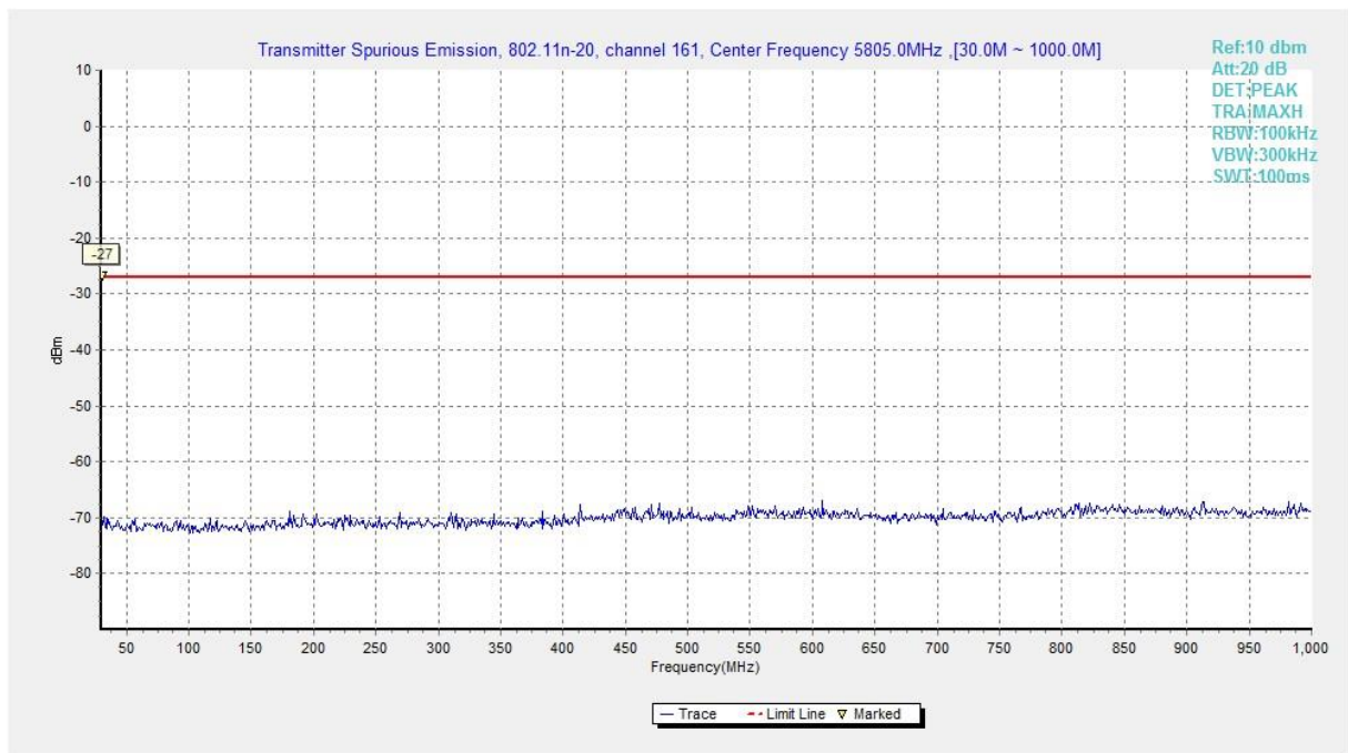
Fig. 91 Conducted Spurious Emission (802.11n-HT20, Ch161, 30 MHz-1 GHz)
