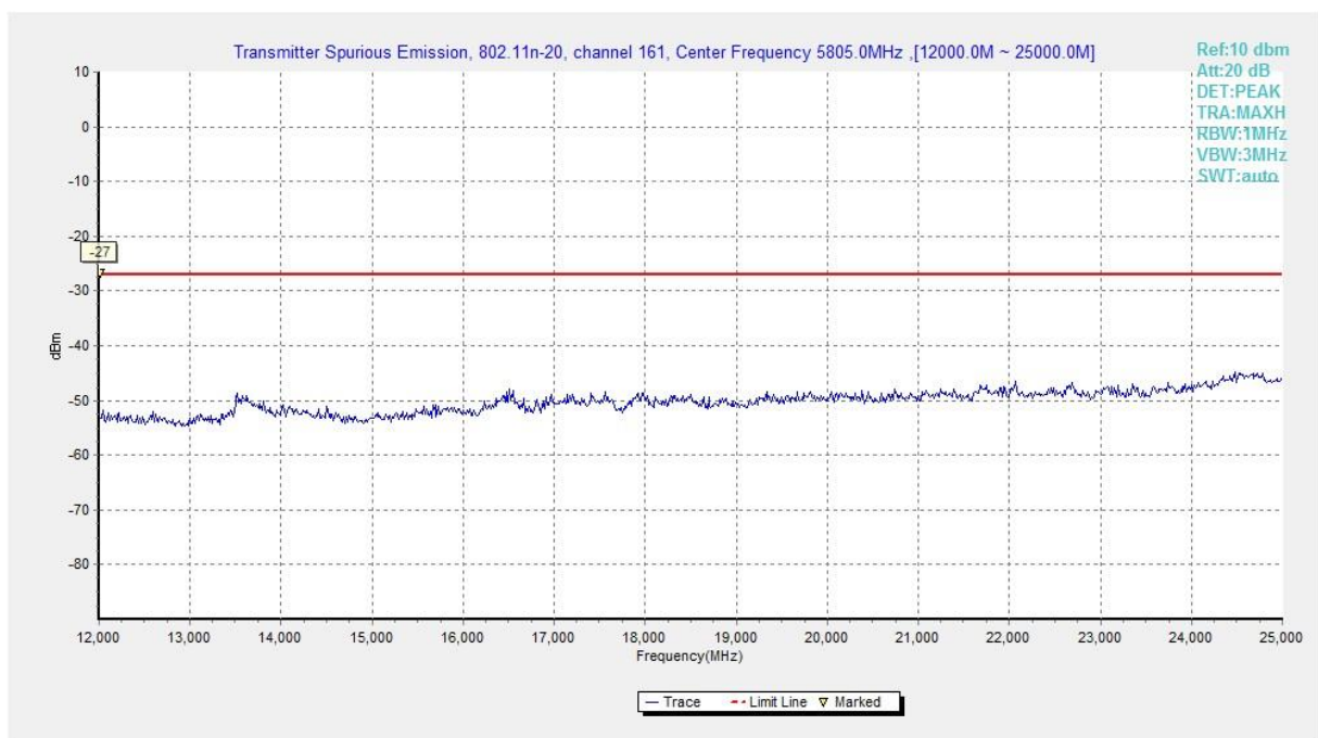
Fig. 93 Conducted Spurious Emission (802.11n-HT20, Ch161, 12 GHz-25 GHz)
