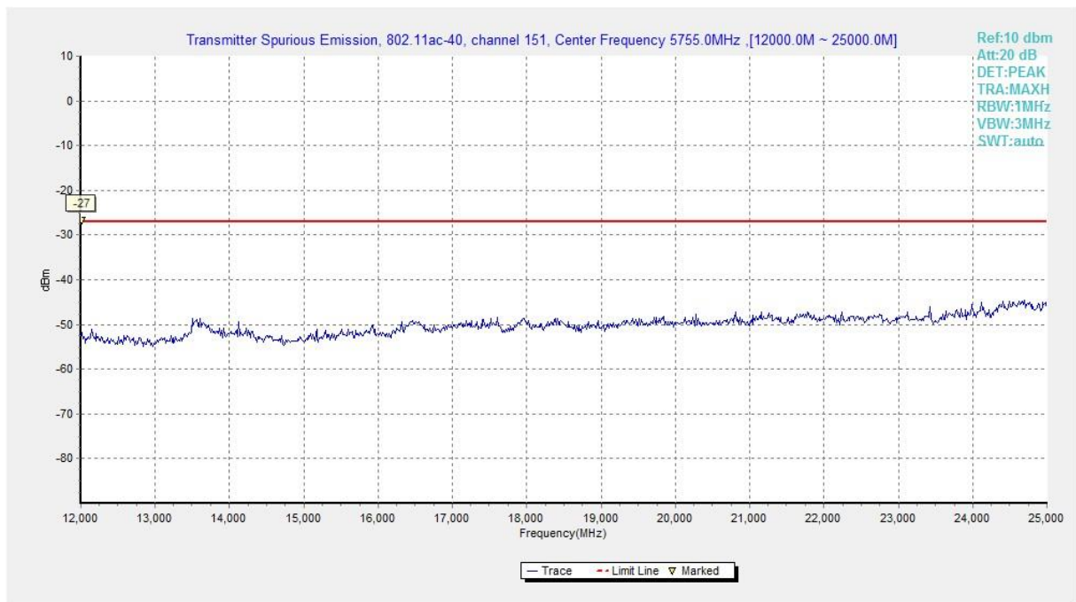
Fig. 117 Conducted Spurious Emission (802.11ac-HT40, Ch151, 12 GHz-25 GHz)
