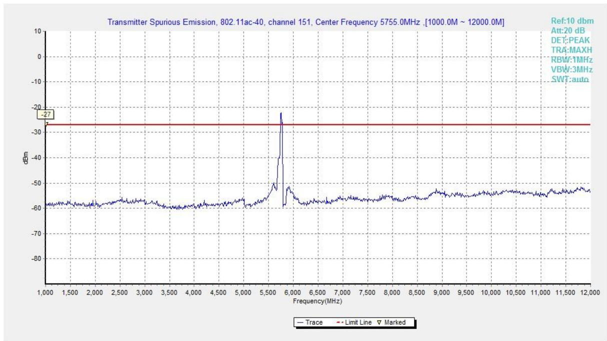
Fig. 116 Conducted Spurious Emission (802.11ac-HT40, Ch151, 1 GHz -12 GHz)
