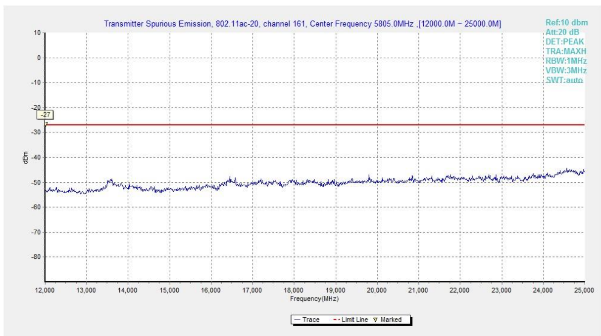
Fig. 105 Conducted Spurious Emission (802.11ac-HT20, Ch161, 12 GHz-25 GHz)
