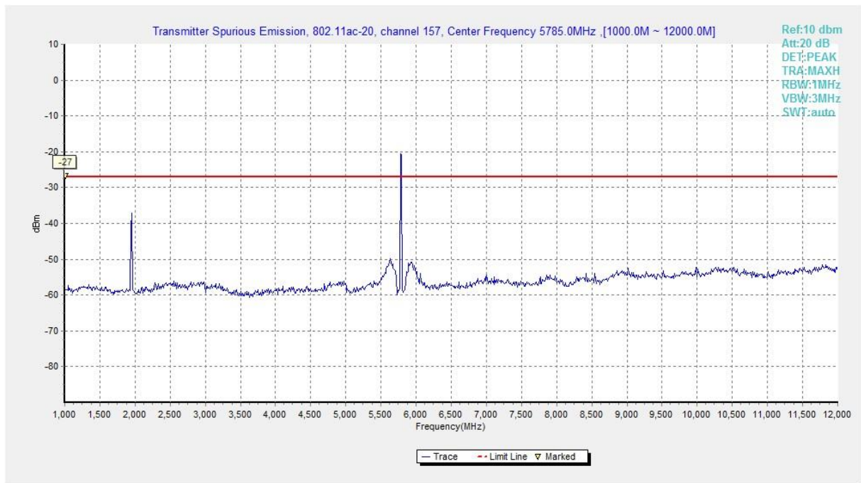
Fig. 100 Conducted Spurious Emission (802.11ac-HT20, Ch157, 1 GHz -12 GHz)
