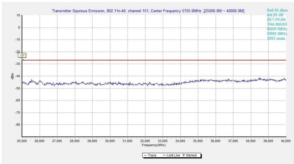
Fig. 110 Conducted Spurious Emission (802.11n-HT40, Ch151, 25 GHz-40 GHz)
