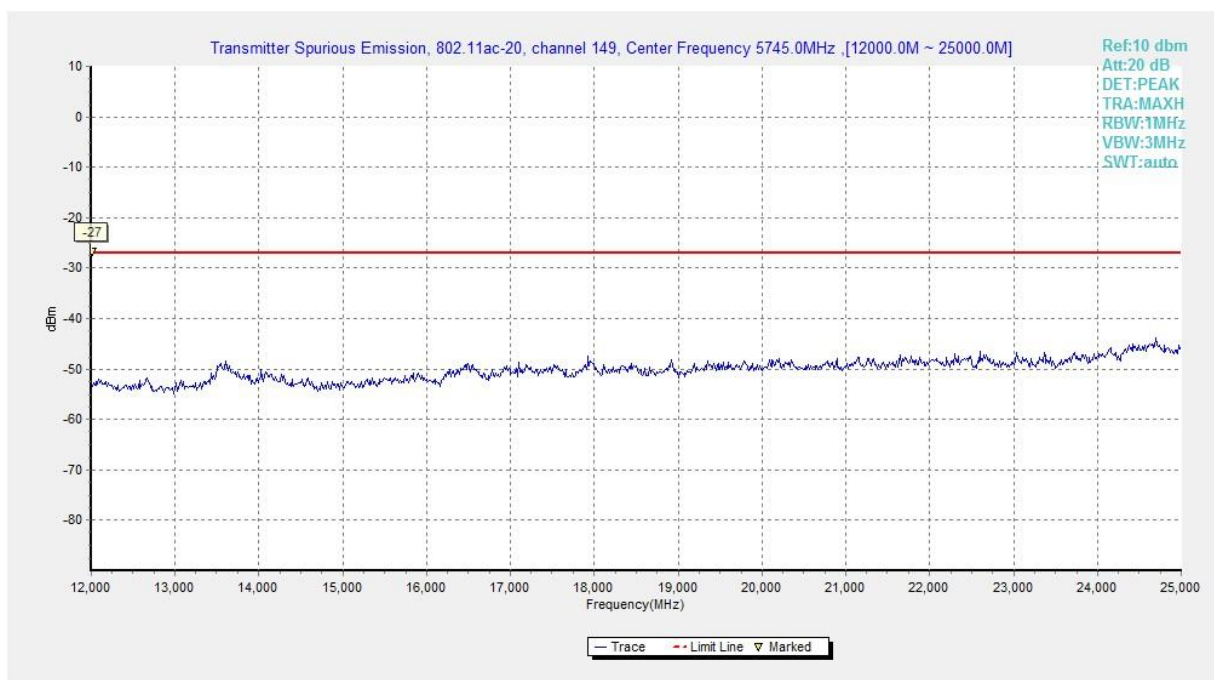
Fig. 97 Conducted Spurious Emission (802.11ac-HT20, Ch149, 12 GHz-25 GHz)
