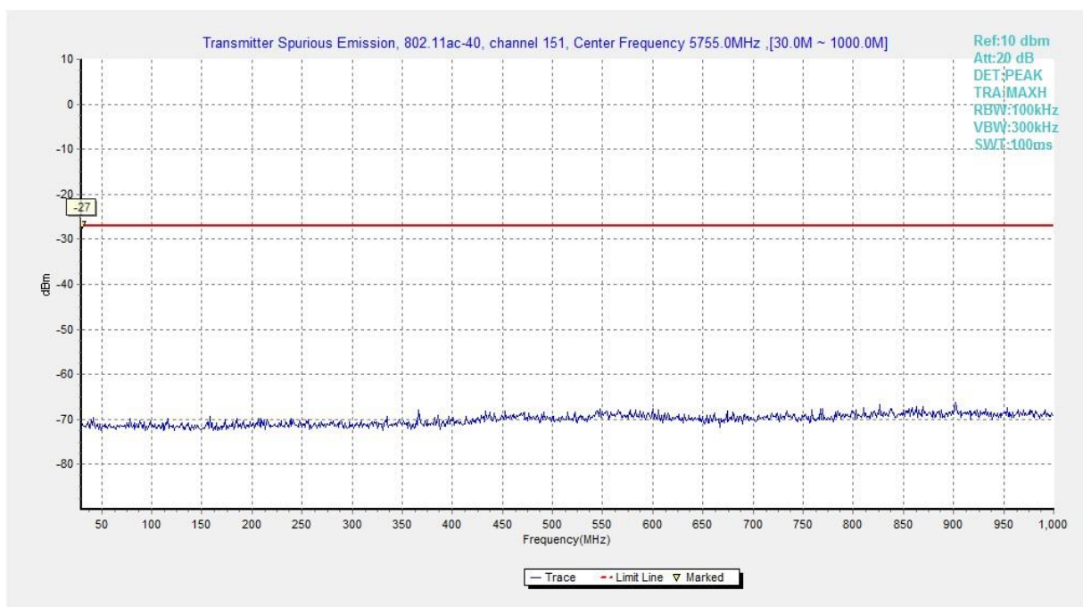
Fig. 115 Conducted Spurious Emission (802.11ac-HT40, Ch151, 30 MHz-1 GHz)
