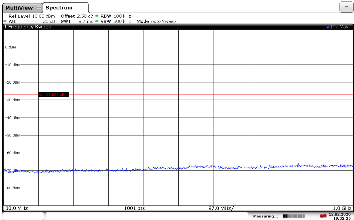
Fig. 67 Conducted Spurious Emission (802.11ax-HE40-RU242-right, Ch159, 30 MHz-1 GHz)
