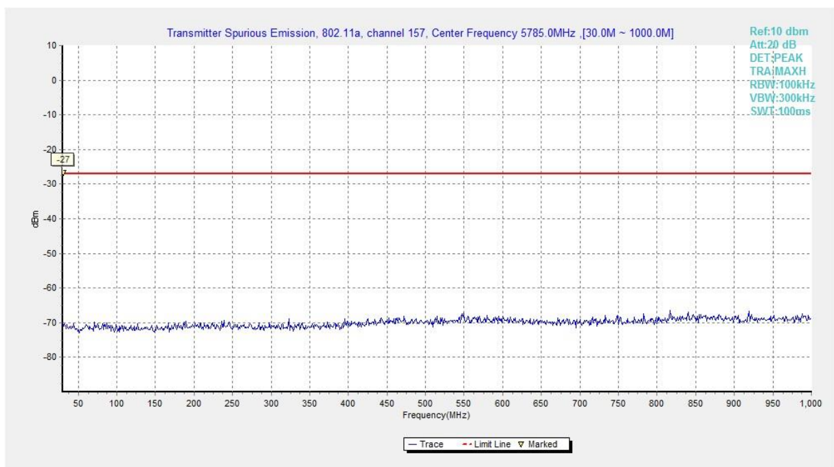
Fig. 75 Conducted Spurious Emission (802.11a, Ch157, 30 MHz-1 GHz)
