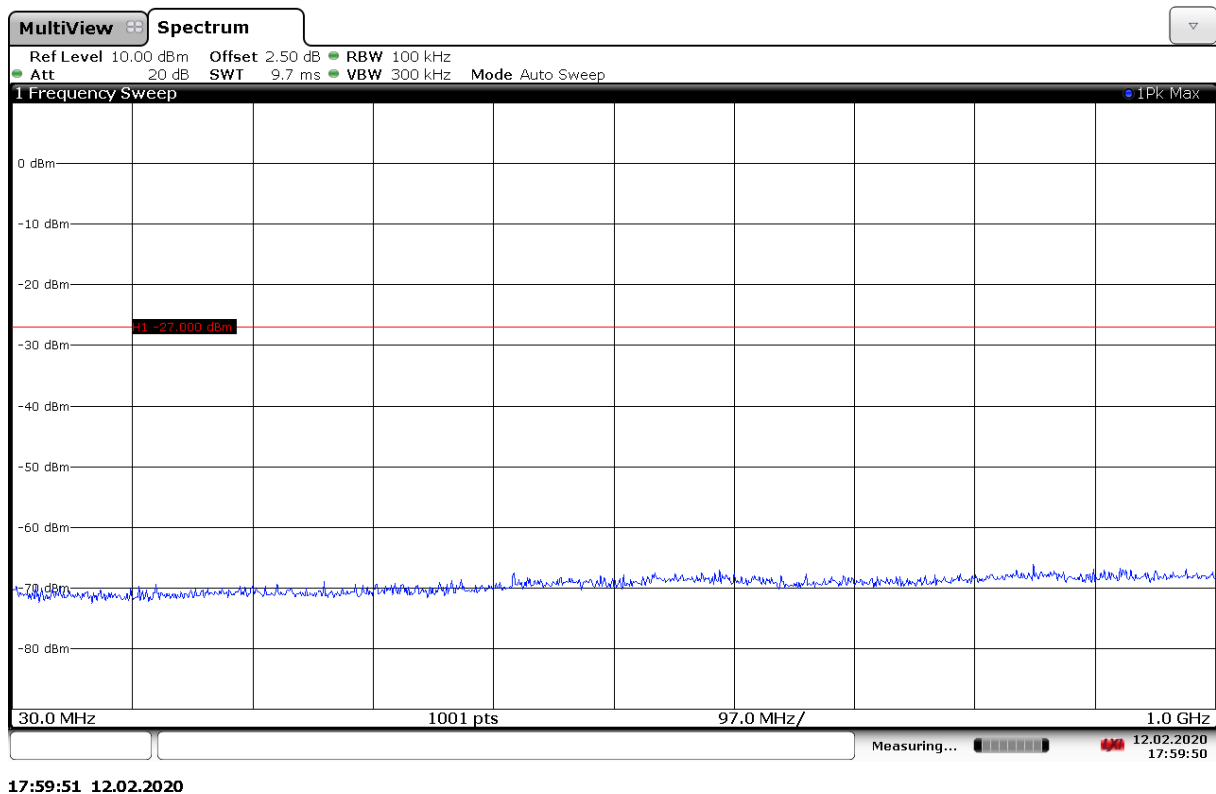
Fig. 127 Conducted Spurious Emission (802.11ax-HE20-RU106-right, Ch149, 30 MHz-1 GHz)
