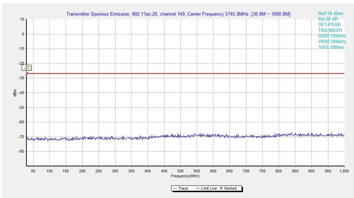
Fig. 95 Conducted Spurious Emission (802.11ac-HT20, Ch149, 30 MHz-1 GHz)
