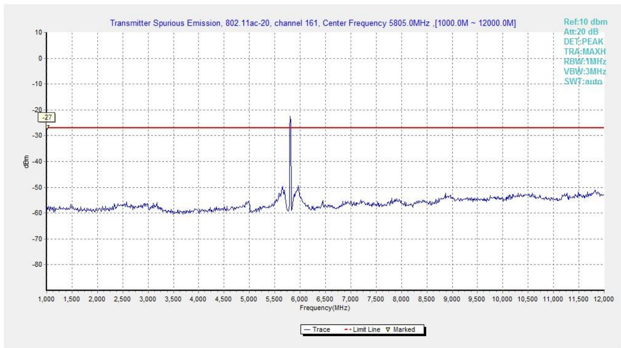
Fig. 104 Conducted Spurious Emission (802.11ac-HT20, Ch161, 1 GHz -12 GHz)
