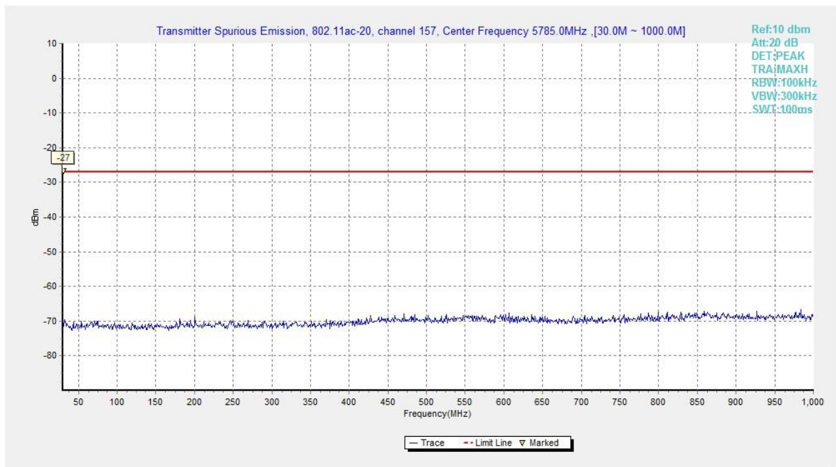
Fig. 99 Conducted Spurious Emission (802.11ac-HT20, Ch157, 30 MHz-1 GHz)
