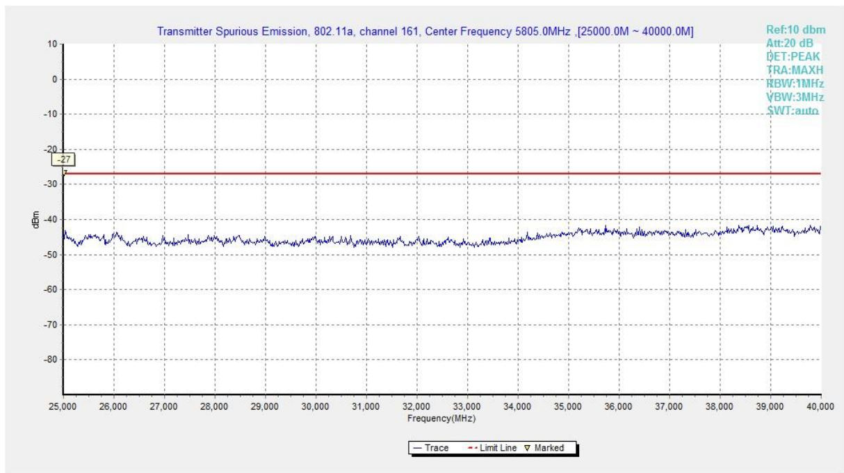
Fig. 82 Conducted Spurious Emission (802.11a, Ch161, 25 GHz-40 GHz)
