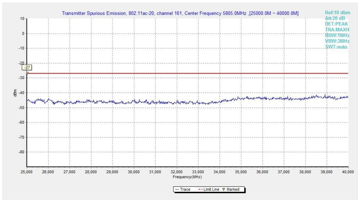
Fig. 106 Conducted Spurious Emission (802.11ac-HT20, Ch161, 25 GHz-40 GHz)
