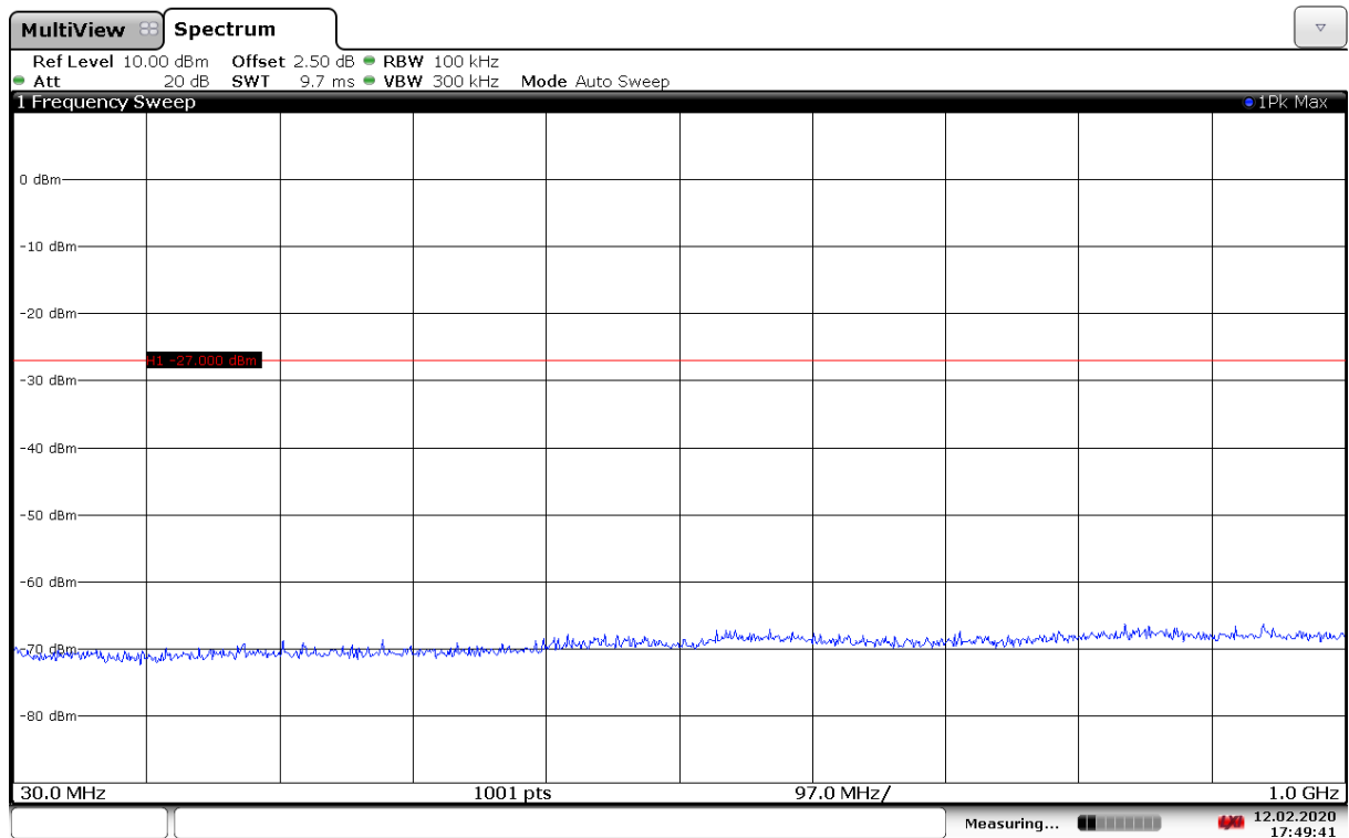
Fig. 129 Conducted Spurious Emission (802.11ax-HE20-RU106-right, Ch157, 30 MHz-1 GHz)
