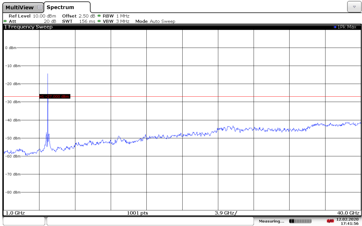
Fig. 64 Conducted Spurious Emission (802.11ax-HE20-RU106-right, Ch161, 1 GHz-40 GHz)
