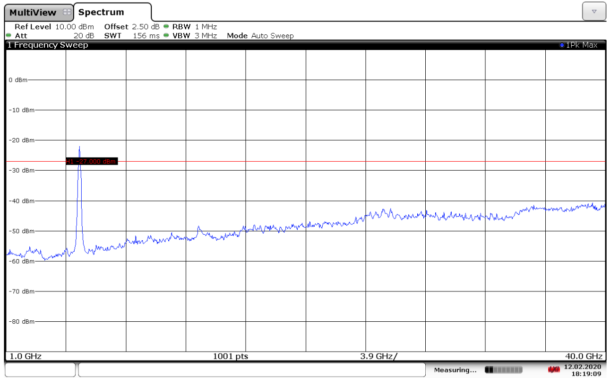
Fig. 138 Conducted Spurious Emission (802.11ax-HE80-RU484-right, Ch155, 1 GHz-40 GHz)
