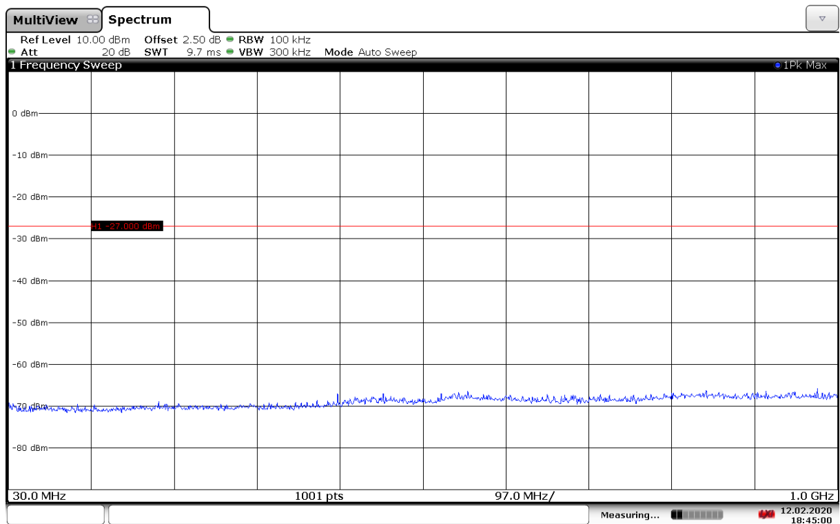
Fig. 135 Conducted Spurious Emission (802.11ax-HE40-RU242-right, Ch159, 30 MHz-1 GHz)
