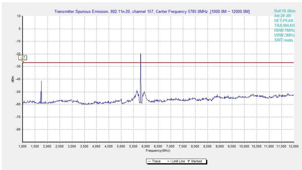
Fig. 88 Conducted Spurious Emission (802.11n-HT20, Ch157, 1 GHz -12 GHz)
