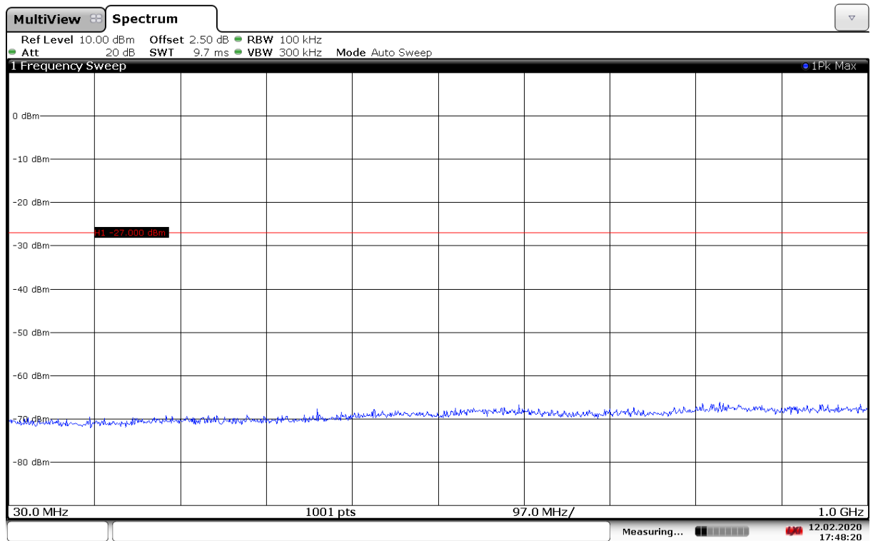
Fig. 131 Conducted Spurious Emission (802.11ax-HE20-RU106-right, Ch161, 30 MHz-1 GHz)
