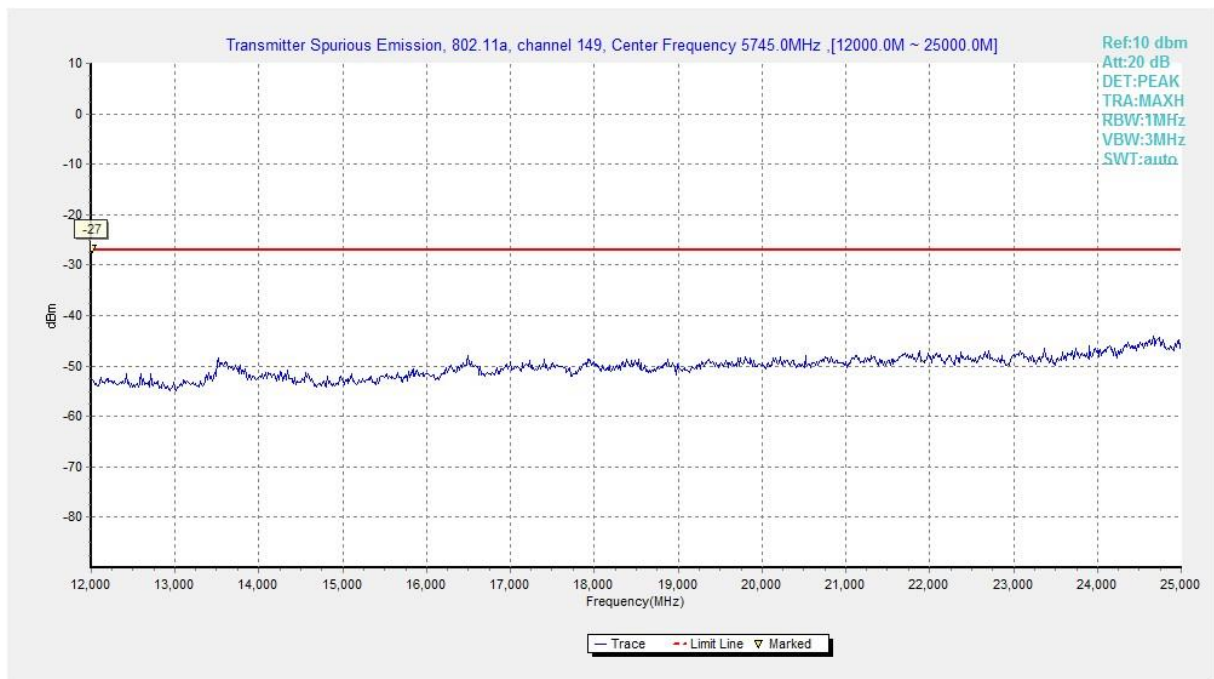
Fig. 73 Conducted Spurious Emission (802.11a, Ch149, 12 GHz-25 GHz)
