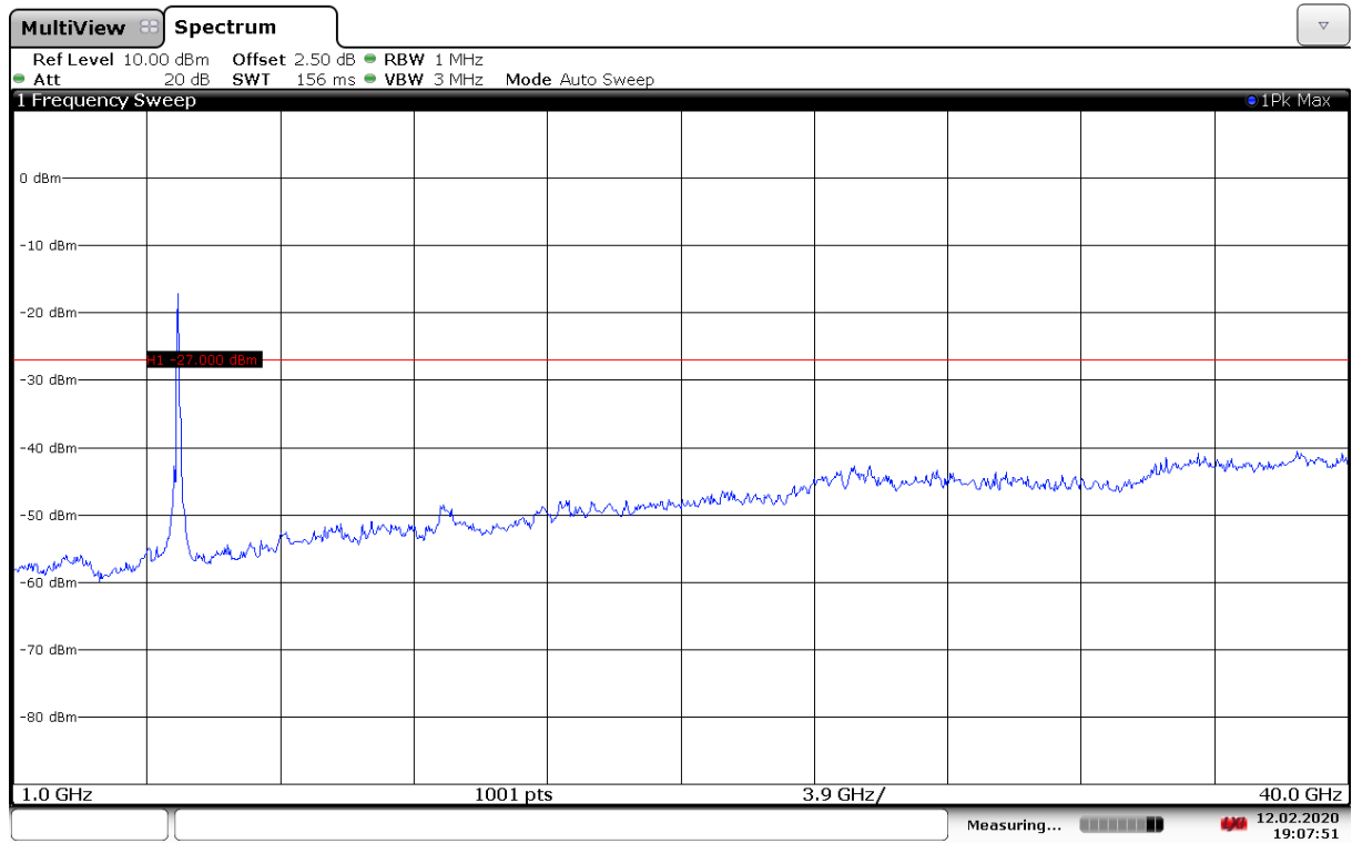
Fig. 68 Conducted Spurious Emission (802.11ax-HE40-RU242-right, Ch159, 1 GHz-40 GHz)
