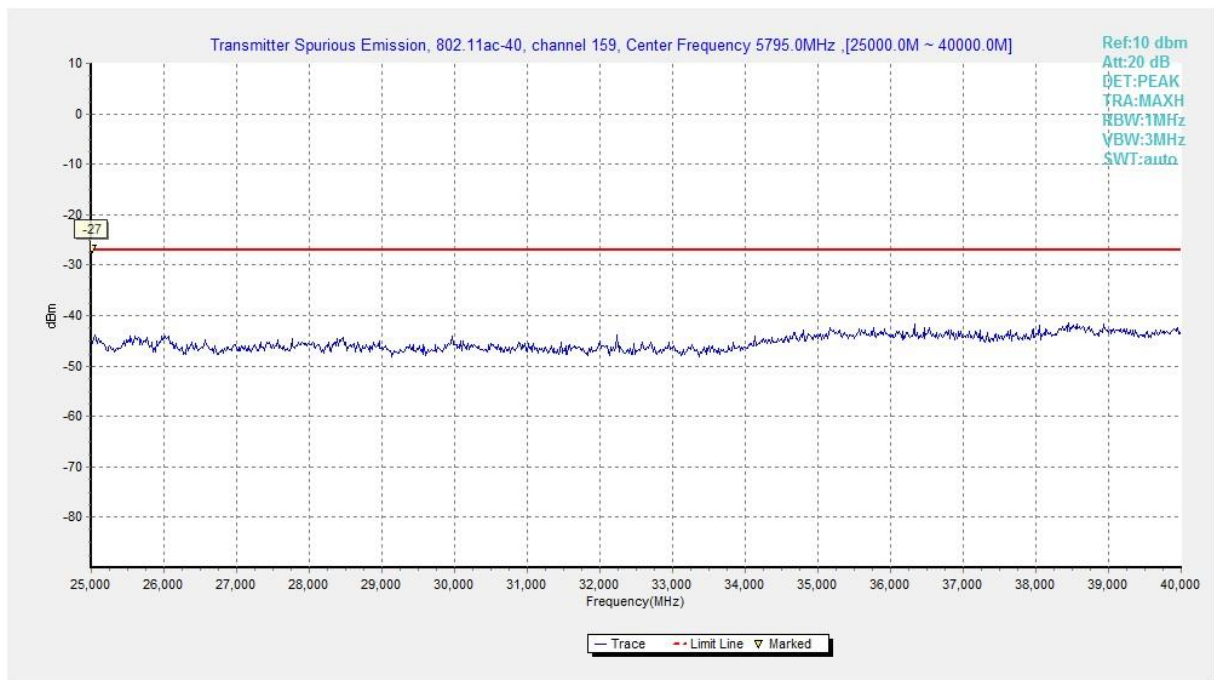
Fig. 122 Conducted Spurious Emission (802.11ac-HT40, Ch159, 25 GHz-40 GHz)
