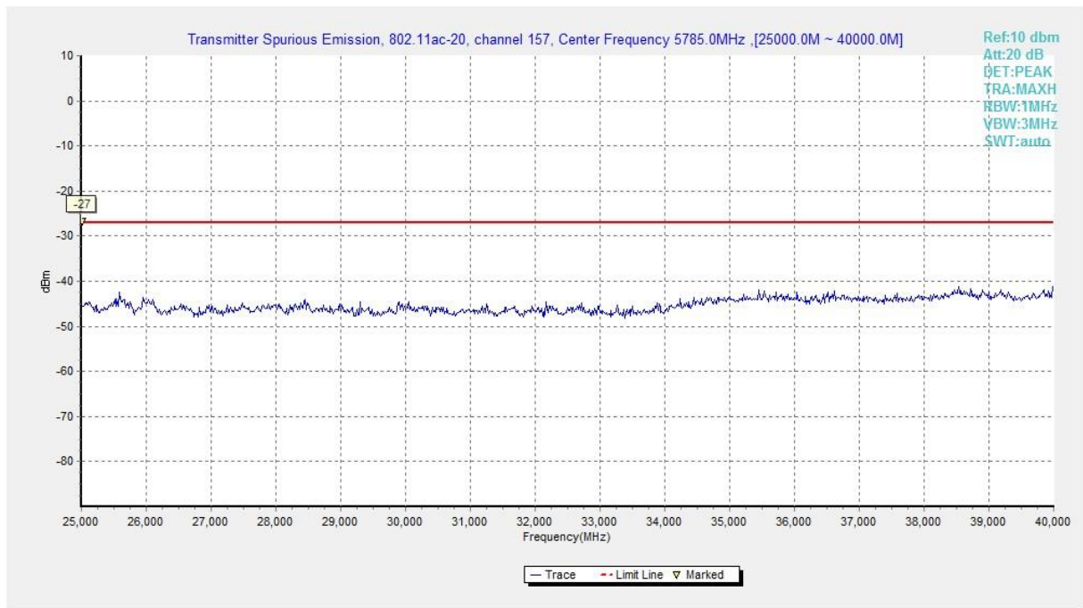
Fig. 102 Conducted Spurious Emission (802.11ac-HT20, Ch157, 25 GHz-40 GHz)
