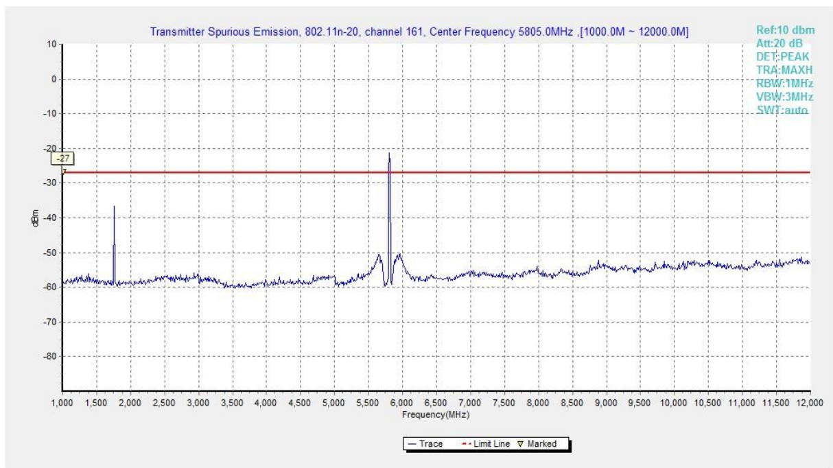
Fig. 92 Conducted Spurious Emission (802.11n-HT20, Ch161, 1 GHz -12 GHz)
