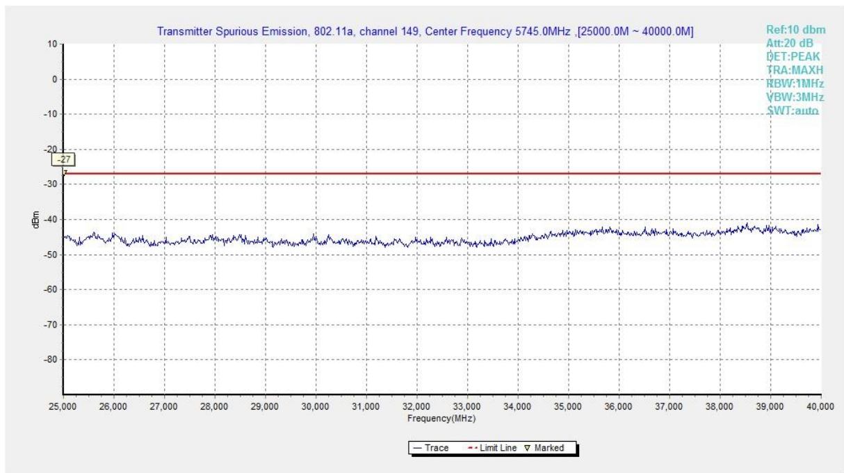
Fig. 74 Conducted Spurious Emission (802.11a, Ch149, 25 GHz-40 GHz)
