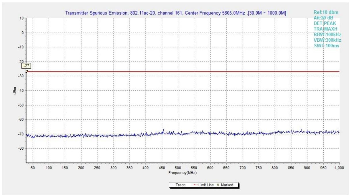
Fig. 103 Conducted Spurious Emission (802.11ac-HT20, Ch161, 30 MHz-1 GHz)
