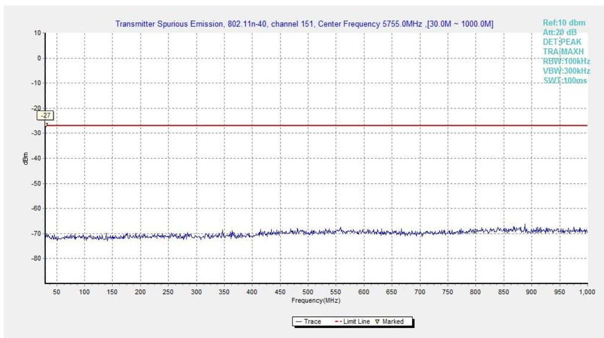
Fig. 107 Conducted Spurious Emission (802.11n-HT40, Ch151, 30 MHz-1 GHz)
