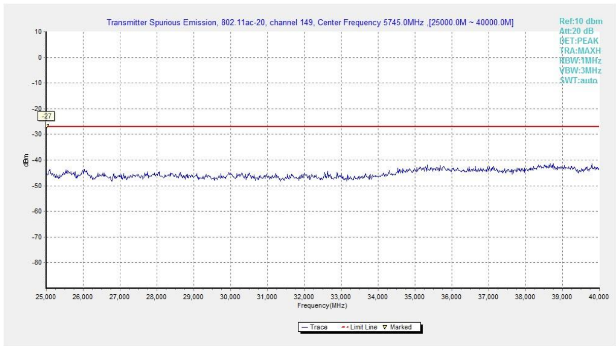
Fig. 98 Conducted Spurious Emission (802.11ac-HT20, Ch149, 25 GHz-40 GHz)
