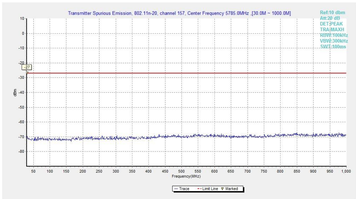
Fig. 87 Conducted Spurious Emission (802.11n-HT20, Ch157, 30 MHz-1 GHz)
