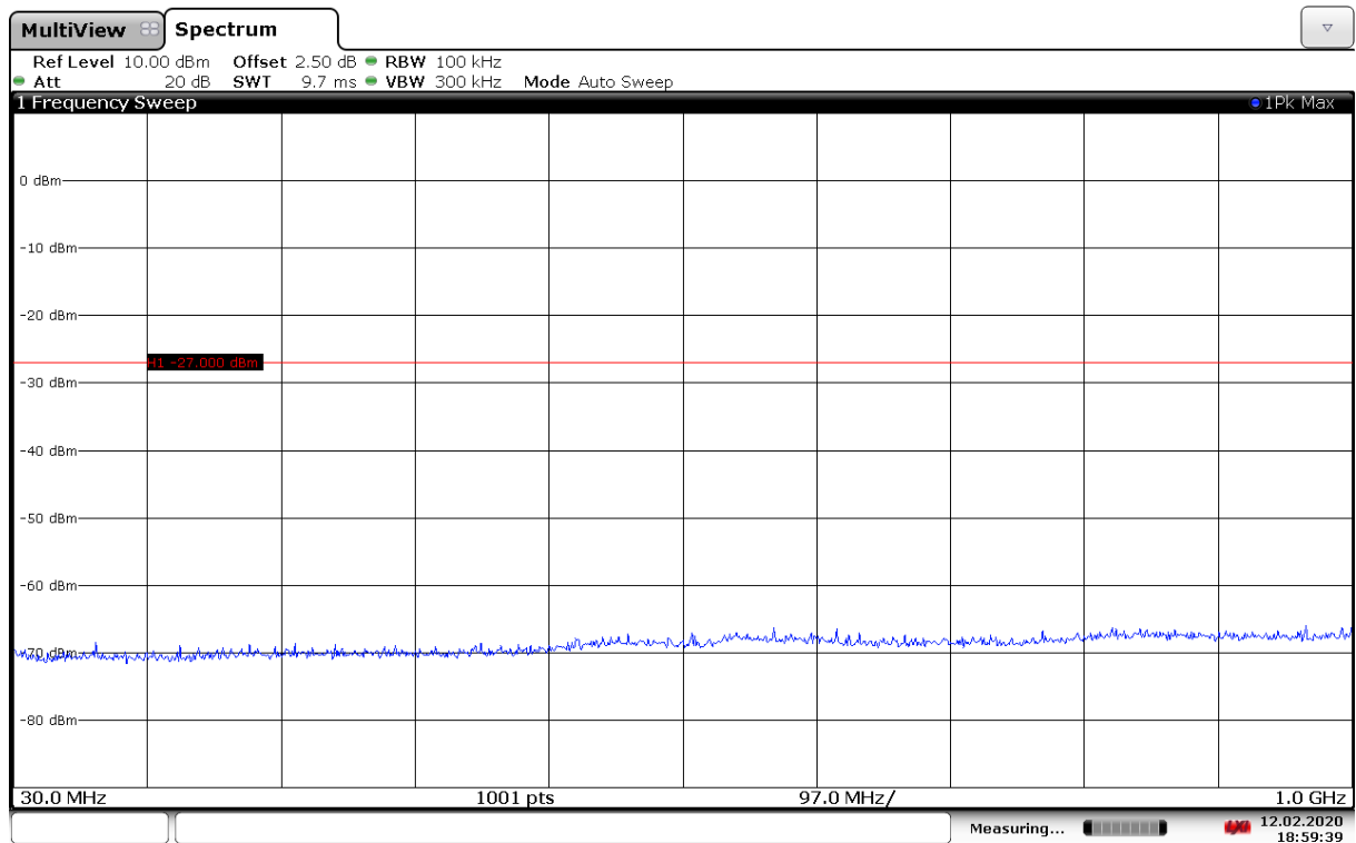
Fig. 65 Conducted Spurious Emission (802.11ax-HE40-RU242-right, Ch151, 30 MHz-1 GHz)
