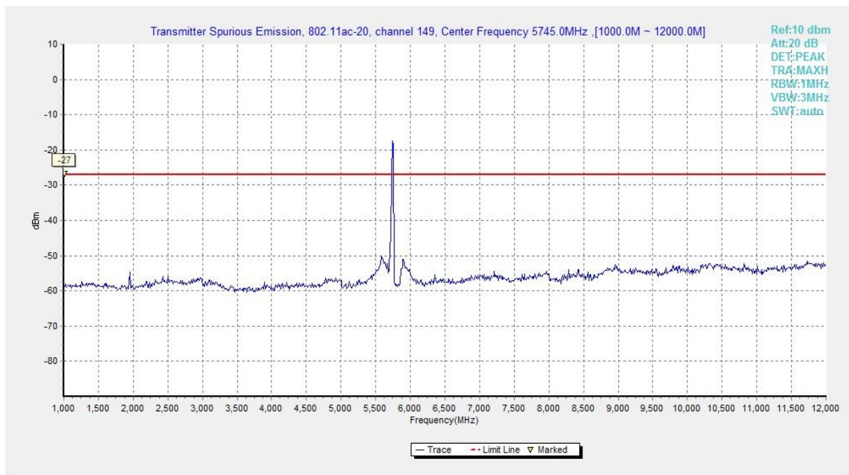
Fig. 96 Conducted Spurious Emission (802.11ac-HT20, Ch149, 1 GHz -12 GHz)
