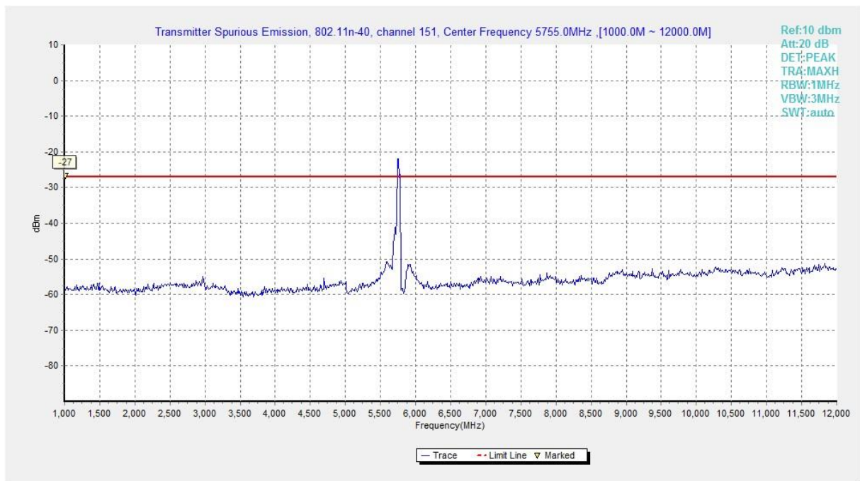
Fig. 108 Conducted Spurious Emission (802.11n-HT40, Ch151, 1 GHz -12 GHz)
