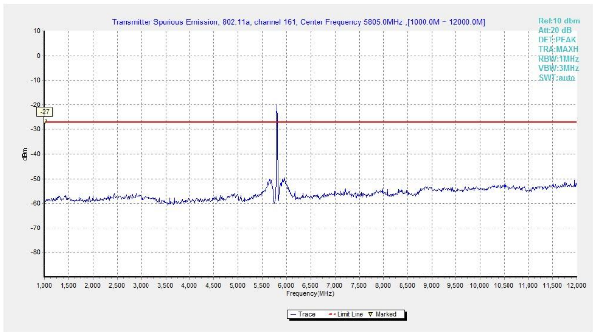
Fig. 80 Conducted Spurious Emission (802.11a, Ch161, 1 GHz -12 GHz)
