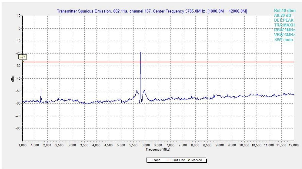
Fig. 76 Conducted Spurious Emission (802.11a, Ch157, 1 GHz -12 GHz)
