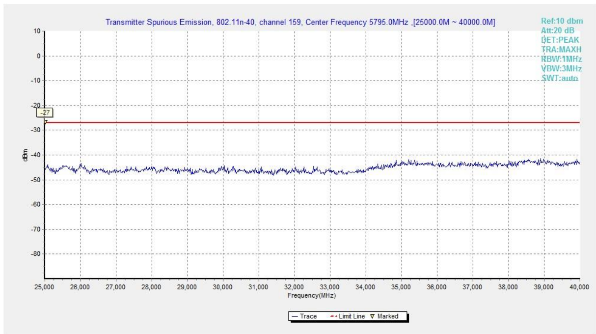
Fig. 114 Conducted Spurious Emission (802.11n-HT40, Ch159, 25 GHz-40 GHz)
