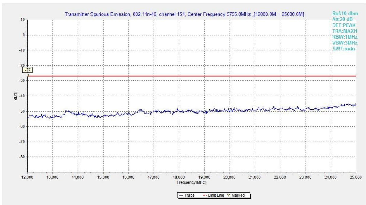
Fig. 109 Conducted Spurious Emission (802.11n-HT40, Ch151, 12 GHz-25 GHz)
