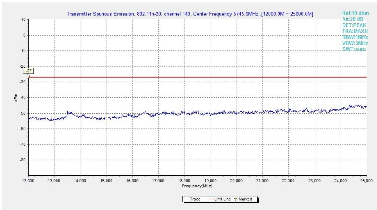
Fig. 85 Conducted Spurious Emission (802.11n-HT20, Ch149, 12 GHz-25 GHz)
