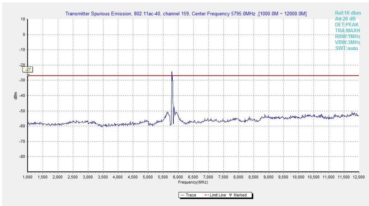
Fig. 120 Conducted Spurious Emission (802.11ac-HT40, Ch159, 1 GHz -12 GHz)
