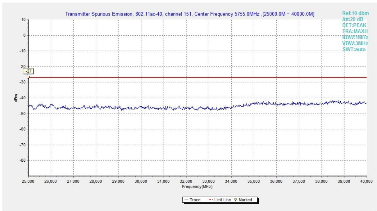
Fig. 118 Conducted Spurious Emission (802.11ac-HT40, Ch151, 25 GHz-40 GHz)
