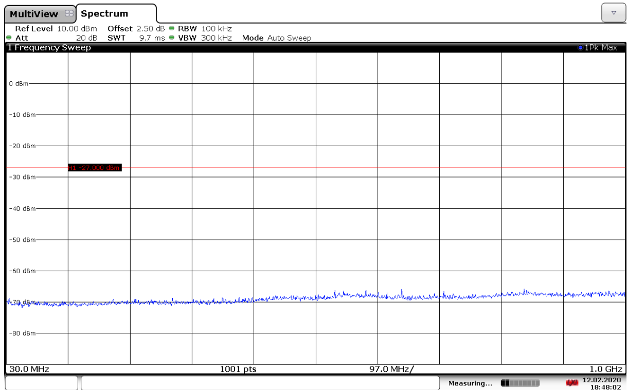
Fig. 133 Conducted Spurious Emission (802.11ax-HE40-RU242-right, Ch151, 30 MHz-1 GHz)
