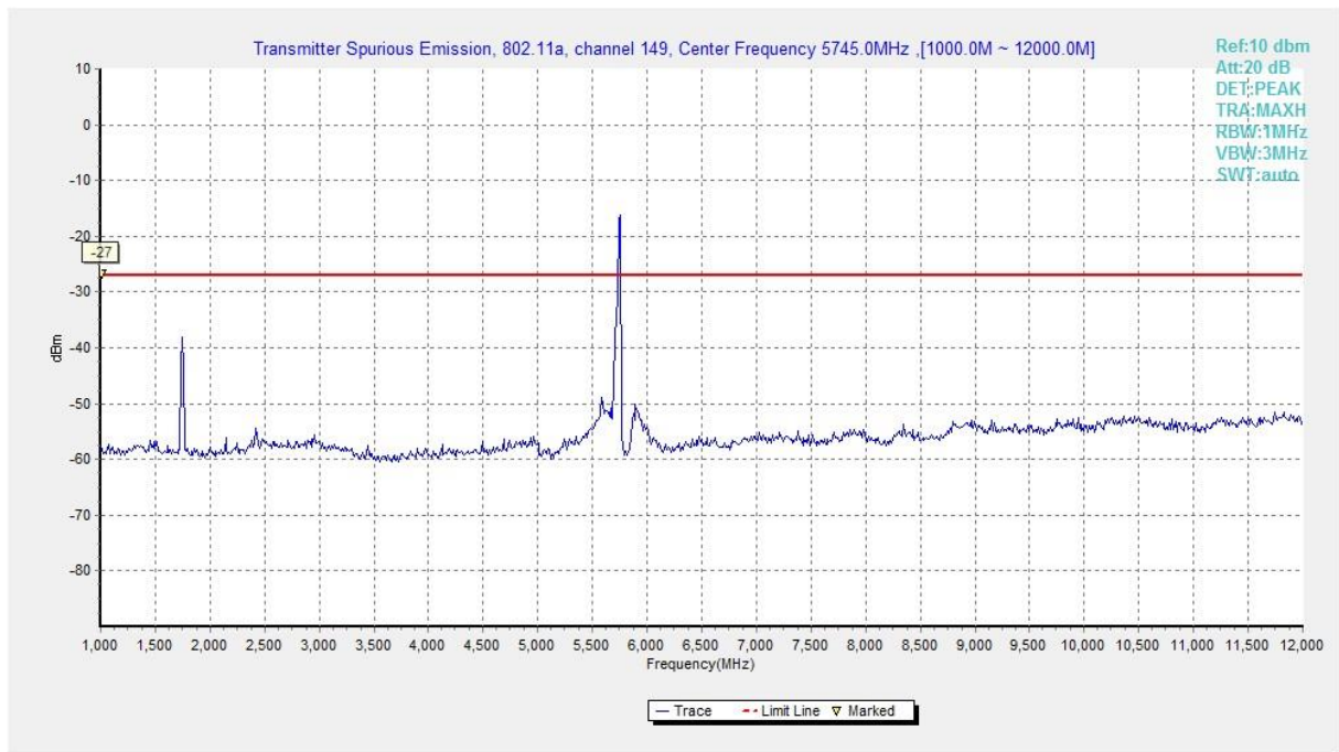
Fig. 72 Conducted Spurious Emission (802.11a, Ch149, 1 GHz -12 GHz)
