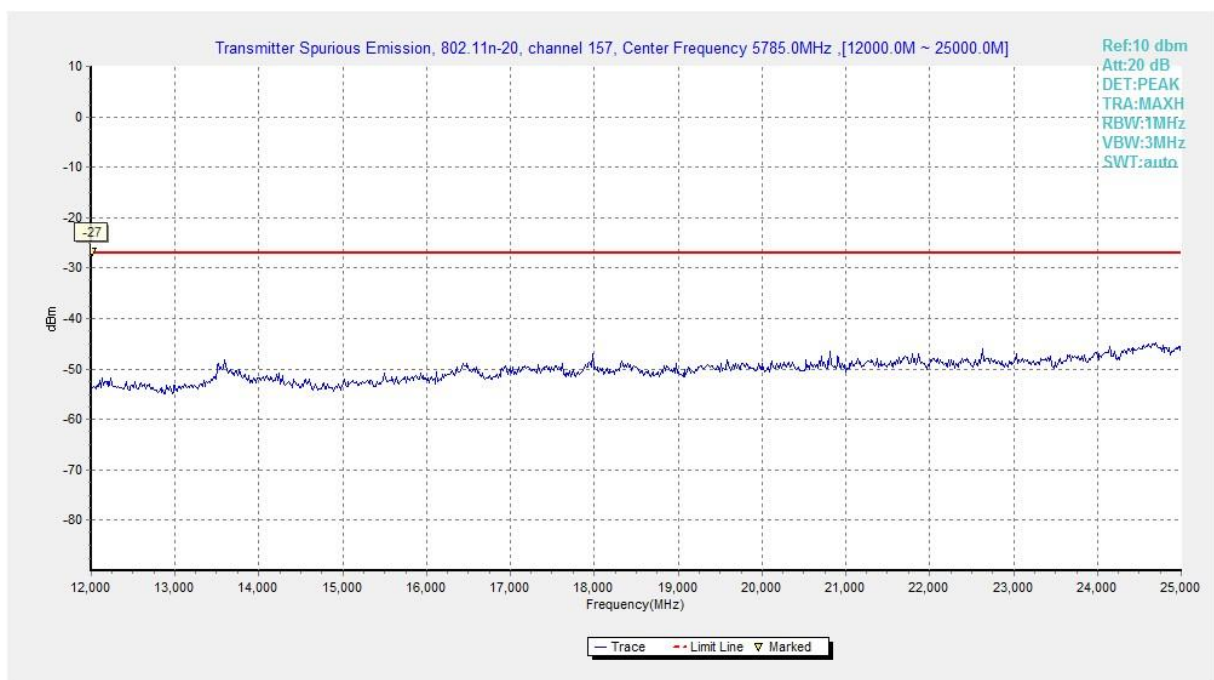
Fig. 89 Conducted Spurious Emission (802.11n-HT20, Ch157, 12 GHz-25 GHz)
