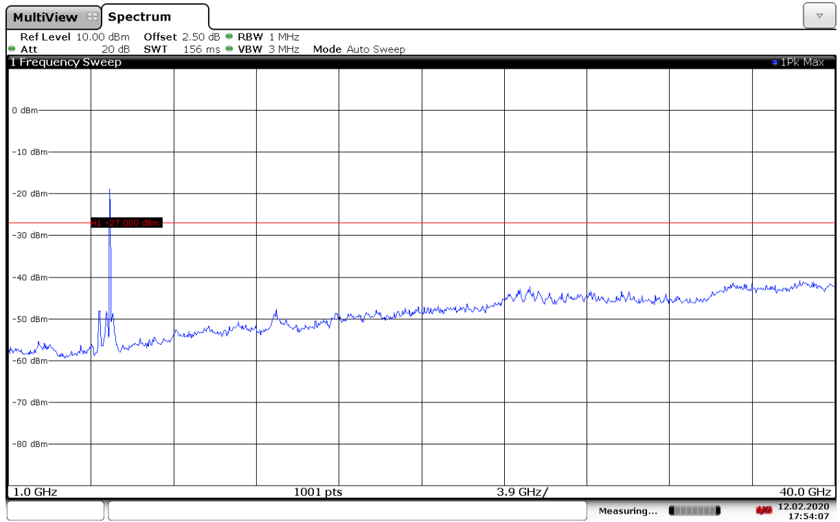
Fig. 130 Conducted Spurious Emission (802.11ax-HE20-RU106-right, Ch157, 1 GHz-40 GHz)
