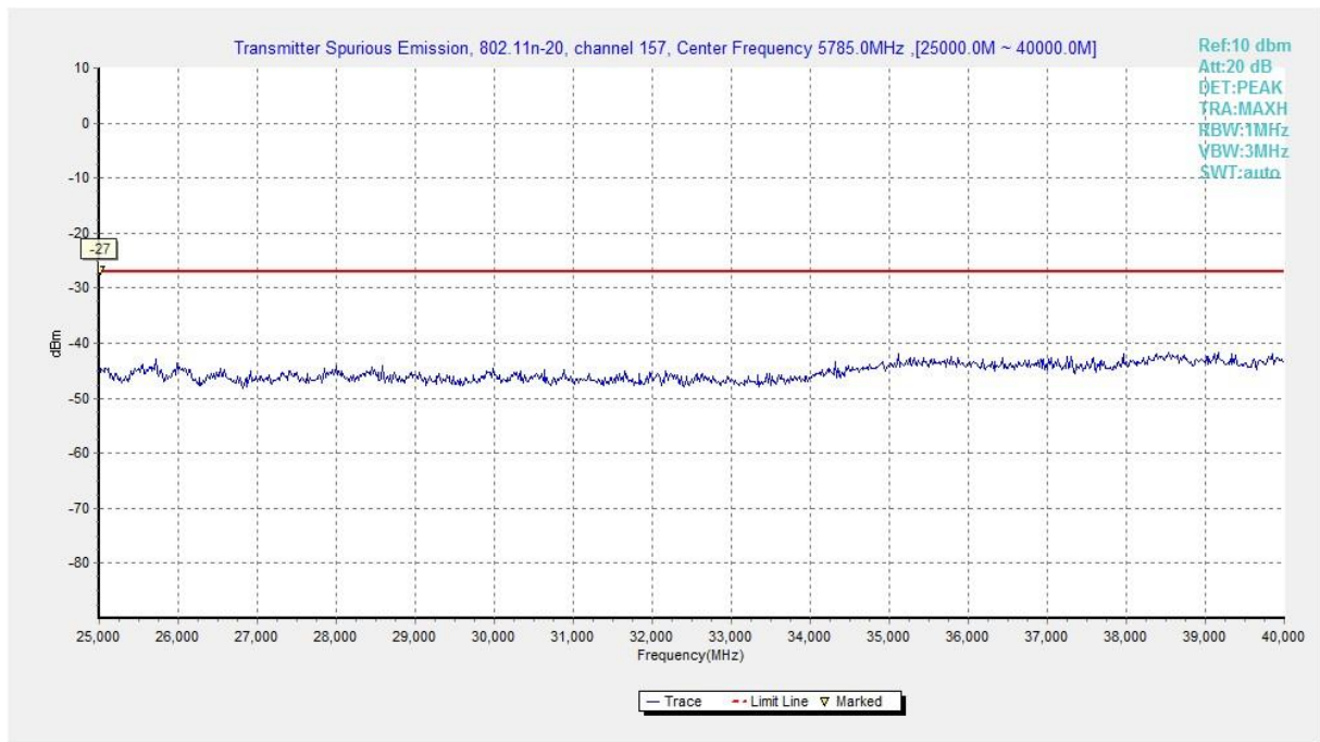
Fig. 90 Conducted Spurious Emission (802.11n-HT20, Ch157, 25 GHz-40 GHz)
