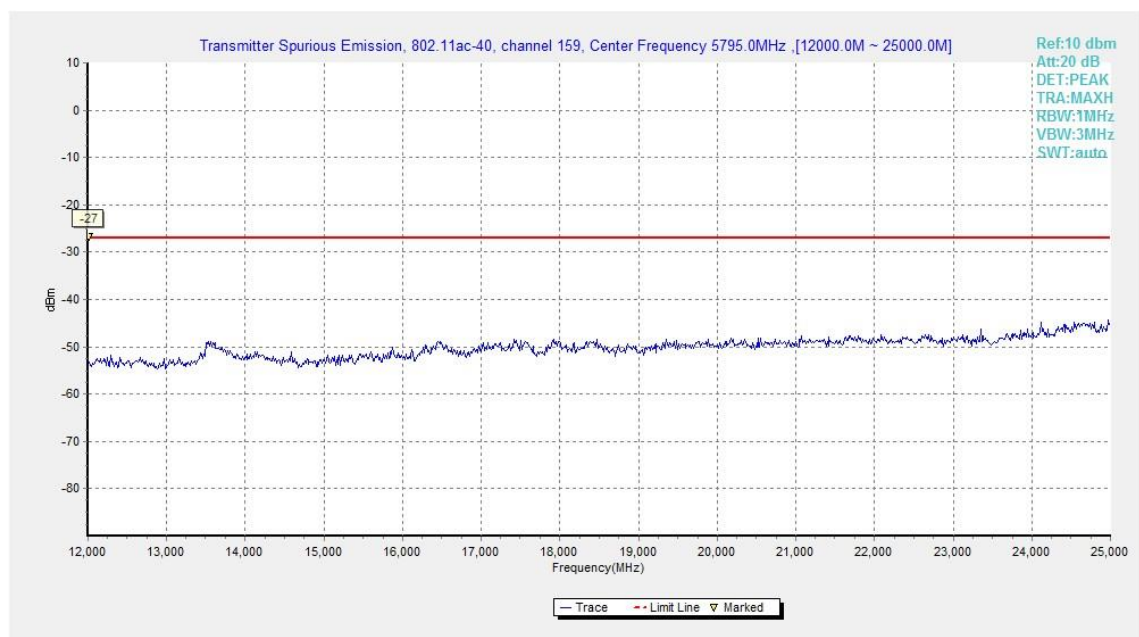
Fig. 121 Conducted Spurious Emission (802.11ac-HT40, Ch159, 12 GHz-25 GHz)
