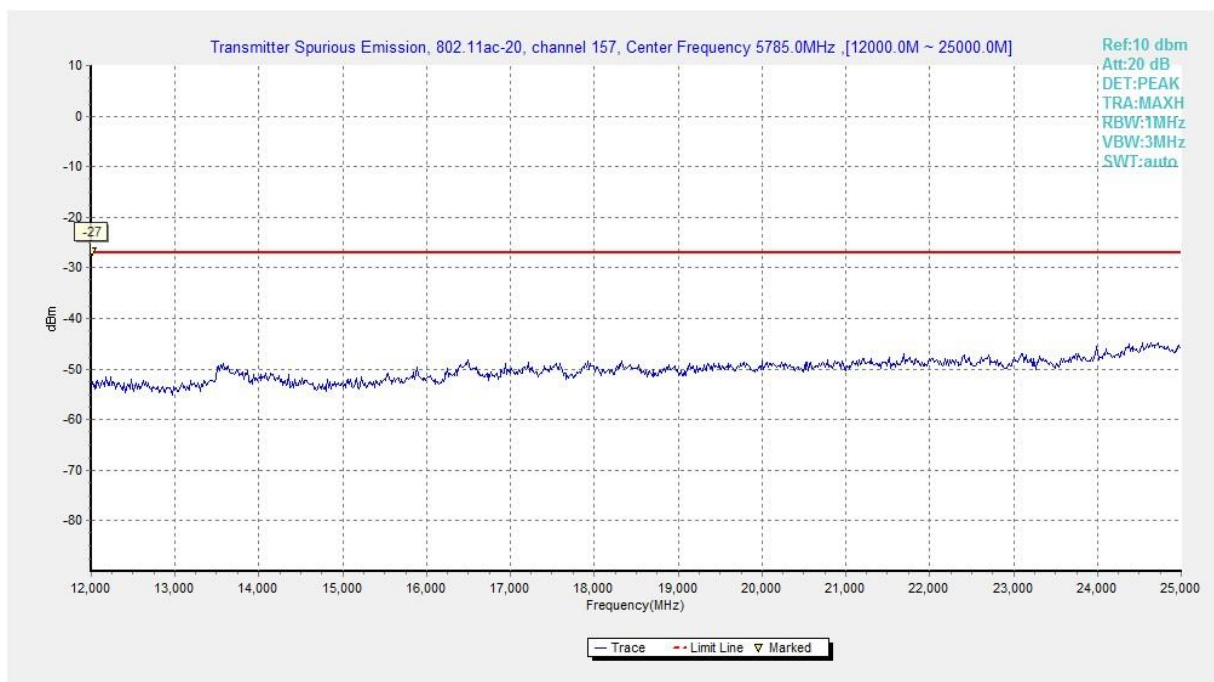
Fig. 101 Conducted Spurious Emission (802.11ac-HT20, Ch157, 12 GHz-25 GHz)
