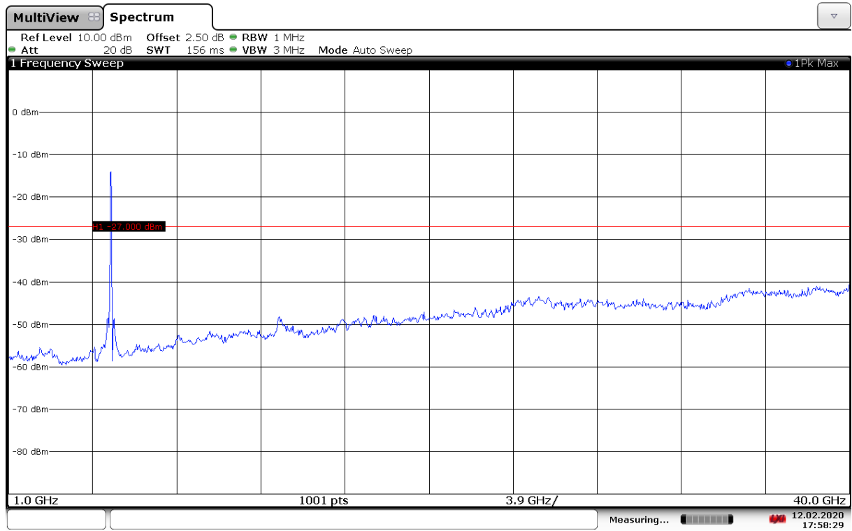
Fig. 128 Conducted Spurious Emission (802.11ax-HE20-RU106-right, Ch149, 1 GHz-40 GHz)
