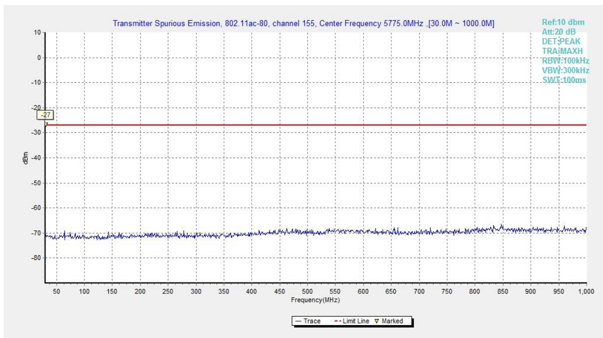
Fig. 123 Conducted Spurious Emission (802.11ac-HT80, Ch155, 30 MHz-1 GHz)
