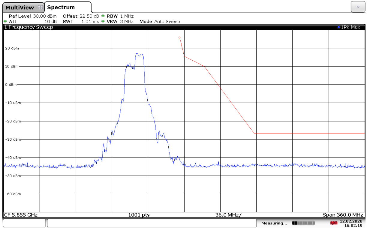
Fig. 178 Band Edges (802.11ax-HE20-RU106-right, 5805MHz)
