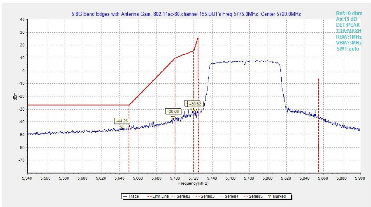
Fig. 149 Band Edges (802.11ac-HT80, 5775MHz)
