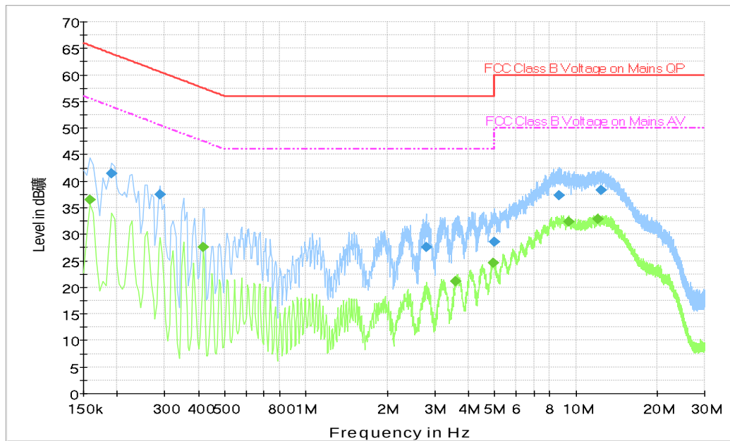
Fig. 201 AC Powerline Conducted Emission-802.11a EUT4(M2001J2G)+AE1+AE3+AE6
