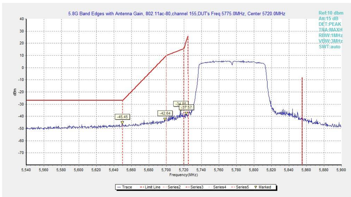
Fig. 171 Band Edges (802.11ac-HT80, 5775MHz)
