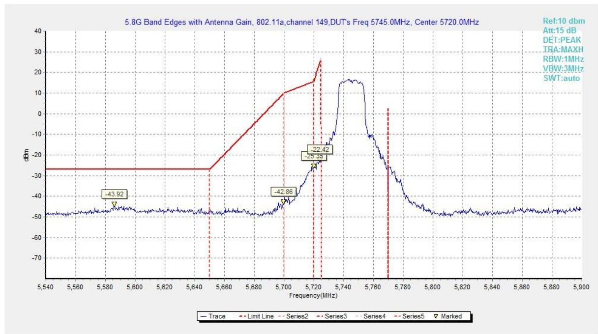
Fig. 139 Band Edges (802.11a, 5745MHz)
