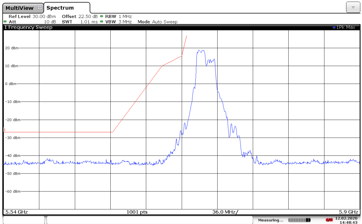
Fig. 155 Band Edges (802.11ax-HE20-RU106-left, 5745MHz)
