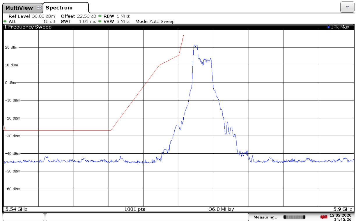
Fig. 153 Band Edges (802.11ax-HE20-RU52-left, 5745MHz)
