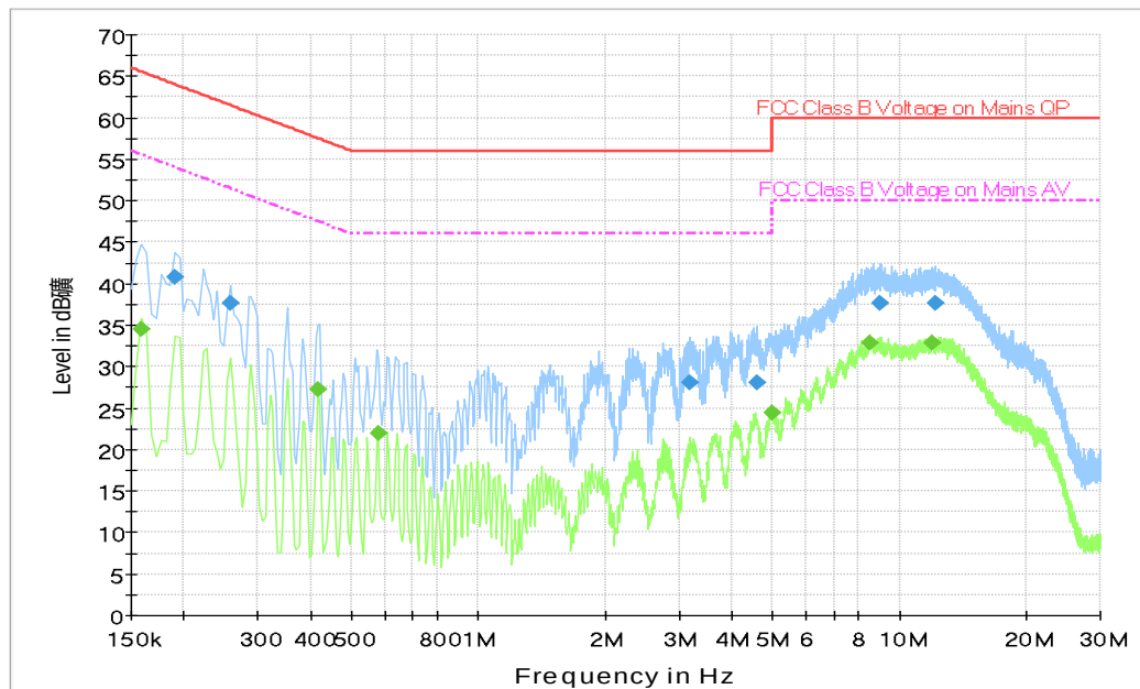
Fig. 202 AC Powerline Conducted Emission-Idle EUT4(M2001J2G)+AE1+AE3+AE6
