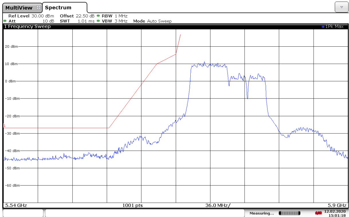
Fig. 181 Band Edges (802.11ax-HE80-RU484-left, 5775MHz)
