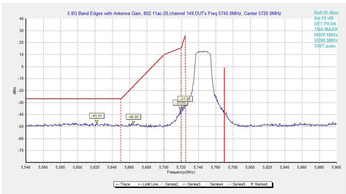
Fig. 165 Band Edges (802.11ac-HT20, 5745MHz)
