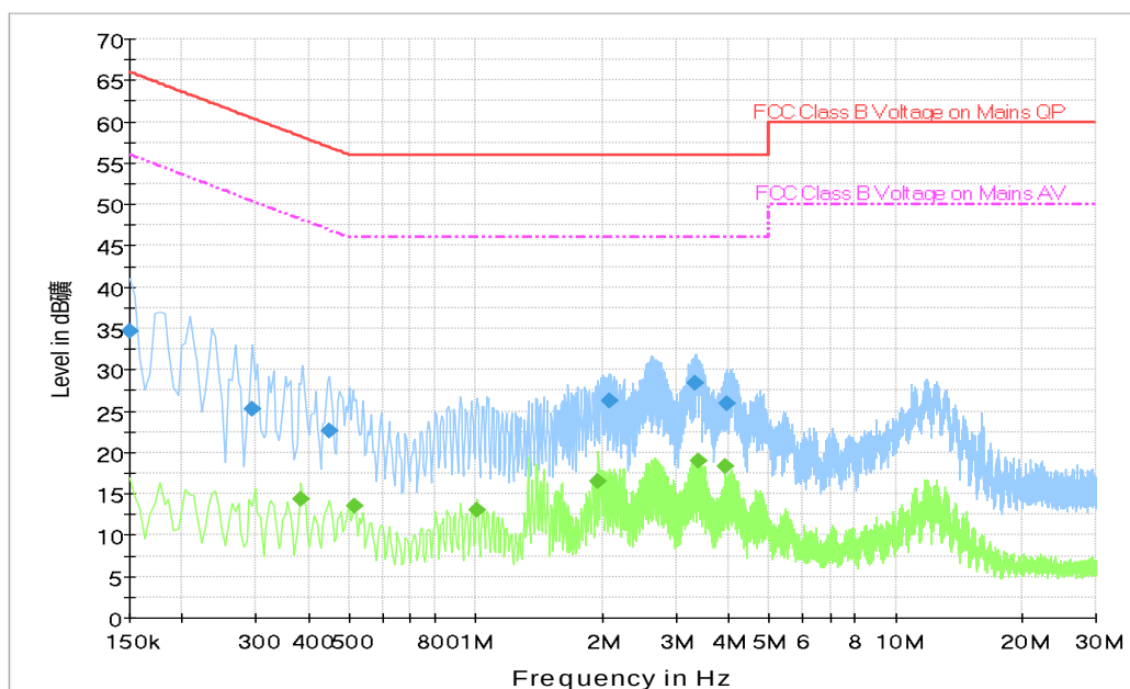
Fig. 204 AC Powerline Conducted Emission-Idle EUT43(M2001J1G)+AE11+AE13+AE16
