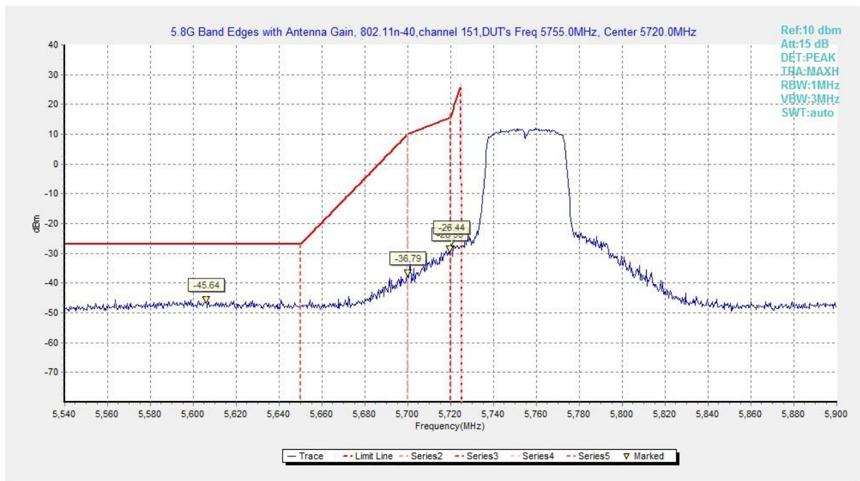
Fig. 145 Band Edges (802.11n-HT40, 5755MHz)
