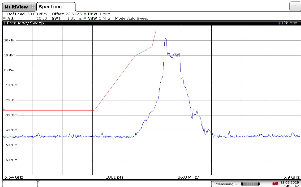
Fig. 173 Band Edges (802.11ax-HE20-RU26-left, 5745MHz)
