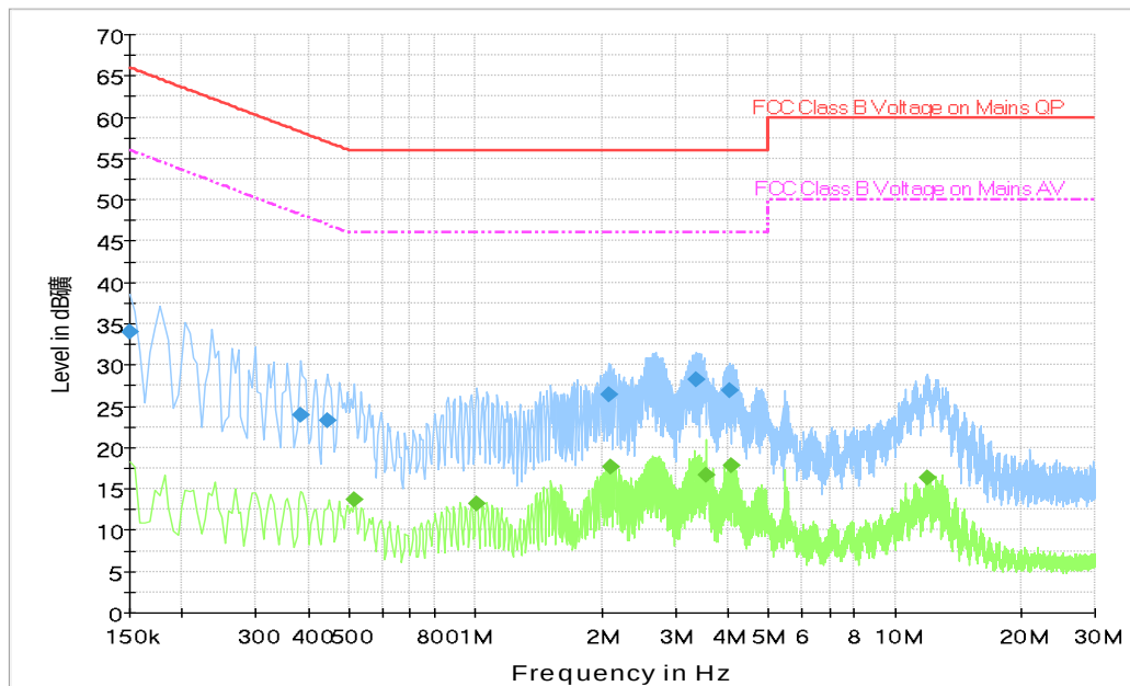
Fig. 203 AC Powerline Conducted Emission-802.11a EUT43(M2001J1G)+AE11+AE13+AE16
