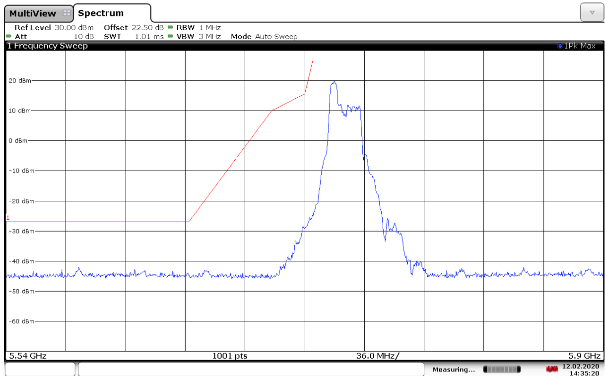
Fig. 175 Band Edges (802.11ax-HE20-RU52-left, 5745MHz)
