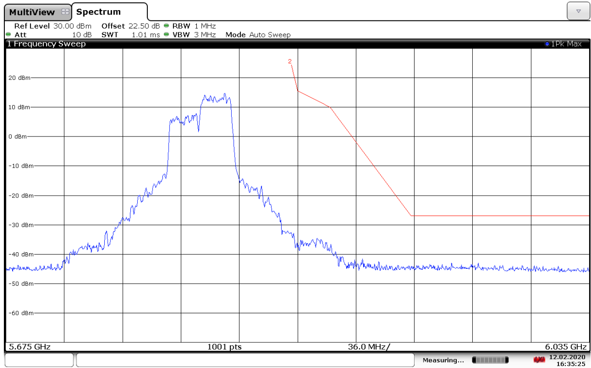
Fig. 158 Band Edges (802.11ax-HE40-RU242-right, 5795MHz)
