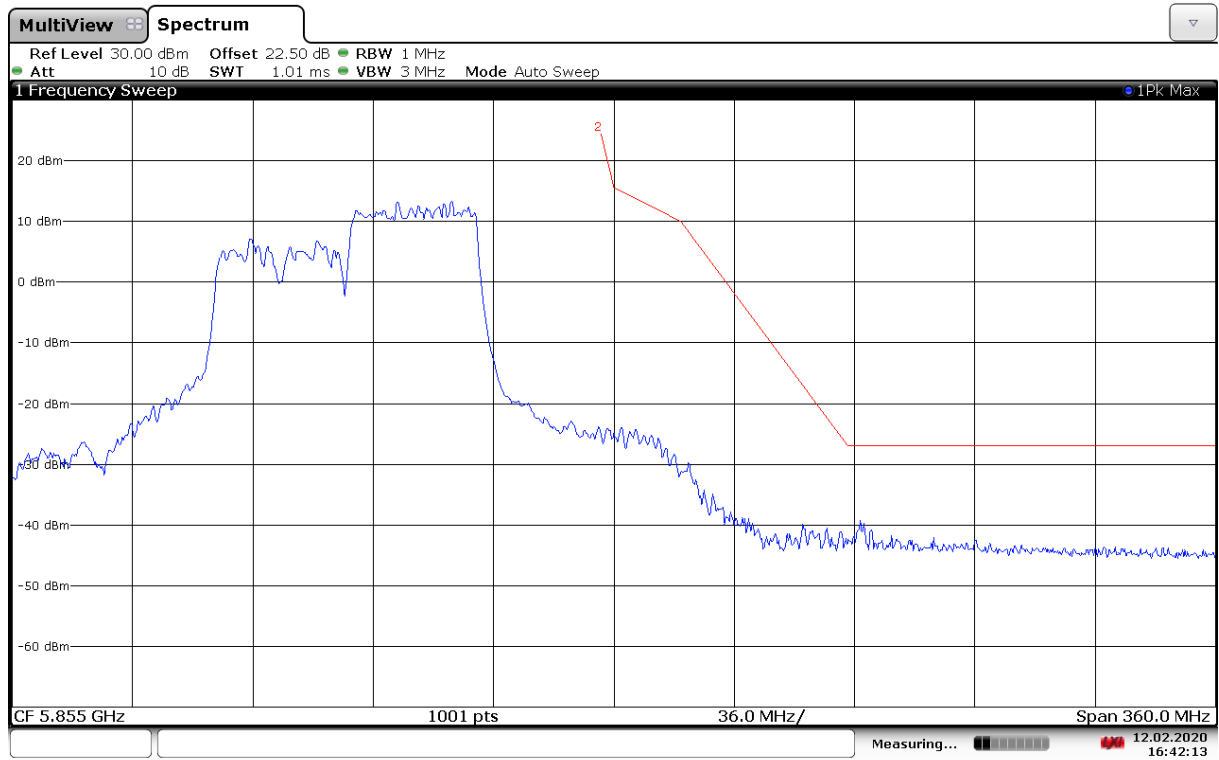
Fig. 160 Band Edges (802.11ax-HE40-RU484-right, 5775MHz)
