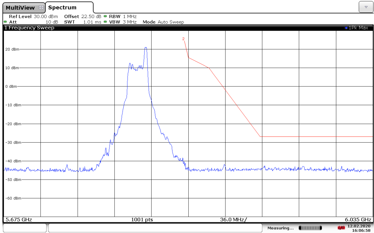
Fig. 174 Band Edges (802.11ax-HE20-RU26-right, 5805MHz)
