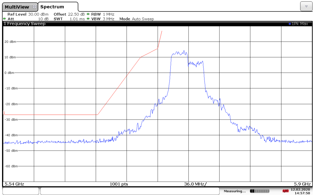
Fig. 179 Band Edges (802.11ax-HE40-RU242-left, 5755MHz)
