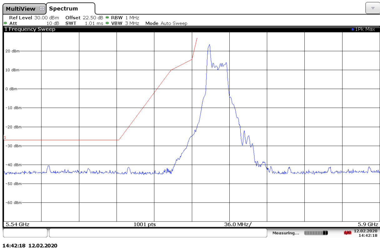
Fig. 151 Band Edges (802.11ax-HE20-RU26-left, 5745MHz)
