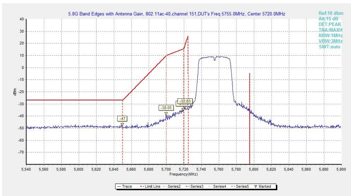
Fig. 169 Band Edges (802.11ac-HT40, 5755MHz)
