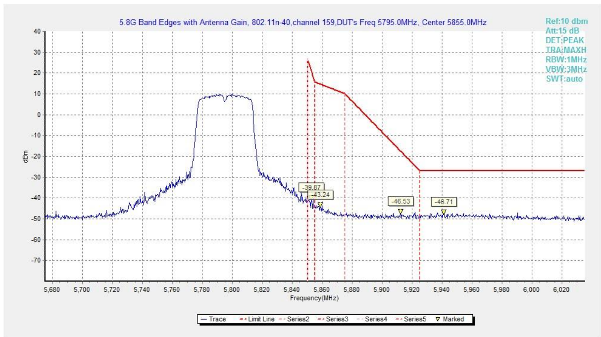
Fig. 168 Band Edges (802.11n-HT40, 5795MHz)
