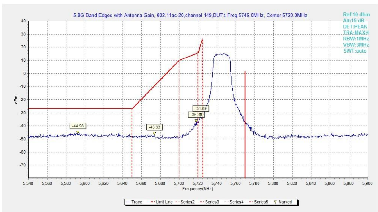
Fig. 143 Band Edges (802.11ac-HT20, 5745MHz)
