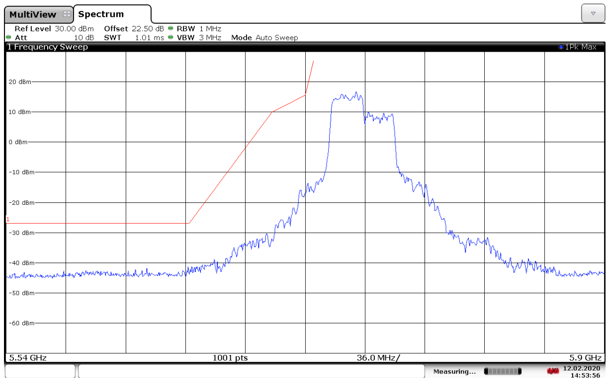
Fig. 157 Band Edges (802.11ax-HE40-RU242-left, 5755MHz)
