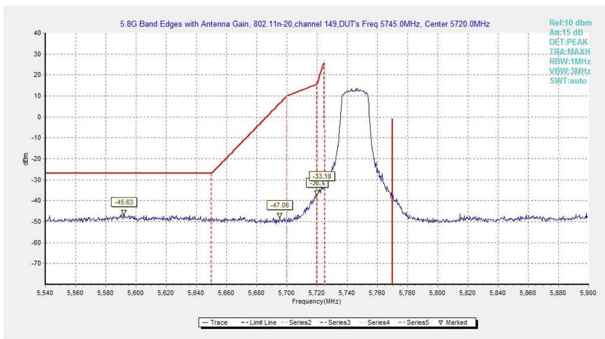
Fig. 163 Band Edges (802.11n-HT20, 5745MHz)
