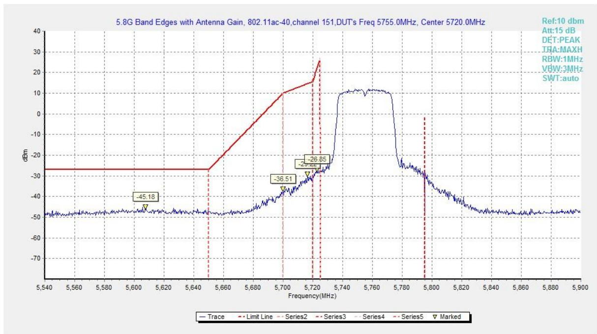
Fig. 147 Band Edges (802.11ac-HT40, 5755MHz)
