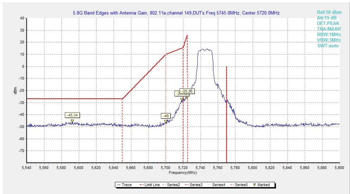
Fig. 161 Band Edges (802.11a, 5745MHz)
