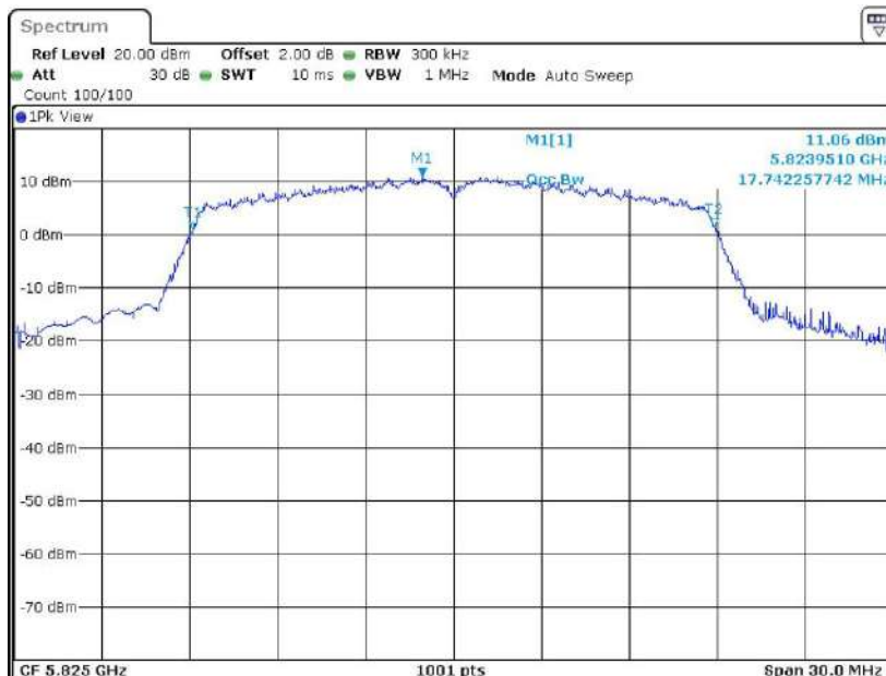
11N20SISO Ant1 5825
