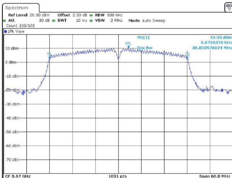
11N40MIMO Ant2 5670
