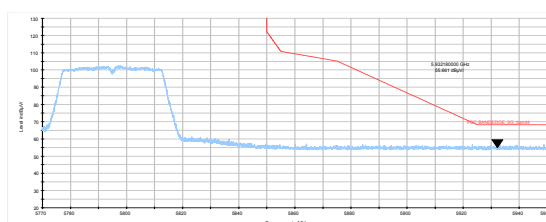
802.11n HT40-Channel 159: Peak
