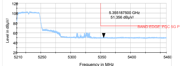
802.11n HT40-Channel 46: Peak
