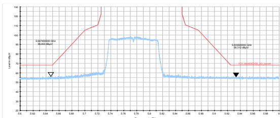
802.11ac VHT80- Channel 155: Peak
