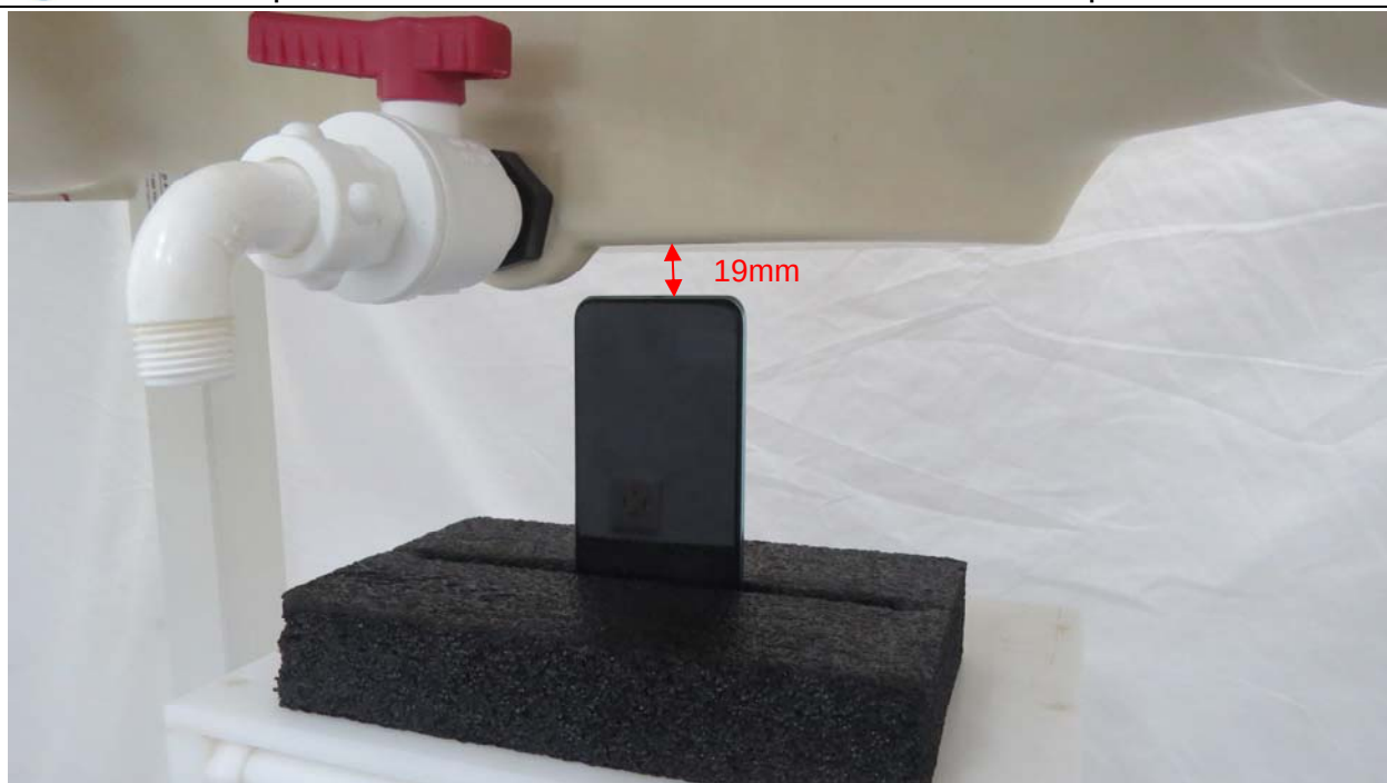
Picture 15: Bottom Edge, the distance from handset to the bottom of the Phantom is 19mm
