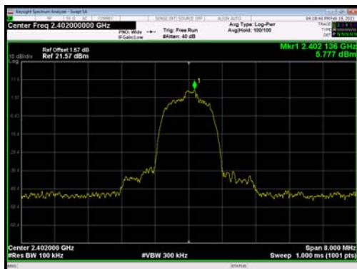
BT 2DH5 CH0, Carrier frequency (MHz): 2402
