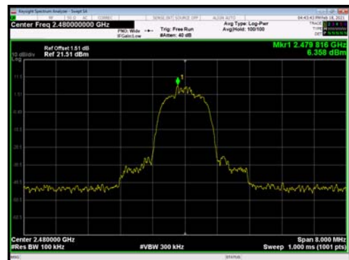
BT 2DH5 CH78, Carrier frequency (MHz): 2480
