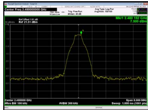
BT DH5 CH78, Carrier frequency (MHz): 2480
