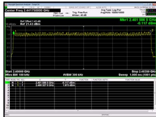
2DH5 2400 MHz – 2483.5 MHz
