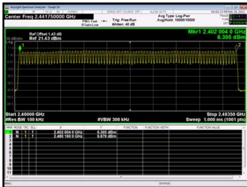
3DH5 2400 MHz – 2483.5 MHz
