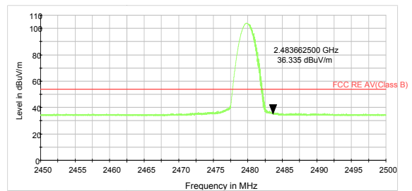
DH5-Channel 78: Average
