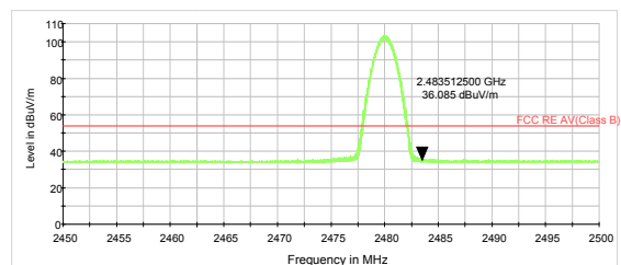
3DH5-Channel 78: Average
