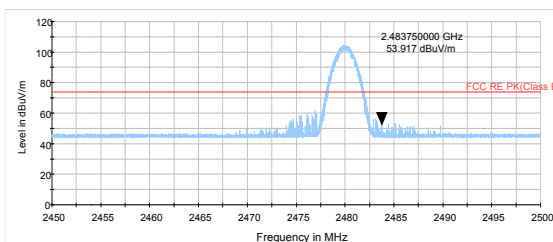
3DH5-Channel 78: Peak
