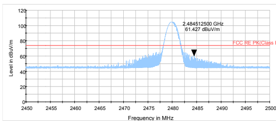
DH5-Channel 78: Peak
