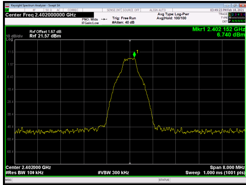
BT DH5 CH0, Carrier frequency (MHz): 2402
