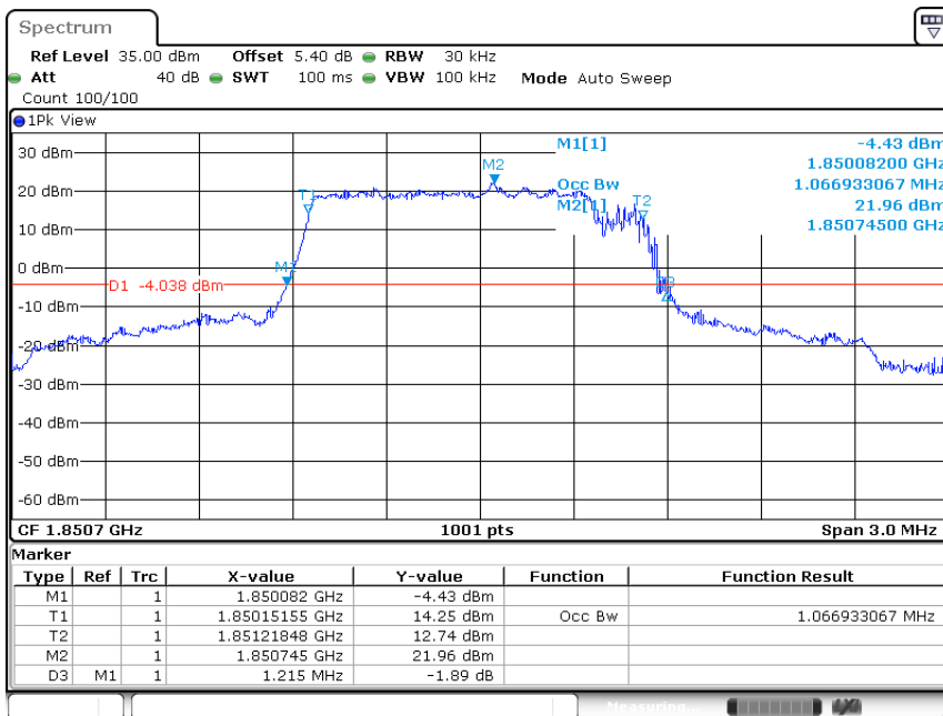
Band2-1.4MHz-QPSK-18607-6RB#0-1.067
