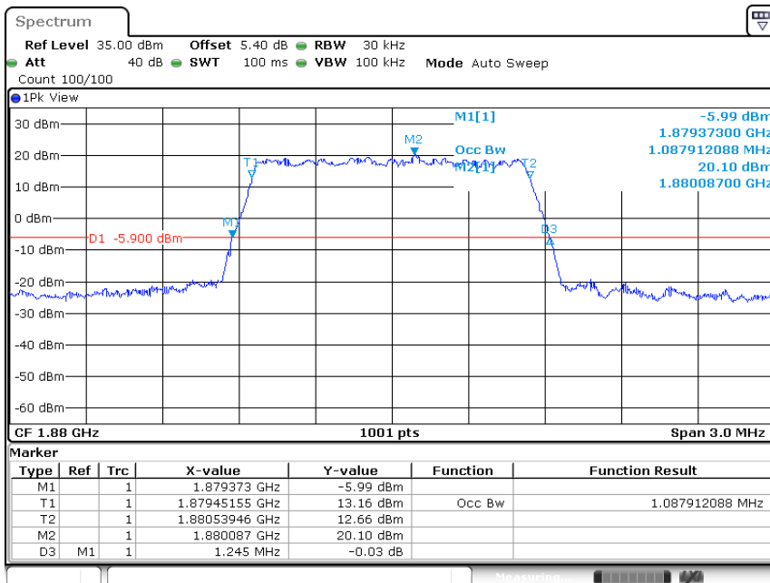
Band2-1.4MHz-QPSK-18900-6RB#0-1.088
