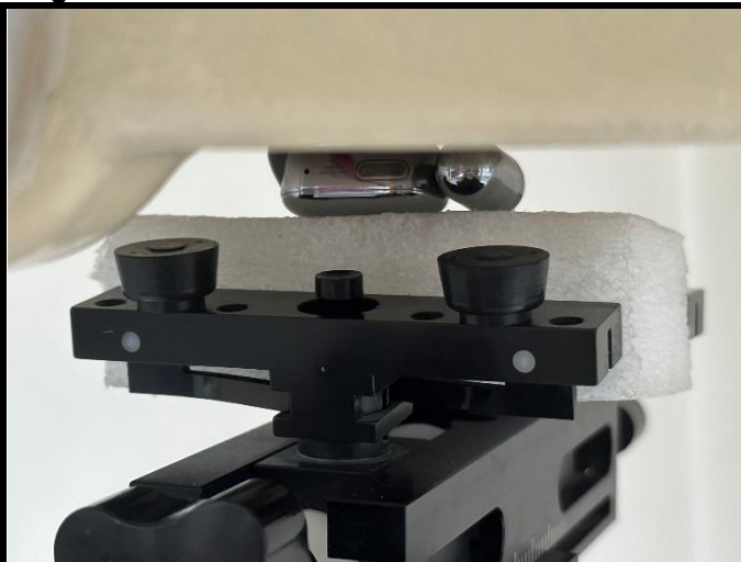
Test Position 1 (EUT with 0 cm Gap)
