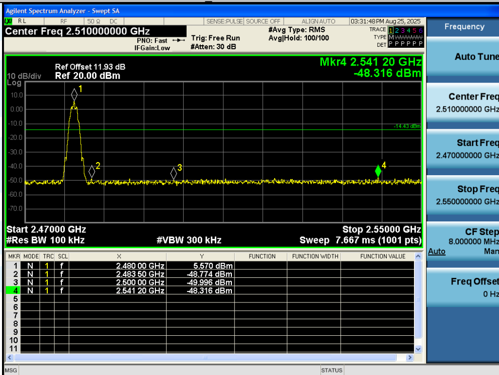
BLE_2M-Ant1-2480-PASS
