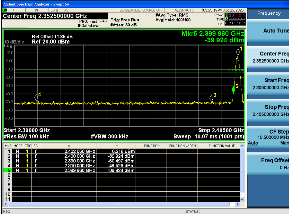
BLE_2M-Ant1-2402-PASS
