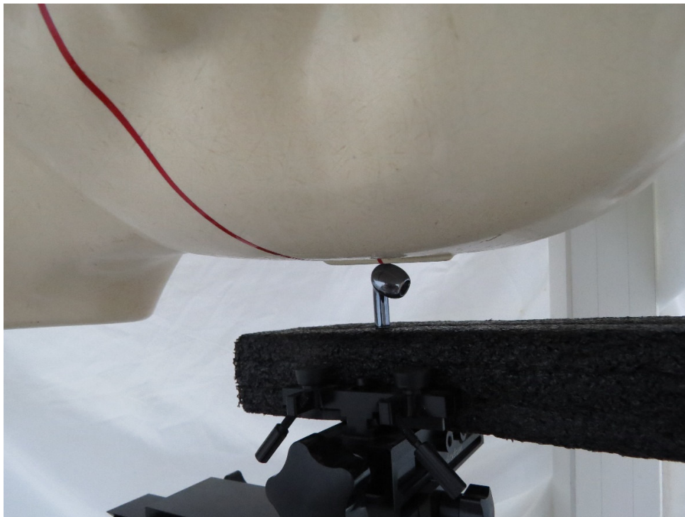
Picture 5: Left Side 5 Hand Touch Cheek Position
