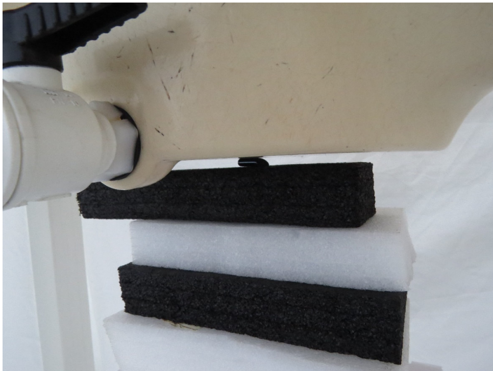
Picture 13: Back Side, the distance from EUT to the bottom of the Phantom is 0mm
