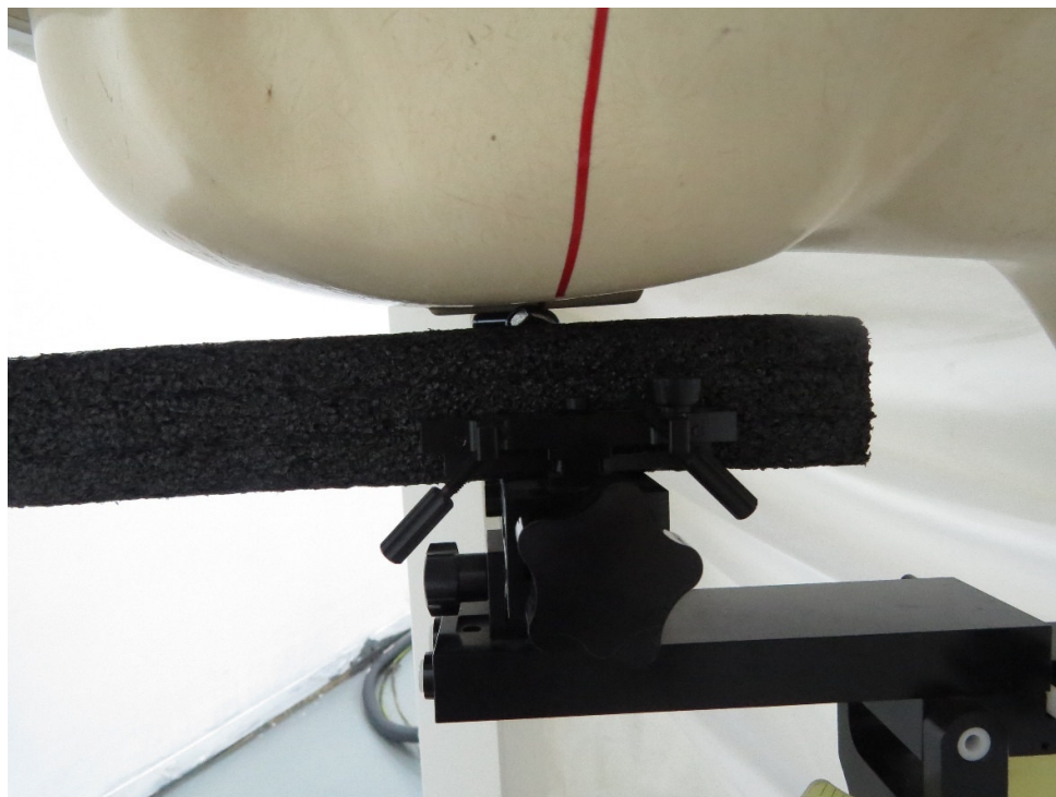
Picture 9: Right Side3 Hand Touch Cheek Position
