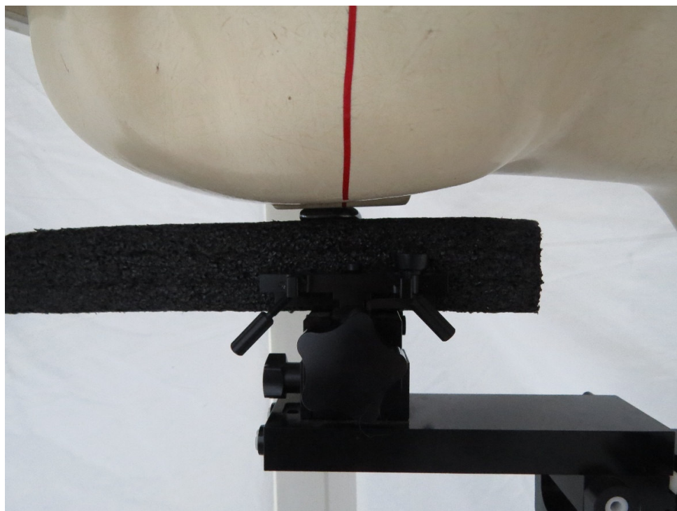
Picture 10: Right Side4 Hand Touch Cheek Position
