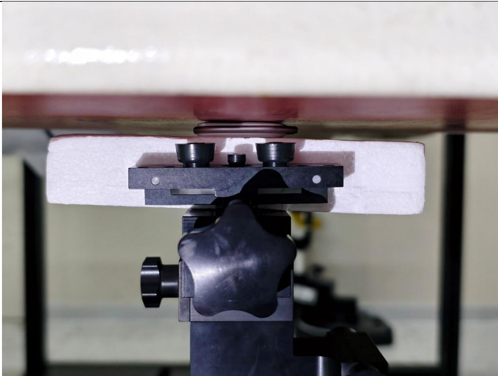
Body SAR Front side
