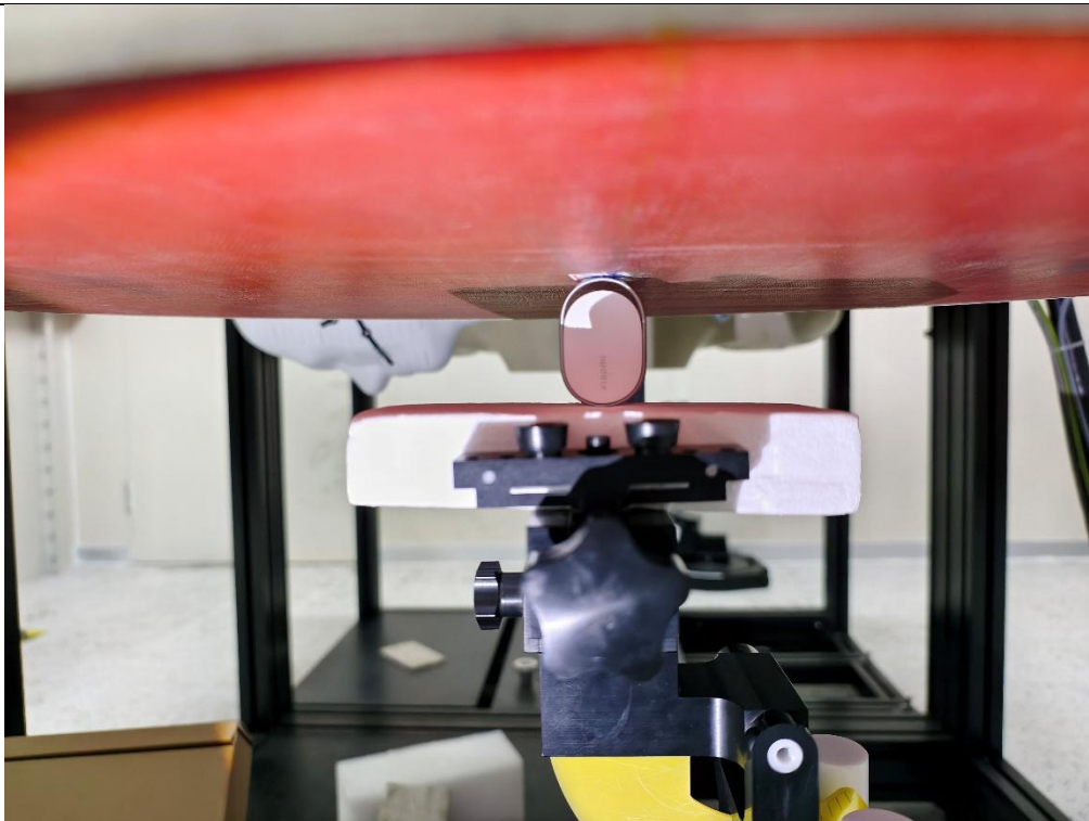
Body SAR Right side
