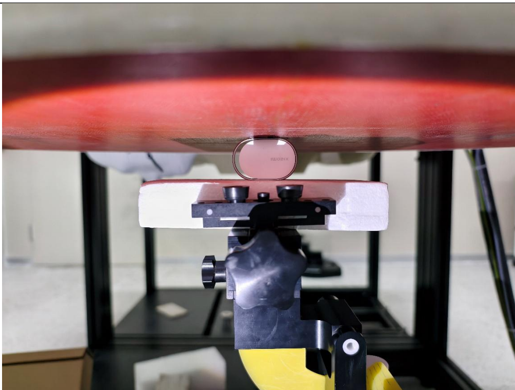
Body SAR Bottom side
