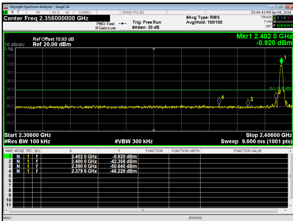
Band Edge Bluetooth LE(1M) 2402MHz Emission
