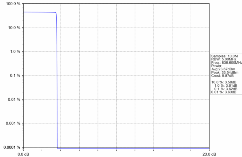
GSM850_GPRS_MCH_836.6MHz_4 TX Slots_NTNV
