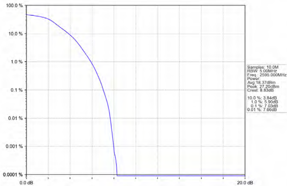
Band38_5MHz_QPSK_MCH_2595MHz_RB_25_0_NTNV
