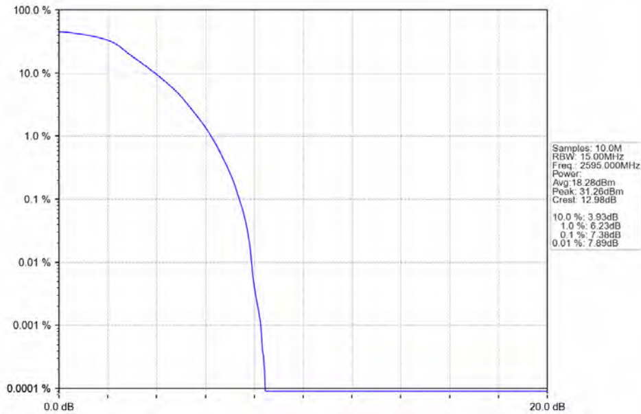
Band38_15MHz_QPSK_MCH_2595MHz_RB_75_0_NTNV
