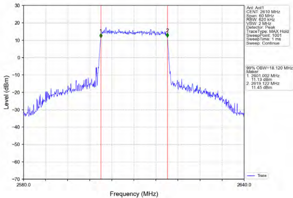
Band38_20MHz_64QAM_HCH_2610MHz_RB_100_0_NTNV
