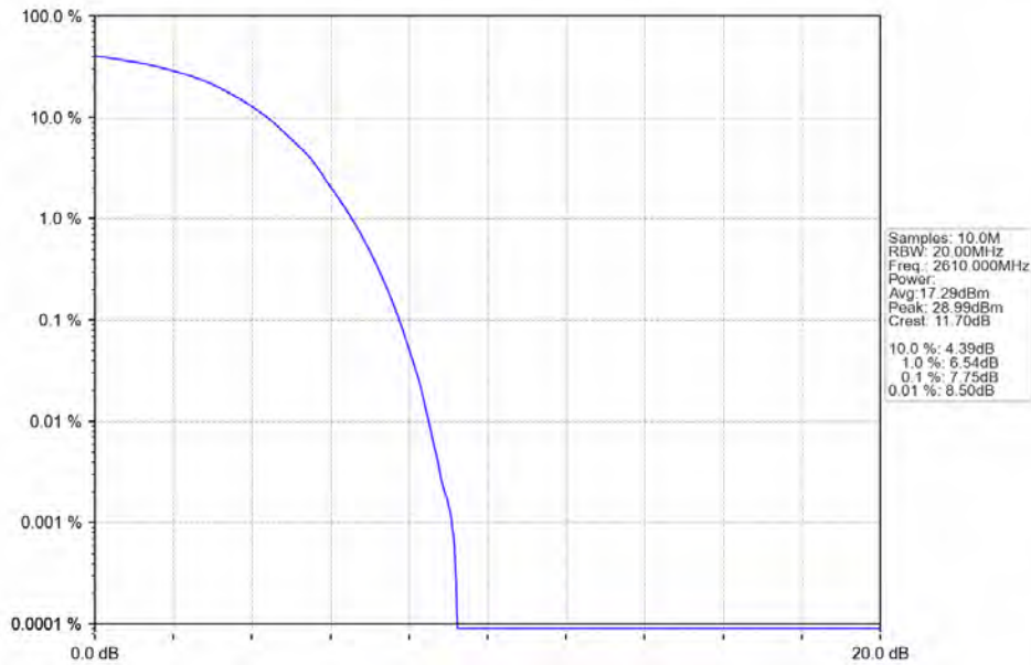
Band38_20MHz_64QAM_HCH_2610MHz_RB_100_0_NTNV
