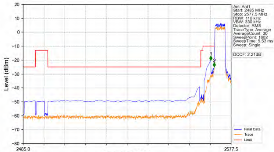
Band38_5MHz_QPSK_LCH_2572.5MHz_RB_25_0_NTNV
